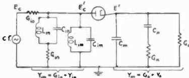
Fig. 11—Diode rectifier circuit with input and output circuits of corresponding admittance variation.
