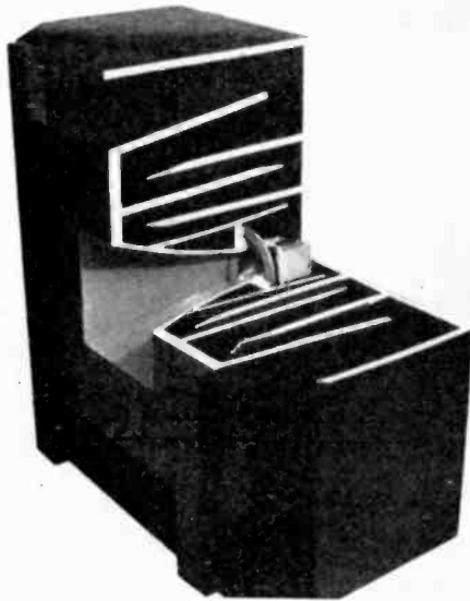
Fig. 7—Sectional view of the single-drive type of compound-horn loud speaker.
