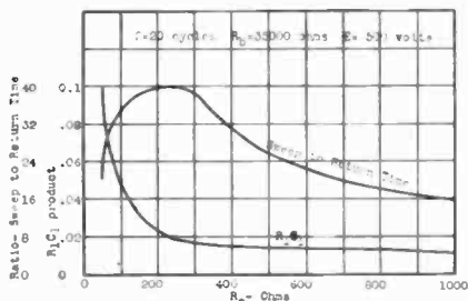
Fig. 3—Curves showing the variation of sweep-to-return time and the variation of the R_1C_1 product with R_e \cdot C_1=0.07 microfarad.
