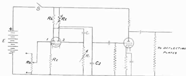
Fig. 1—Schematic diagram of a sweep circuit.
