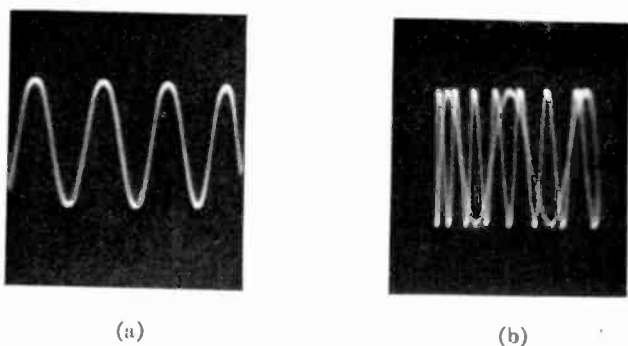
Fig. 5—Oscillograms taken using the sweep circuit described. (a) Oscillogram of a 1000-cycle wave. (b) Oscillogram of a 940,000-cycle wave.
