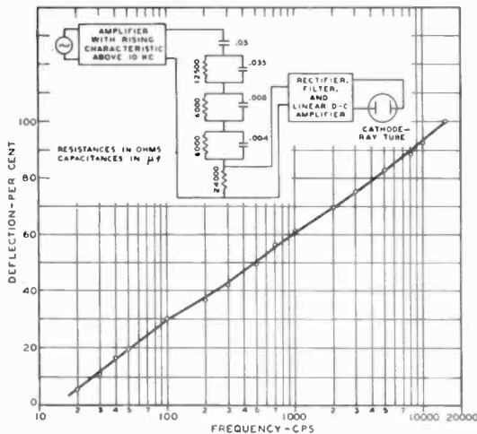
Fig. 2—Network for logarithmic frequency scale.
