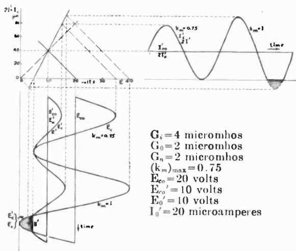
Fig. 10—Graphical analysis of the peak clipping of the rectified output ( I' , E' ) and the peak augmentation of the input voltage envelope ( E_c' ).
