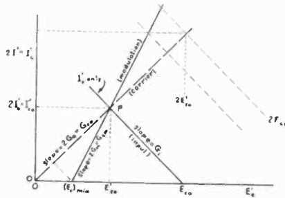
Fig. 9—The current-voltage relations as affected by the input circuit.
