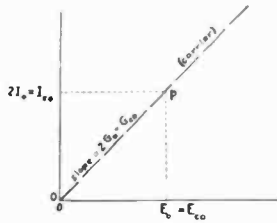
Fig. 3—The linear current-voltage relation of the carrier input ( I_{c0} , E_{c0} ) and rectified output ( I_0 , E_0 ).
