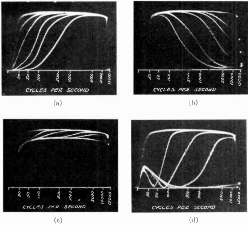
Fig. 8—Amplifier characteristics.
