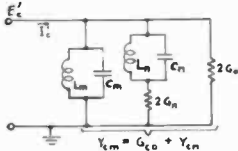
Fig. 12—The apparent input admittance of the diode of Fig. 11 toward components of side-band frequencies.
