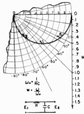
Fig. 5—Vector envelope of E_2/E_1 .
