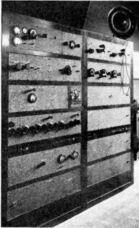
Fig. 9—Radio-Kootwijk. The single-side-band check receiver.
