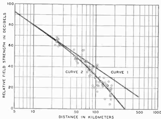
Fig. 2—Replot of data published by Beverage.
