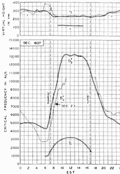
Fig. 1—Virtual heights and critical frequencies of the E, F, and F_2 layers of the ionosphere for December 1937. The solid-line graph represents for undisturbed days. Dotted curve shows values for ionospherically disturbed day of December 23.
