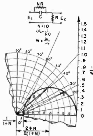
Fig. 6—Vector envelope of E_2/E_1 .
