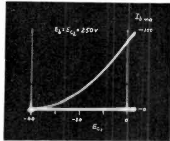
Fig. 6—Transfer characteristic of a typical power pentode.
