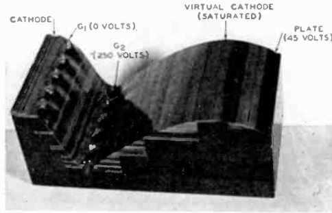
Fig. 25—Topographic model of potential field shown in Fig. 24.
