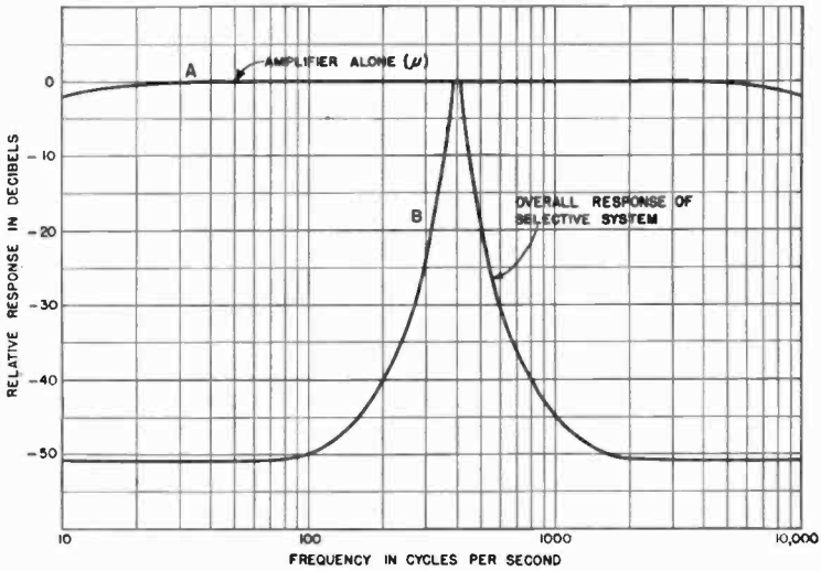
Fig. 4—Characteristics of typical selective circuit based upon degeneration.
