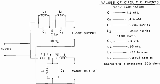
Fig. 3—Schematic diagram of aircraft filter unit.
