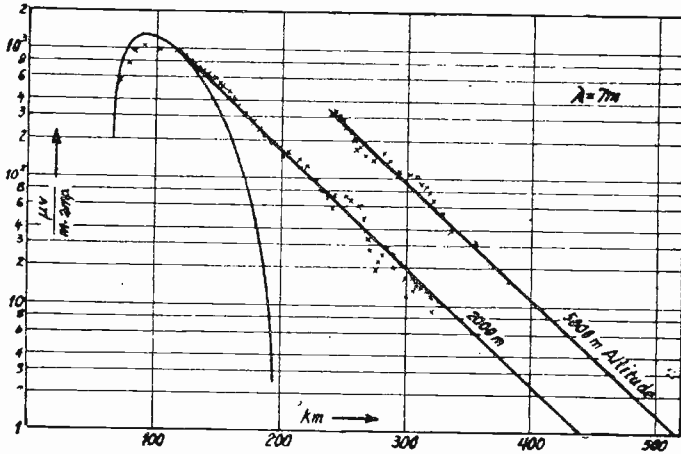
Fig. 5—Field intensity vs. distance. Transmitting antenna 135 meters high. \lambda = 7 meters.
