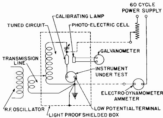
Fig. 1—Circuit and apparatus used in thermal ammeter calibration by means of lamps.
