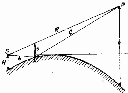
Fig. 3—Reflection of the rays at the curved earth.
