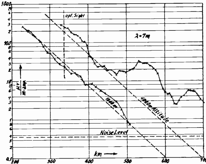
Fig. 18—Example of refraction. Calculated and measured field intensity curves. Transmitter elevation 1000 meters. Power = 7 kilowatts. \lambda = 7 meters.
