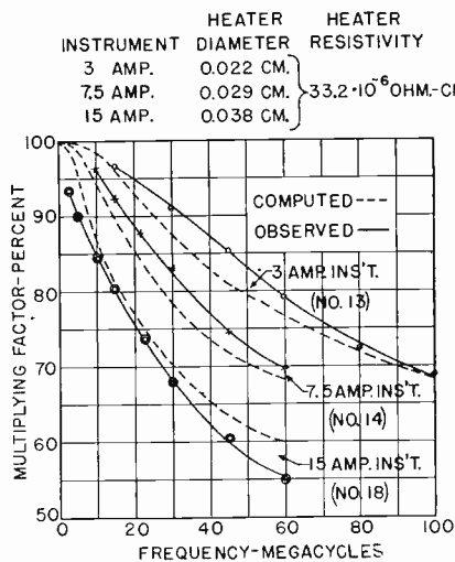
Fig. 5—Computed and observed values of multiplying factors of instruments.
