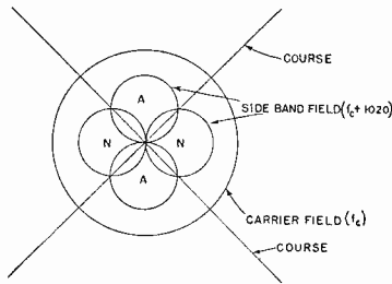
Fig. 2—Field pattern of simultaneous radio range and broadcast station.
