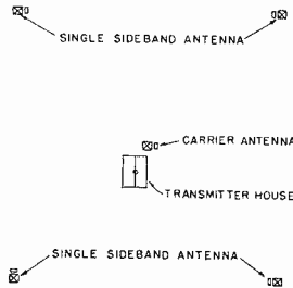
Fig. 1—Layout of radio range plot and antenna system.
