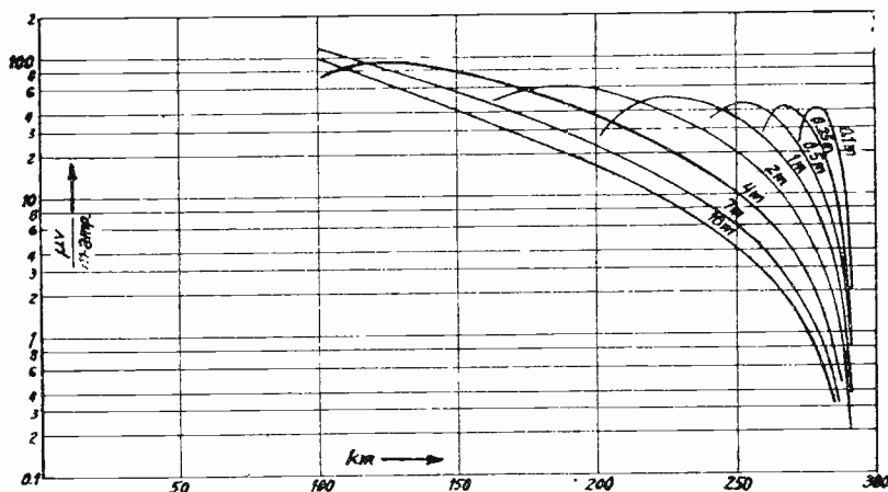
Fig. 4—Field intensity vs. distance within the line of sight. Transmitting antenna 30 meters high. Received at 6000 meters altitude.
