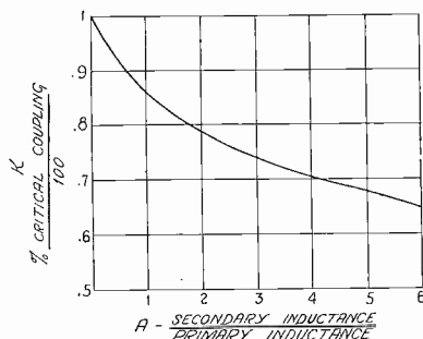
Fig. 3—Optimum coupling if linear detectors are used.
