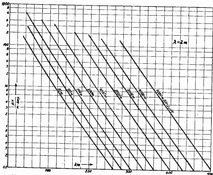
Fig. 12—Field intensity vs. distance for various altitudes. Transmitting antenna 30 meters high. \lambda = 2 meters.
