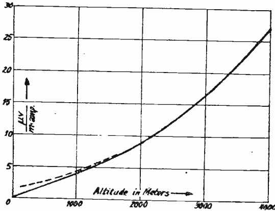
Fig. 6—Field intensity vs. altitude. Distance 335 kilometers. \lambda = 7 meters.
