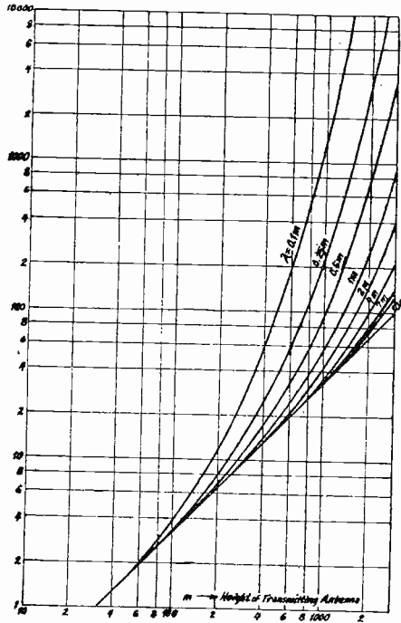
Fig. 17—Increase of field intensity with height of transmitting antenna. \lambda = 0.1 \dots 10 meters.
