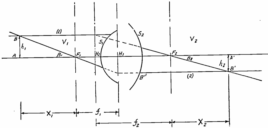
Fig. 5—Location of cardinal points.
