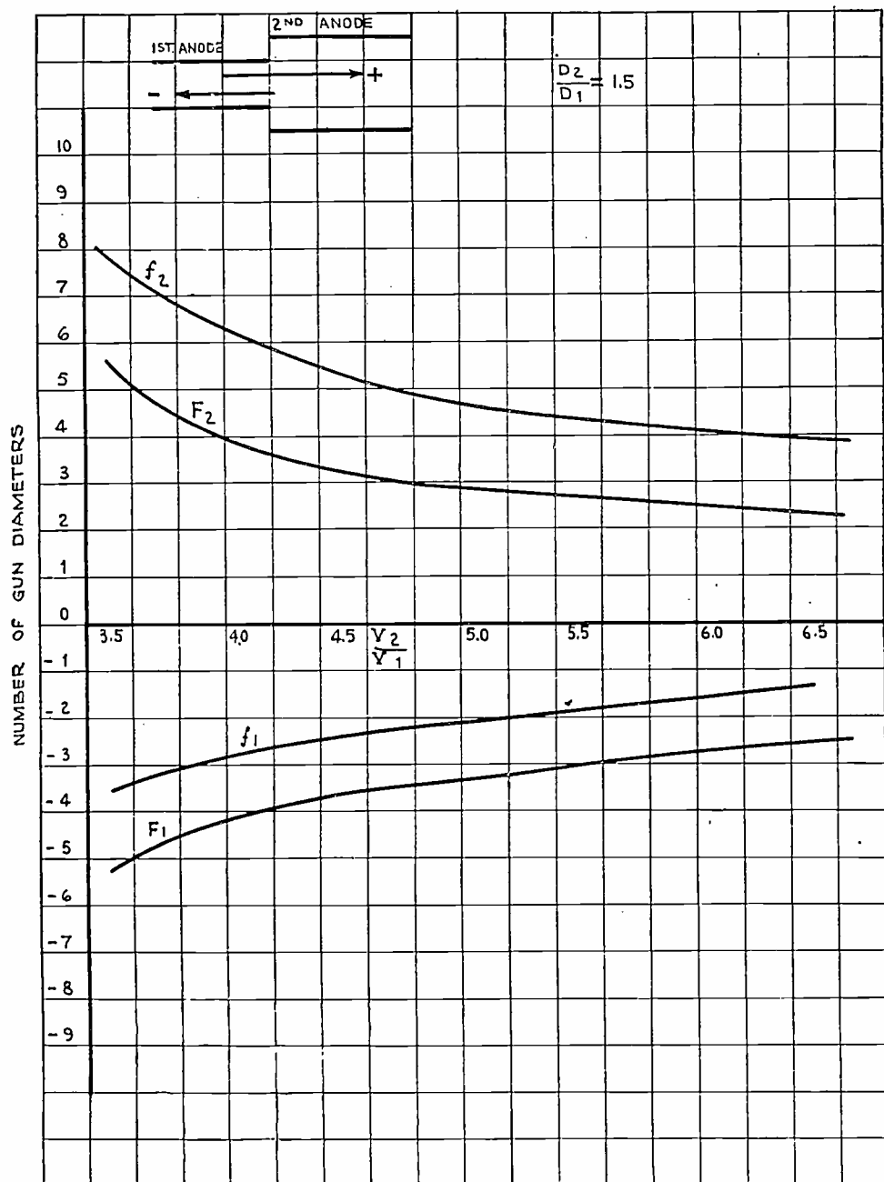
Fig. 10—Variation of optical constants with voltage ratio.
