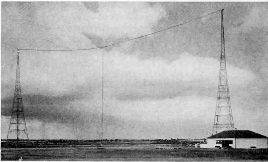
Fig. 1—Transmitter building and directional antenna.
