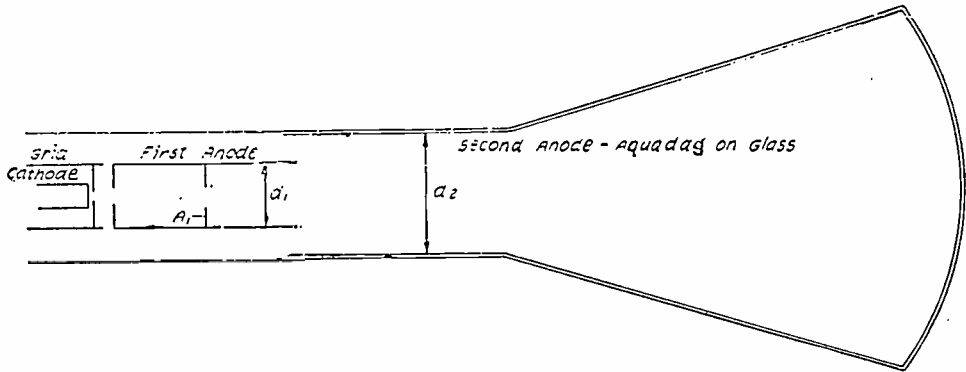
Fig. 1—Cathode-ray tube.
