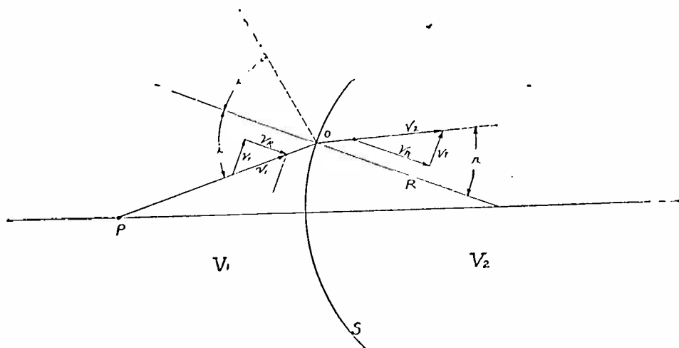
Fig. 3—Electron refraction and reflection at spherical surface.
