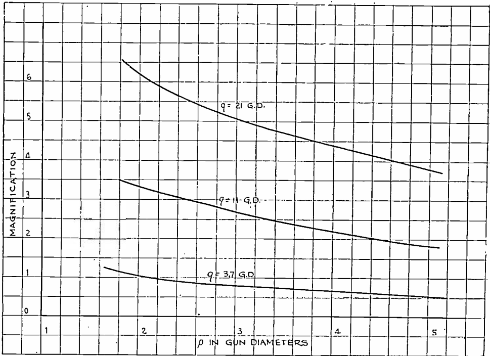
Fig. 17—Magnification vs. object distance.
