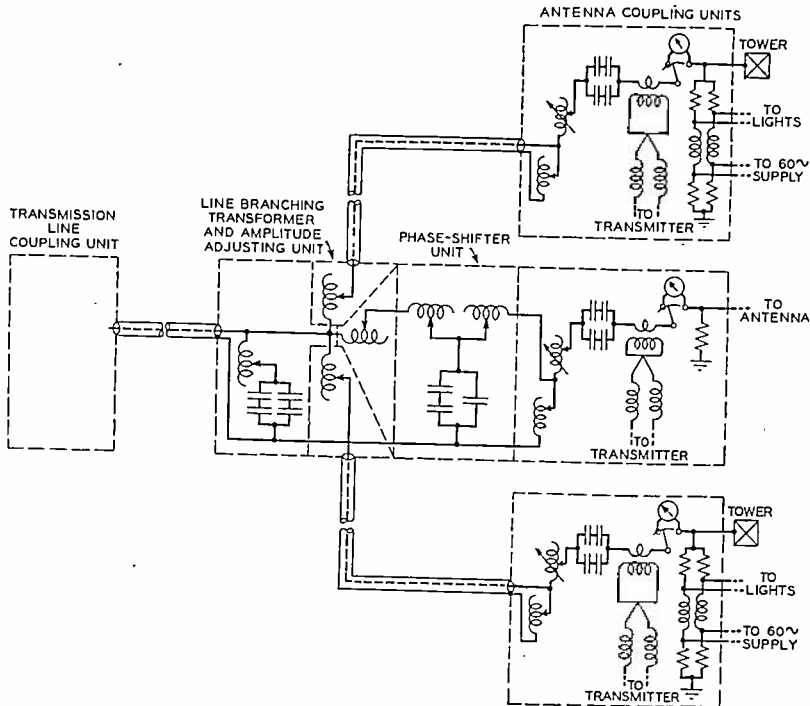
Fig. 3—Antenna array coupling circuits.
