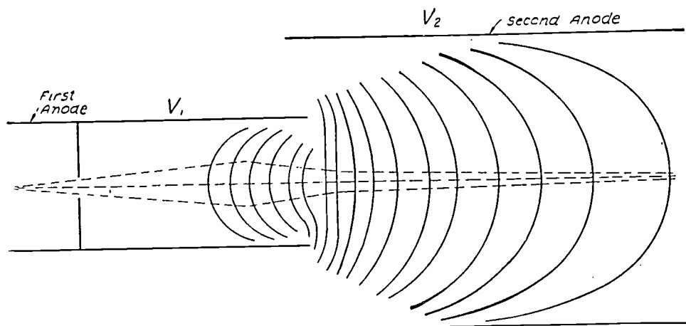
Fig. 2—Equipotential line plot of two cylinders.
