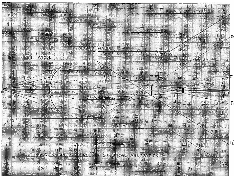
Fig. 21—Imaging in the presence of spherical aberration.
