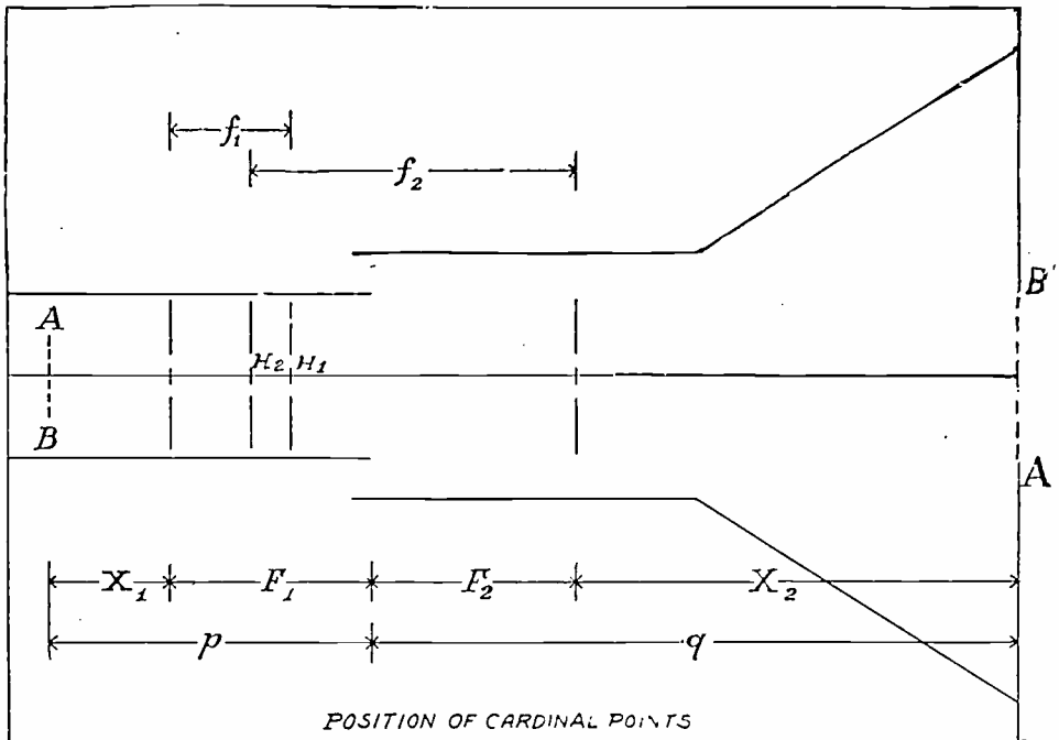
Fig. 7—Position of cardinal points.
