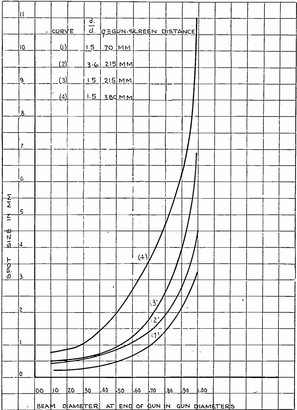
Fig. 26—Minimum spot size vs. beam width.
