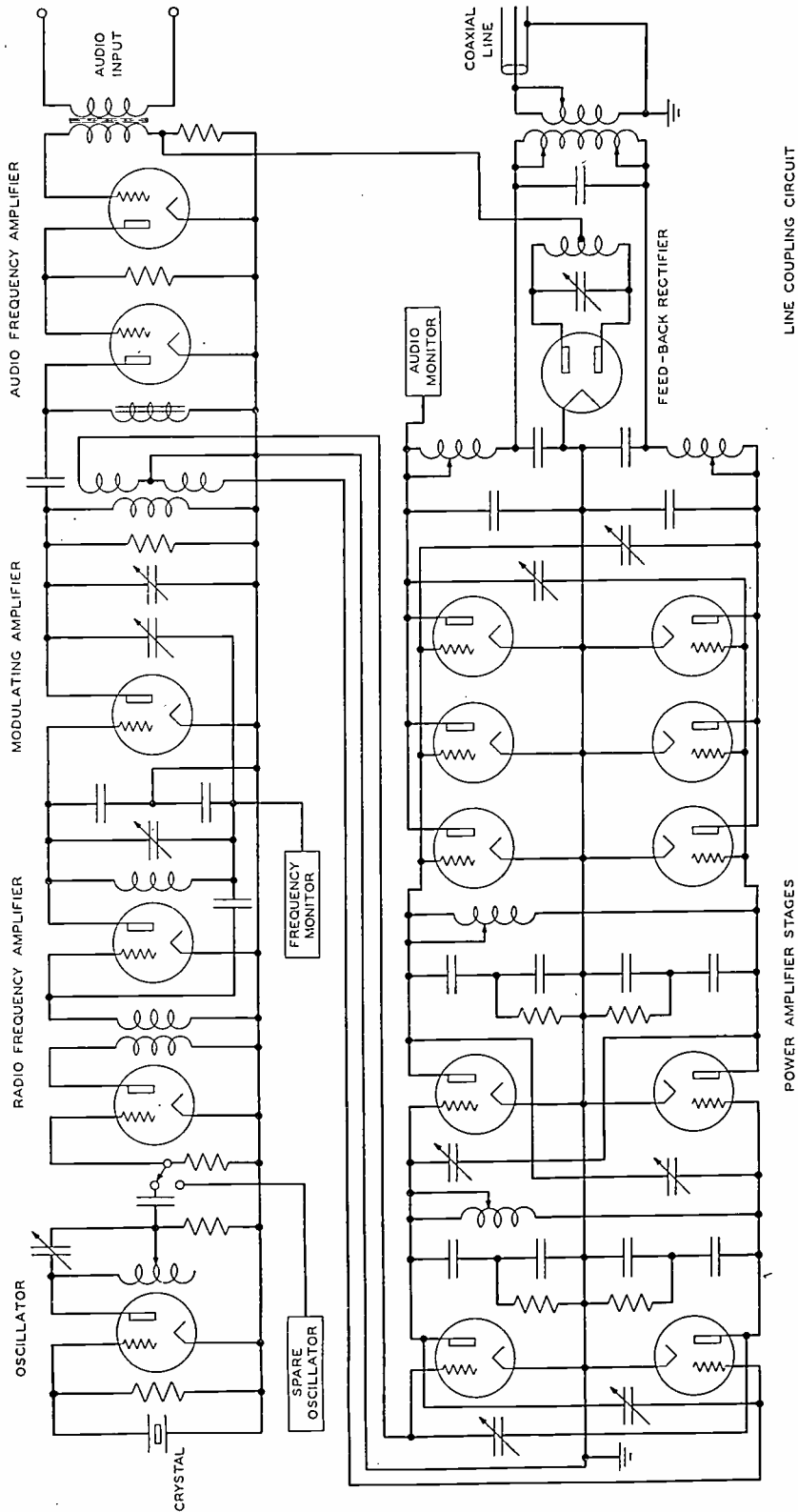
Fig. 7—Fifty-kilowatt transmitter circuits.
