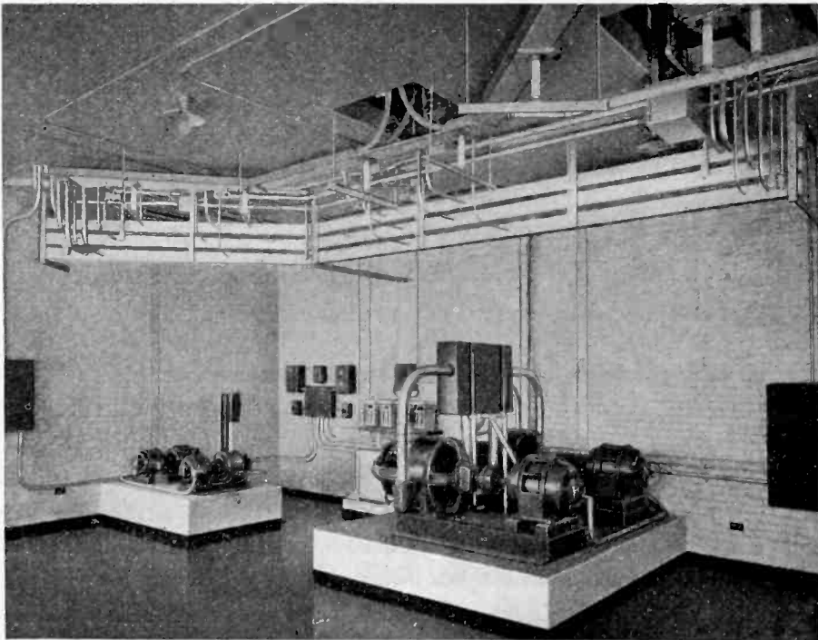
Fig. 10—Basement view showing motor generators, cooling water hose troughs, and wiring ducts.
