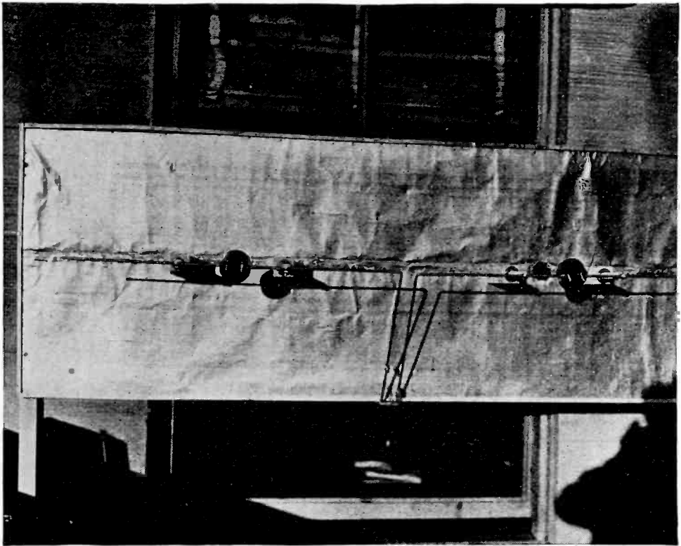
Fig. 7—Experimental directive transmitting antenna with reflector.
