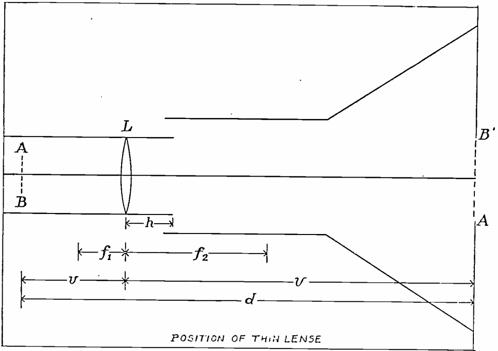
Fig. 19—Position of thin lens.
