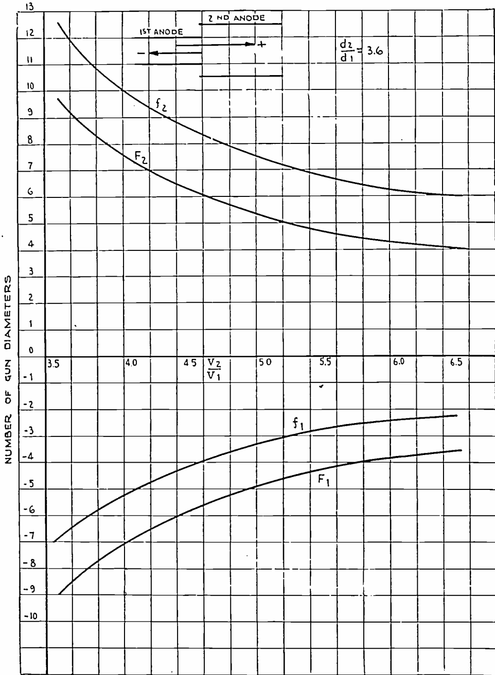
Fig. 8—Variation of optical constants with voltage ratio.
