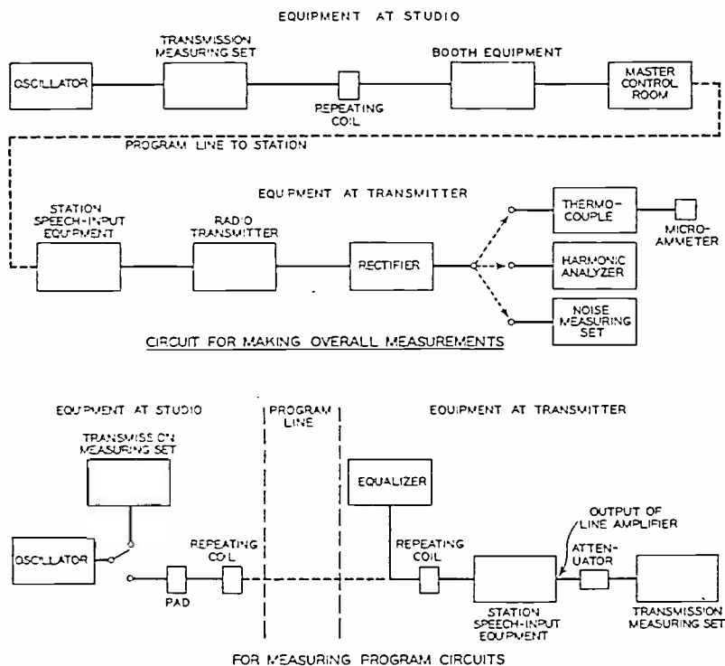
Fig. 13—Circuits used for measurements.
