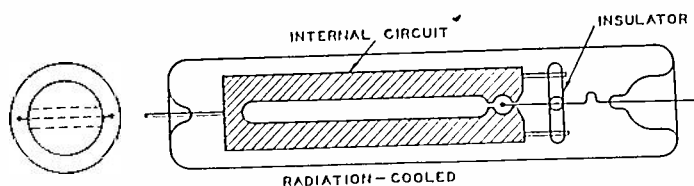
Fig. 13—Sectional view of an internal circuit radiation-cooled magnetron for obtaining high power at ultra-high frequencies.
