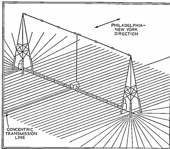
Fig. 2—Antenna and ground system.
