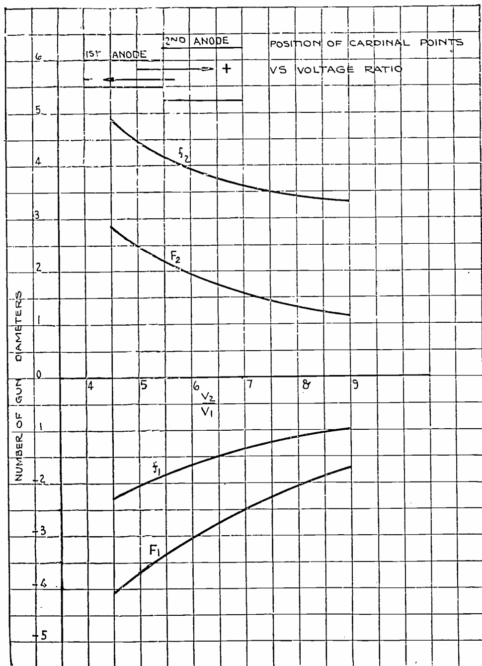
Fig. 16—Position of cardinal points vs. voltage ratio.
