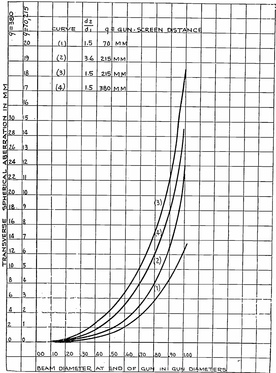
Fig. 24—Spherical aberration vs. beam width.
