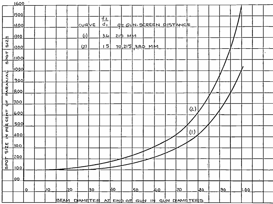
Fig. 27—Minimum spot size vs. beam width.
