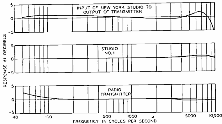
Fig. 14--Frequency response curves.
