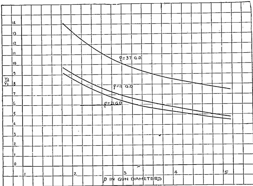
Fig. 18—Voltage ratio vs. object distance.
