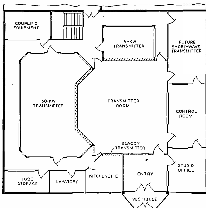
Fig. 4—Main floor plan of transmitter building.
