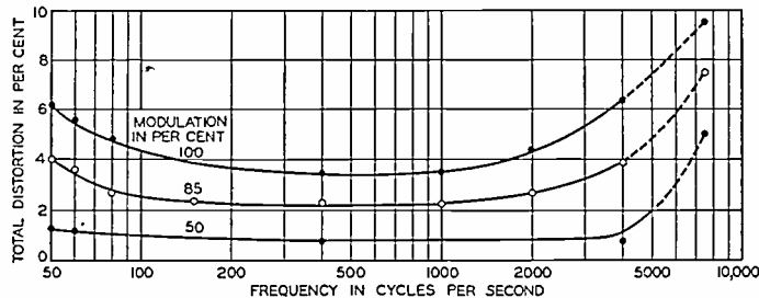
Fig. 15—Audio distortion measurements.
