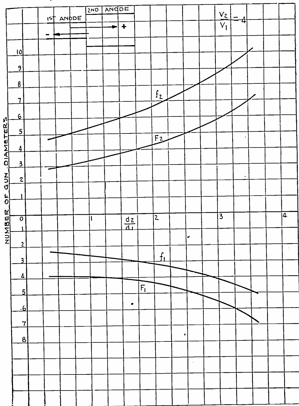
Fig. 12—Variation of optical constants with diameter ratio.
