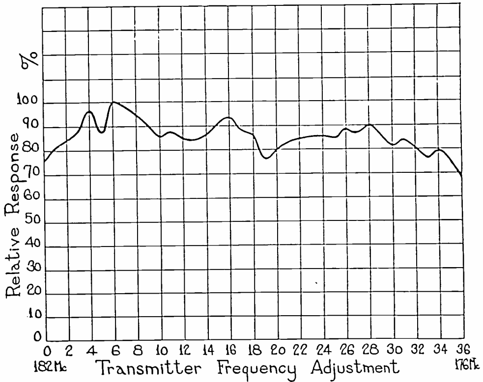
Fig. 12—Response curve with directive transmitting antenna and vertical directivity at receiver. Horizontal polarization, transmitter at sixty-seventh floor.
