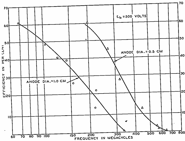
Fig. 9—Efficiency versus frequency for two sizes of magnetrons operating at the same plate potential.
