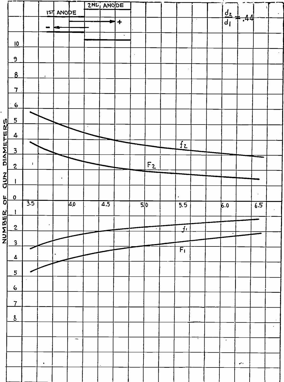
Fig. 11—Variation of optical constants with voltage ratio.
