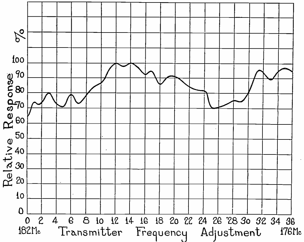
Fig. 11—Response curve with directive transmitting antenna and half-wave dipole at receiver. Horizontal polarization, transmitter at sixty-seventh floor.
