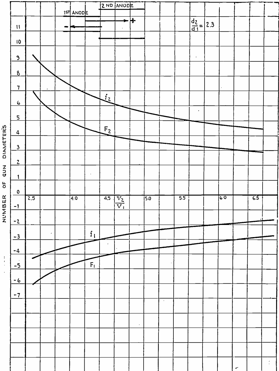
Fig. 9—Variation of optical constants with voltage ratio.
