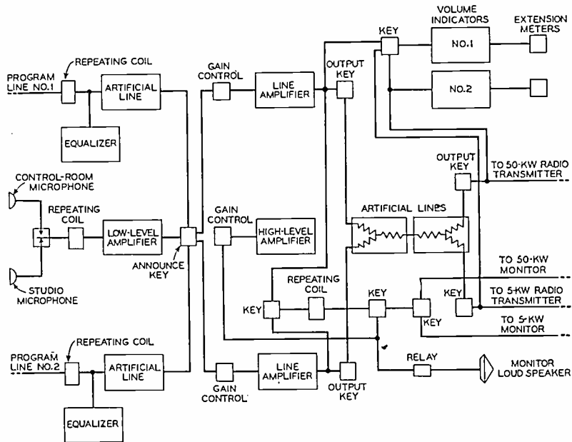
Fig. 12—Diagram of speech input equipment and circuits at the WOR transmitter station, Carteret, New Jersey.
