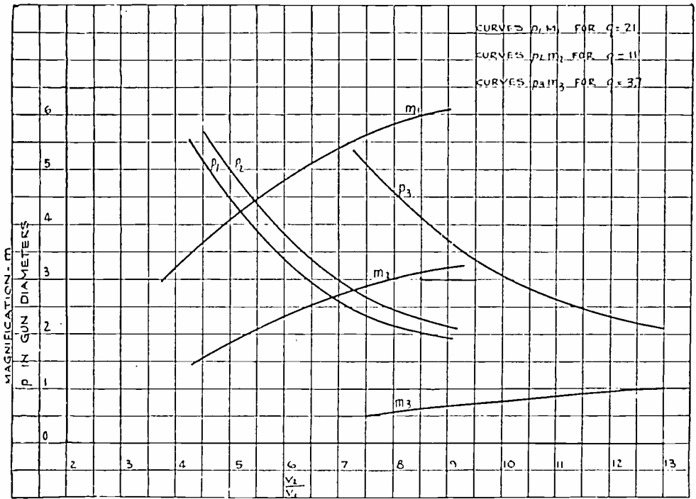
Fig. 15—Magnification and object distance vs. voltage ratio.
