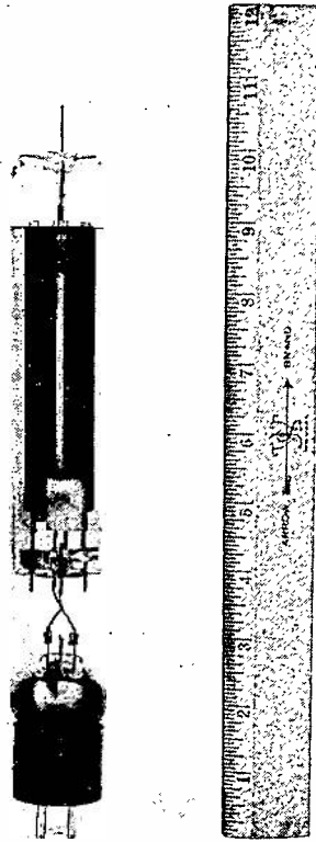
Fig. 14—Photograph of an internal circuit radiation-cooled magnetron oscillator for 550 megacycles.
