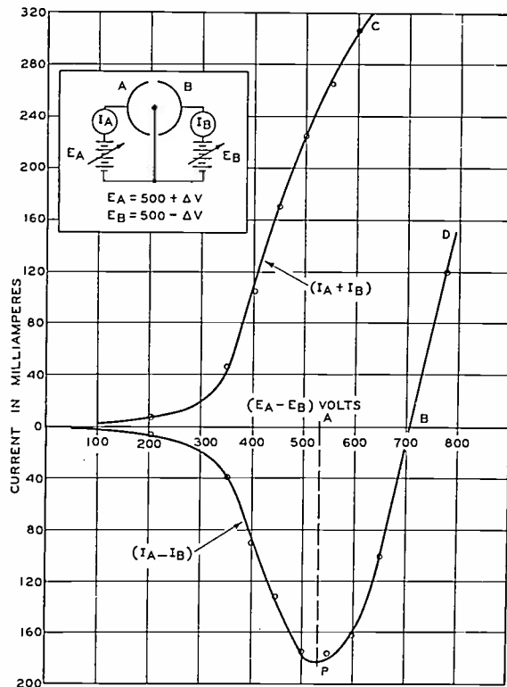
Fig. 3—Static characteristics of a two-segment magnetron.
