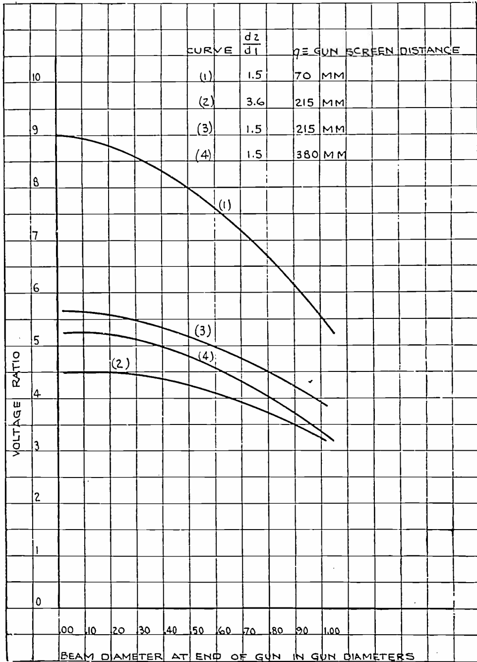
Fig. 25—Voltage ratio vs. beam width.
