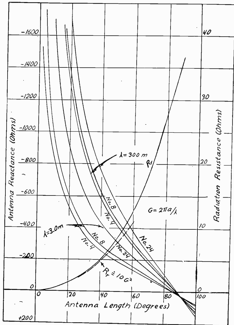
Fig. 11—Resistance and reactance of straight vertical antennas.
