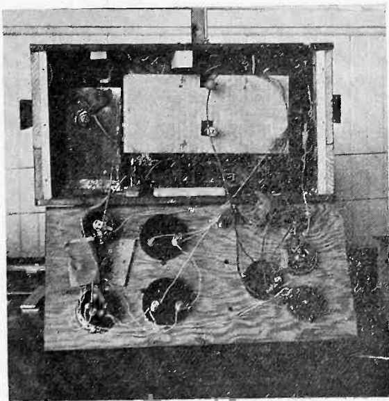
Fig. 4—Interior view of the receiver.
