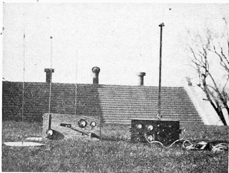
Fig. 2—The apparatus set-up. The receiver is on the right.
