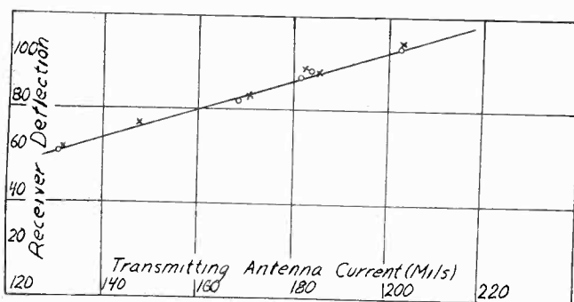
Fig. 7—The receiver deflection vs. transmitter antenna current.
