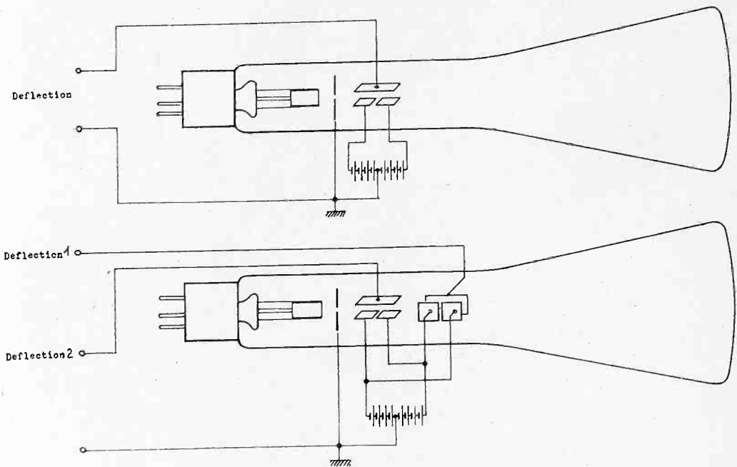
Fig. 1—Connections to eliminate origin distortion.
