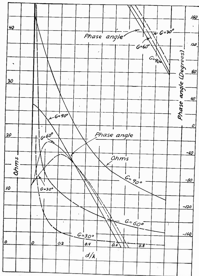
Fig. 13—Mutual impedance between two similar vertical antennas as a function of separation, d .
