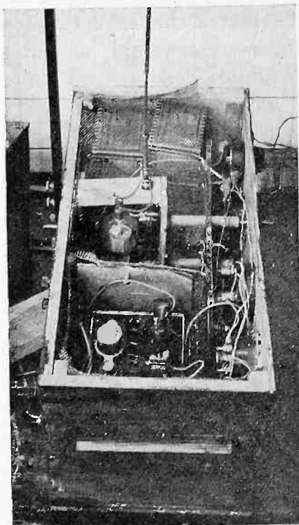
Fig. 3—Interior view of the receiver.
