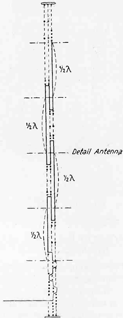
Fig. 10—Detail of Marconi aerial.
