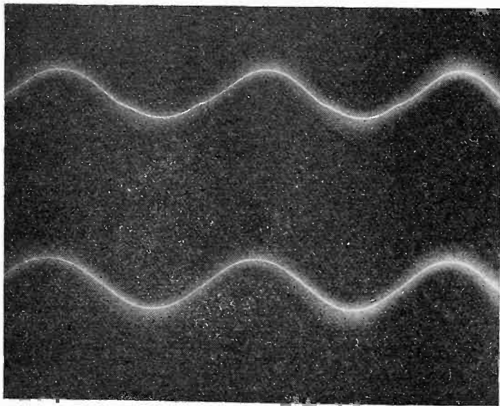
Fig. 5—Oscillogram of a sinusoidal voltage with (upper) and without (lower) space-charge distortion.
