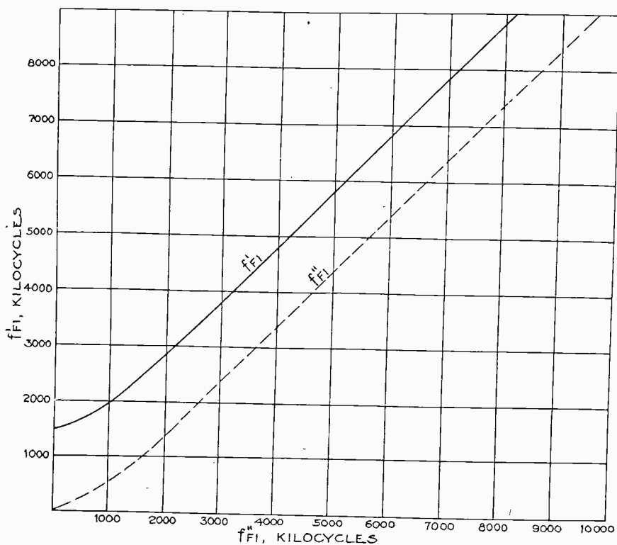
Fig. 1—Graphs showing the frequency separation of the critical frequencies of the ordinary and extraordinary rays due to magnetic double refraction at 180-kilometer height at Washington, D.C.
