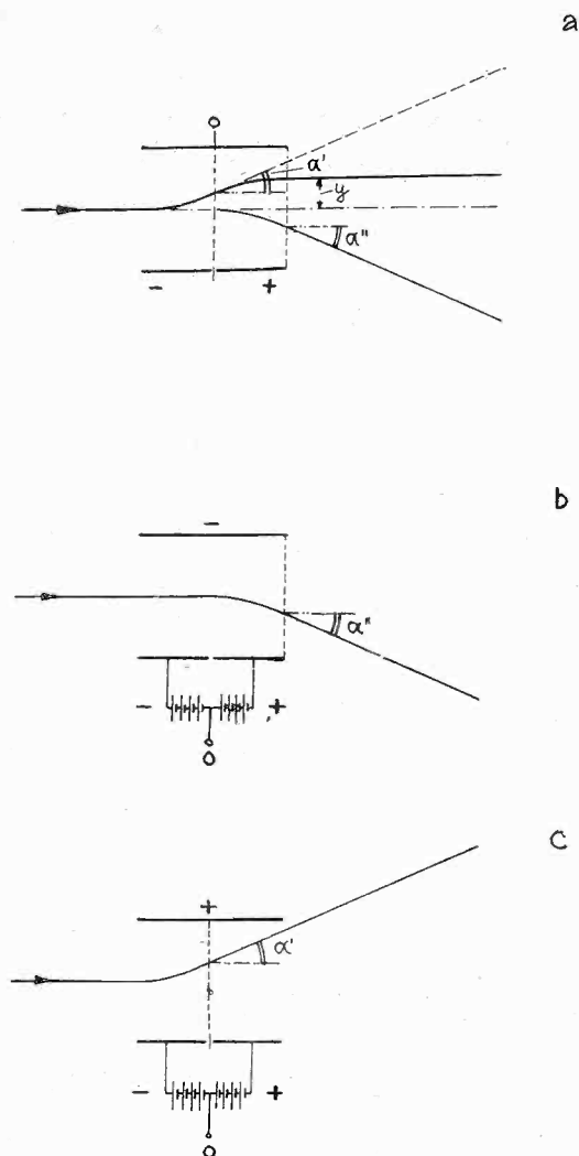
Fig. 2—Beam path at different deflection voltages.
