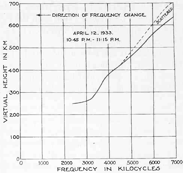
Fig. 9—Evening values of virtual height for April 12, 1933.
