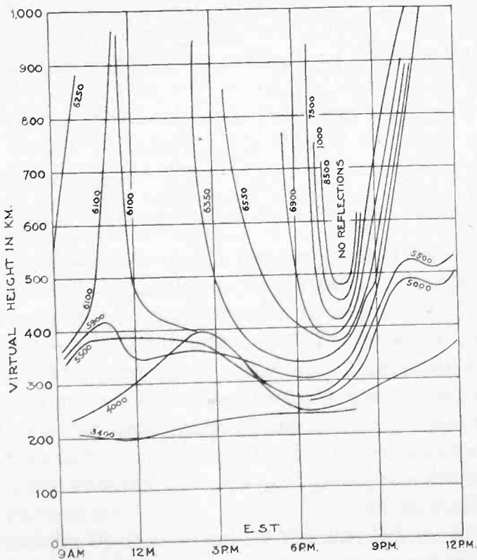
Fig. 22—Virtual height contours for April 5, 1933.
