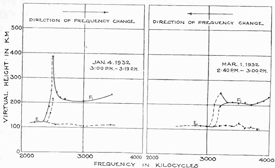
Fig. 2—Typical cases of E layer critical frequency.
