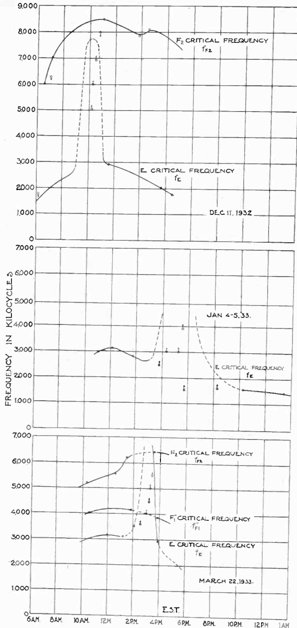
Fig. 6—Examples of occasional random high values of f_E . \circ indicates observations. \delta indicates critical frequency greater than observed frequency. \phi indicates critical frequency is less than observed frequency.
