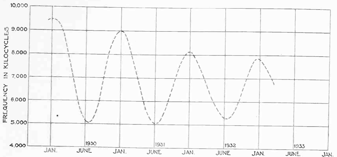
Fig. 19—Average variation as shown in Fig. 18, plotted to indicate change in average values from year to year.
