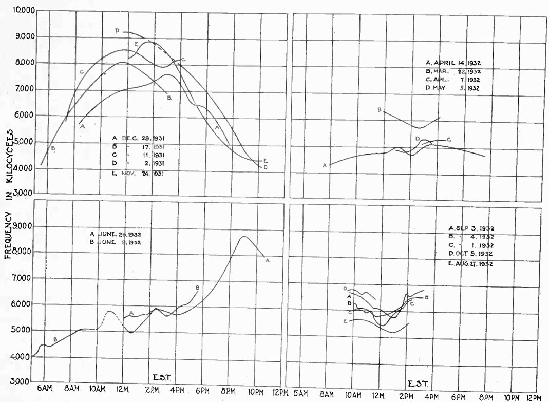
Fig. 17—Seasonal variation of diurnal characteristic of f_{F_2} .
