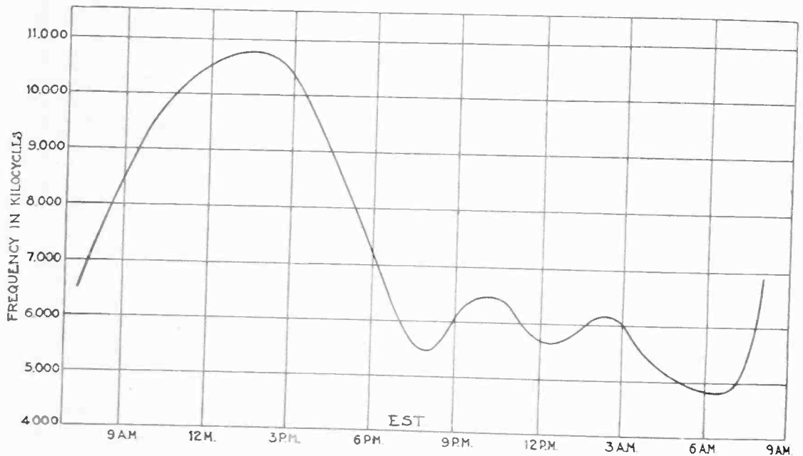
Fig. 20—Diurnal characteristic of f_{F_2} for a winter day of high f_{F_2} .
