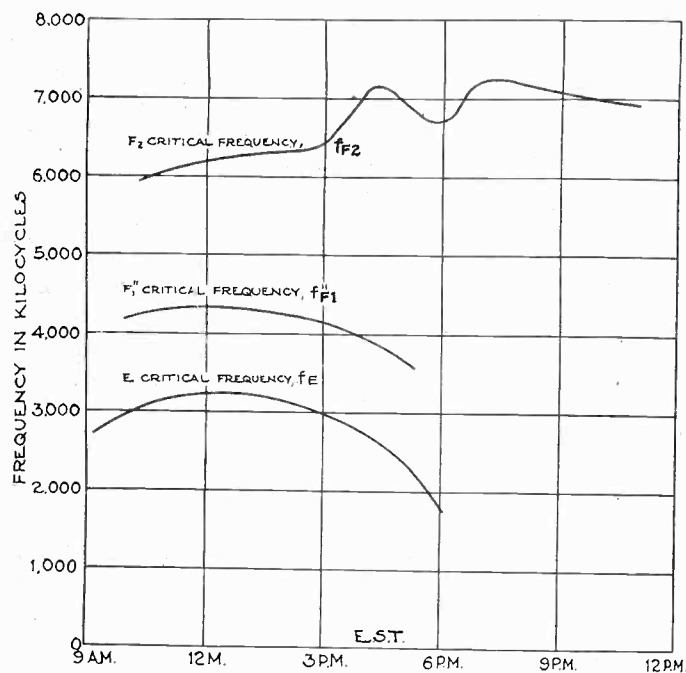
Fig. 11—Typical diurnal variations of f_{F_1}'' showing its relation to other critical frequencies.
