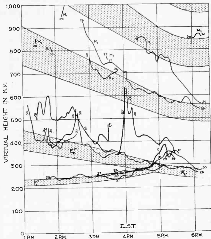
Fig. 16—Envelopes of the virtual heights for 4200 kilocycles for undisturbed days, with the virtual heights of the disturbed days superimposed for the days shown in Fig. 14.
