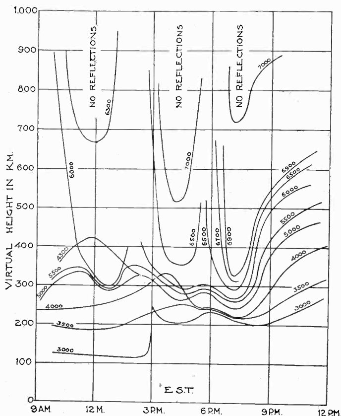
Fig. 23—Virtual height contours for April 12, 1933.
