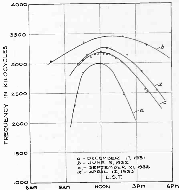
Fig. 3—Typical diurnal variations of f_E selected for days during the various seasons.
