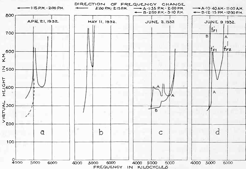
Fig. 25—Examples of rapid changes in f_{F_2} .
