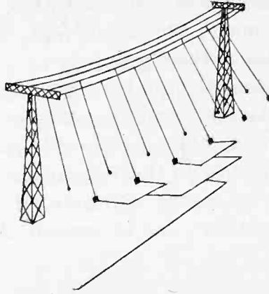
Fig. 9—Suspension of Marconi aerial.
