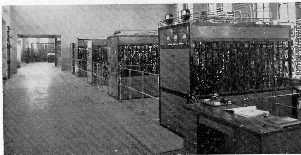
Fig. 7—Medium-wave transmitter—60 to 100 kilocycles.
