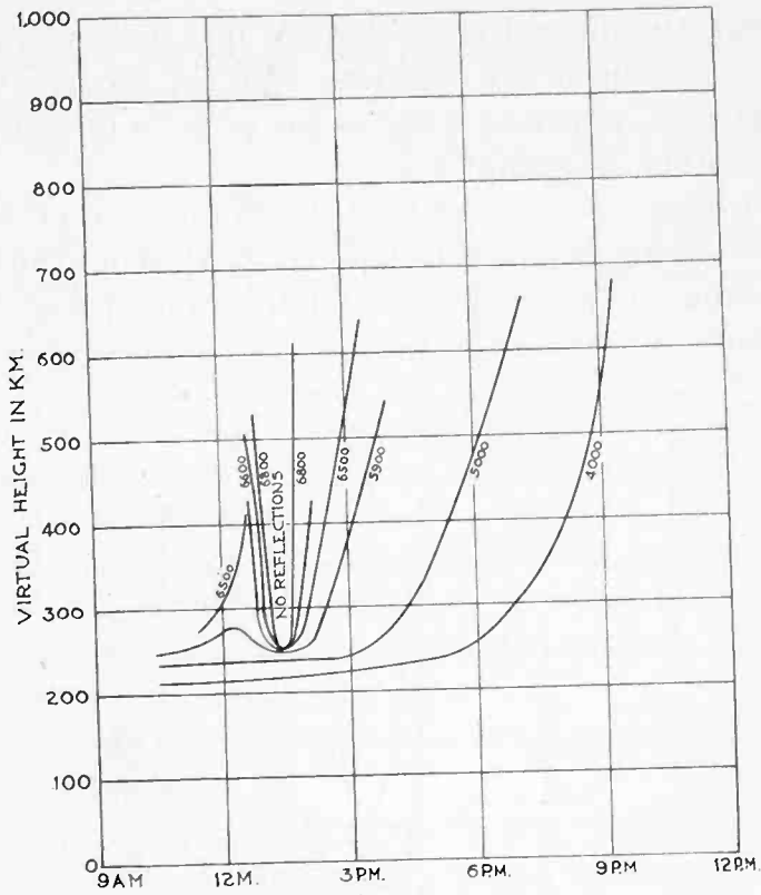
Fig. 21—Virtual height contours for December 21, 1932.
