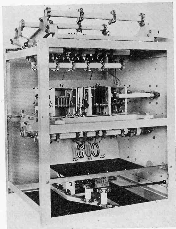
Fig. 12—High-frequency antenna coupling transformers.
