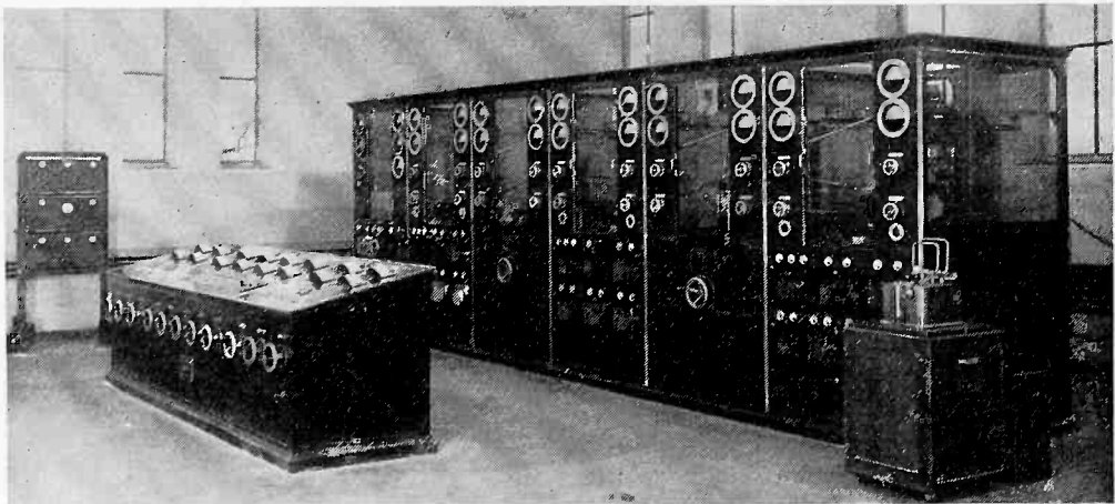
Fig. 4—High-frequency transmitter B.
