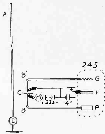
Fig. 1—Circuit diagram of the transmitter
