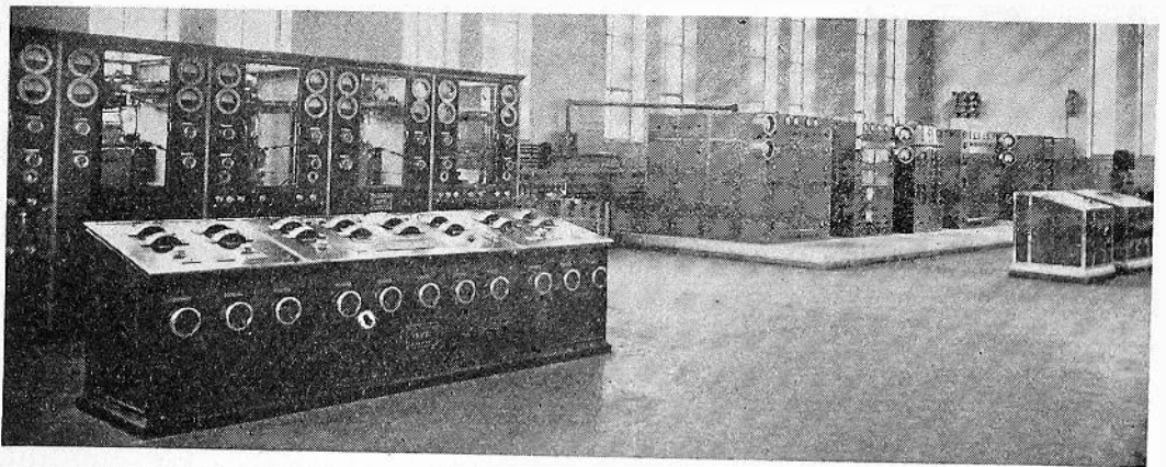
Fig. 5—View of transmitters A and B showing control tables.
