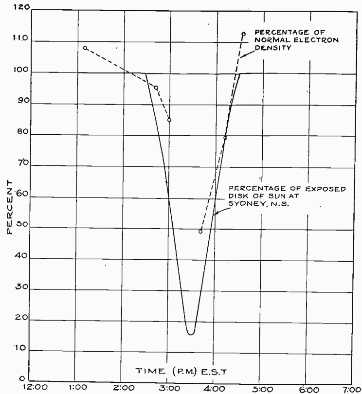
Fig. 4—Percentage of the normal maximum electron density in the E layer for the day of the eclipse together with the percentage of the exposed disk of the sun at Sydney.
