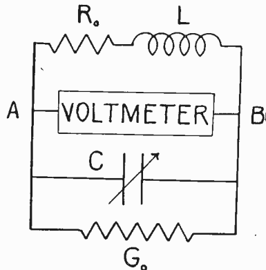
Fig. 1—Resonant circuit with parallel conductance.
