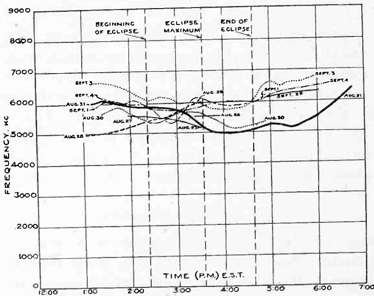
Fig. 14— F_2 critical frequency for the day of the eclipse superimposed on the curves of previous and succeeding days.
