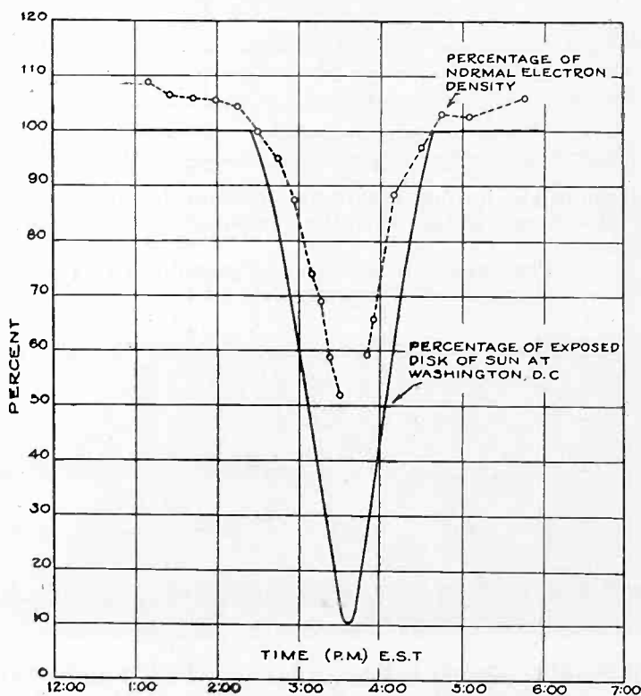
Fig. 3—Percentage of the normal maximum electron density in the E layer for the day of the eclipse together with the percentage of the exposed disk of the sun at Washington. —○— Percentage of the normal maximum electron density. ——— Percentage of exposed disk of the sun at Washington.
