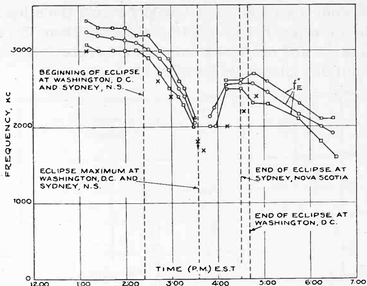
Fig. 2—Variations of f_{E''} during the time of the eclipse. —○— f_{E''} at Washington, mean values. Squares indicate limiting values. X f_{E''} at Sydney.
