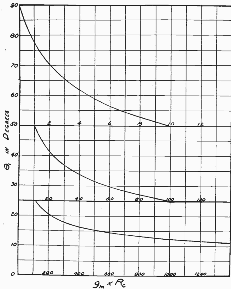
Fig. 5— \Theta_1 as a function of g_m \times R_c in a class B' amplifier.
