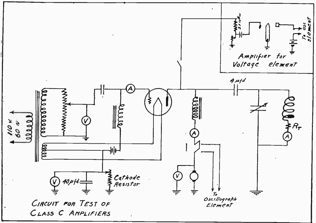
Fig. 3—Test circuit for class C amplifiers.
