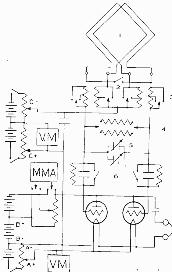
Fig. 2—Essential circuit of field strength meter.
