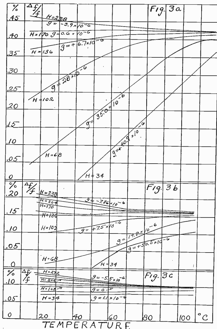
Fig. 3—Variation of frequency with temperature and magnetic field for an alloy containing 8% Cr, 37% Ni, balance Fe. (a) annealed; (b) forged; (c) quenched.
