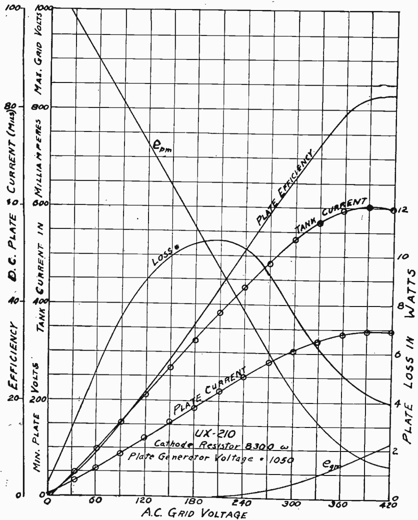
Fig. 4—Dynamic characteristics of linear amplifier with an operating angle \Theta_1 = 45 degrees.
