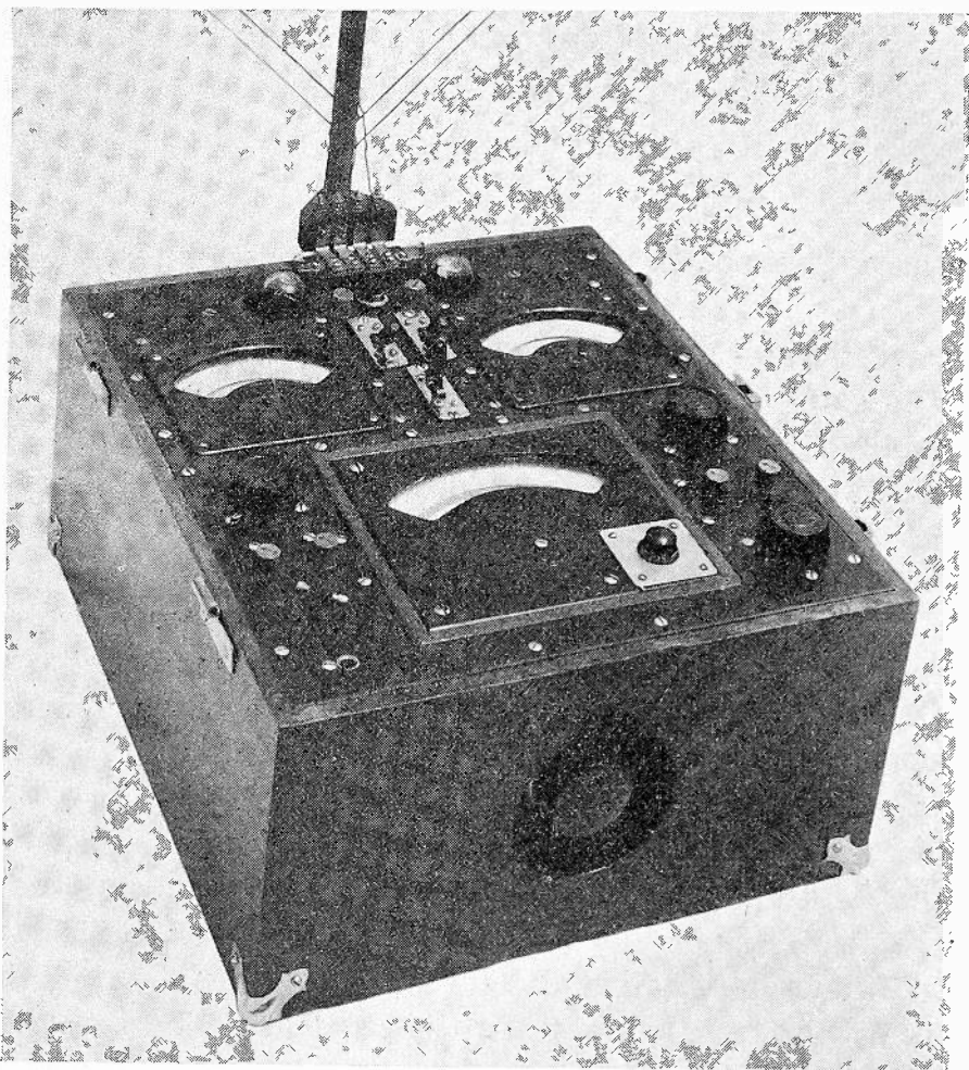
Fig. 3—Radio field strength meter—meter box showing electrical connections to loop.
