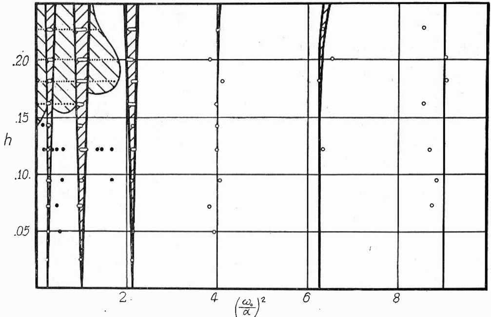
Fig. 9—Plot of the experimentally determined points, showing the character of the oscillations as a function of the several circuit parameters. Legend: white circles = substantially sinusoidal oscillations, black circles = periodic nonsinusoidal oscillations, small dots = no oscillations of any kind. A comparison should be made with the theoretically obtained curve of Fig. 1.
