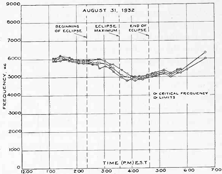
Fig. 13— F_2 critical frequency with limits for the day of the eclipse.
