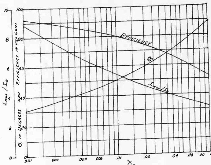
Fig. 11—Functions of \gamma_3 under optimum operating conditions.
