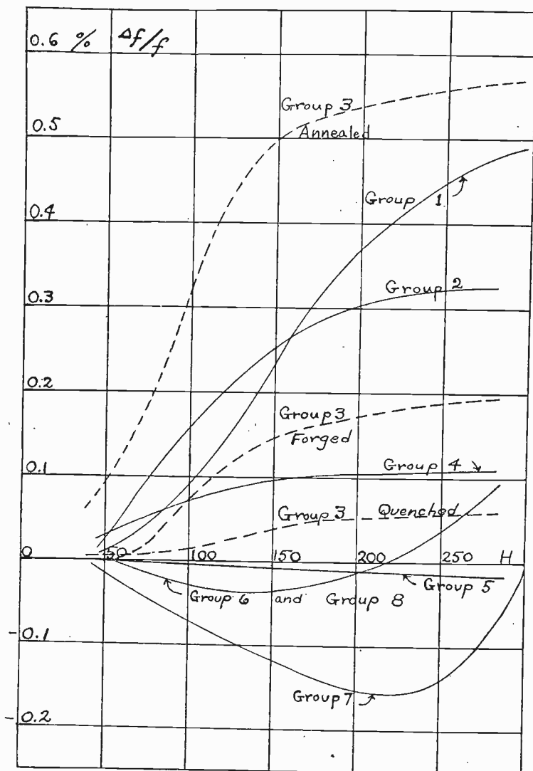
Fig. 2—Variation of natural frequency with magnetic field for eight groups of alloys.
