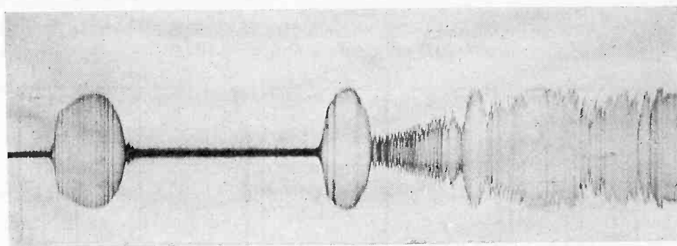
Fig. 7—Oscillograms showing the character of oscillations for C_0 = 1.7 , \Delta C = 1.0 microfarad, and L = 1.3 henrys. The speed of the motor was continuously changed during the taking of the oscillogram such that (\omega_0/\alpha)^2 went from an infinite value at the right (i.e. zero r.p.m. of commutator) to about 0.5 at the left. Unevenness of paper accounts for the irregular blackening observable in the oscillogram.
