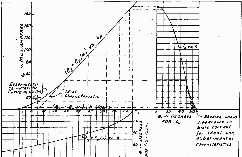
Fig. 1—Actual and ideal composite characteristic of '10 type tube.
