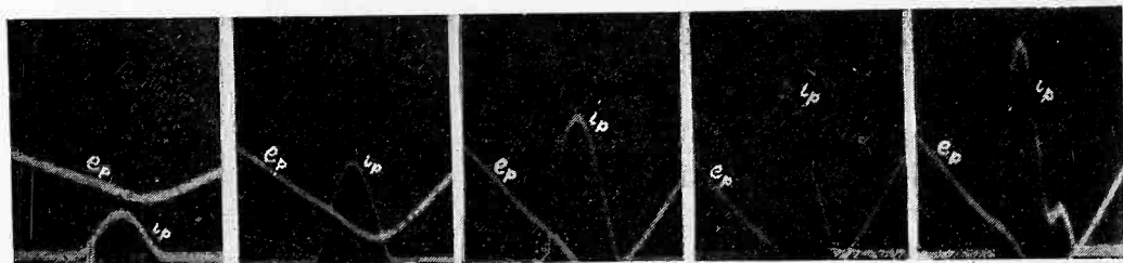
Fig. 6—Oscillograms of plate current in linear amplifier under conditions of Fig. 4.
