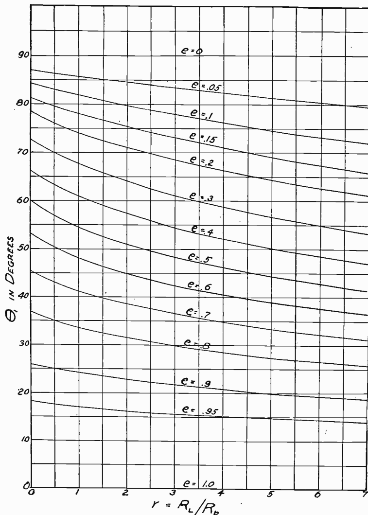
Fig. 9— \Theta_1 as a function of R_L/R_p and E_a/E_g .
