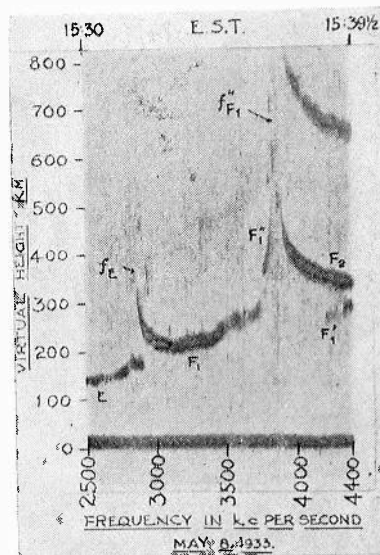
Fig. 5—Photograph showing type of record obtained in daytime. f_E denotes critical frequency for E layer. f''_{F_1} denotes critical frequency for ordinary ray in F_1 layer.
