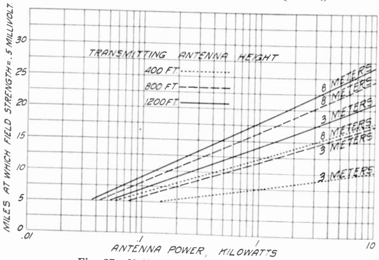
Fig. 27—Half-millivolt range vs. kilowatts.
