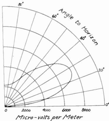
Fig. 33—Theoretical field strength vs. angle to horizon from horizontal Hertz doublet located one-half wavelength over Long Island ground. f=33.3 megacycles; power, 1 kilowatt; distance, 48 kilometers.
