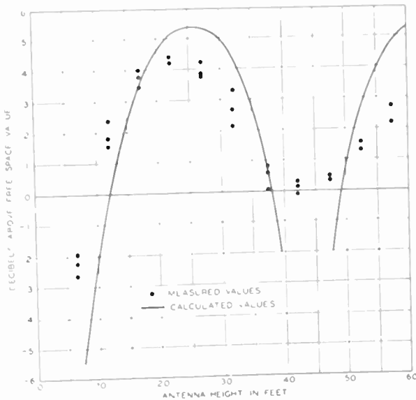
Fig. 14—Local reflection at Beer's Hill. Horizontal polarization \lambda = 4.15 meters.
