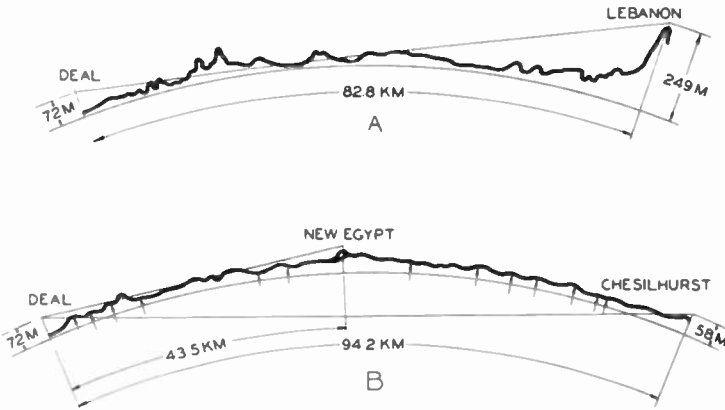
Fig. 6—Profiles of typical overland paths: A, path No. 8, over hilly country, with receiving location not masked by near-by hills; B, paths Nos. 16 and 17, over level country.
