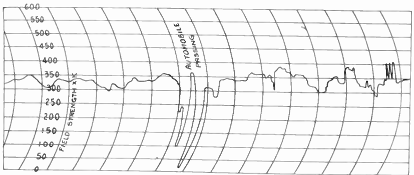
Fig. 20—Field strength at Twenty-fourth Street, 9 P.M.
