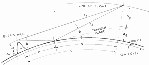
Fig. 22—Geometry of airplane reception.
