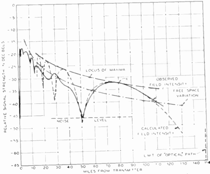
Fig. 16—Flight toward transmitter. Altitude—8000 feet; wavelength—4.3 meters, June 21, 1931.
