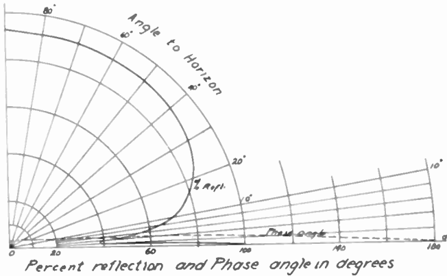
Fig. 29—Coefficient of reflection vs. angle to horizon for vertical polarization over salt water, 33.3 megacycles, assuming \epsilon = 80 , \sigma = 10^{10} electrostatic units.
