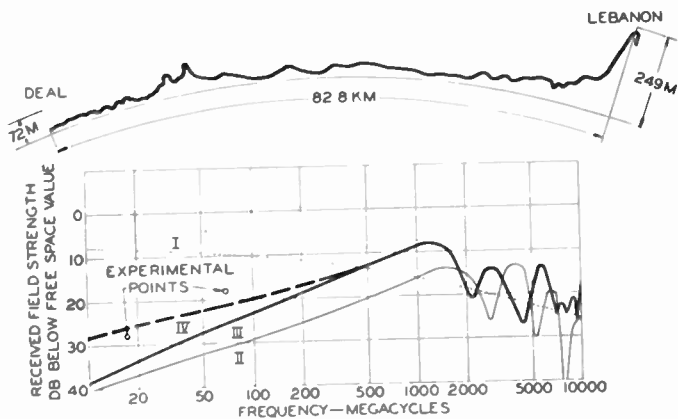
Fig. 17—Above: Profile of "nonoptical" path between Deal and Lebanon. Below: Frequency characteristics for this path calculated on various assumptions.
