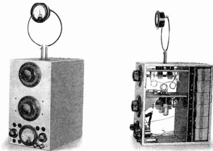
Fig. 1—Standard field generator.
