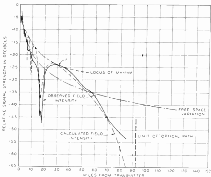
Fig. 18—Flight from transmitter. Altitude—2500 feet; wavelength—4.3 meters, June 26, 1931.
