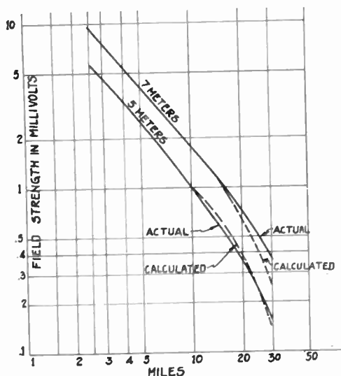
Fig. 25—Actual and theoretical attenuations.
