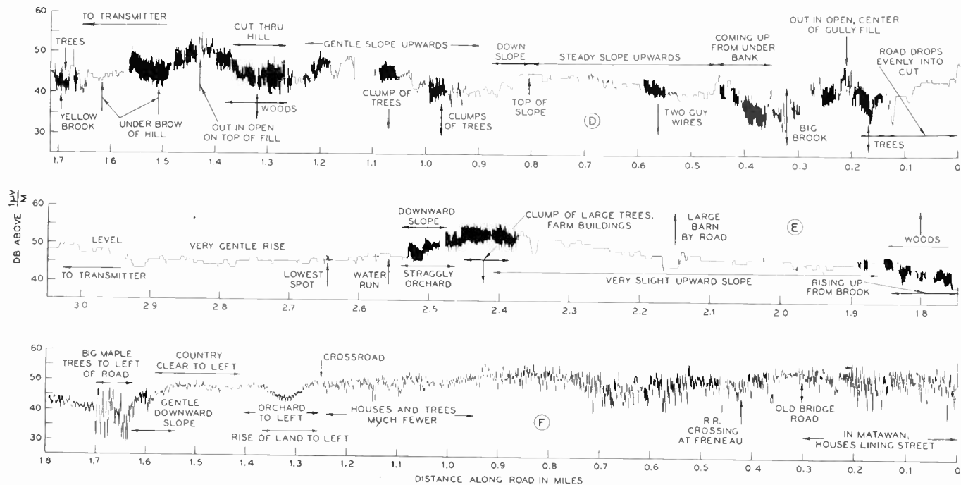
Fig. 5—Three diffraction patterns, two taken along lines radial to transmitter, one along a line perpendicular to transmitter direction.
