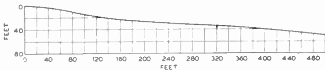
Fig. 9—Profile map of McCatharn's Hill.
