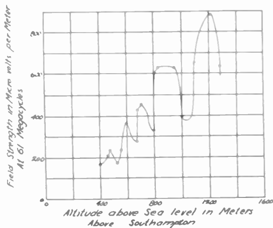
Fig. 14—Field strength vs. altitude at Southampton, 137 kilometers from Empire State 61-megacycle transmitter. Radiation 1 kilowatt.
