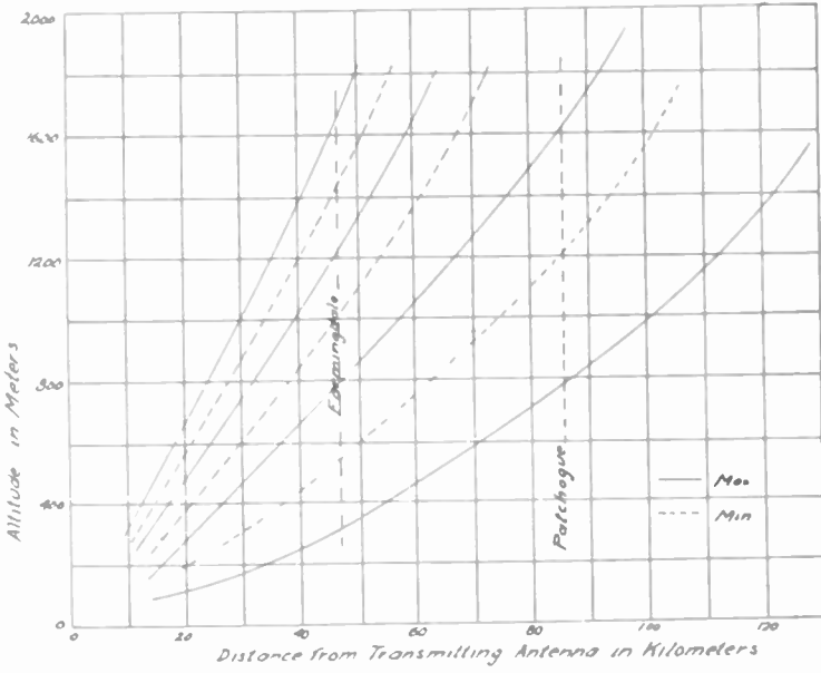
Fig. 38—Theoretical curves showing location of maximum and minimum field strengths produced by the Empire State 41-megacycle transmitter.
