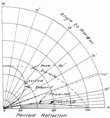
Fig. 30—Coefficient of reflection vs. angle to horizon for vertical and horizontal polarization for Long Island ground, assuming \epsilon = 9 , \sigma = 0 .
