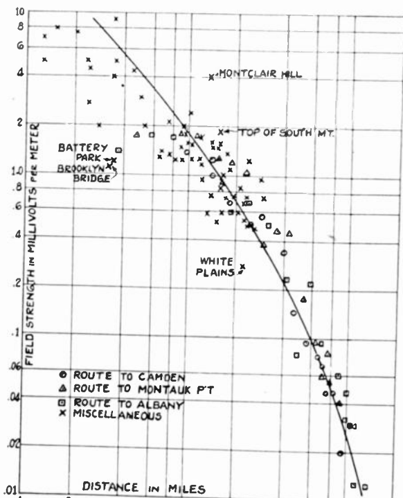
Fig. 6—Attenuation of 44-megacycle signals from Empire State building.
