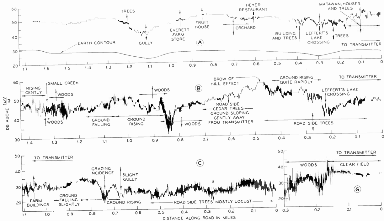
Fig. 4—Four diffraction patterns taken along lines radial to transmitter.
