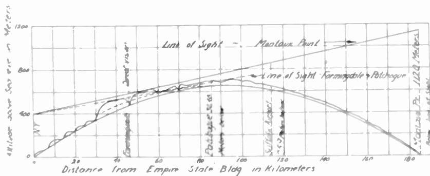
Fig. 2 Profile map airplane route from Empire State building over Long Island
