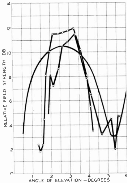
Fig. 11—Field strength as a function of the angle of elevation of the receiver, for transmission over salt water at 80 megacycles. The two experimental curves are from data taken with the receiver in an airplane flying at two constant altitudes. The smooth curve is theoretical.
