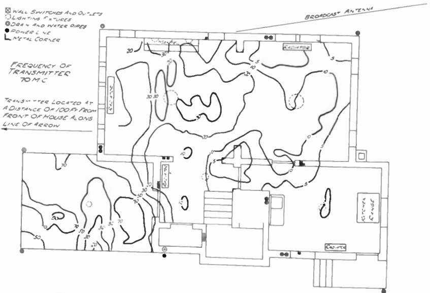
Fig. 17—Field strength within a residence, 70 megacycles.
