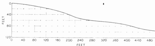
Fig. 12—Profile map of Beer's Hill.
