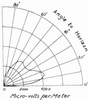
Fig. 34—Theoretical field strength vs. angle to horizon from vertical Hertz doublet located one-half wavelength over Long Island ground. f=33.3 megacycles; power, 1 kilowatt; distance, 48 kilometers.
