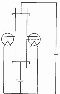
Fig. 3—Regenerative oscillator circuit, Holburn, 1921.
