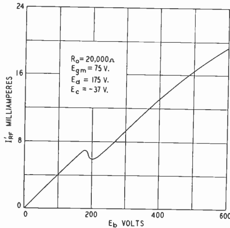
Fig. 36—Calculated r-f characteristics UX-865. Plate tuned circuit impedance R_0 = 20,000 ohms.
