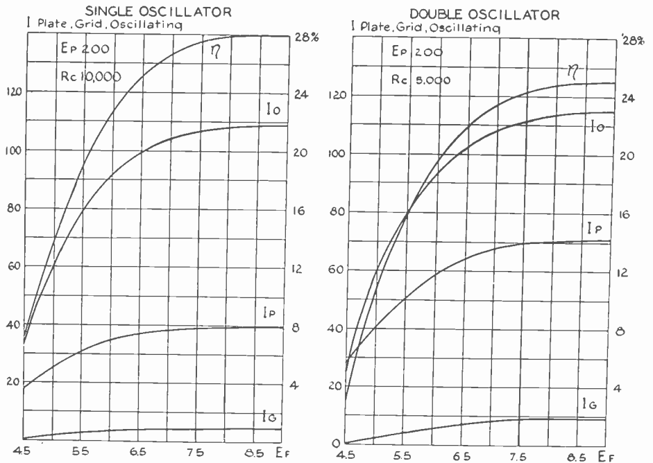
Fig. 7—Filament voltage vs. input, output, efficiency.
