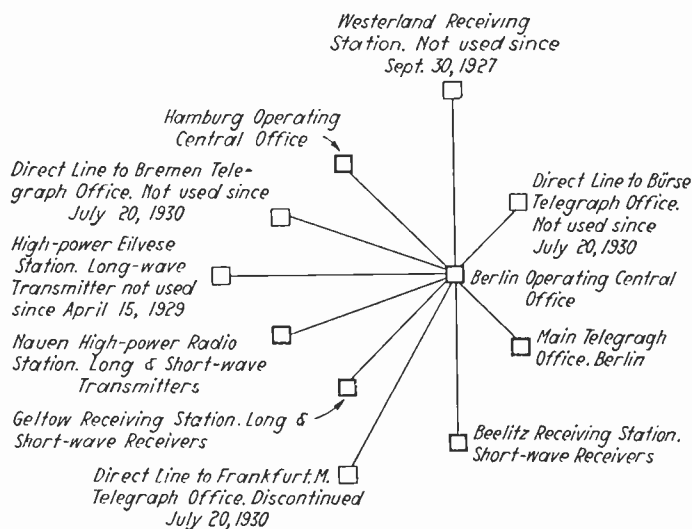
Fig. 22—Transradio operating installation 1920-1930.
