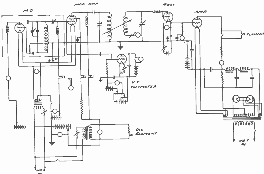
Fig. 2—Schematic diagram—tetrode modulated amplifier experimental set-up.
