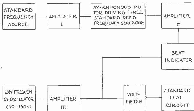
Fig. 8—Schematic diagram of reed calibrating equipment.
