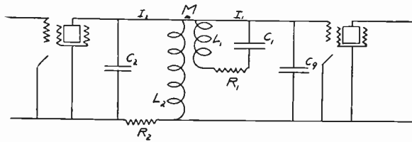
Fig. 4—Equivalent circuit of the r-f transformer.
