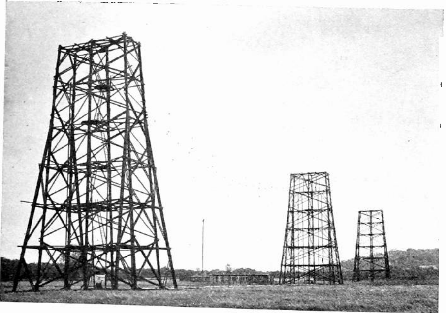
Fig. 17—Temporary directive receiving antenna in Geltow for reception from South America.
