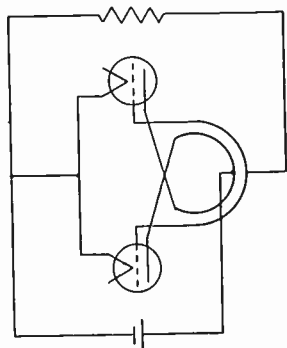
Fig. 4—Regenerative oscillator circuit, Mesny, 1924.
