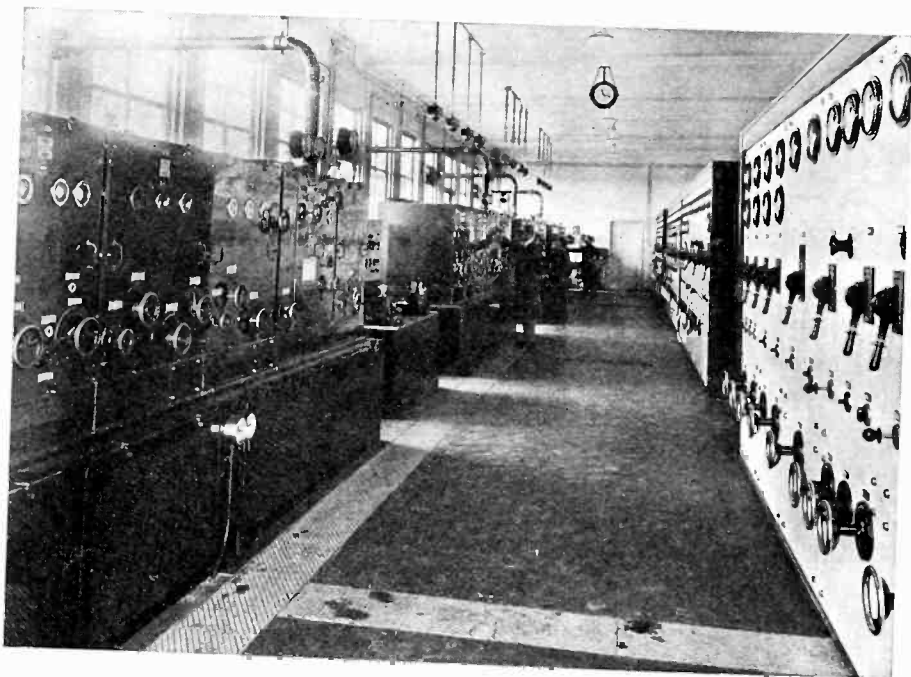
Fig. 14—Transmitting room in short-wave transmitter house II.
