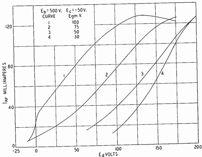
Fig. 15—R-F characteristics UX-865. Screen-grid modulation.
