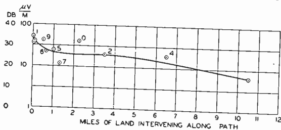
Fig. 3—Strength of signals received at Nantucket on 66 meters as a function of intervening land in path. (Day only.)
