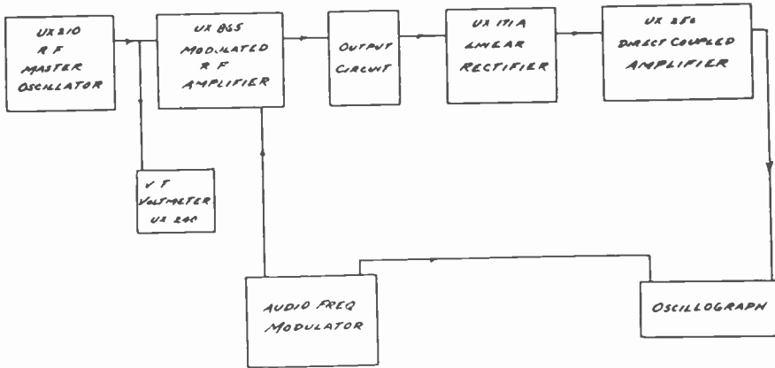
Fig. 1—Block diagram—tetrode modulated amplifier experimental set-up.
