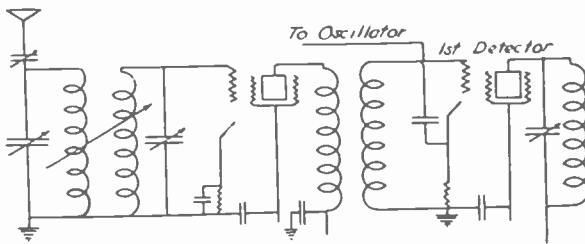
Fig. 1—R-F band selector circuit used in superheterodynes.
