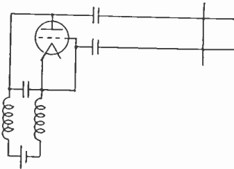
Fig. 1—Regenerative oscillator circuit, White, 1916.
