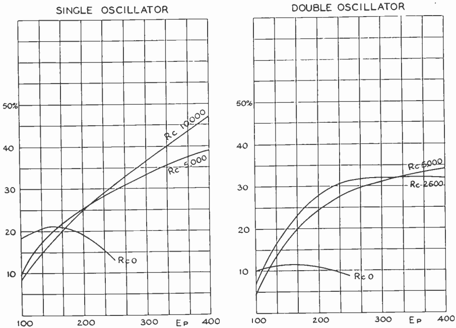
Fig. 6—Plate voltage vs. efficiency.
