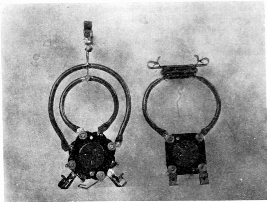
Fig. 2—Single oscillator (right) and double oscillator (left)
