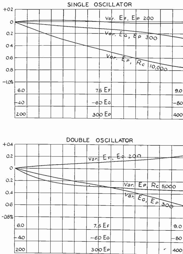
Fig. 11—Frequency stability vs. voltage changes.
