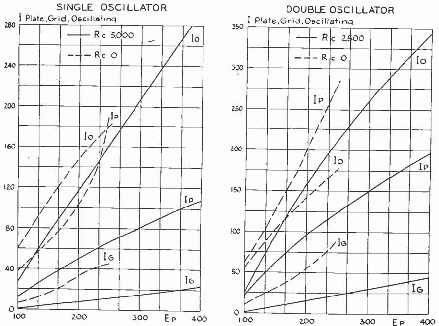
Fig. 5—Plate voltage vs. input, output.
