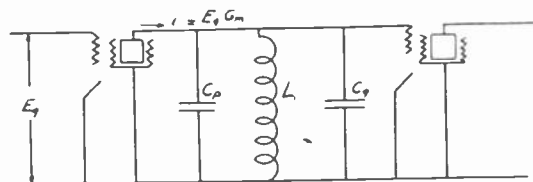
Fig. 3—Battery voltages are disregarded and only r-f potentials are shown.
