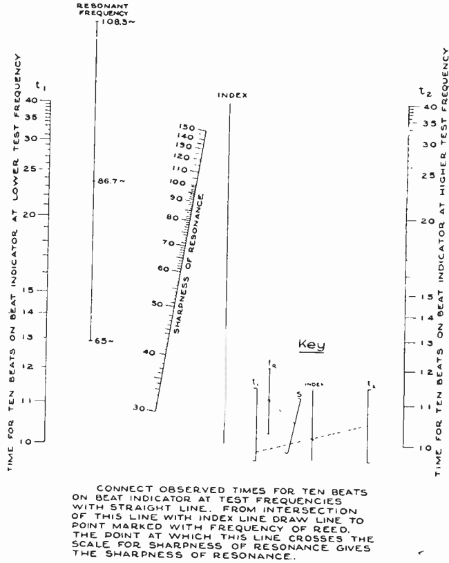
Fig. 10—Chart for determining sharpness of resonance of reeds.
