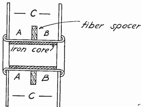
Fig. 5—Construction of aperiodic r-f transformer.
