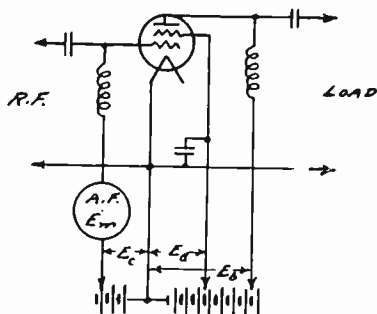
Fig. 5—Grid modulation; screen-grid return to E_d .
