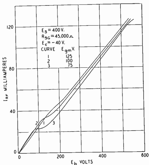
Fig. 24—R-F characteristics UX-865. Screen-grid return to E_s .
