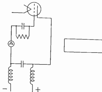
Fig. 2—Regenerative oscillator circuit, Gutton-Touly, 1916.
