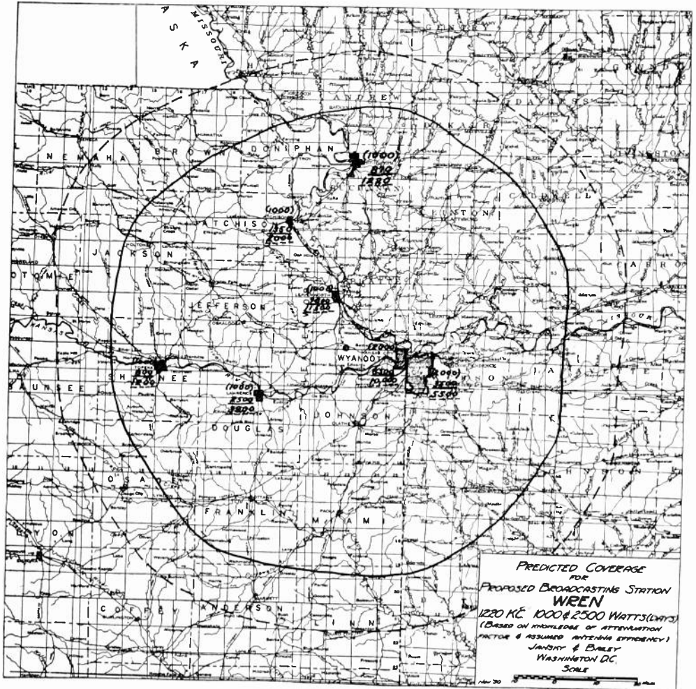
Fig. 3—Estimated coverage for a proposed broadcast transmitter installation, 45 per cent antenna efficiency, rural location eastern Kansas, 1000 and 2500 watts power.
