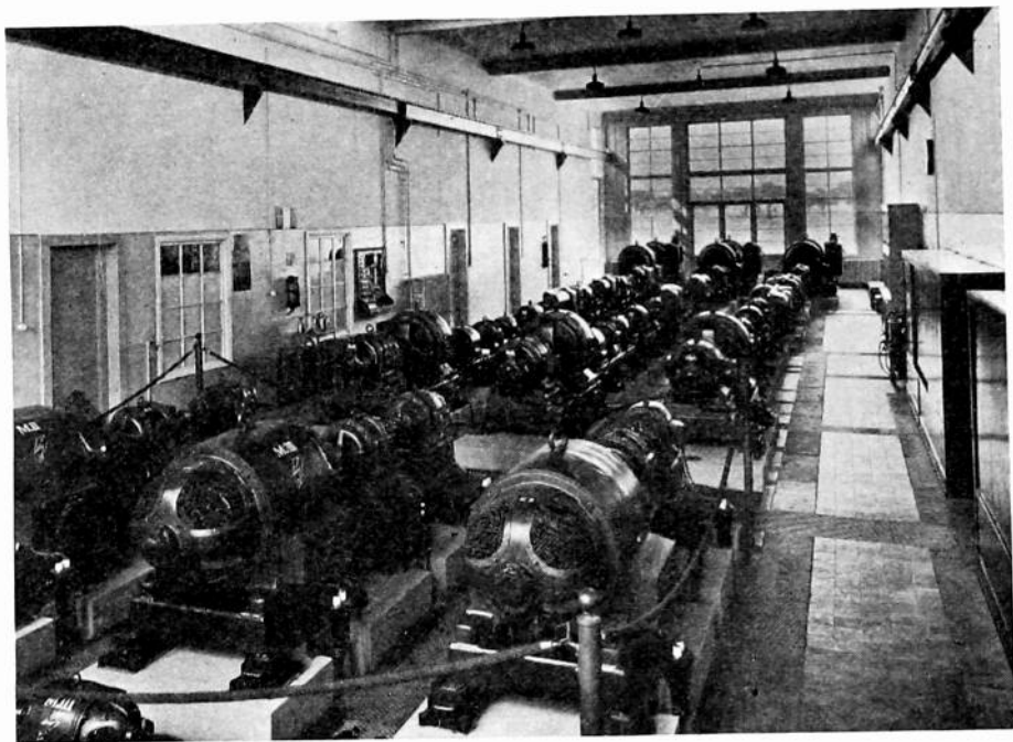
Fig. 15—Machine room of the short-wave transmitter house II.
