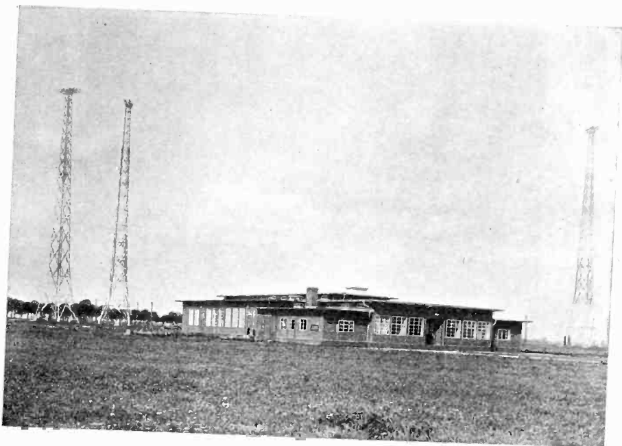
Fig. 13—Short-wave transmitter house II, Nauen, with large directional antenna. (See also Fig. 6.)
