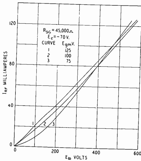
Fig. 30—R-F characteristics UX-865. Screen-grid return to E_b .
