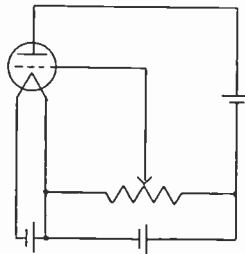
Fig. 5—Electronic oscillator circuit, Whiddington, 1919.
