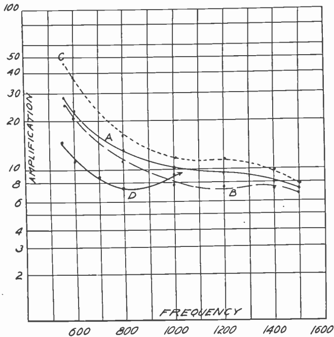
Fig. 7—Comparison of calculated performance with experimental results. A—Calculated amplification curve. B—Experimental curve of same transformer. C—High amplification transformer using extremely low self-capacity windings. D—Part of curve showing effect on low-frequency amplification of trap circuit.
