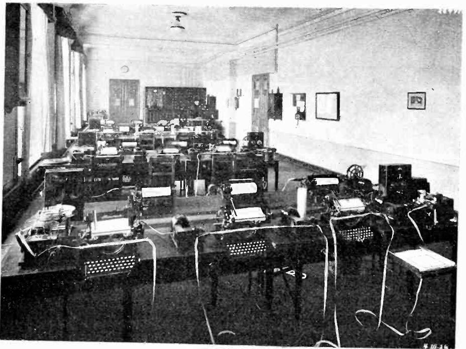
Fig. 5—Receiving table in the Transradio operating central office, Berlin, with recorder, typewriters, and tape movers.
