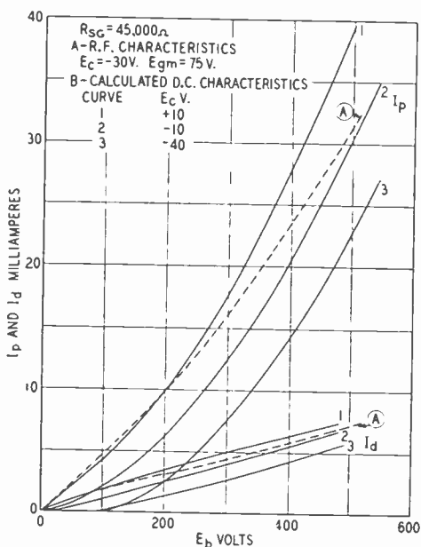
Fig. 37—D-C characteristics UX-865 for screen-grid return to E_b through R_s calculated from normal d-c characteristics. Curve A, an experimental r-f characteristic for a negligible tuned circuit impedance.
