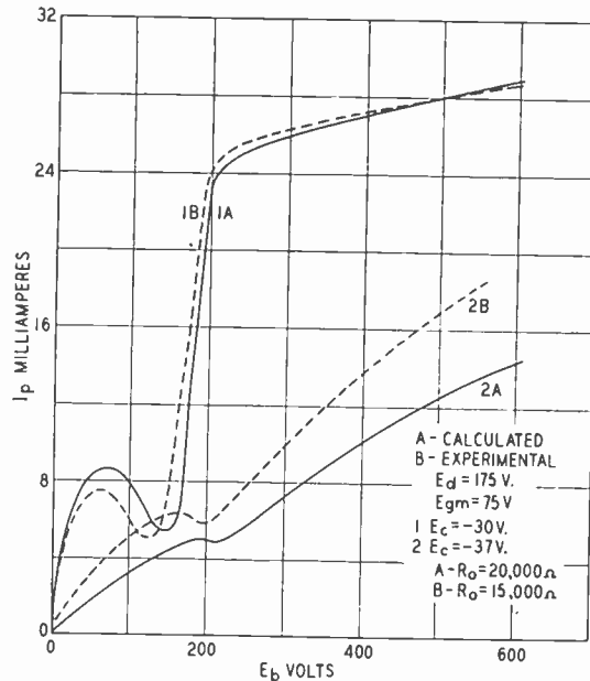
Fig. 35—R-F characteristics UX-865. Comparison of calculated and experimental curves. A—calculated; B—experimental. Note for curve 2A R_0 = 20,000 ohms while for 2B R_0 = 15,000 .
