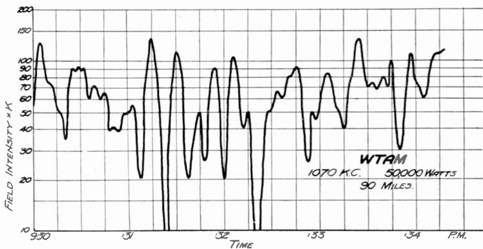
Fig. 4—Fading curves taken at Erie, Pennsylvania on signals from KDKA, 110 miles away and from WTAM, 90 miles away.
