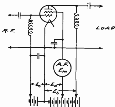
Fig. 7—Screen-grid modulation; screen-grid return to E_d .
