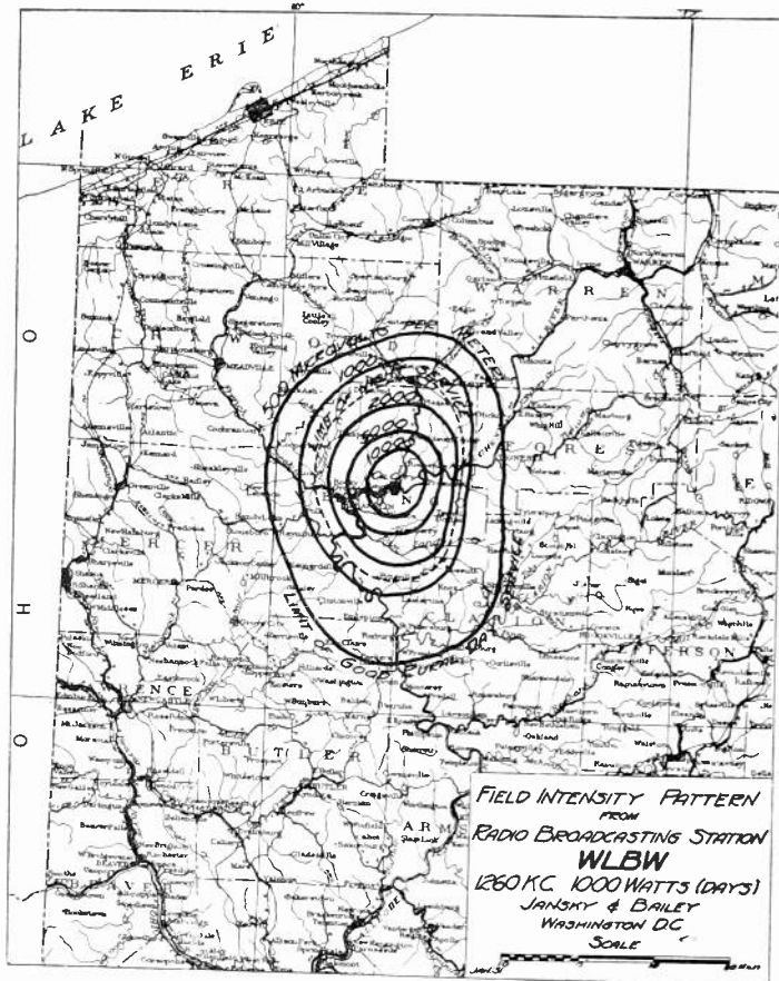
Fig. 2—Field intensity pattern 1000-watt station located in western Pennsylvania, antenna efficiency same as in Fig. 1.
