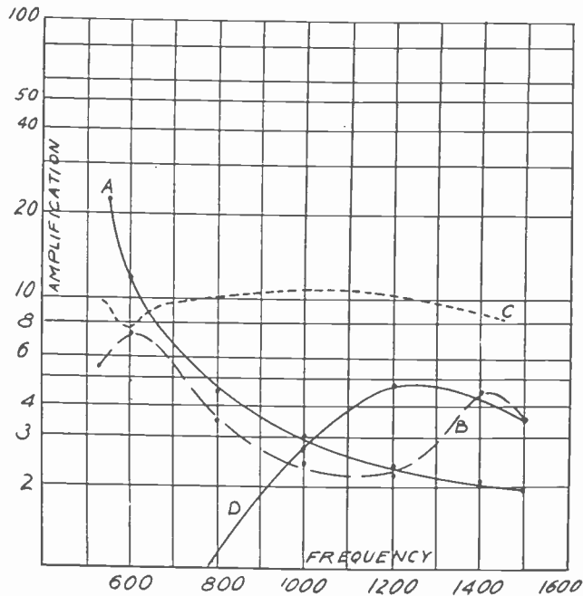
Fig. 2—Amplification curves of various untuned transformers. A—Two wires wound in parallel and resonated below 550 kc. B—Primary resonated at 600 kc and secondary at 1400 kc. C—Primary and secondary wound in single layers on opposite legs of a finely laminated silicon steel core. D—Primary and secondary resonated at the high frequencies.
