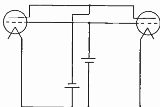
Fig. 8—Electronic oscillator circuit, Scheibe, 1926.
