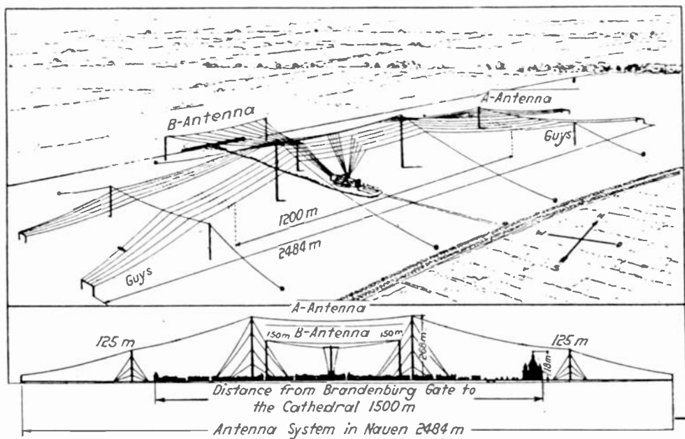
Fig. 6—Antenna system for the Nauen long-wave transmitter, 1920.
