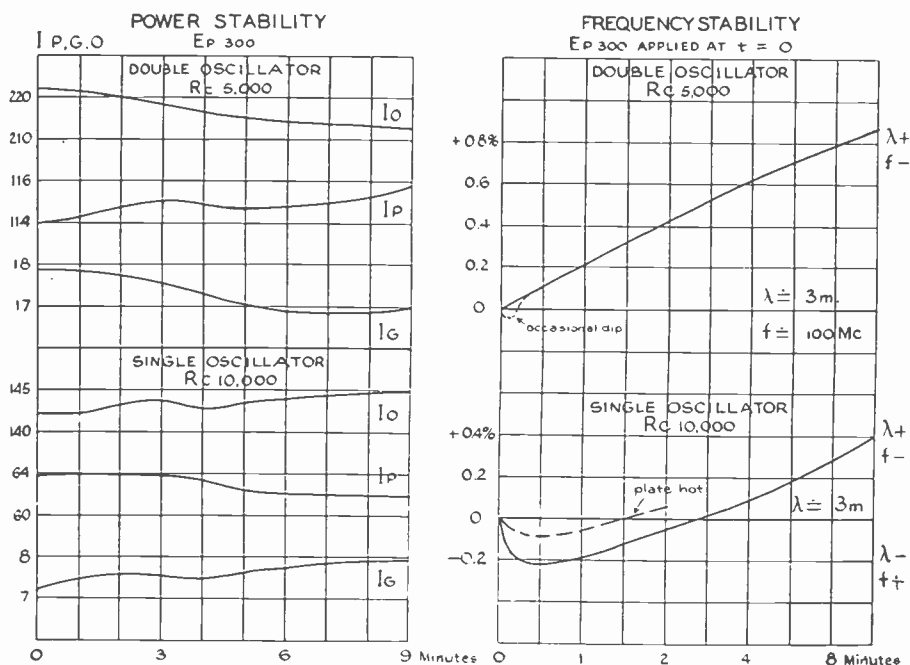
Fig. 10—Power stability and frequency stability vs. time.
