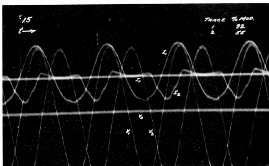
Fig. 38—Oscilloscope for screen-grid modulation method of Fig. 7.
