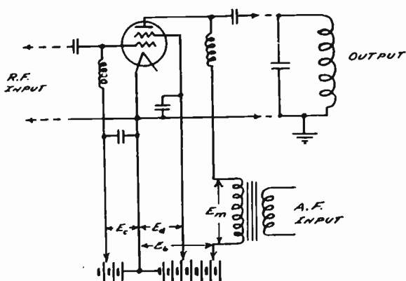
Fig. 9—Plate modulation; screen-grid return to E_s .
