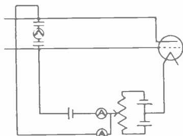
Fig. 7—Electronic oscillator circuit, Gill-Morrell, 1922.
