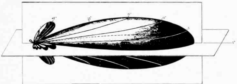
Fig. 20—Approximate three-dimensional diagram. Linear antenna array with reflector. Aperture two wavelengths by eight wavelengths.
