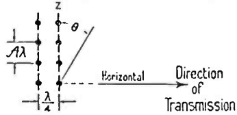
Fig. 17—Vertical plane diagrams due to couplets of coaxial anten
