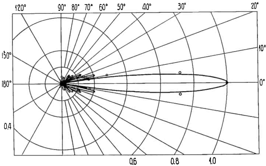
Fig. 11—Calculated directional diagram. Twentyfour couplets spaced one-fourth wavelength. Circles indicate experimental points.
