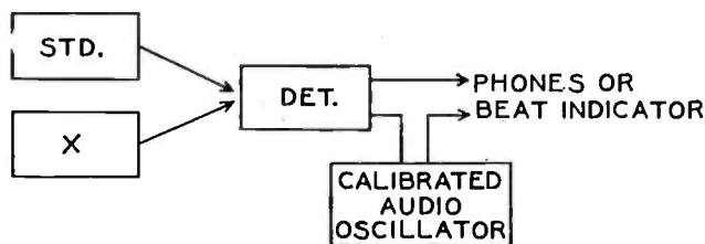
Fig. 2.—A known frequency from the standard source (STD) and the unknown frequency ( x ) are impressed on a detector. The difference beat frequency resulting is matched by a frequency from a calibrated audio oscillator, the matching being indicated by telephones as beat indicator.
