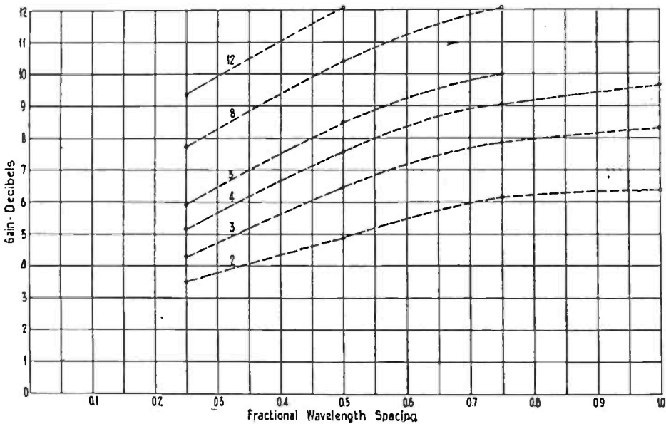
Fig. 19—Calculated gains from stacked antennas.
