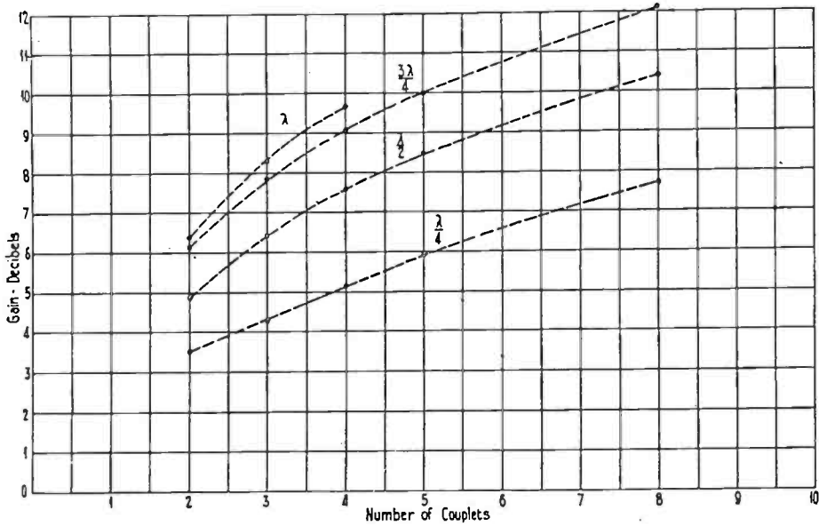
Fig. 18—Calculated gains from stacked antennas.
