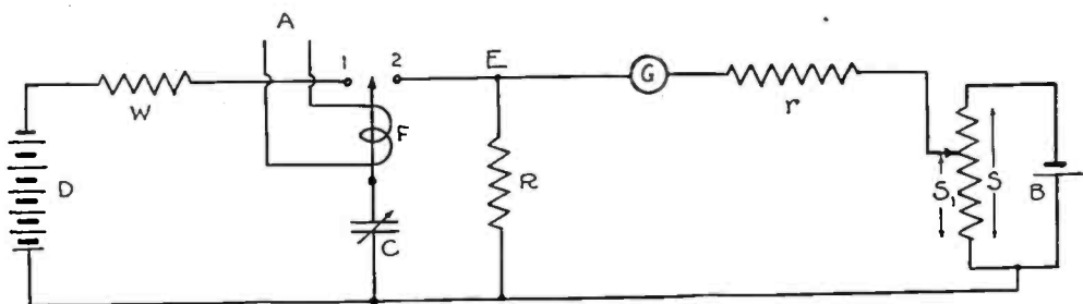
Fig. 2—Schematic diagram of circuit arrangement used for measuring low frequencies.
