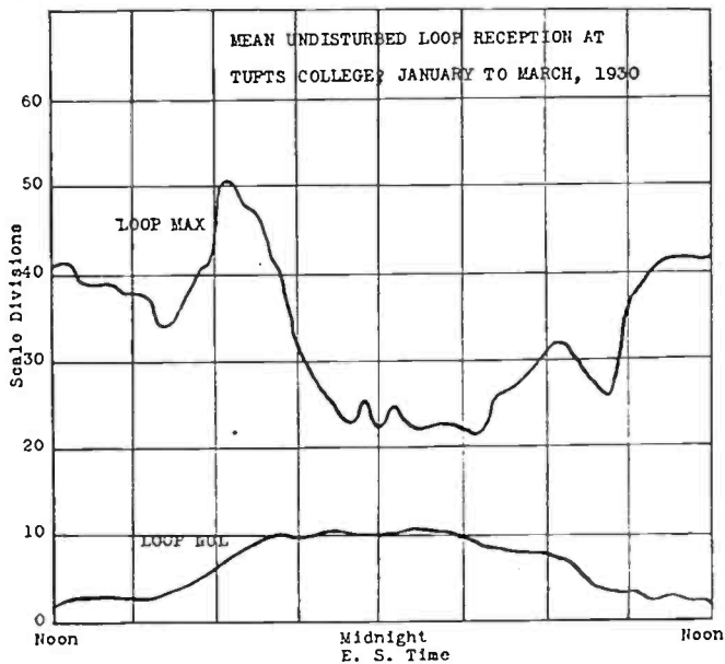
Fig. 9—Mean loop reception. Note polarization during night.
