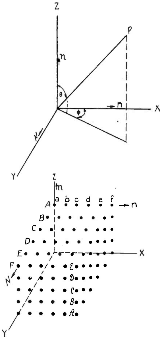
Fig. 21—General case of linear antenna arrays.
