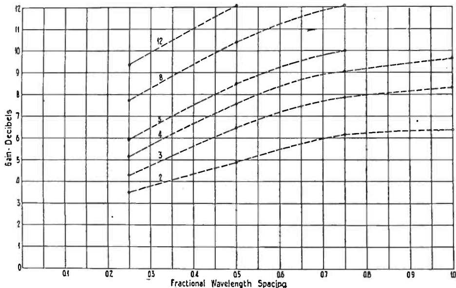
Fig. 19—Calculated gains from stacked antennas.
