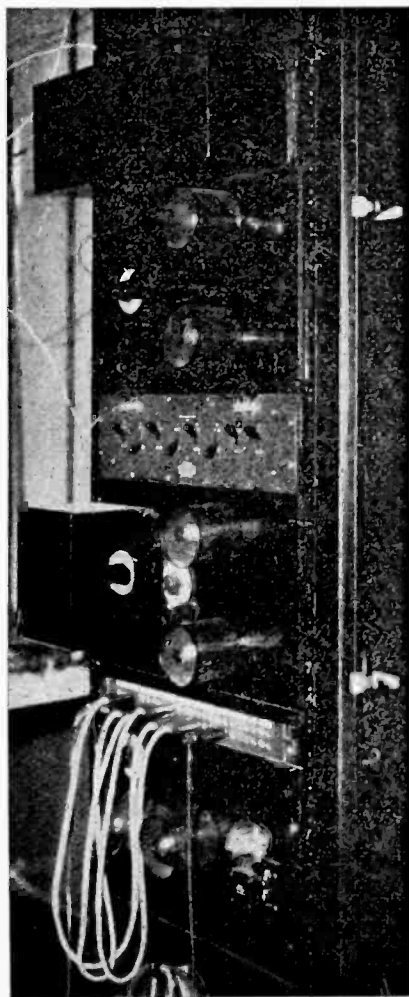
Fig. 7. Front view of recorder amplifier.
