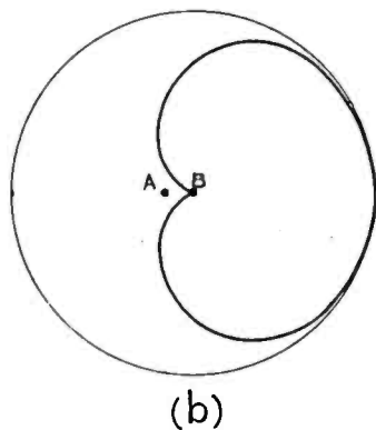
Fig. 2—Interference pattern. Two sources separated in space by one-fourth wavelength and in time by one-fourth period.
