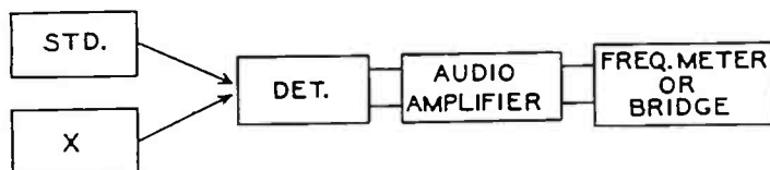
Fig. 3 - The known and unknown frequencies are impressed on a detector and the difference beat frequency resulting is amplified sufficiently to operate a direct-reading frequency meter, a frequency bridge, tape recorder, or similar devices.
