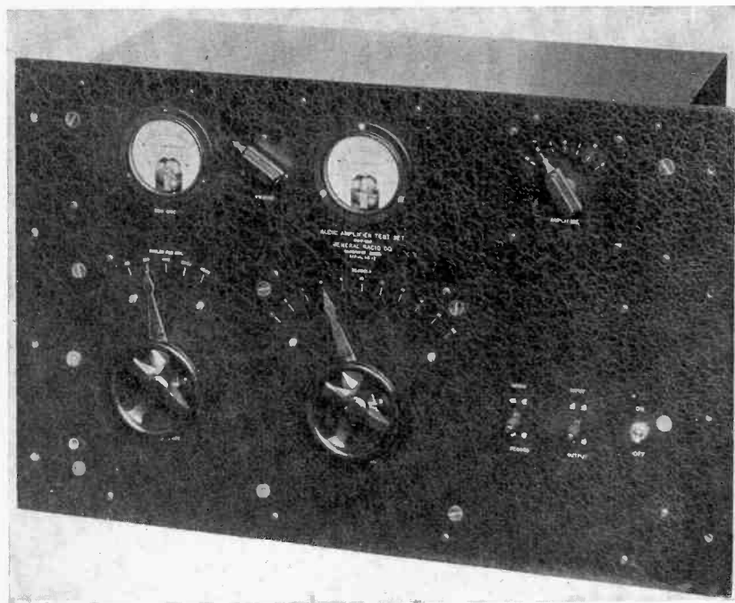
Fig. 7-A—Front view of a complete testing panel used by the Audio Vision Appliance Company of Camden, N. J.
