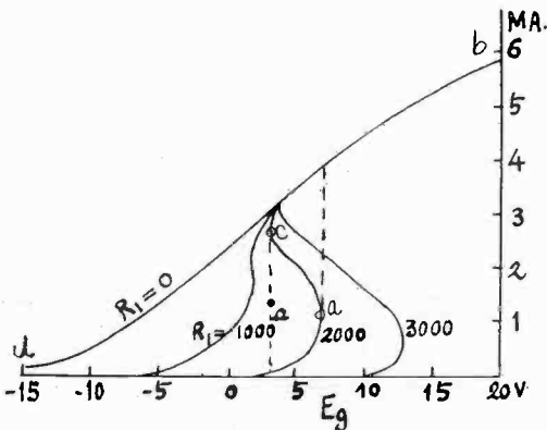
Fig. 3—Heegner's experimental result.
