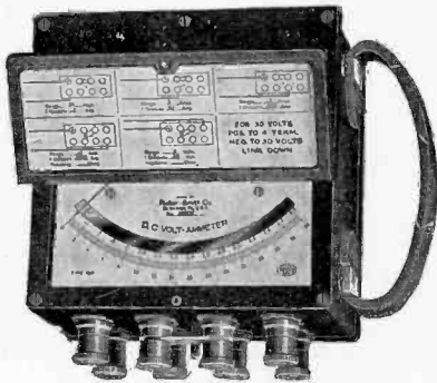
Type ISD VOLT-AMMETER
