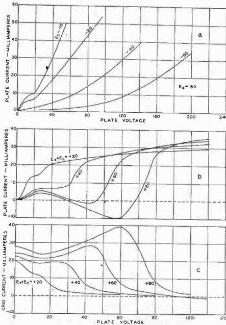
Fig. 17—Secondary electron effects in co-planar grid tube.
