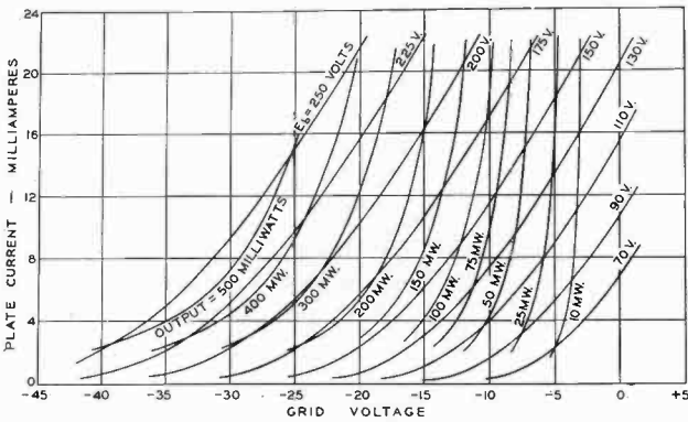
Fig. 1—Type 101-D tube. Characteristic curves and fundamental output power for a sinusoidal input voltage whose peak value, v , is equal to the grid potential, E_c , at all points. The load resistance, R , is equal to the plate resistance, R_p .
