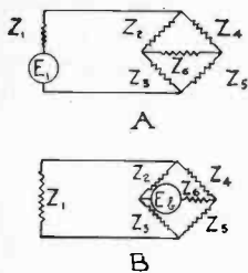
Fig. 3— E_b = E_3 - E_5 ( Z_6 open) I_s = I_2 - I_3 ( Z_6 shorted) Z_b = E_b / I_s I_6 = \frac{E_b}{Z_6 + Z_b}
