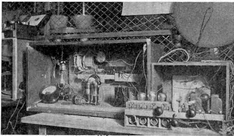
Fig. 4—Photograph of oscillator, filter, and receiver setup.
