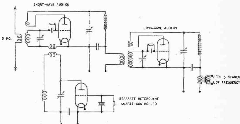
Fig. 7—Quartz-controlled short-wave receiver with intermediate frequency.
