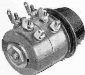
No. 590-590. Metal shell, composition element only. Resistances from 5,000 ohms to 1 megohm. All curves. Potentiometer or rheostat types. Units insulated from each other. Diameter, 1 5/16 in. Depth of shell, 1 1/8 in.
