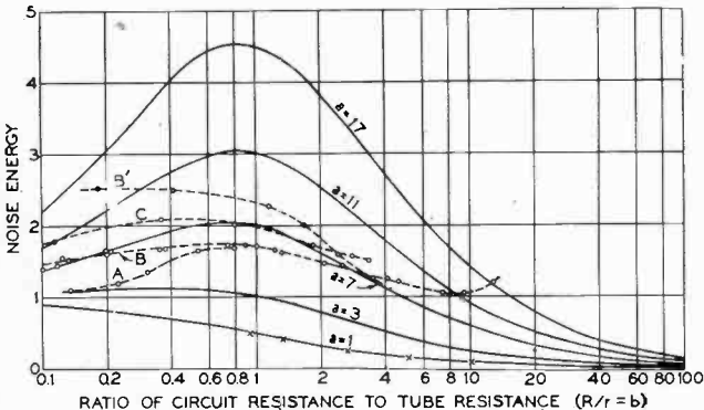
Fig. 3—Noise from thermal agitation in the plate circuit when the plate resistance is varied. The various curves are for different values of filament temperature.
