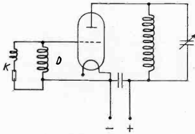
Fig. 3—Quartz-controlled transmitter. Representation of the impedance of the quartz crystal.
