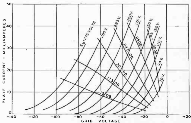
Fig. 5—Type 104-D tube. Second harmonic, F_2 , in decibels below the fundamental, F_1 . v = E_c ; R = R_p .
