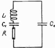
Fig. 6—Equivalent circuit diagram of the quartz crystal.
