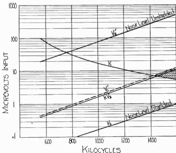
Fig. 2—The relation between useful receiver sensitivity and ignition interference level. V_2 = microvolts input for nearly complete shielding, V_2' = microvolts input for no shielding, V_1' = ideal sensitivity characteristic for receiver, V_1 = common sensitivity characteristic of a receiver.
