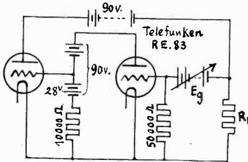
Fig. 2—Circuitual arrangement for obtaining characteristic of regenerative resistance amplifier (Heegner).
