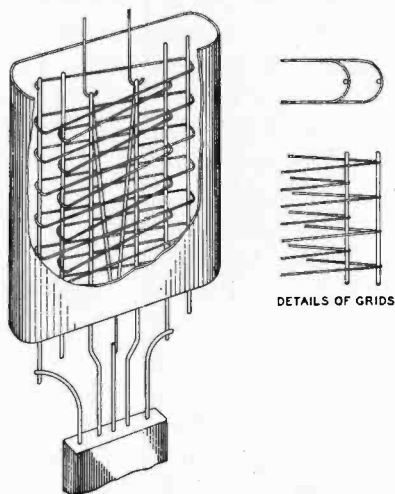
Fig. 11—Schematic diagram of co-planar grid tube.
