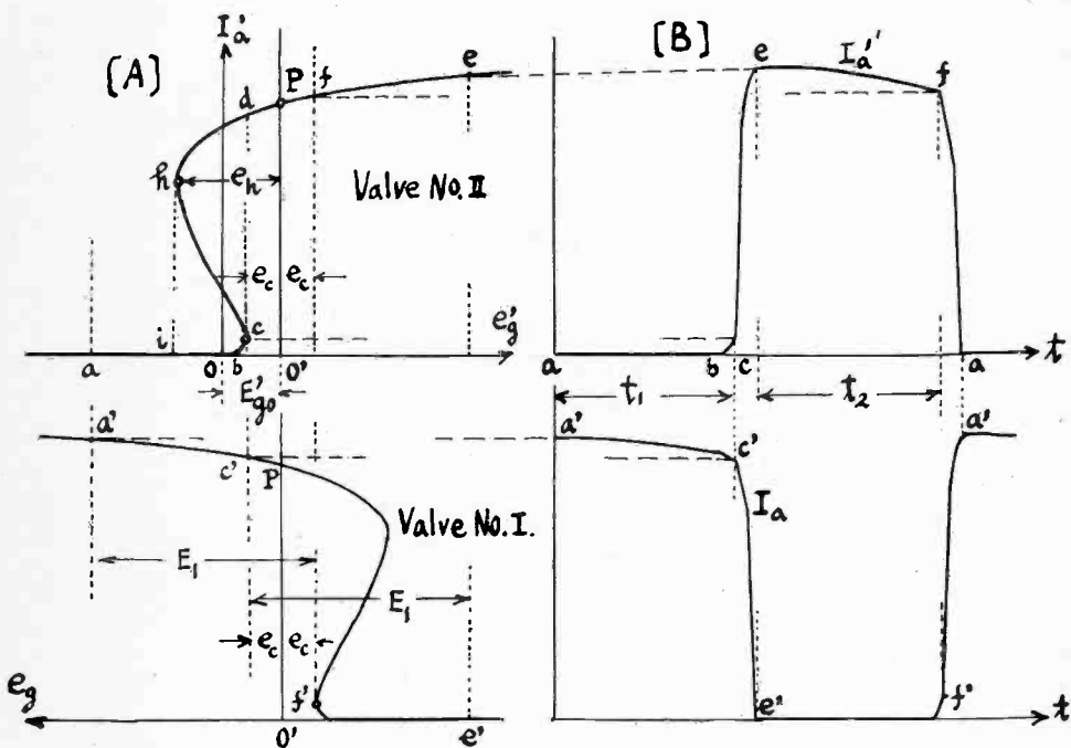
Fig. 8—Diagrams showing the oscillation cycle.
