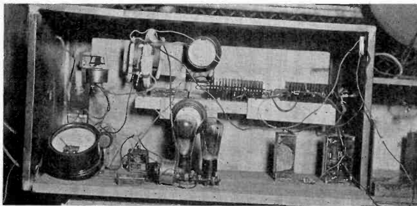
Fig. 6—Close view of oscillator.
