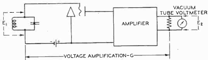
Fig. 2—Circuit to illustrate method of detecting or measuring noise from the thermal agitation of electricity in conductors.
