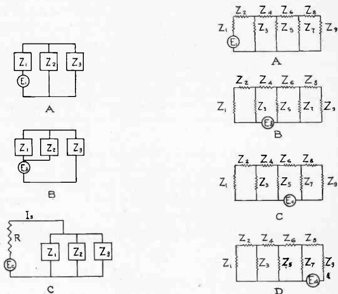
Fig. 2—Each of above circuits has same value of current in Z_3 E_b = voltage across Z_3 if Z_4 is opened in circuit A E_c = voltage across Z_6 if Z_6 is opened in circuit A or B E_d = voltage across Z_7 if Z_8 is opened in circuit A, B, or C.
