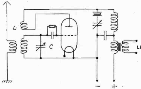
Fig. 4—Quartz-controlled oscillating audion with additional feed back.
