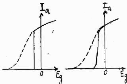
Fig. 10—Non-falling characteristics.
