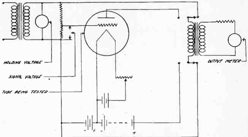
Fig. 8—Circuit arrangement for the a-c test.
