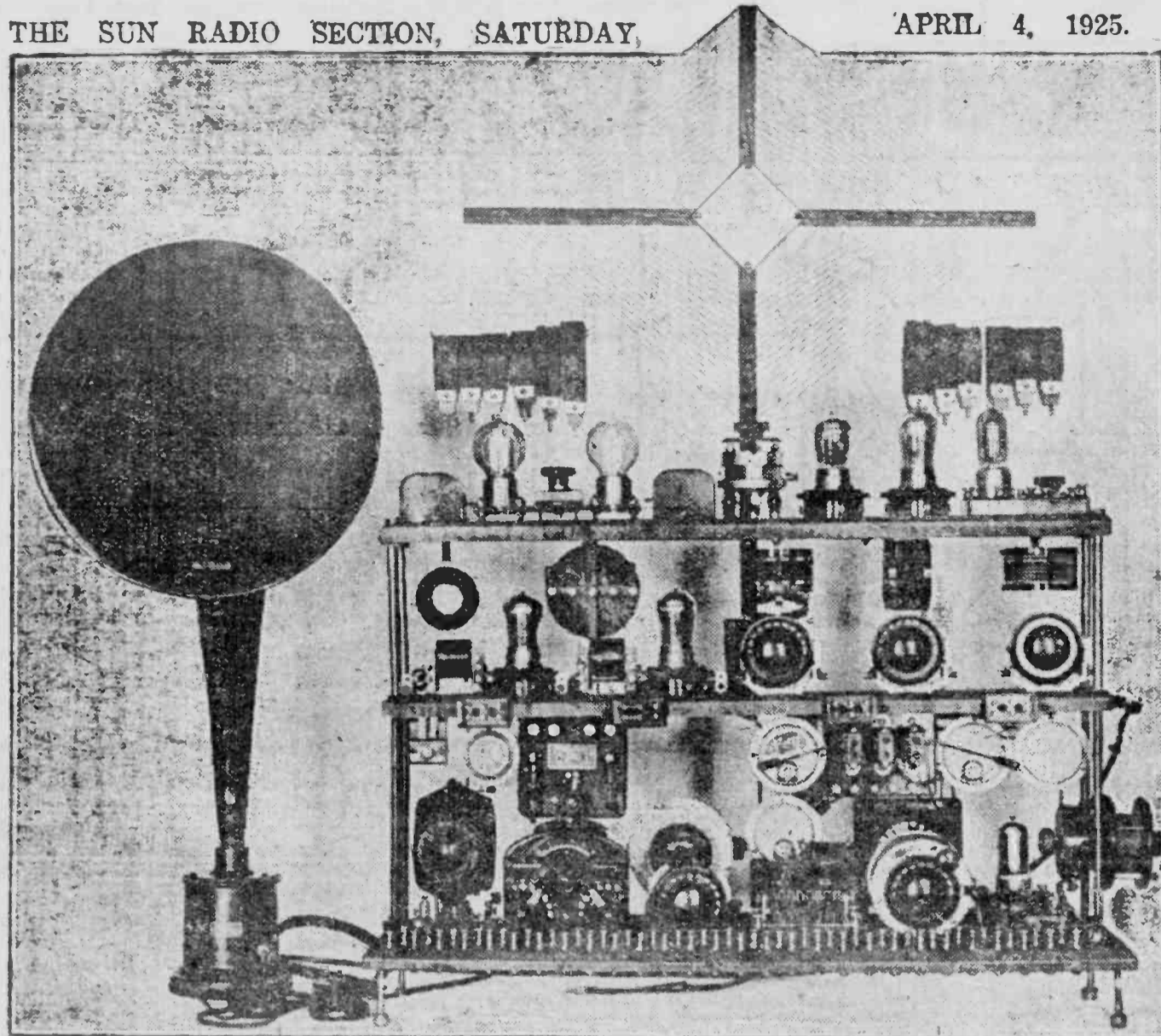
A view of Mr. Fox's set showing layout of apparatus. Note array of 60 binding posts on base.
