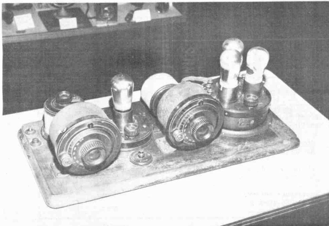
The Atwater Kent Model 9 breadboard, a jewel in the collector's treasures.
