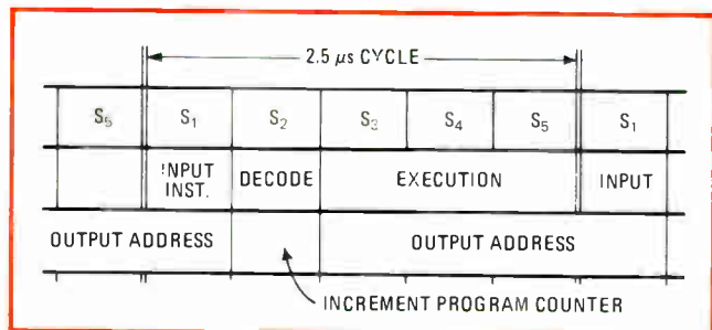
3. Simple. Operating the 8748/8048 is extremely straightforward, with each 2.5- \mu s cycle consisting of five states. Instruction inputs are made in state 1, decoding and program incrementing in state 2. Program executions begin in state 3 and run through 4 and 5.
