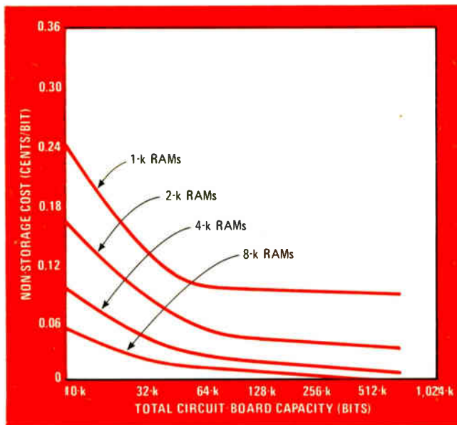
6. Non-storage. The memory cost per bit for non-storage hardware varies with device density, as well as the total bit capacity built onto one printed-circuit board. The curves tend to flatten out beyond the point of maximum capacity for typical pc boards.
