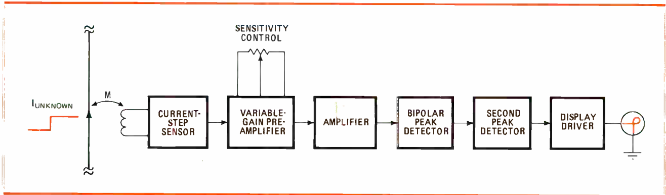
2. Gain stages. The voltage induced from an unknown current spike as small as 1 milliamperere requires multiple stages within the tracer to be amplified and stretched enough to drive an incandescent lamp to visible levels.
