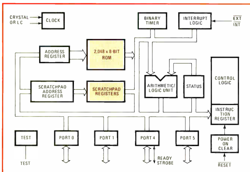
New chip in town. Mostek's one-chip F-8 has a 2-kilobyte ROM and extensive scratchpad facility to increase performance at about half the price of two-chip version.
