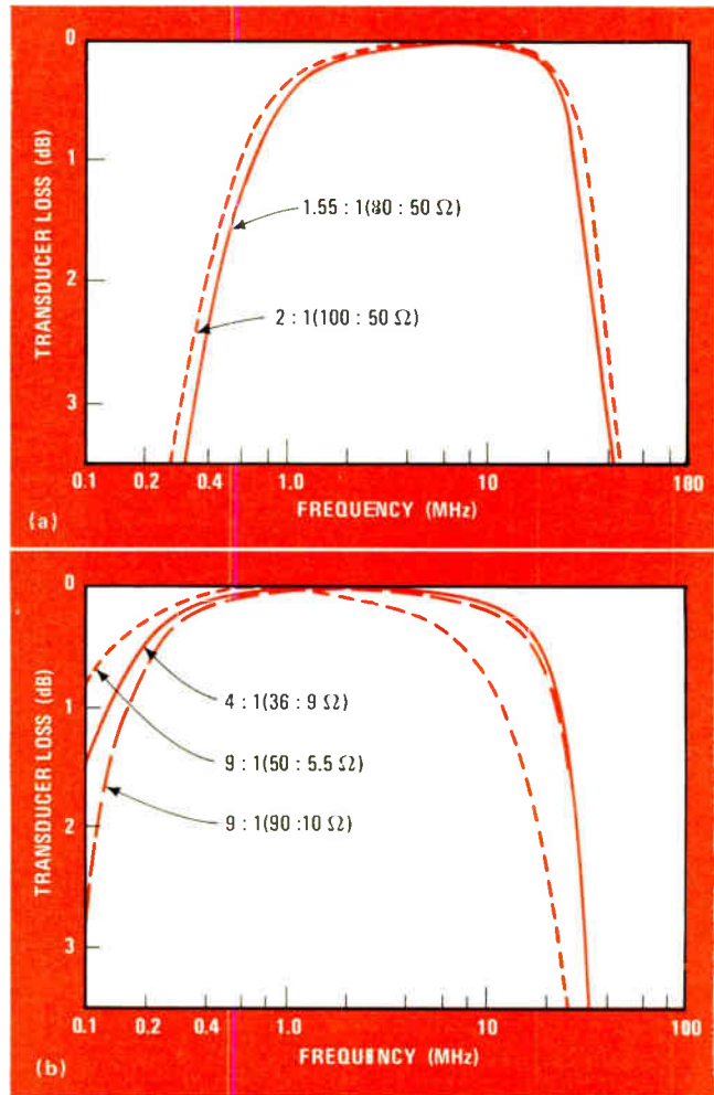
7. Plotting response. The characteristic impedance is optimum for the 4:1 transformer but for the 9:1 transformer only when matching 90 to 10 ohms, not 50 to 5.5 ohms. For the latter case this less-than-optimum impedance causes a more rapid falloff at high frequencies, but, since an inductive reactance of only 5.5 ohms, not 10 ohms, has to be exceeded, the low-frequency end is improved.
