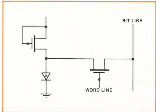
7. As a memory cell. If the lambda diode is fabricated with complementary-MOSFETs, a complete unit cell for a static C-MOS memory can be built with only four transistors, rather than the six normally required for the conventional C-MOS memory cell. The size of a memory chip, therefore, can be reduced by about two thirds.
