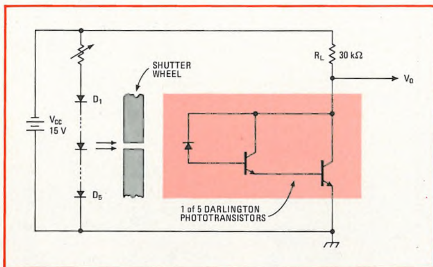
Light dial. Combinations of light-emitting diodes and phototransistors do the job of an electromechanical dial selector on new spectrum analyzer from Tektronix Inc.
