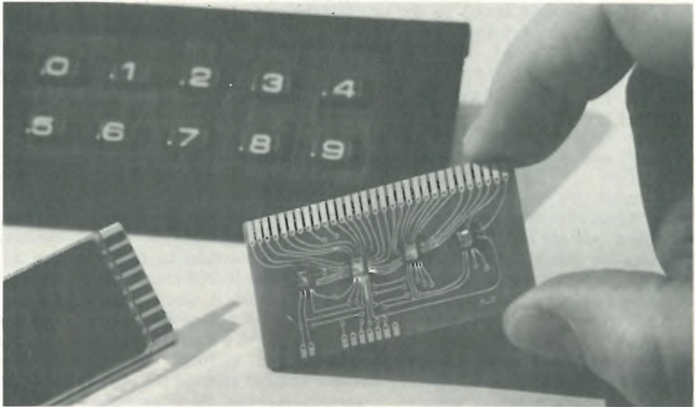
Polished. Digital tuner from F. W. Sickles is said by its manufacturer, a division of General Instrument, to be inexpensive enough for eventual use in all color receivers. It's based on MNOS memory.
