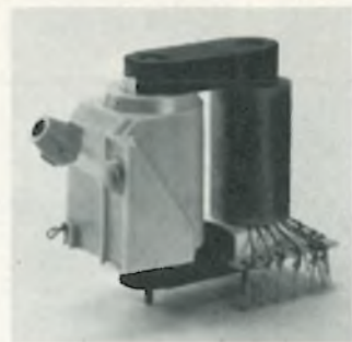
Diode-split transformer
