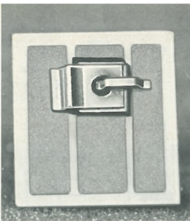
5. Power in chip form. SCRs, triacs, and diodes are available from Unitorde Corp. as fully glass-passivated devices in solderable chip form. Voltage ratings for this ChipStrate family go up to 600 V at currents of 1 to 55 A. General Electric offers a similar line.
