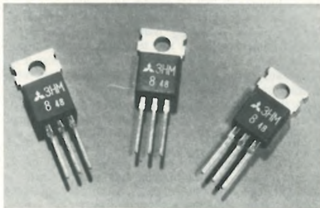
9. Plastic for high current. SCR rated at 400 V and 180 A is packaged in plastic for electronic photoflash applications. Made by Mitsubishi, the device has such a small charge storage that it can be turned off by an auxiliary commutation circuit in a mere 6 \mu s.
