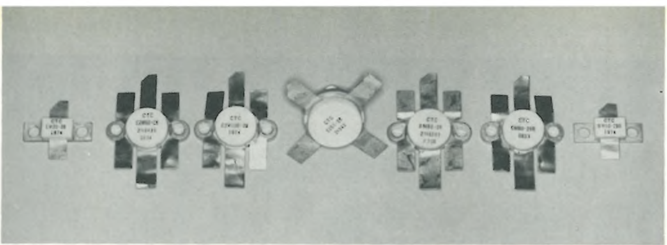
11. Communications lineup. Rf and microwave bipolar transistors made by Communications Transistor Corp. are available in a variety of stripline packages, including the newer rectangular ones that can accommodate bigger chips for higher power outputs.
