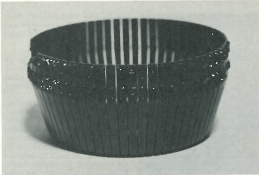
System crown. Print head for Badminton machine has 128 characters. Rotation is controlled by one dc servo and elevation by another. Impact hammer is inside head.
