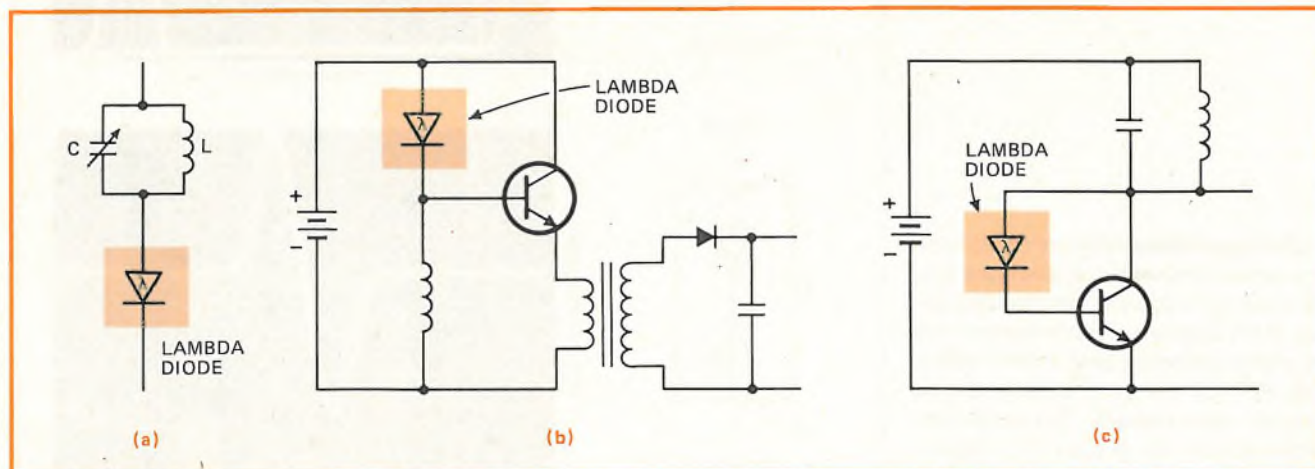
5. As an oscillator. Building a sine-wave oscillator (a) is easy with the lambda diode—it is merely connected in series with an LC tank circuit. Similarly, the device can be used for a voltage-step-up circuit (b) or for a blocking oscillator (c).
