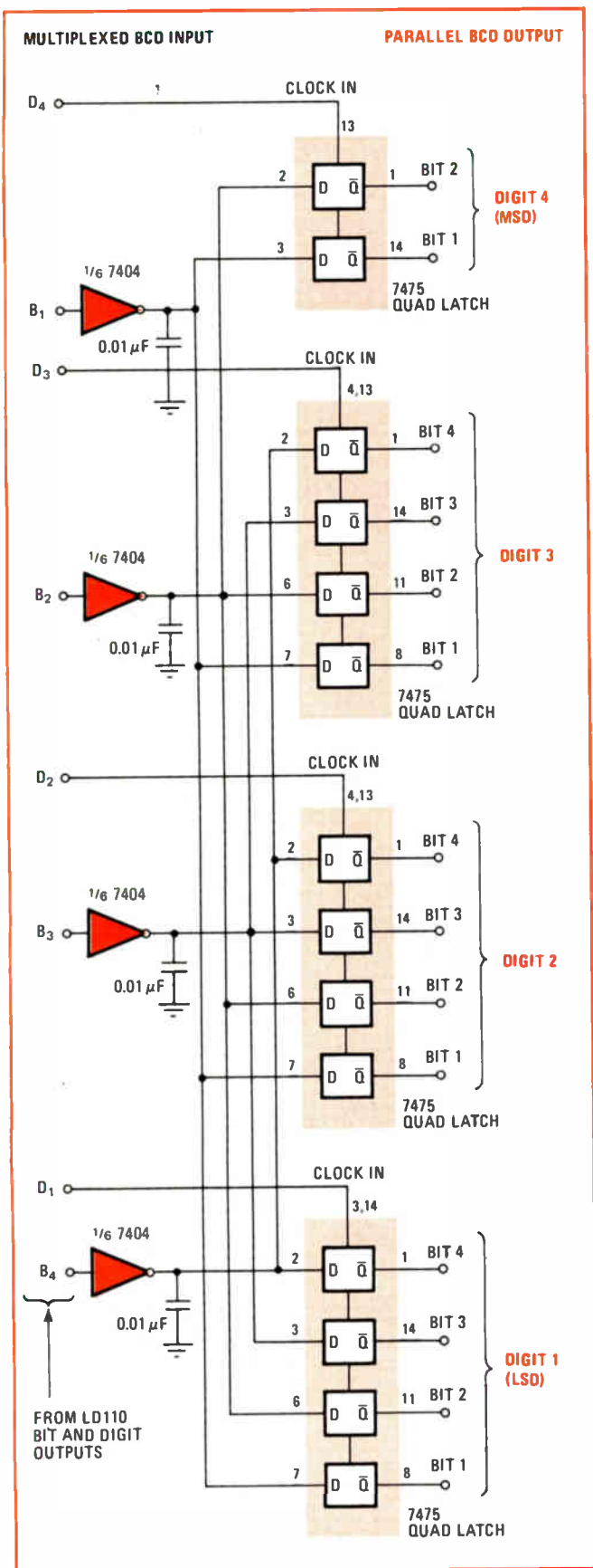
11. Parallel output. For those jobs where the BCD data for all four digits should be available in a parallel format—for example, as printer inputs—this multiplexed-BCD-to-parallel-BCD converter has four quad bistable latches activated by LD110 output.
