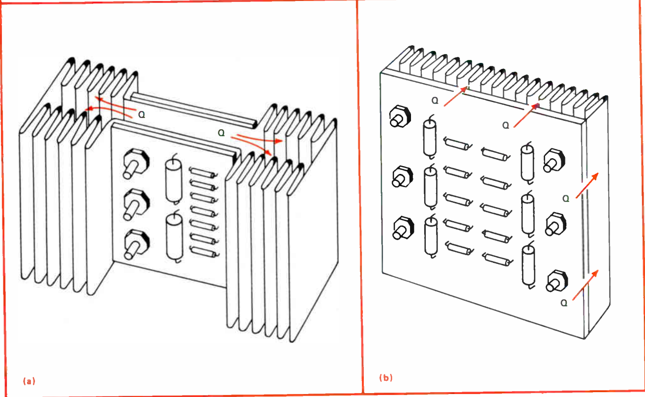
4. Go coplanar. The in-line construction (a) accounts for the large temperature rise—90.1°C. By contrast, the heat-transfer path in the coplanar structure (b) is very short, and temperature rise is significantly less—66.1°C.
