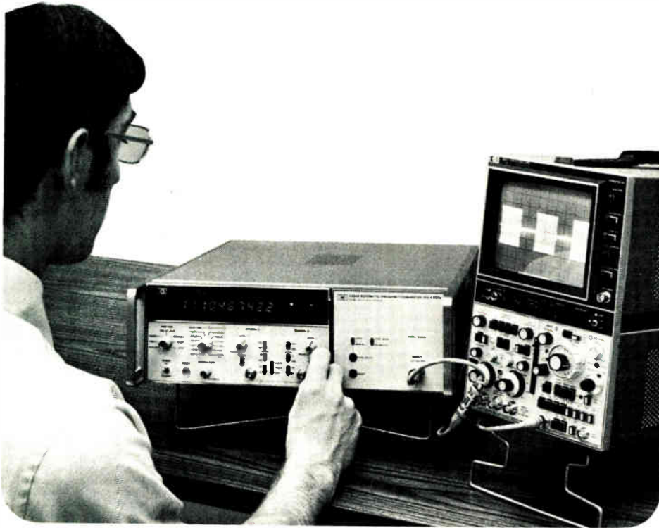
Pulsed RF and CW up to 4 GHz are measured automatically with a heterodyne converter plugged into the new counter.
