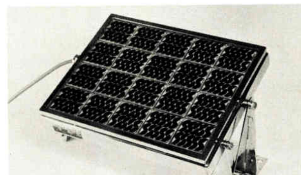
Safe harbor. With packing demands less critical than those of space, terrestrial arrays use all the silicon in a wafer. Cells from Sharp Corp. provide power for this Japanese lighthouse.
