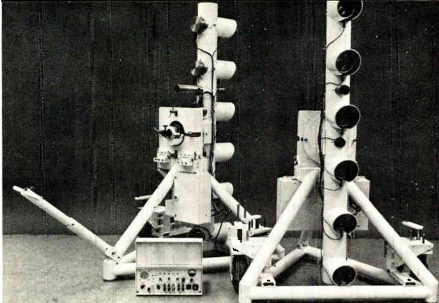
Intruder detector. Laser fence has six devices in vertical row. Their beams are picked up by optical receiver. Small instrument is local collector/display unit of the system.
