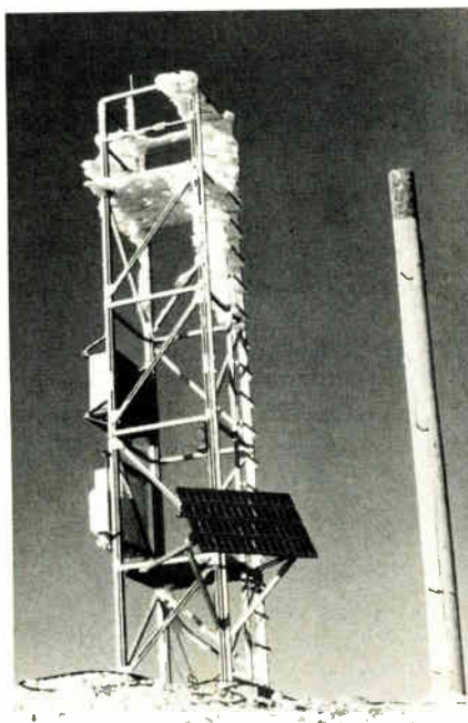
3. At work. Arrays from Solar Power Corp. are being put to use aboard offshore oil rigs (below). NASA's plastic-encapsulated cells get snowy test at Mammoth Mountain, Calif. (right), while 3-W array from Centralab provides power for stream-gaging telemetry.
