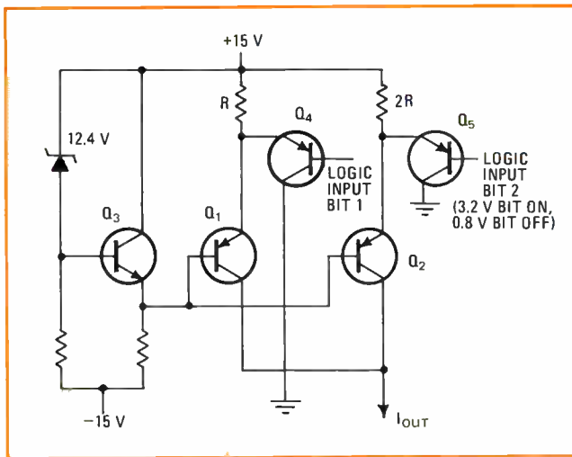
3. Pnp-pnp. Replacing diodes of Fig. 2 with transistors eliminates diode storage times and thus raises speed, but this change does not affect problems of changing current gain and base-emitter voltages.
