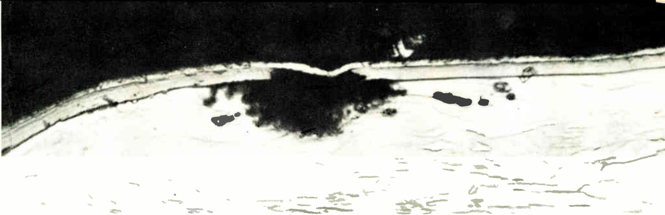
1. Trouble. If pores exist in gold plating, contaminants can destroy the contact face. This contact was attacked by a nitric acid vapor that in just two hours penetrated the 30 microinches of gold, attacked the nickel underplate, and ate into the copper beneath.
