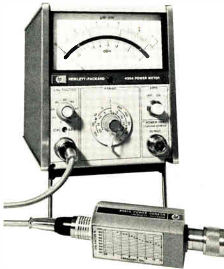
The 435A power meter's internal RF power reference provides added confidence in overall measurement accuracy.
