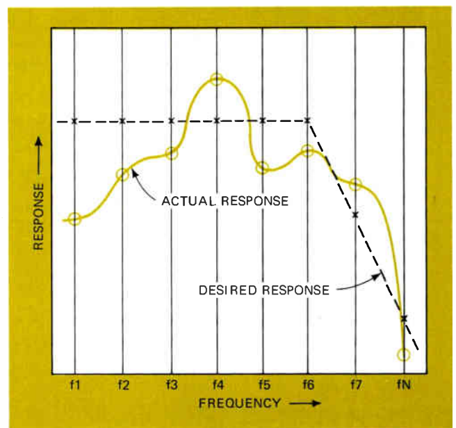
1. The optimization process. Magic optimizes a circuit design by minimizing a weighted error function that represents the difference between the desired response and the actual response. Optimization is done only at the frequencies specified by the user.
