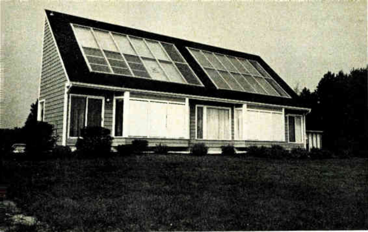
6. Test house. Under direction of Karl W. Böer (right), Institute of Energy Conversion has built Solar One, an experimental house for testing solar-heating and cooling methods and cadmium-sulfide solar cells (the darker panels at lower left on the roof).
