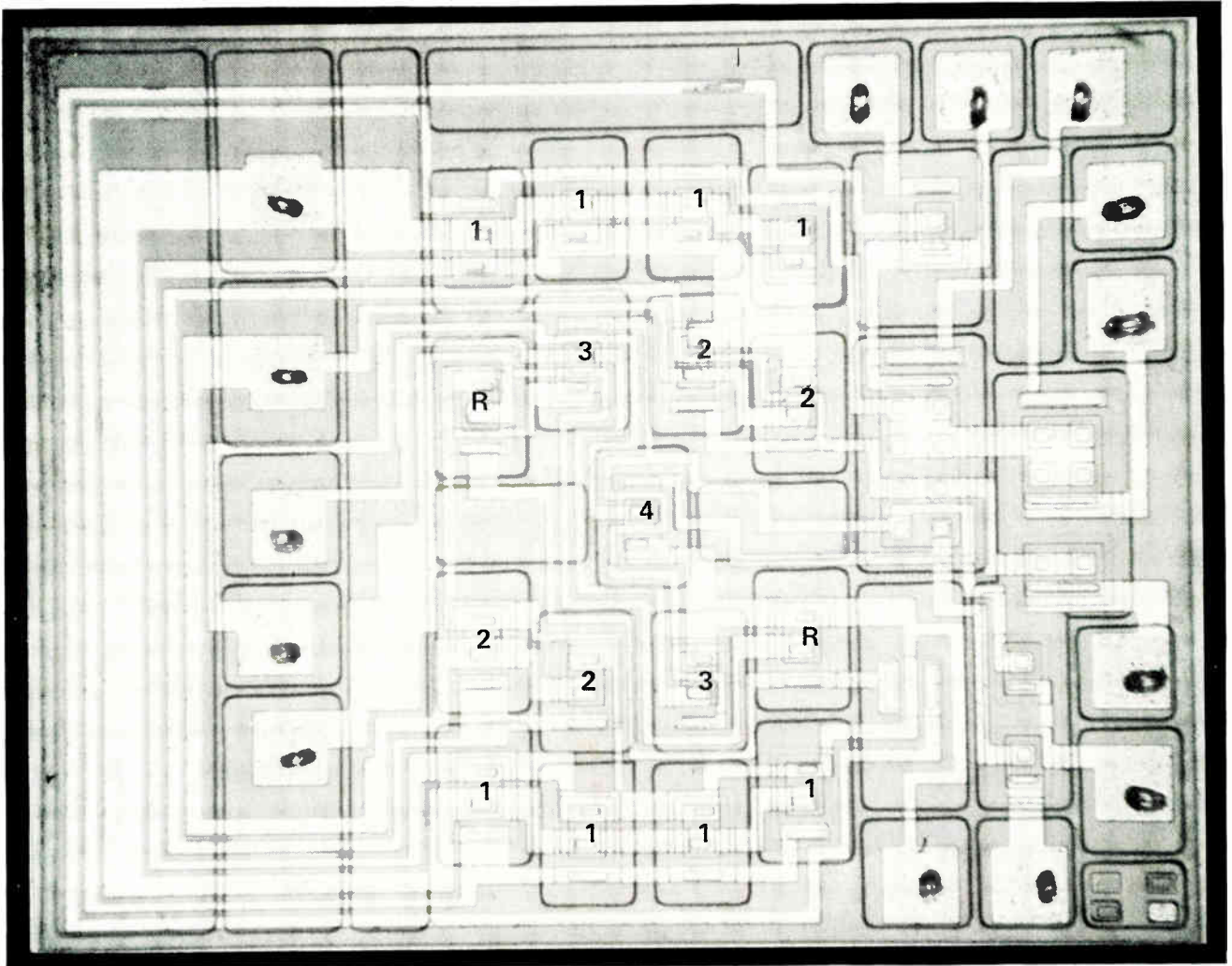
7. Current-steering geometry. Multiple-bit transistors are arranged symmetrically around geometric center so that gradients tend to average out—eight transistors for bit 1, for example, have same average temperature as four transistors for bit 2.
