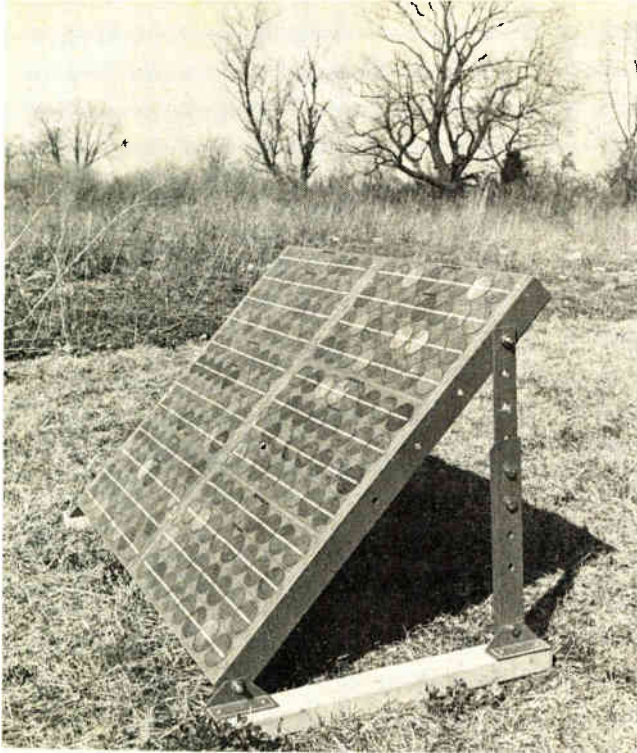
2. Solar arrays. Six 9¾-by-18-inch modules are put (left) into a 50-watt (at peak) array from Solarex Corp. NASA's Lewis Research Center is experimenting with encapsulating space-type solar cells between sheets of plastic for structural strength and easy handling.
