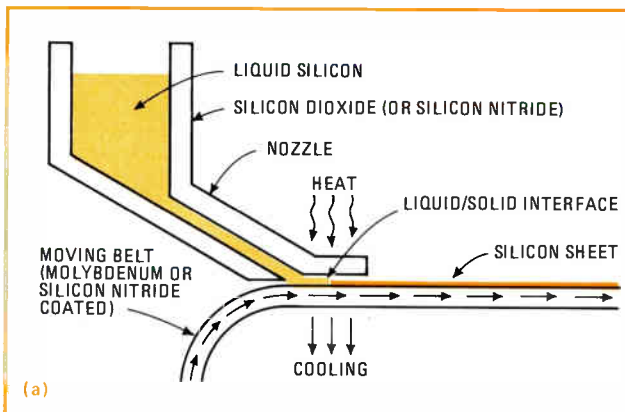
4. Mass production. The possibility of producing silicon in sheets at least a meter wide (left), is being considered by the University of Pennsylvania. Pn junctions could be diffused the length of the sheet, which could be processed sequentially at individual work stations.
