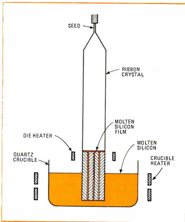
5. Another way. Ribbon-growing method at Tyco Laboratories entails pulling single-crystal silicon from melt through die. So far, inch-wide ribbons 18 inches long have been formed.
