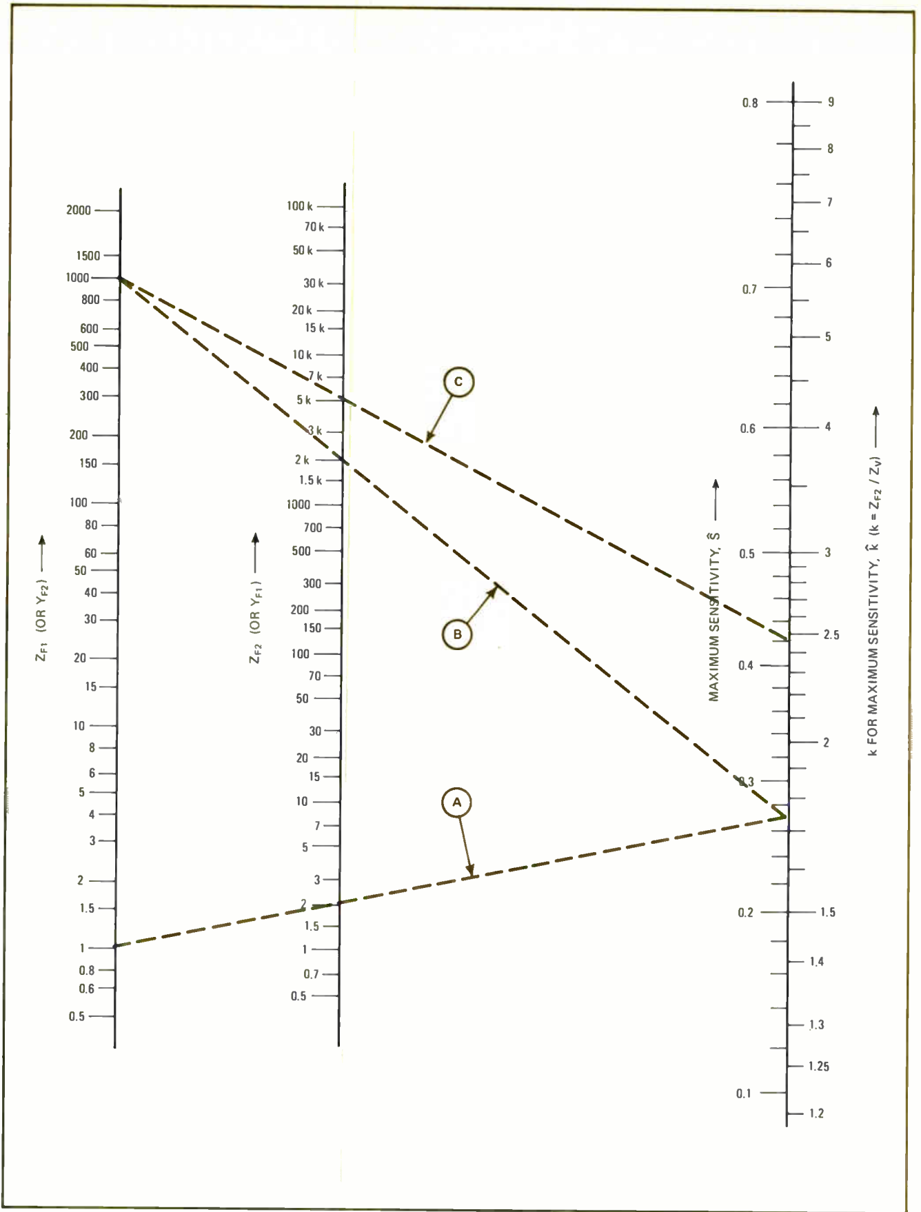
4. Design aid. Nomograph helps to determine the fixed-component values needed to limit the maximum sensitivity of the improved network. The value of impedance ratio \hat{k} can also be read from the same right-hand axis. The left-hand and center axes can be used for impedances (resistors and inductors) or admittances (capacitors). Units for values must be consistent within the same determination.
