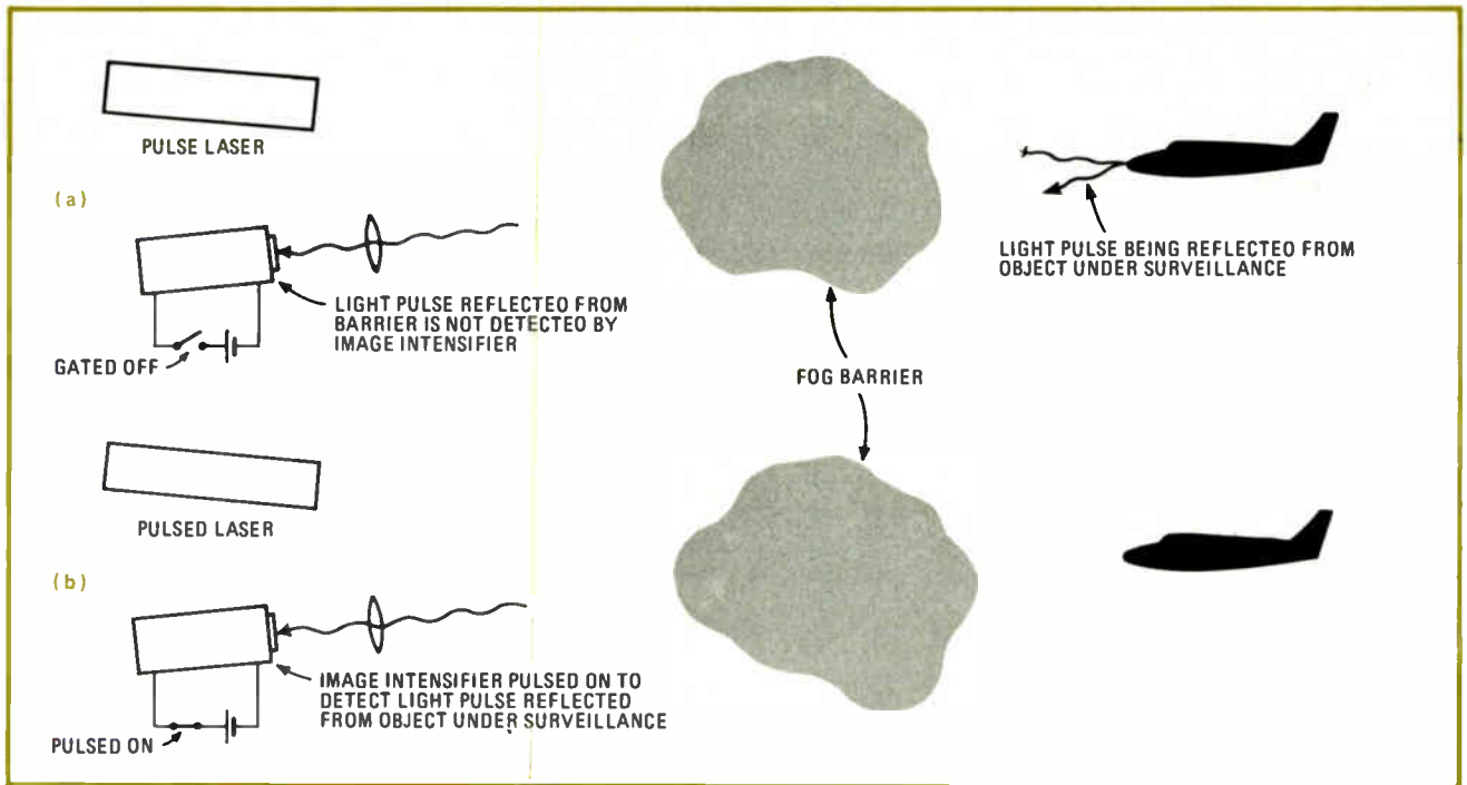
9. Clearing the fog. Gated viewing system makes use of image intensifier to "see through" fog barrier. Intensifier is gated off during period in which light is being reflected from barrier (a), but is pulsed on when light is reflected from target (b). High-gain intensifier system is capable of reducing the barrier-to-target illumination ratio by factors of over 5,000.
