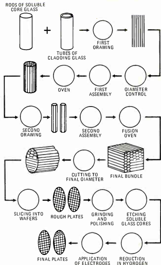
(c) MICROCHANNEL PLATE MANUFACTURING PROCESS
