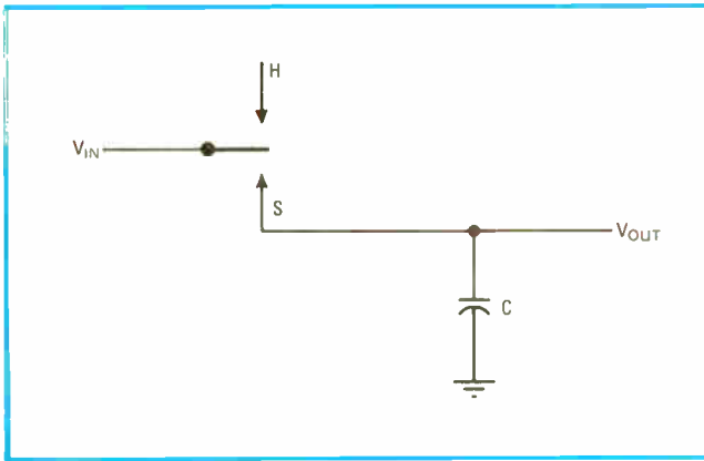
1. Simplest. If speed and circuit loading are not too important, a capacitor and a switch make an effective sample-and-hold circuit.
