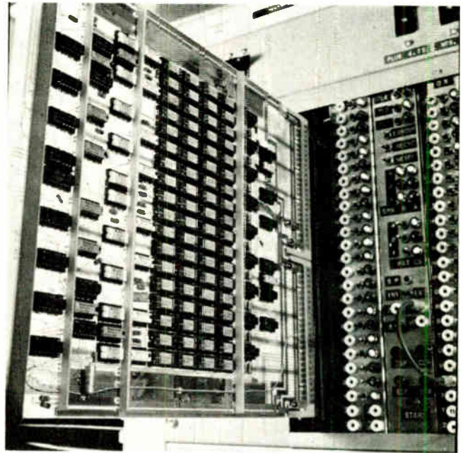
Extended for maintenance. In the Burroughs B-1700, the memory proper is the dark array at center, surrounded by support circuitry.
