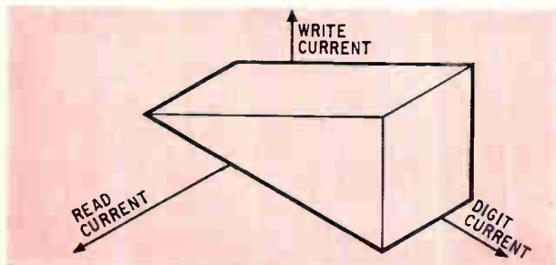
Theoretical. Satisfactory operation of a memory element depends on all currents going through it having optimum values. Above is the relationship between the theoretical maximum variations for these currents.
