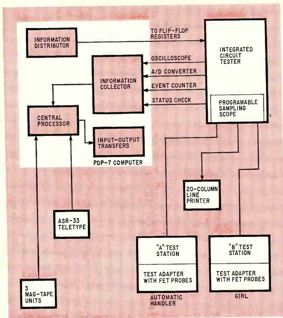
Central Processing. Test system is built around a computer and other standard equipment.
