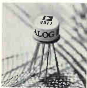
Differential d-c comparator model 351 is a monolithic IC device in a T-100 case, and designed for accurate sensing and measuring applications. It is capable of resolution in the fractional millivolt and sub-microamp regions and will handle 10^5 ohm signal sources. Unit lists singly for $11.70; $7.80 in lots of 100. Analog Devices Inc., 221 Fifth St., Cambridge, Mass. [436]
