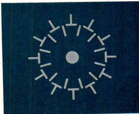
Angel fish and T-bar. Magnetic modulation inchworms bubbles along the permalloy wedges, left. This is called angel fish. The T-bar method, right, magnetically polarizes permalloy bars using a rotating field in plane. Masks shown are for 12-position shift registers.
