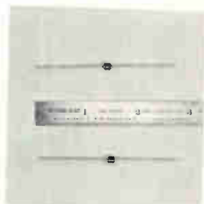
Glass, 5-watt, axial lead JAN and JAN TX zener diodes 1N4954 through 1N4969 meet MIL-S-19500E/356A and MIL-STD-701 specifications. Voltage ranges of from 6.8 v through 30 v are available. Size is 0.140 in. maximum diameter by 0.230 in. maximum length with 0.040 in. diameter silver leads. MicroSemiconductor Corp., 11250 Playa Court, Culver City, Calif. 90230 [443]
