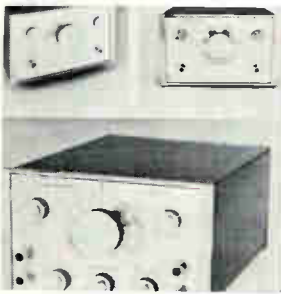
Precision signal generators for general lab use produce sine, square, triangle, and ramp waveforms over the range of 0.2 hz to 2 Mhz with an adjustable output of 10 v peak-to-peak into a 50-ohm load. Model 130 is a function generator; model 131, a voltage-controlled generator; model 134, a sweep/trigger voltage-controlled generator. Wavetek, Box 651, San Diego, Calif. [361]
