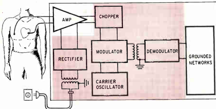
An isolated example. Medical instrument makers, challenged on safety of their wares, are turning to circuit isolation. Above, transformers ensure that there's no electrical path connecting the patient to ground.
