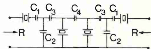
Example of IR filter with n = 4 Identical Resonators. By changing capacitors C_1 to C_n , a continuous range of different filter responses becomes possible.
