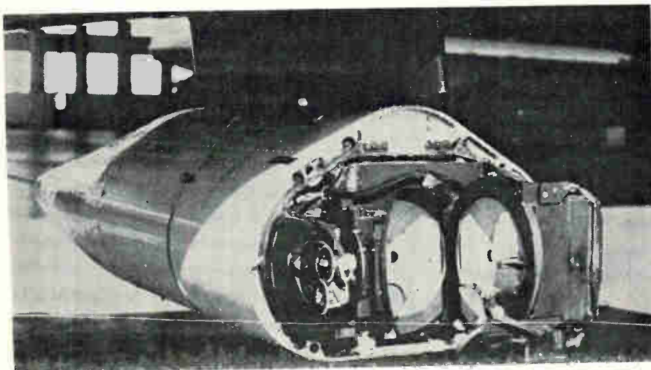
Multifunction pod. Weapons delivery system has low-light-level tv camera (with optics folded open), combined with a laser ranging unit, mounted in an under-slung wing pod. The system, built by Westinghouse Aerospace as an outgrowth of the Air Force's Tropic Moon #2 program, also contains an automatic video tracker, electronic zoom intensifier, and weapons computer.
