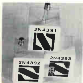
FET choppers 2N4391, -2 and -3 feature a switching time of 15 nsec (typical) and low leakage of 100 pa maximum. Units offer optimum performance in microvolt amplifiers and meters, multiplexers, commutators, tv equipment, oscilloscopes, a-m and c-b receivers. Price is from $2.50 to $3.50 for 100 up. National Semiconductor Corp., San Ysidro Way, Santa Clara, Calif. [440]
