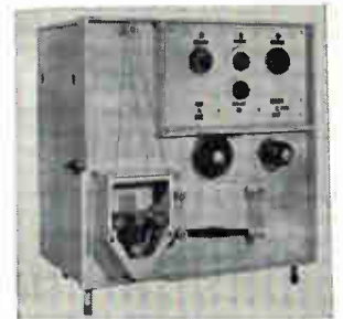
Sea-Saw model 700 is for wafering and dicing silicon and similar hard, fireable materials. It enables dicing of crystals up to 3 in. in diameter. Cutting is done by thin, oscillating tungsten wires which pass through an abrasive slurry. Wafers as thin as 0.0055 in. can be sliced with an 0.004 in. diameter wire. Geoscience Instruments Corp., E. Third St., Mt. Vernon, N.Y. [424]
