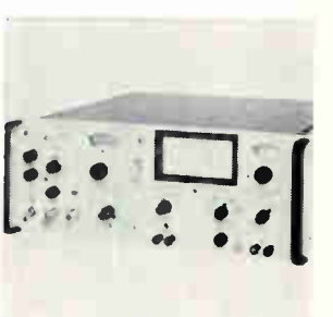
A-m/f-m vhf/uhf signal generator model 6301 originally designed for ground check-out of military aircraft communication and data links is available as a general purpose unit. It fetures a-m modulation to 80%, and f-m to \pm 100 khz, or phase modulation, together with 2 v (+19 dbm) of r-f output. Price is $4,450. Wiltron Co., 930 East Meadow Dr., Palo Alto, Calif. 94303 [368]
