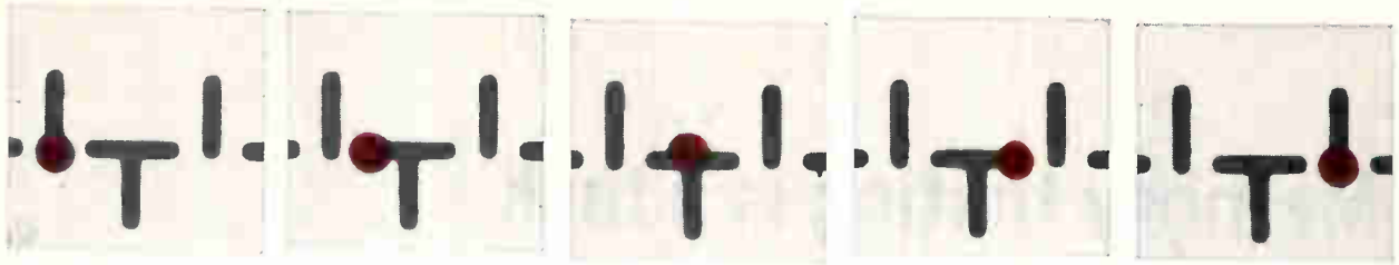
Jumpers. Magnetic bubbles favor positive-polarity magnets. Rotation of the in-plane field changes the polarity of each vertical and horizontal bar every 90° of field rotation, and bubbles moves to right.
