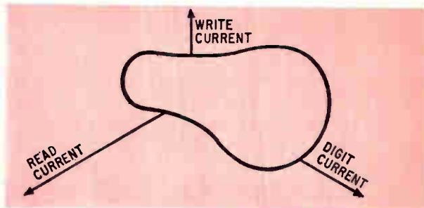
Actual. Noise and other parasitics round off the sharp corners so that the region of satisfactory operation is pear-shaped rather than prismatic. The curve is called a shmoo plot.
