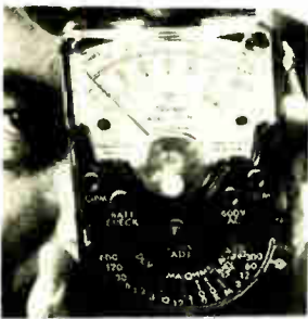
Volt - ohm - milliammeter model 310-FET features field-effect-transistorized circuitry, 10-megohm constant input resistance on all d-c voltage ranges, and sensitivity about 10 times greater than the conventional bench-type vtvm in the 0.3 v range and resistance readings to 5,000 megohms. Price is $70 (with probes and leads). Triplett Electrical Instrument Co., Bluffton, Ohio [381]
