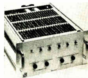
Data modem AE-96 can quadruple the capacity of a 2,400 bps voice grade line to 9,600 bps. This is achieved by a digital adaptive equalizer that allows the model to automatically measure and compensate for the intersymbol interferences caused by circuit amplitude and delay distortion. Initial circuit equalization takes 3.5 seconds. Codex Corp., Watertown, Mass. [364]
