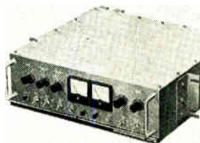
Solid state predetection combiner PDC-2T is designed to be used with telemetry receivers for data acquisition and monitoring and will provide optimum predetection combining for signals of any bandwidth up to 4 Mhz. It provides true maximal ratio combining of signals without regard to modulation type or index down to a 0 db output S/N ratio. Raytheon Co., Norwood, Mass. [363]
