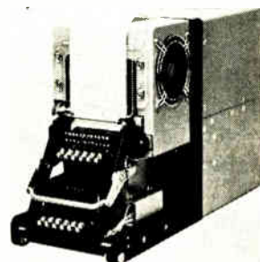
High-speed printer HSP3608 is especially designed for aerospace applications. The 19-lb unit is capable of operating in a zero G hard vacuum environment for prolonged durations. It provides 24 columns of printout with 48 characters (ASCII code) and speeds of 10 to 40 characters per second, serially. Potter Instrument Co., East Bethpage Road, Plainview, N.Y. 11803. [368]
