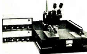
All lead flatpack soldering system features an X-Y table that allows fast precise positioning of the circuit board under the soldering head by use of a visible tooling templet. The table handles circuit boards up to 8 x 8 in. and positions within 0.001 in. accuracy. Price of the complete system is $4,900. Development Associates Controls, 725 Reddick Ave., Santa Barbara, Calif. [421]
