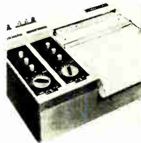
Chart recorder model 2741 has 11 switch-selected d-c voltage ranges, any of which can be set with front panel controls to become segmented scale or zero-center scale ranges. This allows the operator to custom make the recording range for his specific need. Result is better resolution and an easier-to-read recording. Simpson Electric Co., 5200 W. Kinzie St., Chicago [383]
