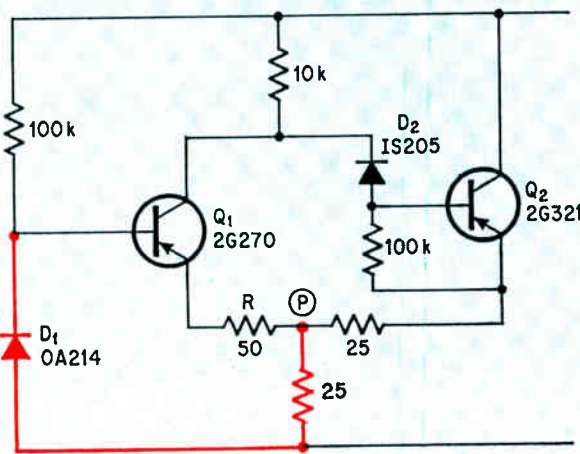
CURRENT-CONTROLLED
