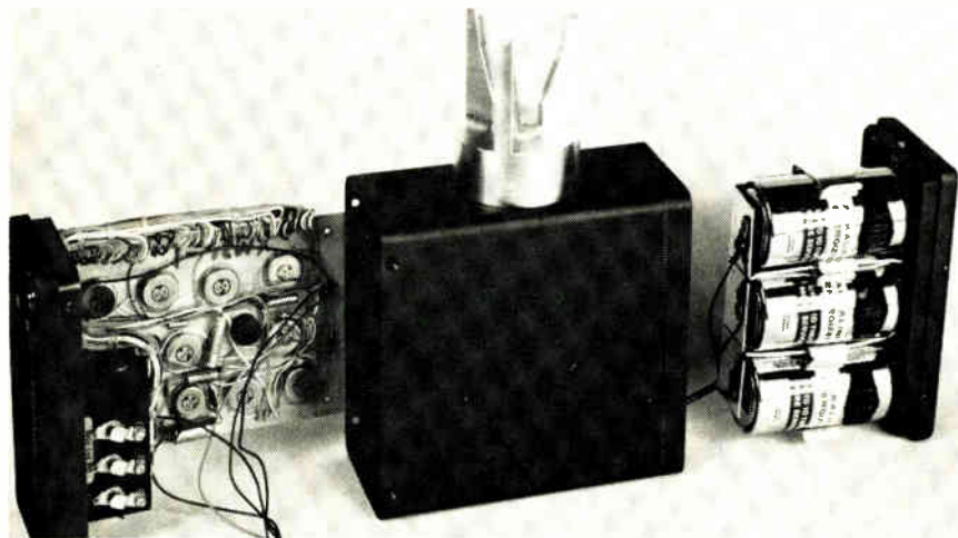
Ready, aim . . . Fuze setter using IC's promises accurate timing and ease of operation. "Crown" atrop black box fits over artillery shell's nose.
