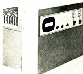
Compact positioning head drum system CPHD features a storage capacity of 900,000 eight-bit characters accessible in an average time of 60 msec. An important aspect in the design is that eight write/read heads are mounted on one head pad, resulting in compactness and economy to the end user. Bryant Computer Products, 850 Ladd Road, Walled Lake, Mich. 48088 [367]
