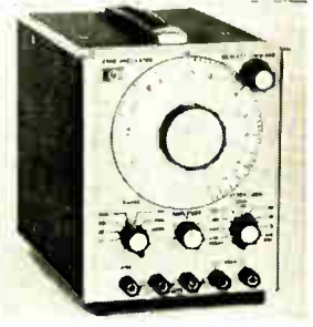
Precision oscillator 204D has an 80-db attenuator for making measurements over a wide amplitude range, from 2.5 v rms into 600 ohms (5 v open circuited), down to less than 250 \mu v rms. Frequency range is 5 hz to 1.2 Mhz. The a-c line operated version costs $325. Equipped for mercury battery operation the price is $340. Hewlett-Packard Co., Palo Alto, Calif. [384]
