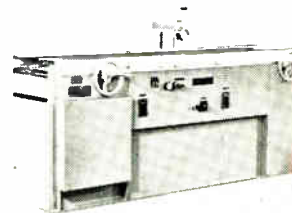
Wavesolder system 409 can process p-c boards as small as 2 x 1 in. and as large as 10 x 24 in. without pallets or board holders. It has a 10 in. Teflon coated foam fluxer, panel preheater with 3-position heat selector switch and an adjustable width conveyor. It is capable of production speeds from 1.5 to 10 ft per minute. Electrovert Inc., 86 Hartford Ave., Mt. Vernon, N.Y. [424]
