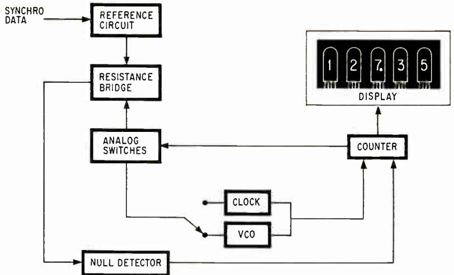
Null search. When the null point is found on the resistance bridge, the number in the counter tells the angular position of the synchro.
