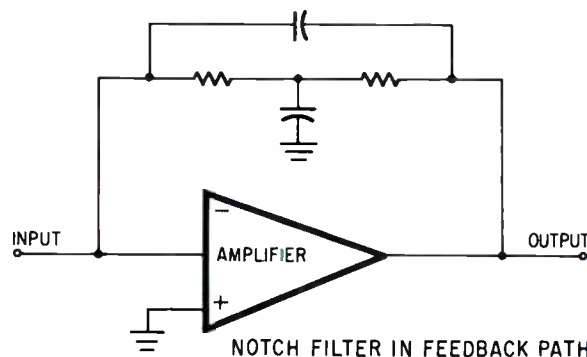
NOTCH FILTER IN FEEDBACK PATH
