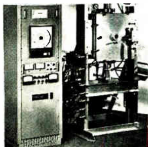
Hot press vacuum furnace model 1082-AP is for vacuum diffusion bonding and pressing powdered metal, ceramic and composite materials. The furnace, for operation to 3,000°F, is resistance heated. Forces of 25 tons can be applied to temperatures higher than 2,000°F. The unit will accept dies up to 7 1/2 in. diameter. Richard D. Brew & Co., 90 Airport Rd., Concord, N.H. 03301. [426]
