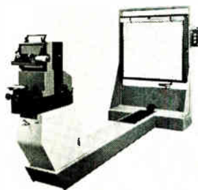
Dual ratio cameras series 1700 are for the production of high-resolution integrated circuit, printed circuit, reticle and chemical milling photomasks. Standard units are now available for the following reduction ratios: 5 to 1 and 10 to 1; 10 to 1 and 20 to 1; and 20 to 1 and 40 to 1. HLC Manufacturing Co., 700 Davisville Road, Willow Grove, Pa. 19090. [422]
