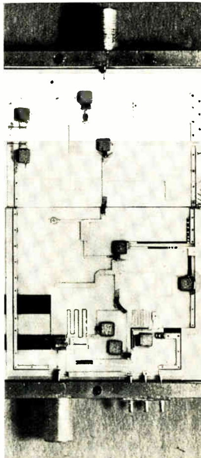
Sending. Microwave transmitter using TI's thin-film hybrid IC's.
