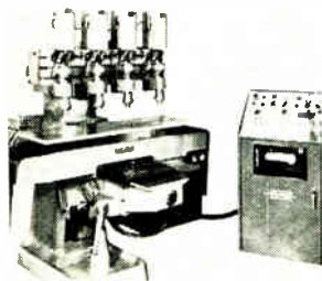
Numerically controlled multi-head machine model 83-600 is for circuit board work. It can be equipped with up to 6 heads which can operate either individually or in groups of 2 or 3. Its power quills have a speed range of 15,000 or 45,000 rpm. Drilling capacity ranges from 0.010 in. to 3/16 in. diameter holes. Moog Inc., Hydra-Point Division, P.O. Box 143, Buffalo, N.Y. [425]
