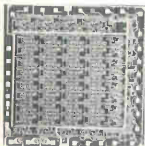
Random access read/write memory TT \mu L9035 has a 285-gate complexity organized in a 16-word by 4-bit format. It features a read access time of 35 nsec and a 25 nsec write time. It is designed for scratch pad memories and other applications where rapid access temporary storage is desired. Fairchild Semiconductor, 313 Fairchild Dr., Mtn. View, Calif. 94040. [436]
