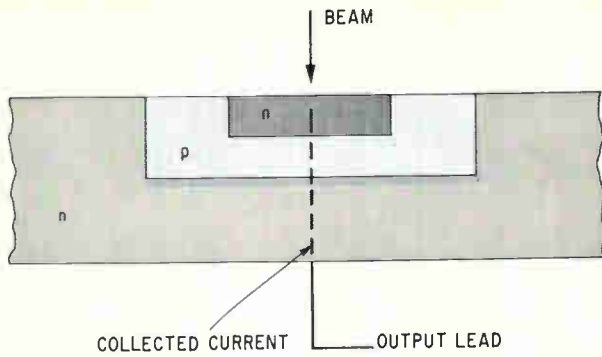
Beam bias. The simplest way of biasing the device is to use the beam to generate potentials across the junctions.
