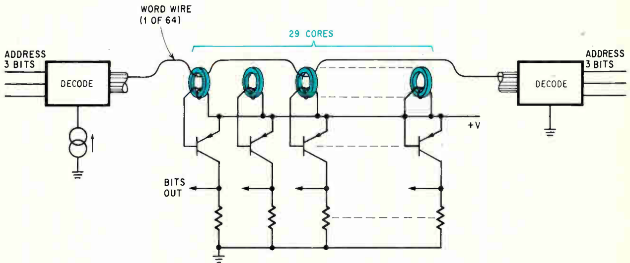
Braid memory. Microinstructions that control both the ferrite-core memory and the linear array are stored in a braid memory containing 64 words of 29 bits each.
