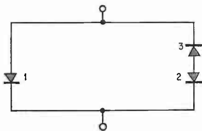
One more. The 3d barrier is in series with the 2d, but opposite in direction.
