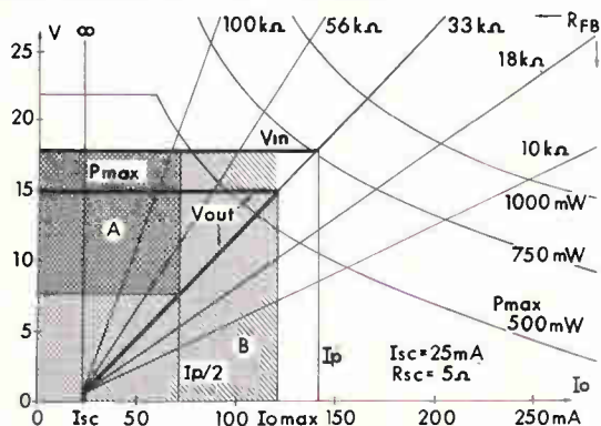
Peak power prediction for typical output characteristics. Programmable foldback permits maximum power dissipation ("A" above) only 1/3 that resulting from conventional current limiting ("B" above) or optionally, 3x greater output current with the same power dissipation.
