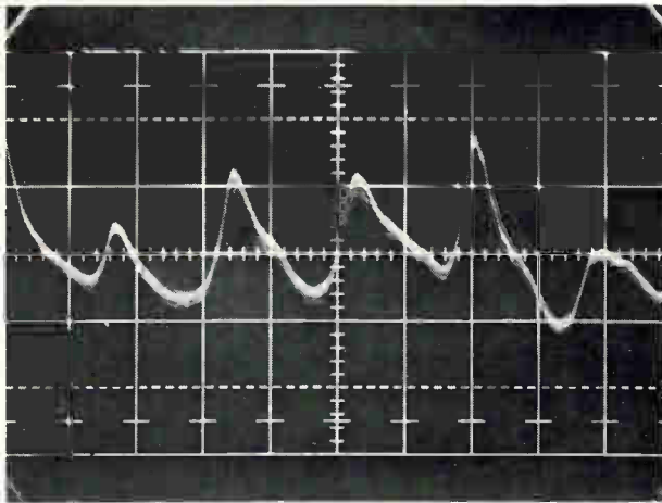
Demonstration. Dots of indium on the CdS crystal (top) simulate the local conductivity variations that would be caused by a projected image. Output current changes appreciably when the domain passes the dots, as indicated by the oscilloscope trace.
