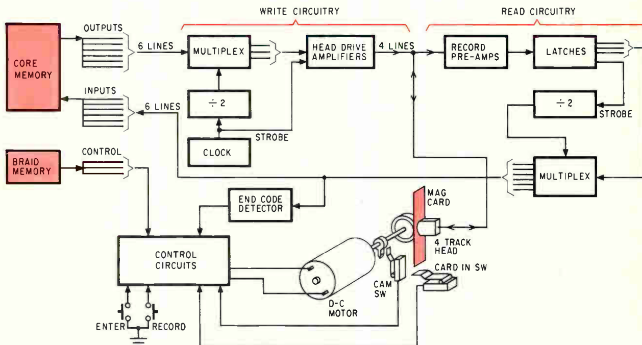
Card reader. A program in the calculator's core memory can be transferred to the magnetic card through the write circuits. When reading, data on the card is transferred to the core memory along paths parallel to those from the keyboard. The card records data on four tracks—three bits and a strobe; each code is recorded in two groups of three bits.
