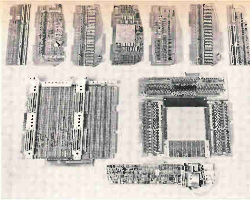
Calculator exploded. The multilayer board at left center contains all the calculator's logic gates plus sockets into which the five boards at top center plug in. The read-only memory, on the bottom of the calculator, is tied into the system through the small connectors shown at either end of the top row.
