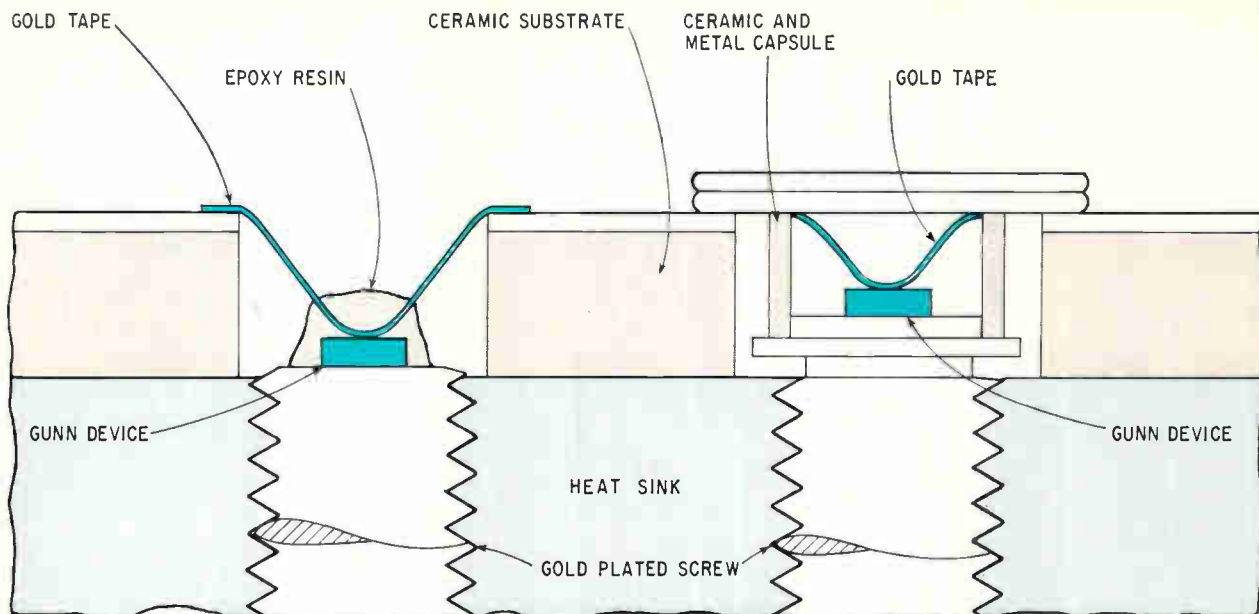
Epoxy or pill. In STL modules, the Gunn device is mounted on the ceramic substrate either in a ceramic pill package (right) or by a globule of epoxy resin. The gold-plated screw provides a thermally conductive path from the device to the heat sink.
