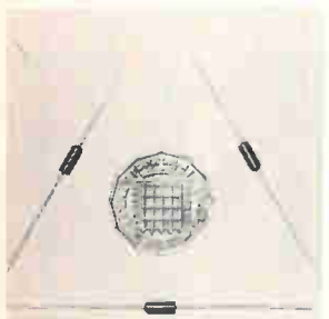
Zener diodes types BZX61 and BZX70 have power ratings of 1 and 2.5 w respectively, and voltage tolerances of \pm 5\% . The BZX61's are enclosed in a modified DO-7 plastic encapsulation, and are available with voltage ratings from 6.8 to 75 v. The BZX70's are wire-ended and enclosed in a plastic encapsulation, and cover 10 to 75 v. Mullard Ltd., London W.C.1. [440]
