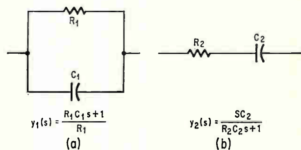
RC networks. Because of the electrical properties of the op amp—high input impedance, low output impedance, and very high gain—the engineer need only connect RC network combinations, such as these, to obtain a desired frequency response curve.
