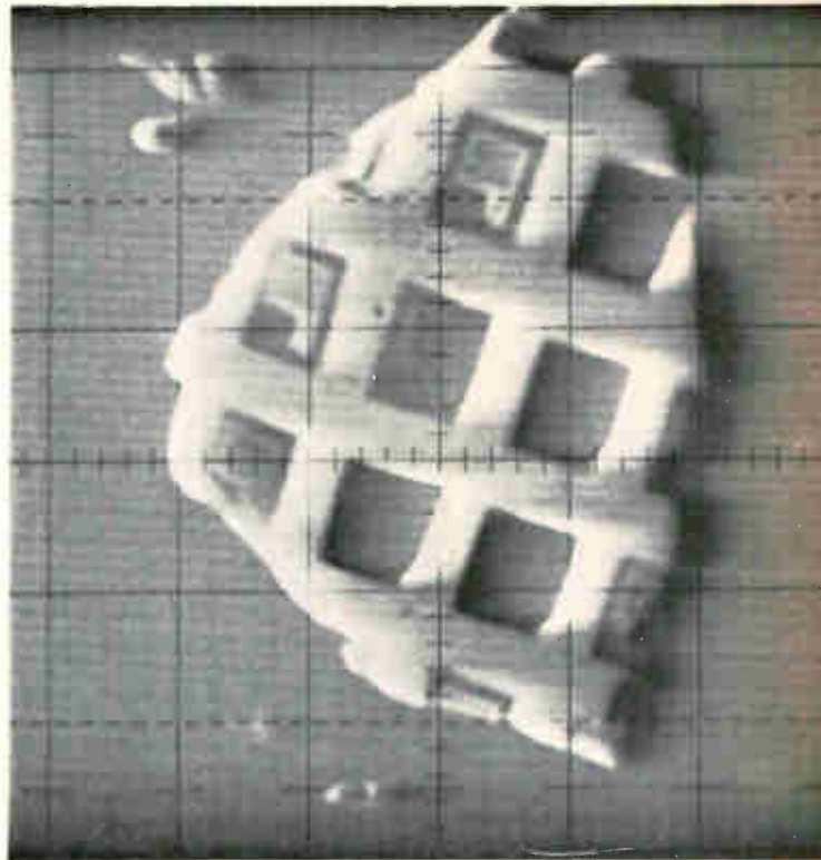
Good and bad. Tv-like picture uses output of control loop as video signal to reveal defective junctions in transistors. For demonstration purposes, oxides and metal were removed from the device surfaces.
