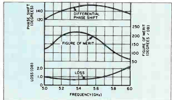
TYPICAL PERFORMANCE OF PACT-DEVELOPED PHASE SHIFTERS
