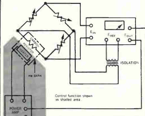
LOCK-IN AMPLIFIER USED AS BRIDGE OSCILLATOR/NUL DETECTOR
