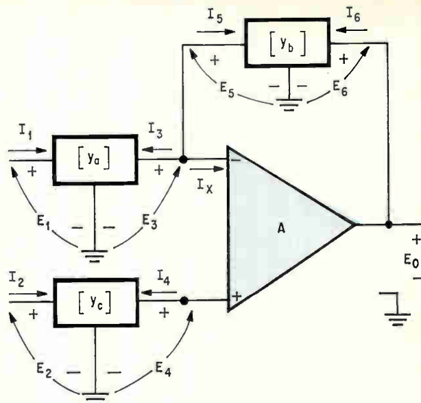
Feedback. Basic op amp containing feedback and two input signals is represented in block-diagram form. This configuration is used to produce second-order transfer functions.
