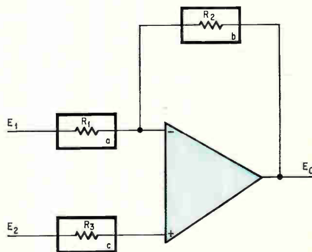
Verification. Resistors R_1, R_2 , and R_3 , connected to the op amp produce an output signal that is proportional to both input voltages and the feedback network.
