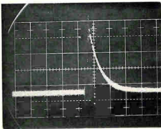
Junction capacitance. If the beam is suddenly switched on the base region of the device (the vertical step in the photomicrograph), the collector junction bias changes from an initial zero to the steady-state value. The time that this change takes indicates the capacitance of the collector junction. The vertical scale is 0.01 volt per large division; horizontal scale is 20 microseconds per large division.
