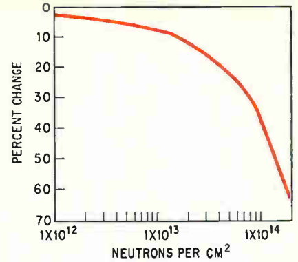
Falloff. Open loop gain of Radiation's hardened op amps drops rapidly near specified radiation limit.
