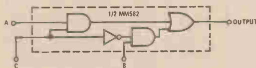
FIGURE 4. The MM582 is a Logic Steering Circuit That Performs the Function of a Single-pole, Double-throw Switch. When the Control Signal C is "True," A Appears at the Output; When it is "False," B Appears at the Output. Operation is Similar in the Input, Output and Comparison Selectors in Memory System.
