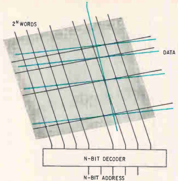
Fast plane. The simplest memory organization addresses one side of an array and brings data out at right angles to the addressing. The scheme is fast but expensive.
