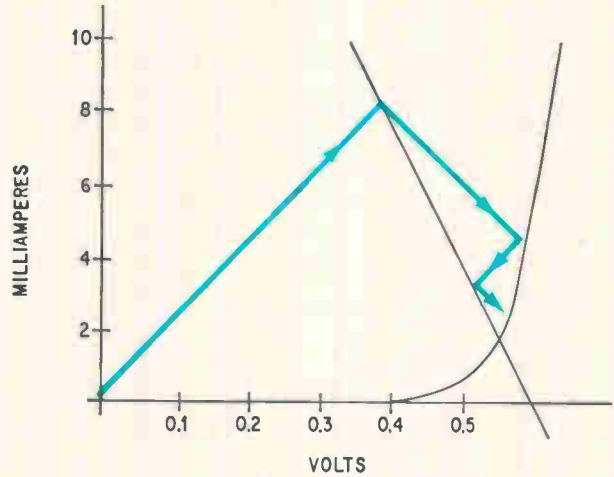
Nonlinear load. A diode is the load to a transmission line and the current and voltage values for the line are calculated from the graph.
