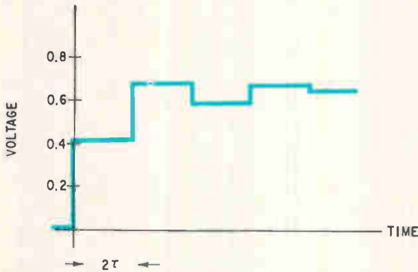
Sending-end voltage. Plot of the voltage at the sending end as a function of time indicates the additions and subtractions that result from the reflections. This plot is based on calculated values taken by the engineer from the graphic solution.
