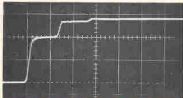
Verification. Photo of sending-end voltage of a line with a diode load has close agreement with calculated plot directly above.
