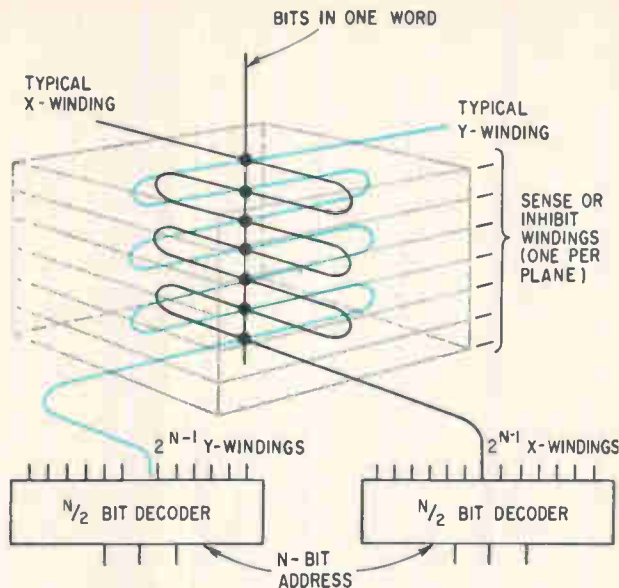
In depth. In the most common memory organization, 3-D, two sides of a stack are addressed to locate a vertical column of cores containing the stored data.
