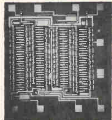
Founder. Dual 25-bit shift register is first of new line of MOS IC's.
