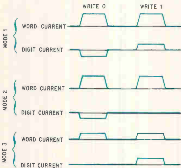
Three ways to write. Starting from the 0 state, a core switches or not depending on the digit current's direction, or on its presence or absence.
