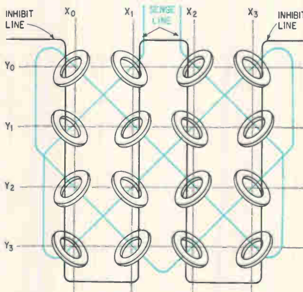
Sense and inhibit. Two additional wires in a 3-D stack sense a core's switching when reading a 1 and inhibit its switching when writing a 0.
