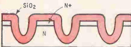
GROWTH OF SiO 2
