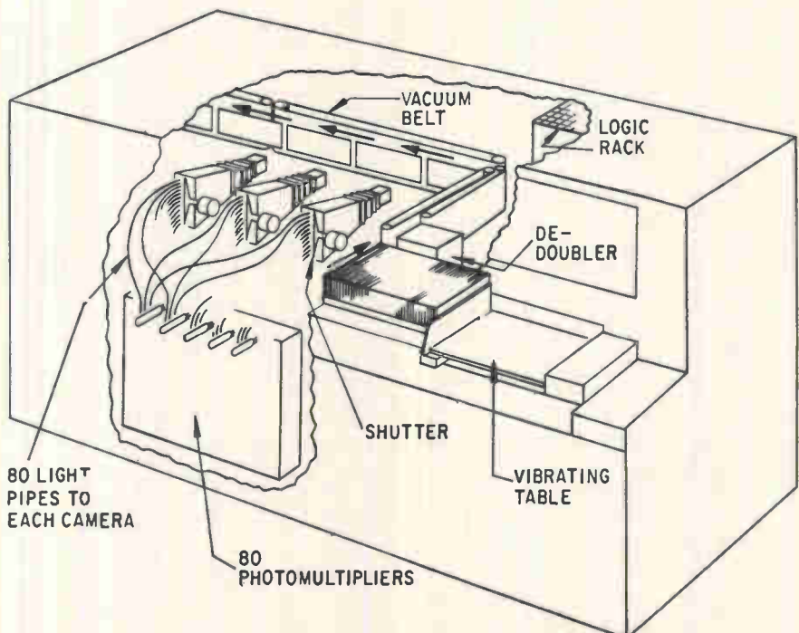
Fibers for reading. Documents travel from the vibrating table, past the de-doubler to the scanner, and on to the sorter (above). In the scanner, images are projected onto a column of 80 optical fibers.
