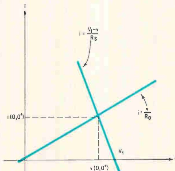
Crosspoints. The point at which the sending-end conductance line crosses the transmission-end conductance line represents the value of voltage and current as it starts down the line.
