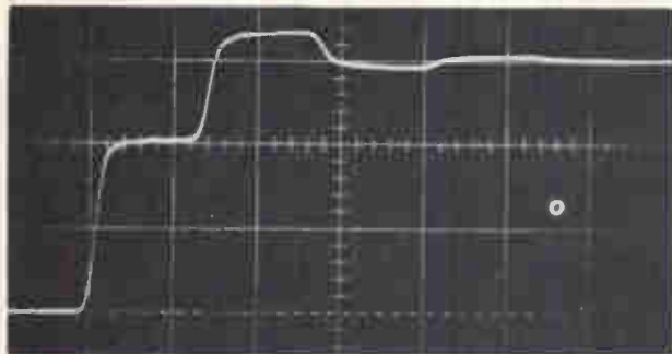
Proof-of-the pudding. Photo taken from the face of an oscilloscope attached to the transmission line verifies the calculated voltage values at the sending end of a transmission line, directly above.
