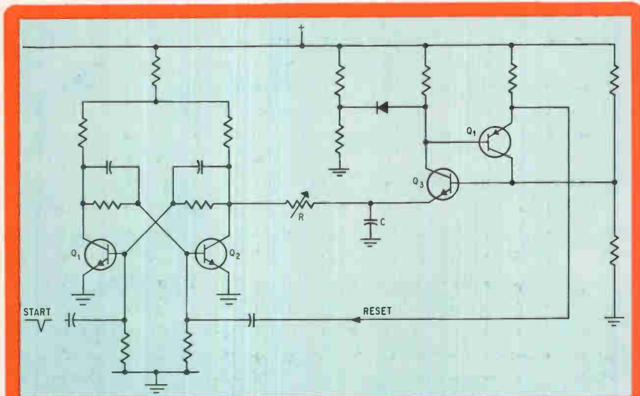
Combination. An astable multivibrator connected to a flip-flop forms a monostable multivibrator with the same input characteristics as a Schmitt circuit. The range of output pulse durations is as wide as the frequency range, so it's not hard to design a circuit with a range of three decades.
