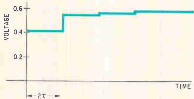
Sending-end voltage. Voltage values at the sending end of a transmission line terminated by a diode are calculated and plotted.
