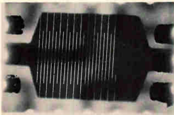
Thin-film resistors of the type made at the VEB Ceramics Works in Hermsdorf. Film with a resistivity of 300 ohms per square has been scribed to form a 100,000-ohm resistor (left). The two resistors at the right have values of 5,000 and 50,000 ohms and were cut from 200-ohm film. The lines, scribed with an electron beam, are 30 microns wide.
