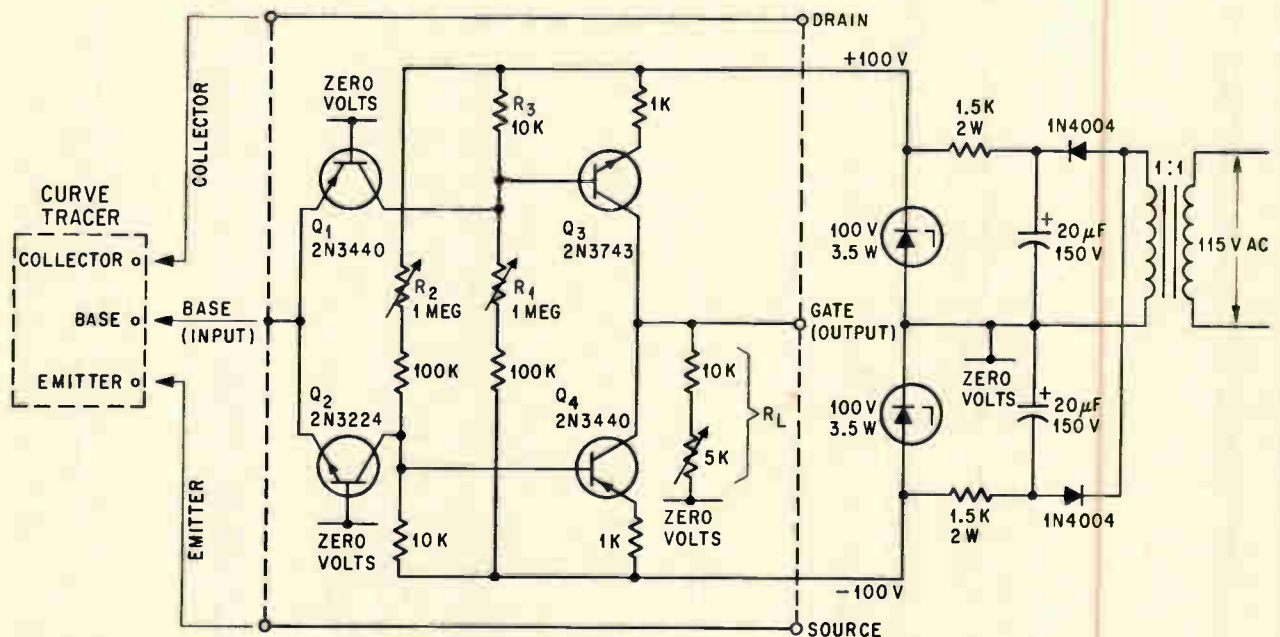
Adapter converts input current steps from curve tracer into output voltage steps for FET gate.
