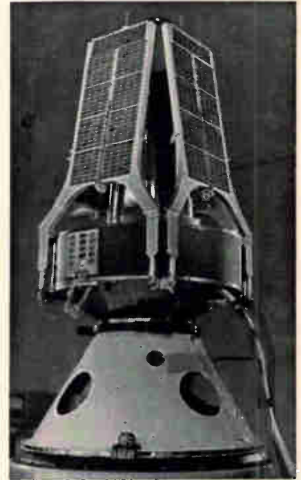
Folded solar-cell panels on all-French satellite D-1A open out when spacecraft goes into spin-stabilized orbit. Cone-shaped structure below satellite is instrument package for trajectory data telemetering, separates from satellite 13 minutes after lift-off.
