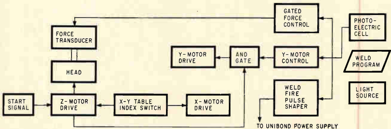
Pushbutton microwelder is controlled by an optical reader. A film pattern of the weld locations and the assembly being welded are placed on a table that moves the assembly under the welding head and pauses each time a weld is to be made.
