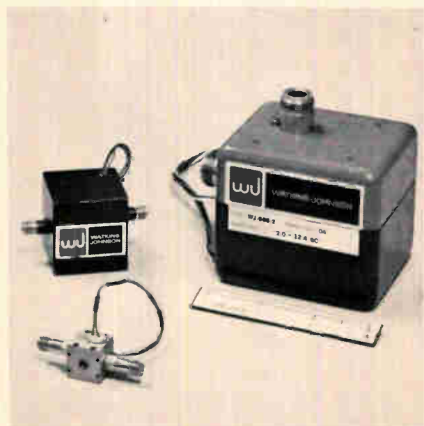
Reduction in YIG filter size is shown by the Watkins-Johnson Co.'s standard, compact and miniature filters.
