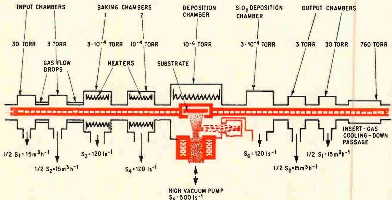
Vacuum chamber arrangement in the deposition system. Vacuum pumping speed and pressure for each chamber are in the lower part of the drawing. The substrate-transfer mechanism and the electron-beam vaporizer are in color.
