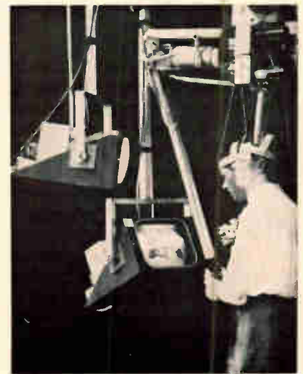
Motion of the head, as shown in this double exposure, produces a similar movement on a television camera and the monitor, providing a change of perspective for the operator of a remote-controlled manipulator. If the operator moves his head to the left, the camera that's trained on the "hands" of the manipulator (picture on the left) moves to the left and the tv monitor also moves to the left, remaining within the operator's field of view.
