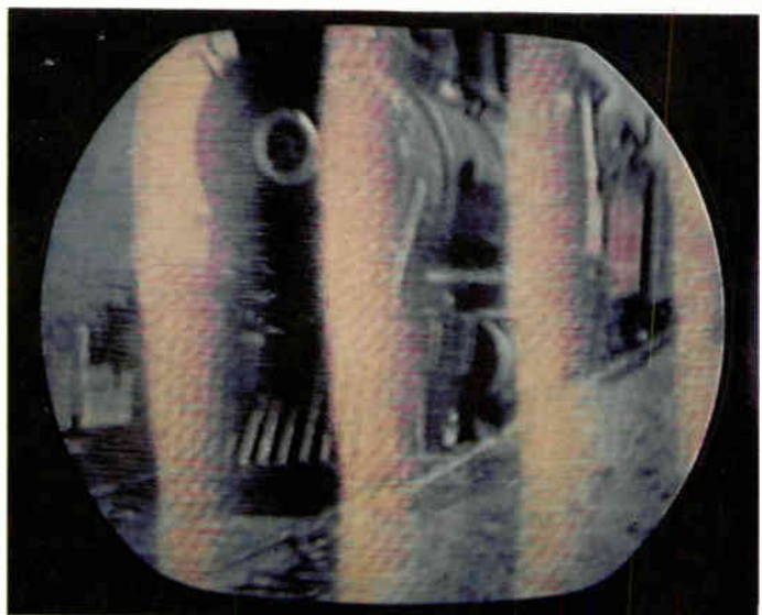
Windshield-wiper effect appears when cross-modulation components are 40 decibels below signal level.
