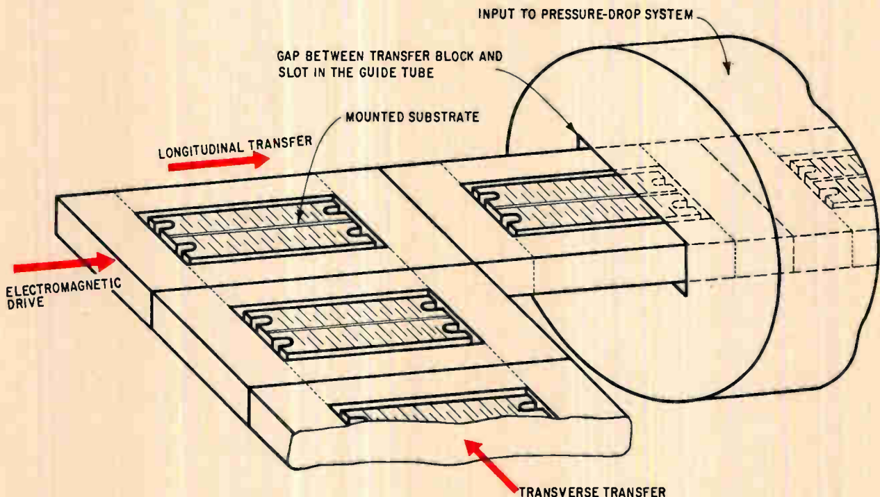
Transfer mechanism employed in the vacuum systems. The transfer blocks are pushed by electromagnetic drives.
