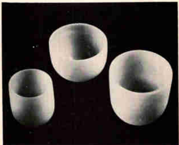
Semi opaque quartz crucibles contain molten semiconductor material during crystal formation process. Crucibles are contaminant-free and virtually non-breakable.
