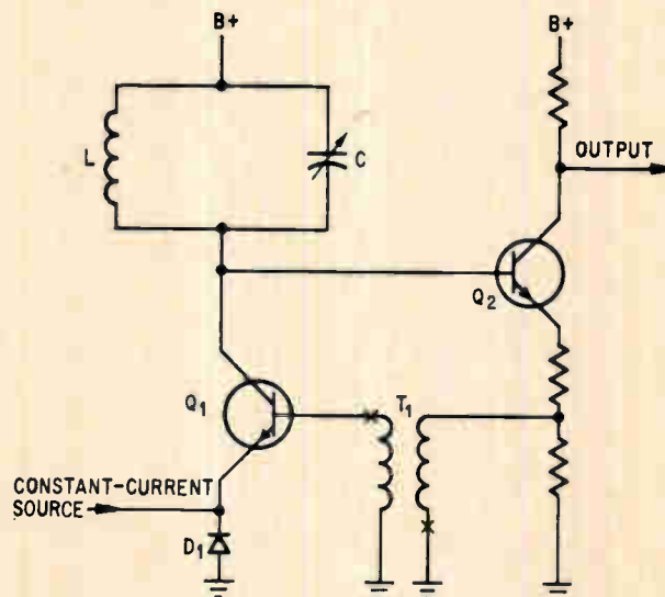
Simple LC tuned circuit determines the frequency of pulse repetition oscillator. The feedback to sustain oscillation is fed to Q_1 through inverted transformer.
