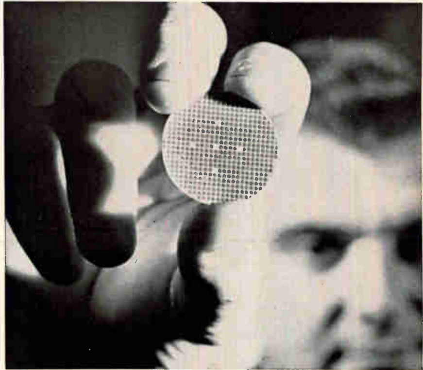
Ceramic mosaic contains 8,000 silicon tiles. The small squares that are visible in this picture are groups of tile. The entire array will go through semiconductor diffusion and metalization processes and will emerge as 440 intermediate-frequency amplifiers.
