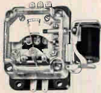
Model 813 Miniature — compact and lightweight; sensitive and Sensitrol (magnetic) contacts; single or double contact; ranges as low as 2-0-2 \mu\text{a} .
