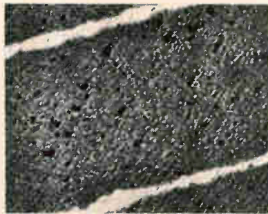
Dielectric of a second make of conventional CK ceramic
