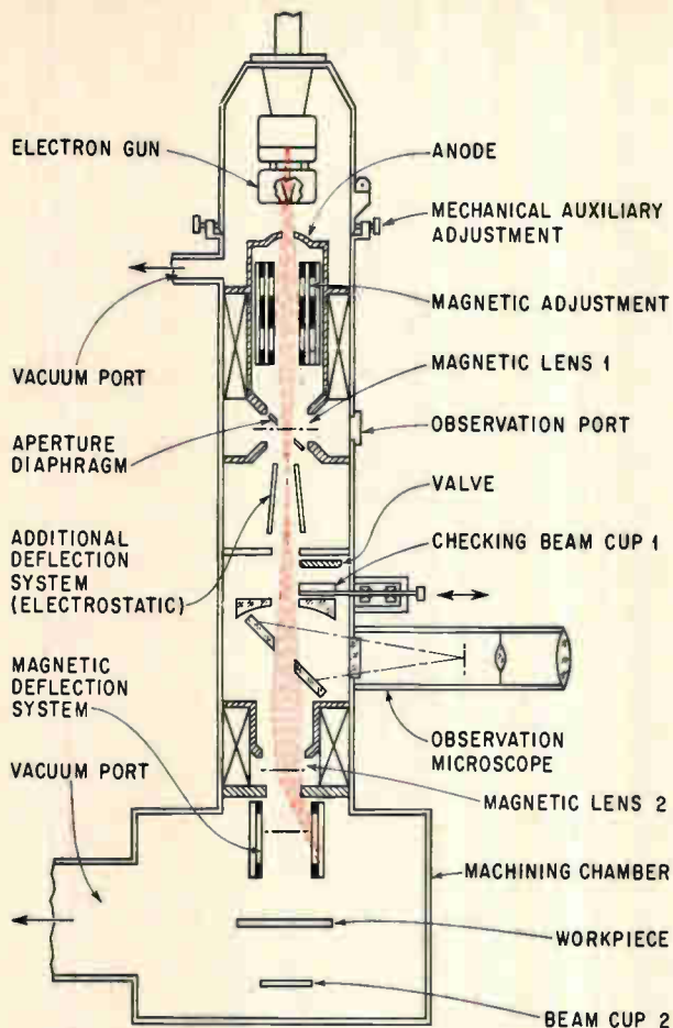
Electron-optical system of the electron-beam machining equipment. It is similar to the Carl Zeiss equipment which is being used in the United States for microwelding and micromachining of electronic components. The beam is in color.
