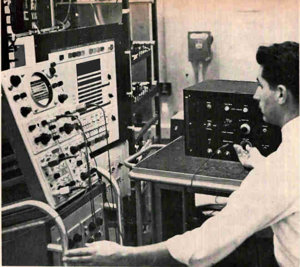
System in the background is subjected to voltage dip from cycle sag simulator, right. The design engineer monitors the simulator's output and a system parameter on oscilloscope.
