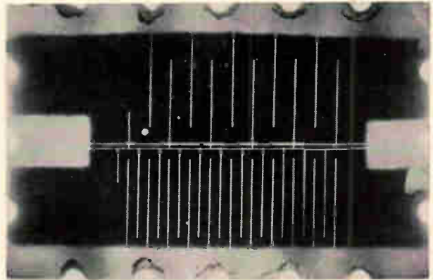
Thin-film resistors of the type made at the VEB Ceramics Works in Hermsdorf. Film with a resistivity of 300 ohms per square has been scribed to form a 100,000-ohm resistor (left). The two resistors at the right have values of 5,000 and 50,000 ohms and were cut from 200-ohm film. The lines, scribed with an electron beam, are 30 microns wide.
