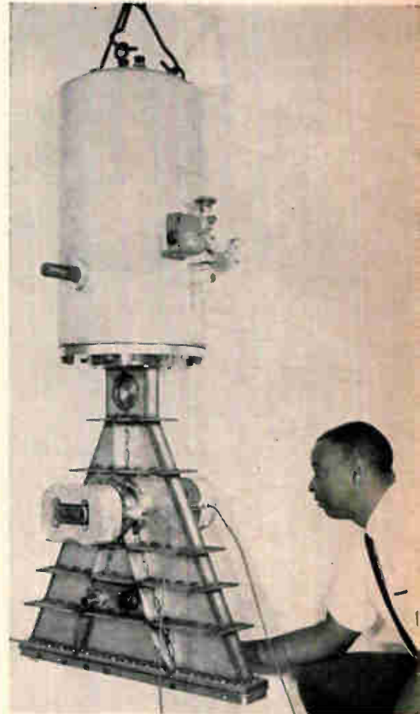
Ford physicist Allen Turner makes adjustment on electron-beam gun developed by company to cure paint on wood, metal and plastic. The process may be adapted for producing printed-circuit boards and multilayer boards.
