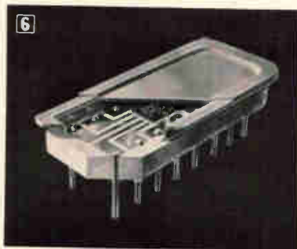
6 Cut-away view of TI's new 16-pin plug-in package, optional for all 39 digital industrial circuits.
