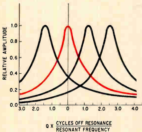
Adding universal response curves of several cavity resonances vectorially, lower sketch, results in a smoother conductance curve, top, which is the frequency characteristics of the cavity.
