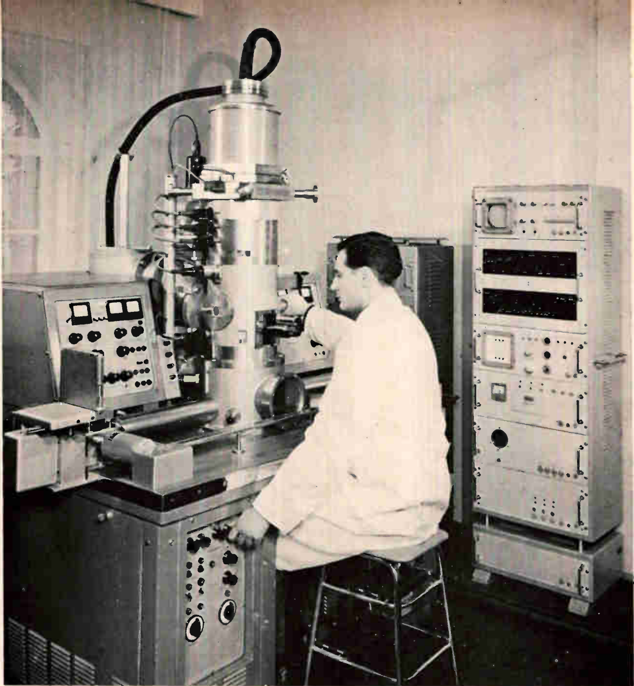
Electron-beam machining system trims thin-film resistors a rate of one substrate every 2.4 seconds. Substrates are fed continuously into the vacuum system over the track in front of the operator. The programmer is at right.
