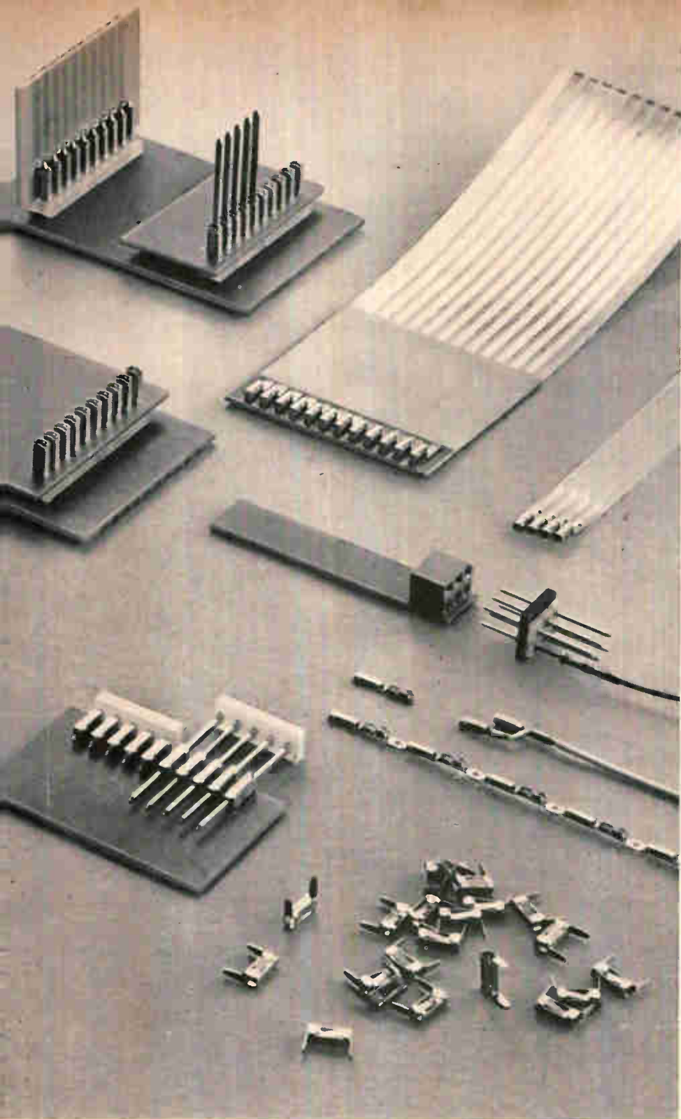
The AMPMODU female contacts may be mounted in one of three ways for modular connection versatility
