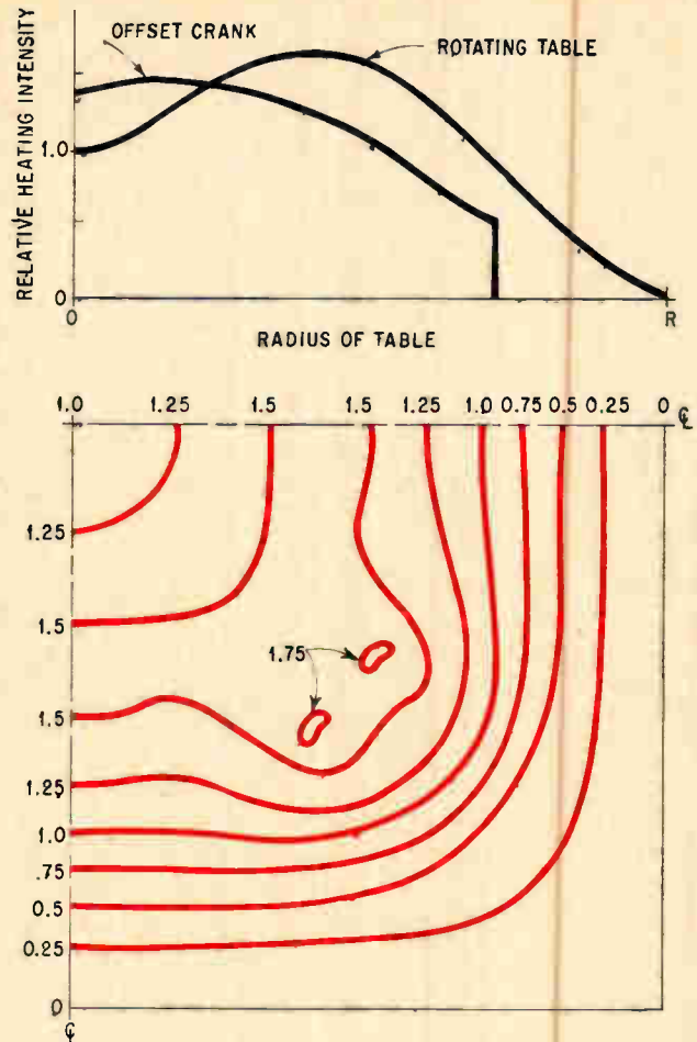
Contours of equal relative heating-intensity in a quadrant of a square cavity illuminated by equal amounts in the TE_{111} mode (1,000 Mc), TE_{112} mode (2,450 Mc), TE_{211} mode (2,450 Mc) and the TE_{212} mode (4,000 Mc) illustrate smoothing of contours when several resonant modes are present. Fairly uniform heating is obtained over a major portion of the oven. If the load is placed on a rotating table, differences in heating intensity within the load will be averaged out as the table revolves. If the table is mounted on an offset crank that rotates at one-fifth the rate of the load, the differences can be decreased further.
