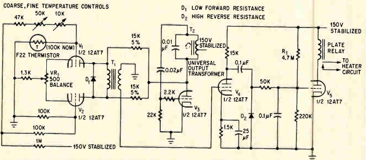
Temperature regulator uses high-resistance thermistor in bridge circuit. Variation of its resistance unbalances chopper circuit, generating pulses to control heater circuit.
