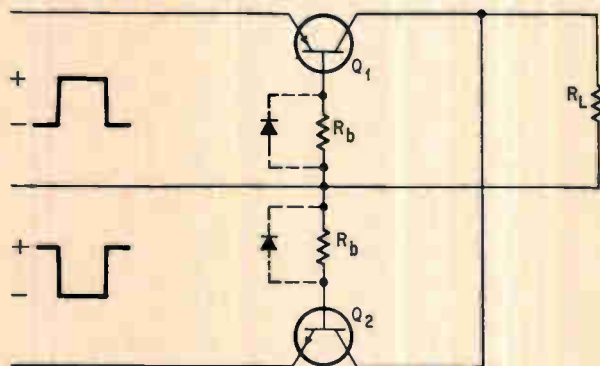
Signal-powered OR circuit provides an output pulse for a positive voltage at A or a negative voltage at B. When either transistor is nonconducting, its high reverse impedance prevents pulses of the opposite polarity from reaching the source.
