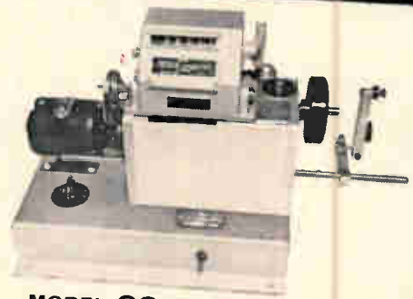
MODEL CS BOBBIN WINDER
