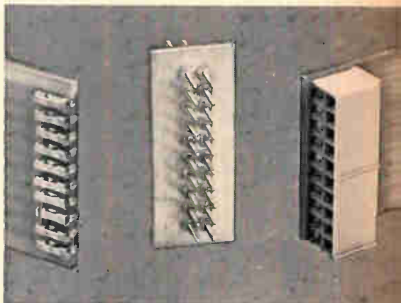
Miniature AMPMODU contacts may be mounted ten to the inch
