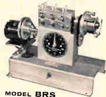
MODEL BRS PRECISION STRIP WINDER
