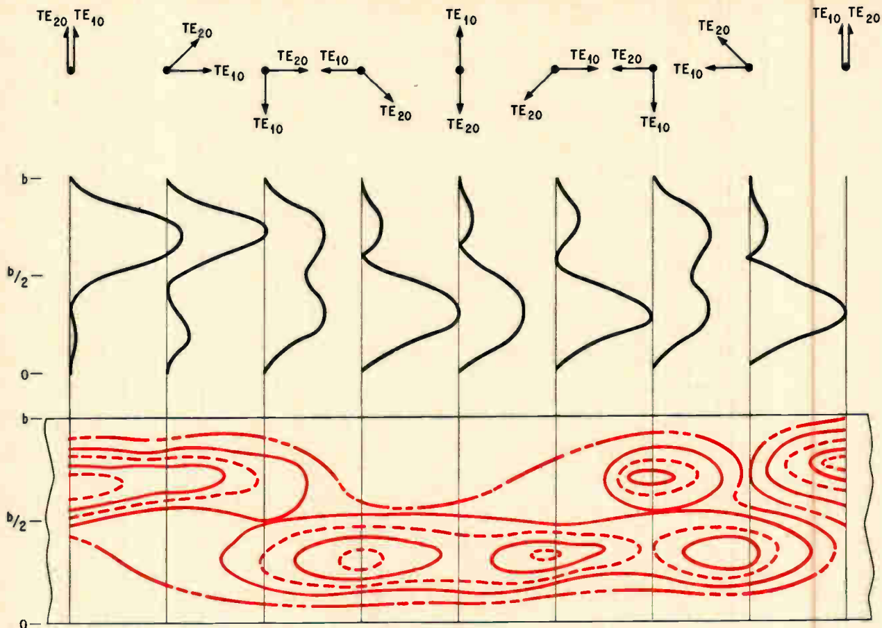
Development of contours for the average heating density is shown for a waveguide carrying the TE_{10} and TE_{20} modes. Vectors at the top indicate the relative time phase of the two modes in planes perpendicular to the direction of power flow. Heating density (see equation 3) in these planes is shown in center illustration. Contours of equal heating density are shown in bottom drawing.
