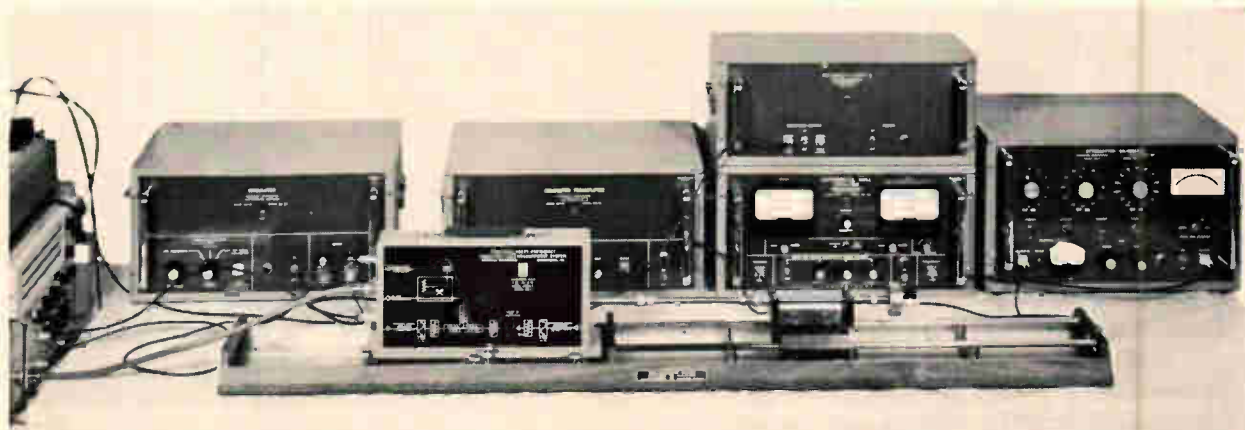
Versatile, sensitive measuring system operates over wide range of high frequencies to pinpoint insertion losses.
