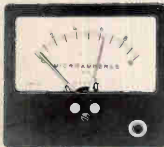
Model 1073 Mag Trak — long scale; shielded; positive contact; combines LCCA with magnetic attraction; self-contained reset; single or double adjustable contacts, ranges from 10 \mu\text{a} .
