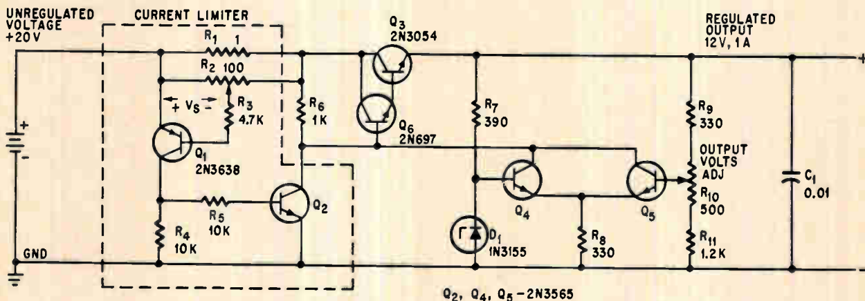
Current-limiting protection is added to a series-regulated power supply. The two transistors, shown within the dotted lines, accomplish the protection without degrading the performance of the power supply.
