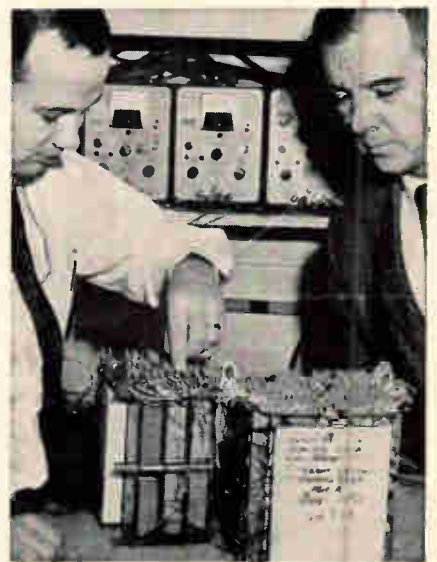
Satellite memory, designed by James C. Perschy, left, and Leo C. Miller of Applied Physics Laboratory, enables the satellite to tell ships and aircraft where it is.
