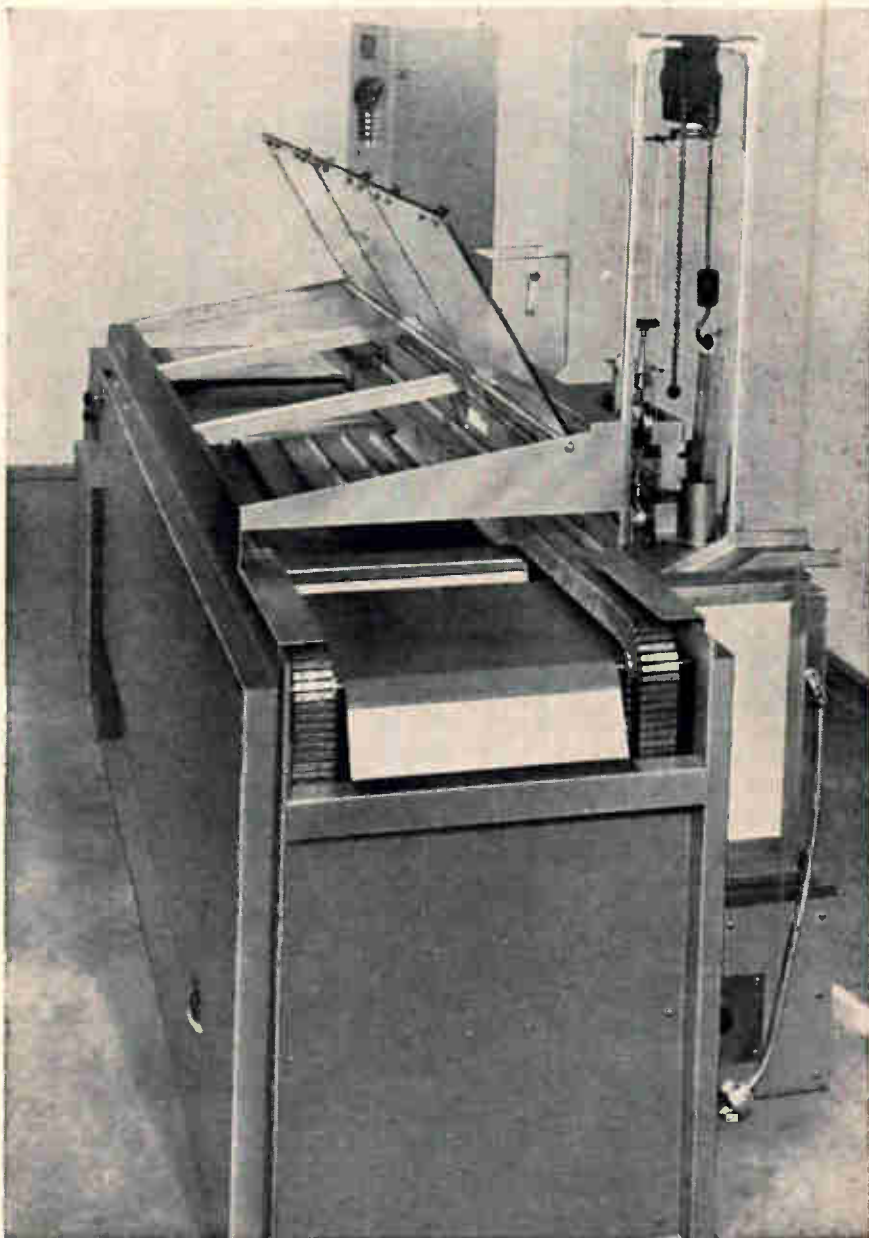
Stainless-steel fingers on wave soldering equipment transport pallets from p-c board assembly line through the wave-soldering process.
