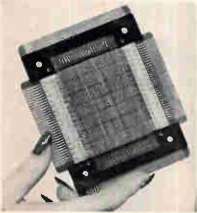
Scratch-pad memory for Gamma 140/141 computers uses Permalloy-plated wires as magnetic elements, woven wires for the matrix.
