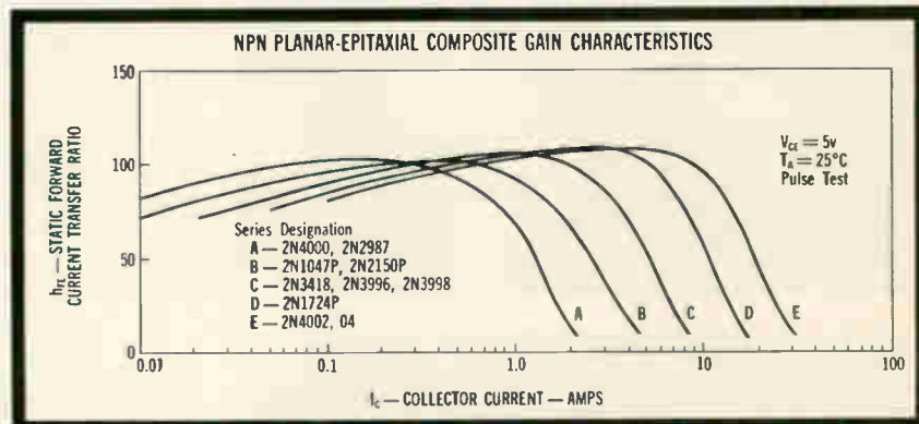
Figure 4: Uniform beta of five families of planar-epitaxial NPN silicon power transistors
