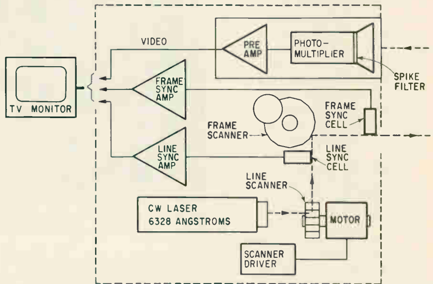
Laser-television system developed by the Perkin-Elmer Corp. uses a multiplier photocell as its tv camera while a laser beam supplies the light.
