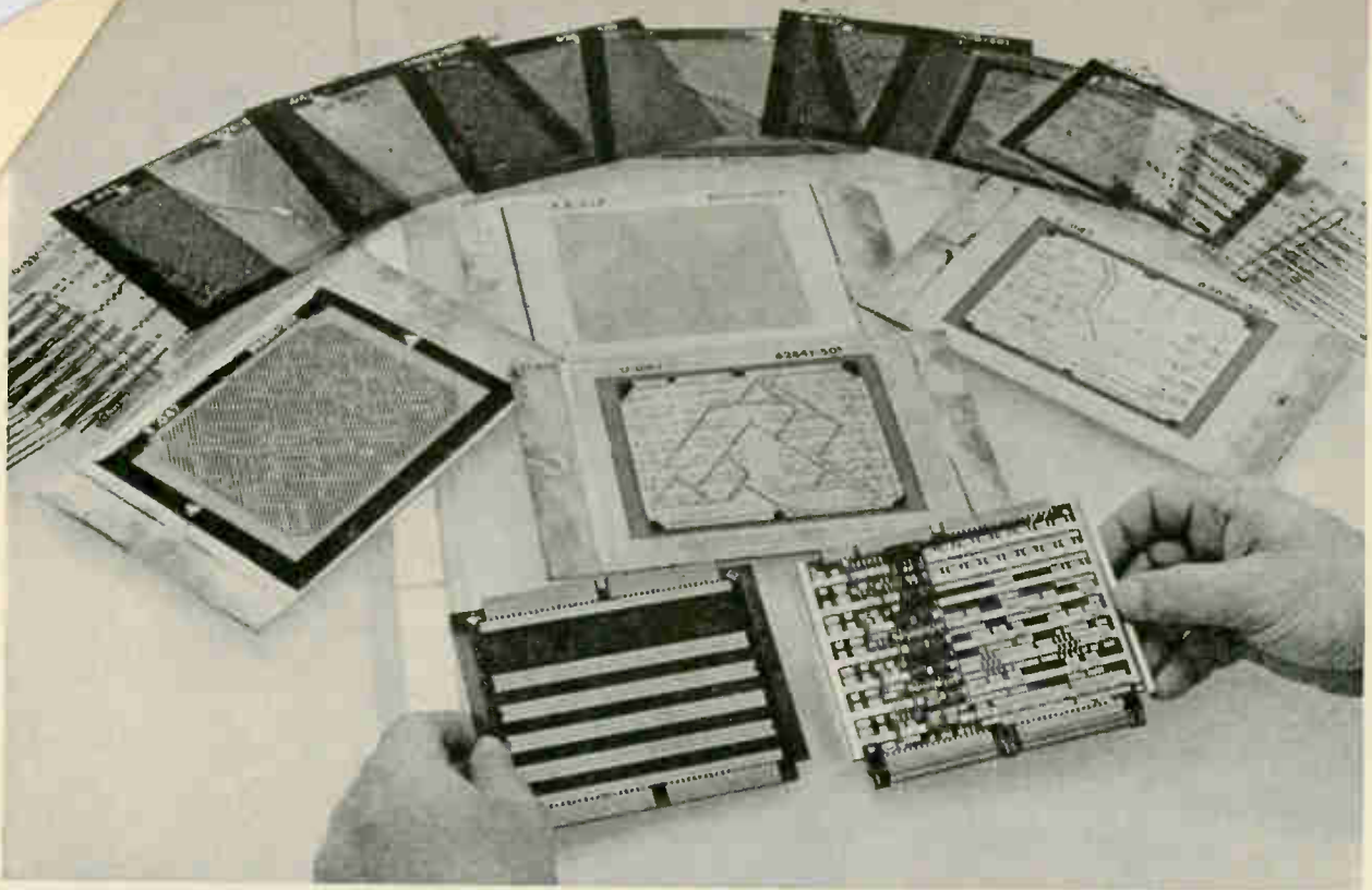
All the tool films for a complete board are spread in a semicircle at the top of the photo. In the center are laminates in various stages of fabrication. The left hand holds a laminated board and the right, a module.
