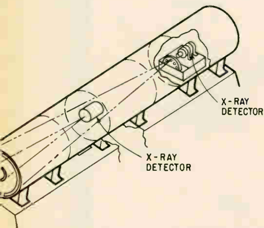
Two-in-one x-ray telescope will gather details on solar flares. Rays entering the slits on the face of the telescope are picked up by detectors and converted into video signals.
