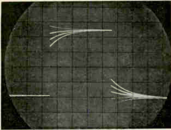
Single exposure photograph shows results of adjustments made to a system being tested with a square wave. Persistence is adjusted here so responses to the last five adjustments are all shown for comparison purposes.
