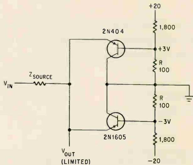
Transistor limiter uses minimal d-c power to establish reference voltages and simulates a diode with small internal d-c resistance.
