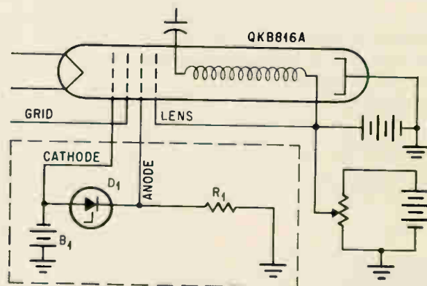
Zener diode circuit in the plate supply prevents excessive anode-to-cathode voltages.
