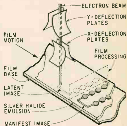
Basic elements of electron beam recorder
