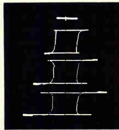
With new cores, the hysteresis loop has a constant shape once the threshold field is exceeded. Threshold is determined by value of horizontal spikes.
