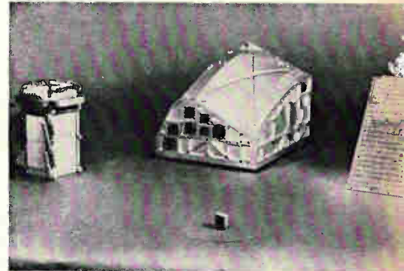
Gemini computer (center) shown with its memory element (left). In foreground is example of microcircuit used; these are interconnected with printed wiring plane similar to that shown at right.
