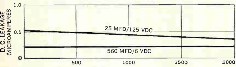
Typical life-test data: TLS-E capacitors.
