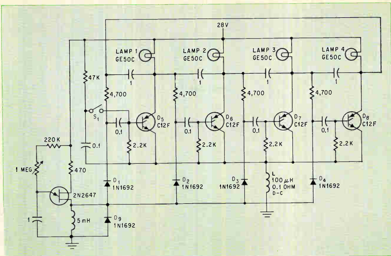
Rotating light (beacon) circuit. Lamps light one at a time beginning with L_1 when power is applied.
