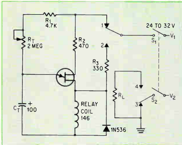
Use of a single unijunction transistor and a microminiature relay is practical and provides excellent isolation for time delays ranging from 0.5 second to 3 minutes. Capacitor C_T and resistor R_T determine the timing interval.
