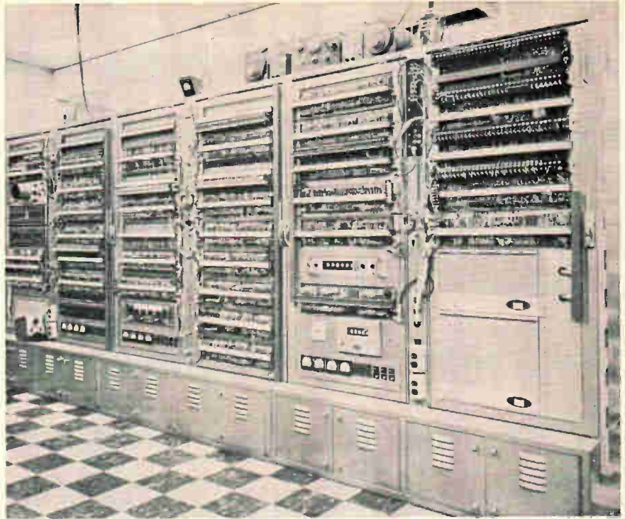
MIT's sequential encoder/decoder (SECO) here in lab form transmitted one billion bits without error. The LET uses a modified SECO system.
