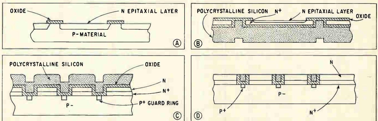
Three routes to the transistor islands: Sketch A illustrates etch regrowth; B shows dielectric isolation and etch regrowth; C and D show dielectric-junction isolation before and after the excess polycrystalline silicon is removed.
