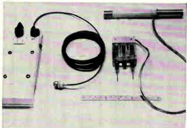
Control transmitter, left, is connected to small spherical hydrophone with coaxial cable. The receiving hydrophone, upper right, contains decoder circuitry that operates, on command, three hypodermic syringes (above foot rule). The system was designed by H. A. Baldwin and G. F. Ingle of the Sensory Systems Laboratory.
