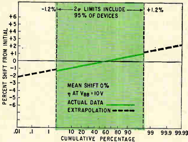
Probability distribution for intrinsic standoff ratio shows that 95% of devices exhibited a shift of less than 1.2% after 1,000 hours. Fifty units were tested at 600 milliwatts and 10 volts with temperature cycling. The mean shift was zero. Since a typical delay circuit is designed to withstand a shift of 5%, this performance is highly satisfactory. Green area indicates range of shift by 95% of units.
