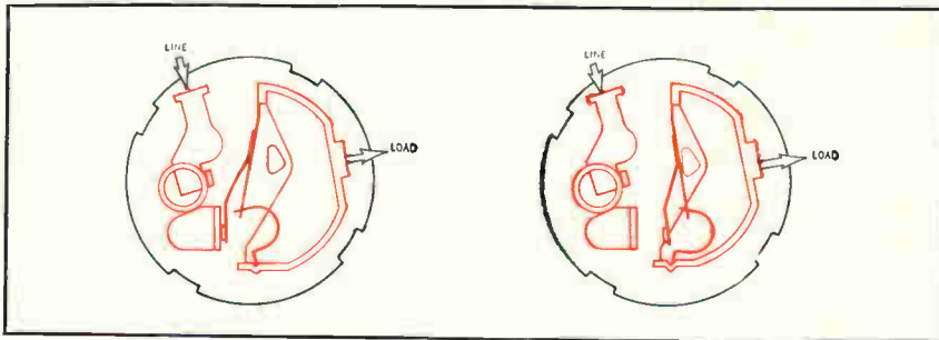
Diagrams show operation of breaker mechanism: at left, in MAKE position; at right, in BREAK position.
