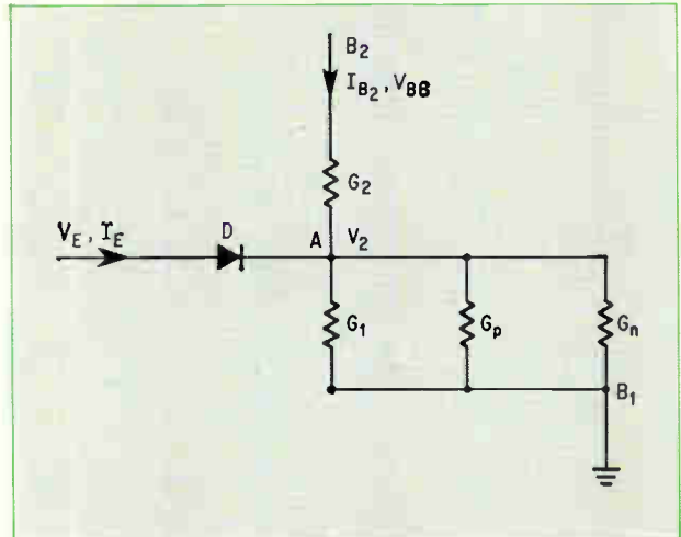
Equivalent circuit for a unijunction transistor. G_p and G_n represent the excess hole and electron conductivities between the emitter and base one. G_1 and G_2 are the conductivities corresponding to R_{B1} and R_{B2} .
