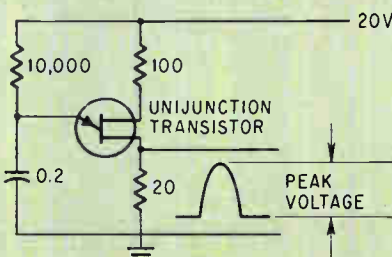
Test circuit commonly used for measuring base-one peak pulse voltage
