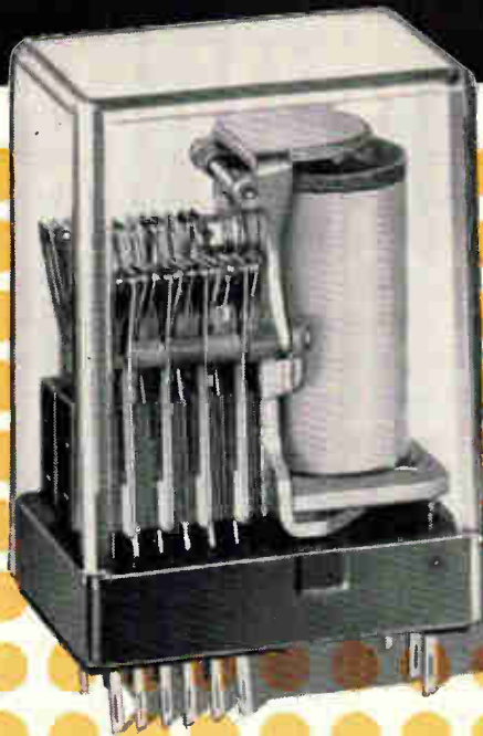
Type JDP Relay with mating socket for plug-in mounting
