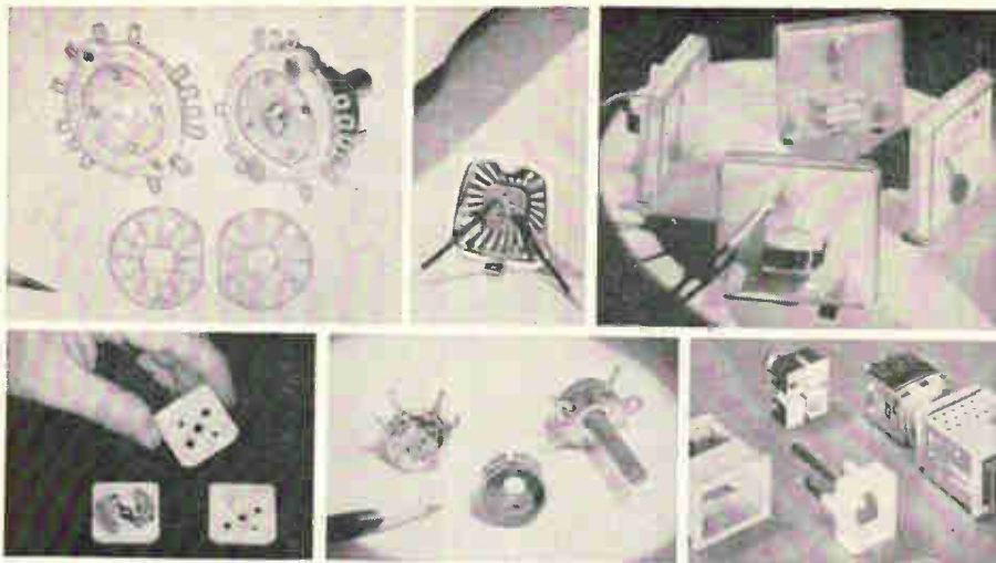
Fiberglass reinforced thermoplastic molding compounds are solving problems of precision, strength and reliability in dozens of electrical-electronic applications.
