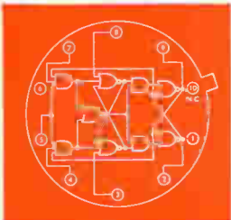
LU320 J-K BINARY ELEMENT
