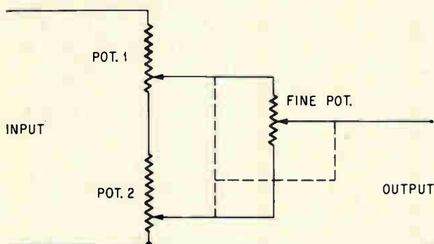
Vernier potentiometer is used to improve accuracy of hand-set resistance values.
