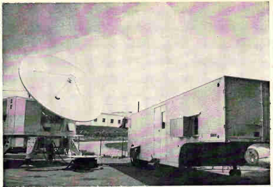
Lincoln Experimental Terminal. From the laboratory grounds at Lexington, Mass., this transportable terminal communicates with experimental satellite.
