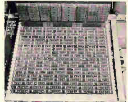
Integrated circuits cut LET's SECO size to five inches of panel space from three 6-foot racks.
