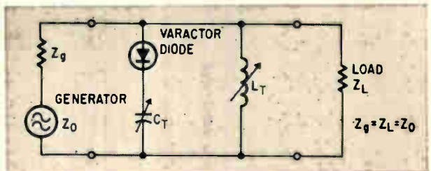
Simplified parallel tuned switching circuit. The switch is in the on condition (allows transmission of power) when the varactor diode is in the off condition (reverse biased).
