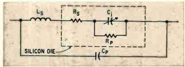
Small-signal equivalent circuit for a reverse-biased (non-conducting) varactor diode. The package contributes components L_s and C_p . The components R_s , C_j , and R_p represent the device itself.
