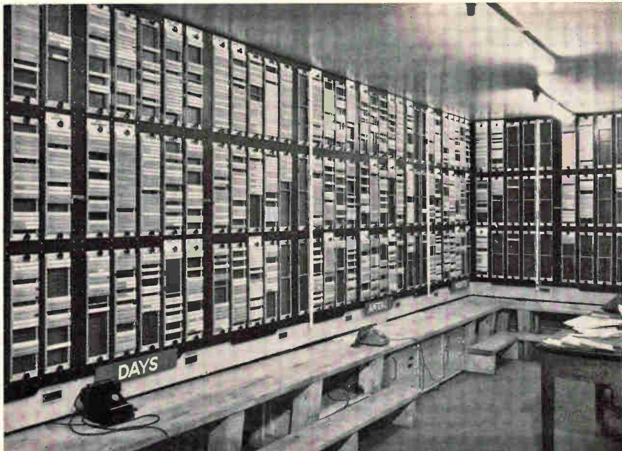
Time office at Brookhouse colliery. Boards are scanned for binary-coded wage data from each name plug. Control electronics fit under counter beneath grey telephone. Printout is done by teleprinter at extreme right.
