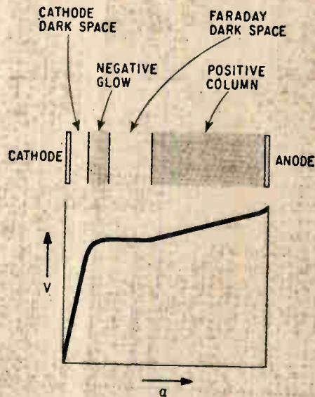
Voltage distribution between anode and cathode of a gas diode shows relation to the glow discharge
