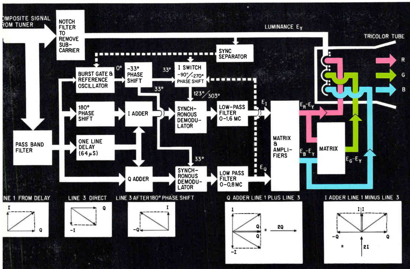
Deluxe PAL receiver. Simultaneously adding and subtracting the delayed signal (line 1) and the direct signal (line 3) recovers separate I and Q components averaged over two lines. The PAL transmitter is exactly the same as the NTSC transmitter except that the subcarrier in the I modulator reverses in phase every line.
