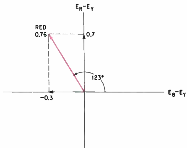
Resultant chrominance signal has an instantaneous phase and amplitude that can be shown vectorially using as axes the two difference signals that are modulated 90^\circ apart. Saturated red is shown.
