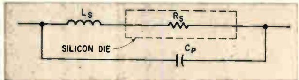
Small signal equivalent circuit for the varactor diode when forward biased. The semiconductor portion of the device is represented by R_s .
