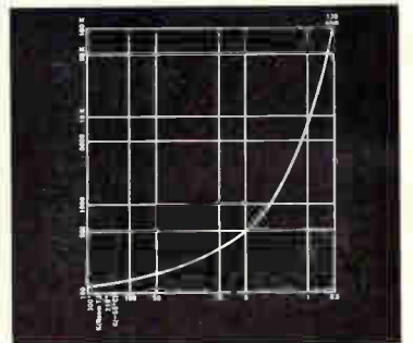
Log graph shows resistance-temperature characteristic of Speer 130-ohm carbon resistor between 300°K and .1°K.
