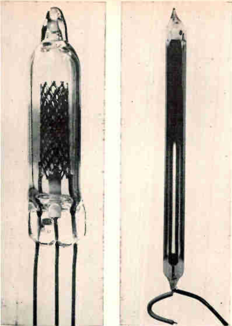
New cold-cathode indicator tubes are being designed specifically for transistor circuits. An example is Mullard's ZA1004. Tube is 26 millimeters long.
