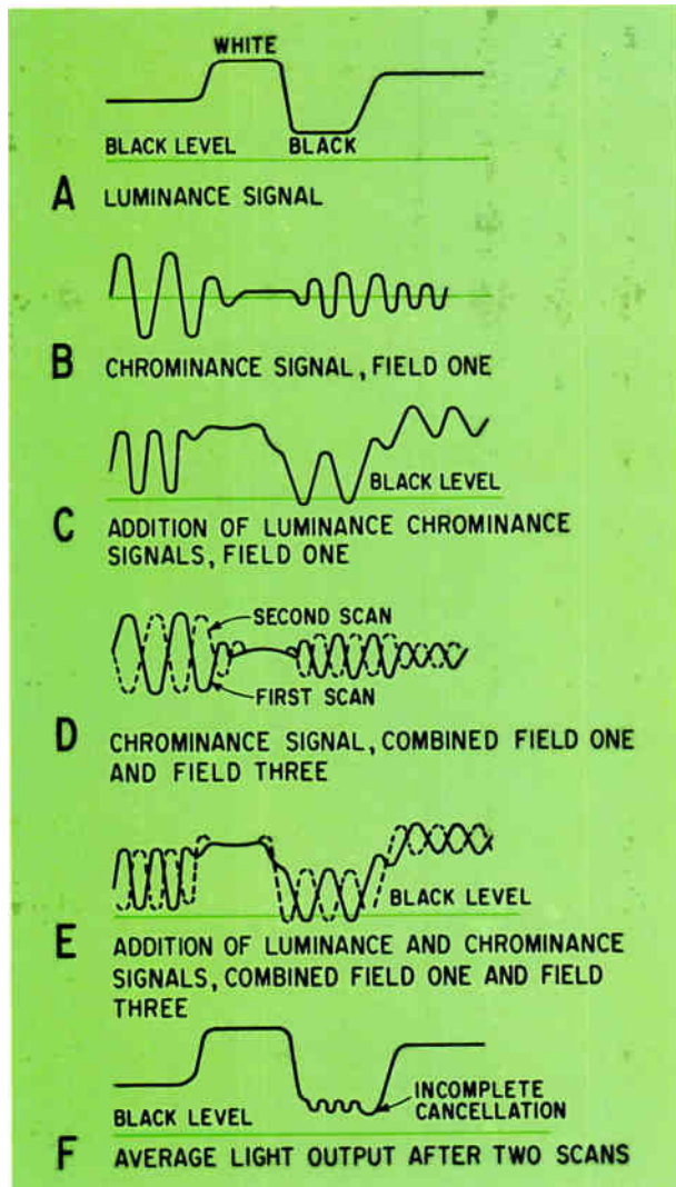
Frequency interlace, plus persistence of vision, leaves original luminance information undistorted despite addition of chrominance signal. Subcarrier frequency is chosen so that it reverses every frame, canceling after two frames.
