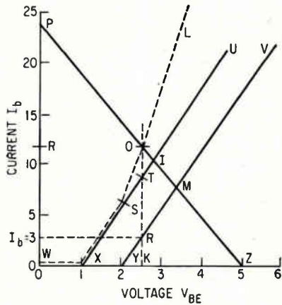
TWO UNEQUAL diode type loads in parallel leads to unequal load currents in DCTL logic. See text for discussion—Fig. 3
