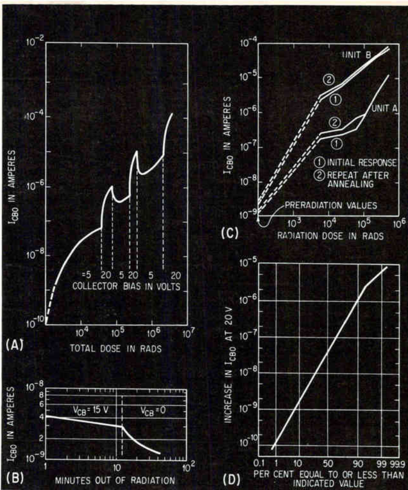
CURRENT I_{CBO} increases steeply as circuit voltage is raised, recovers slightly when it is lowered (A). Decay of radiation effect with and without bias (B). Transistors return nearly to their original state if they are heat treated after being irradiated (C). Large variation in resistance to radiation of a single type transistor is illustrated in (D); if this device were to be used in radiation, careful selection of individual units would be desirable—Fig. 2
