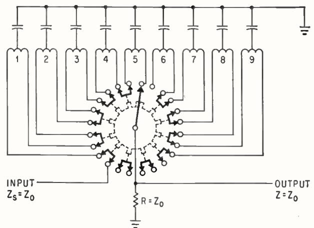
DELAY LINE SECTION INSERTION SWITCHING (V492)
