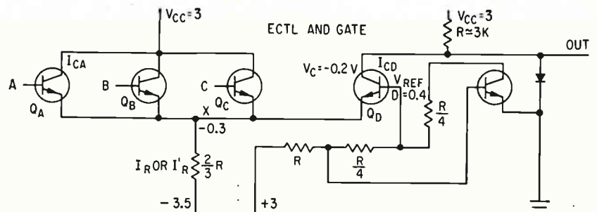
GATE has manufacturing simplicity of DCTL and is free from current hogging but uses two supplies—Fig. 8
