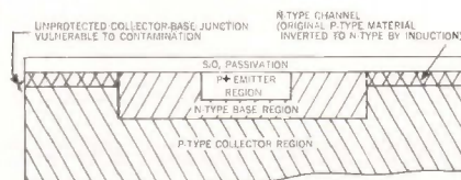
Cross Section of Planar Transistor
