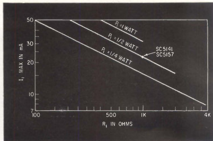
CURRENT LEVEL is limited by the power rating of R_L for switching applications—Fig. 4
