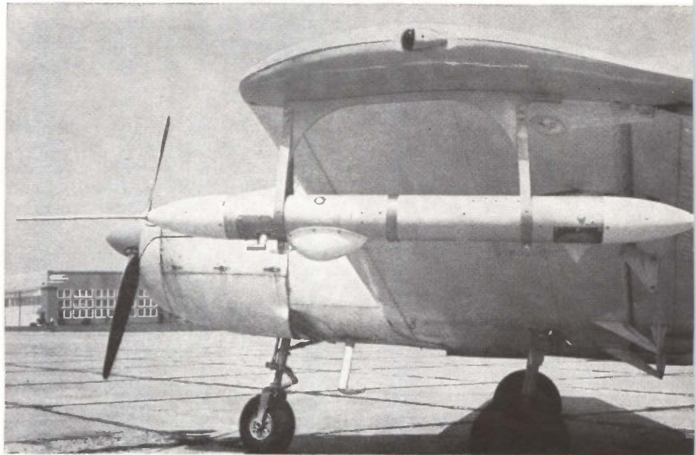
WEATHER DATA telemetry pod mounts to wings of subsonic aircraft. Maneuverability of aircraft, including drones, provides a flexible way to obtain weather profiles at altitudes up to 40,000 feet
