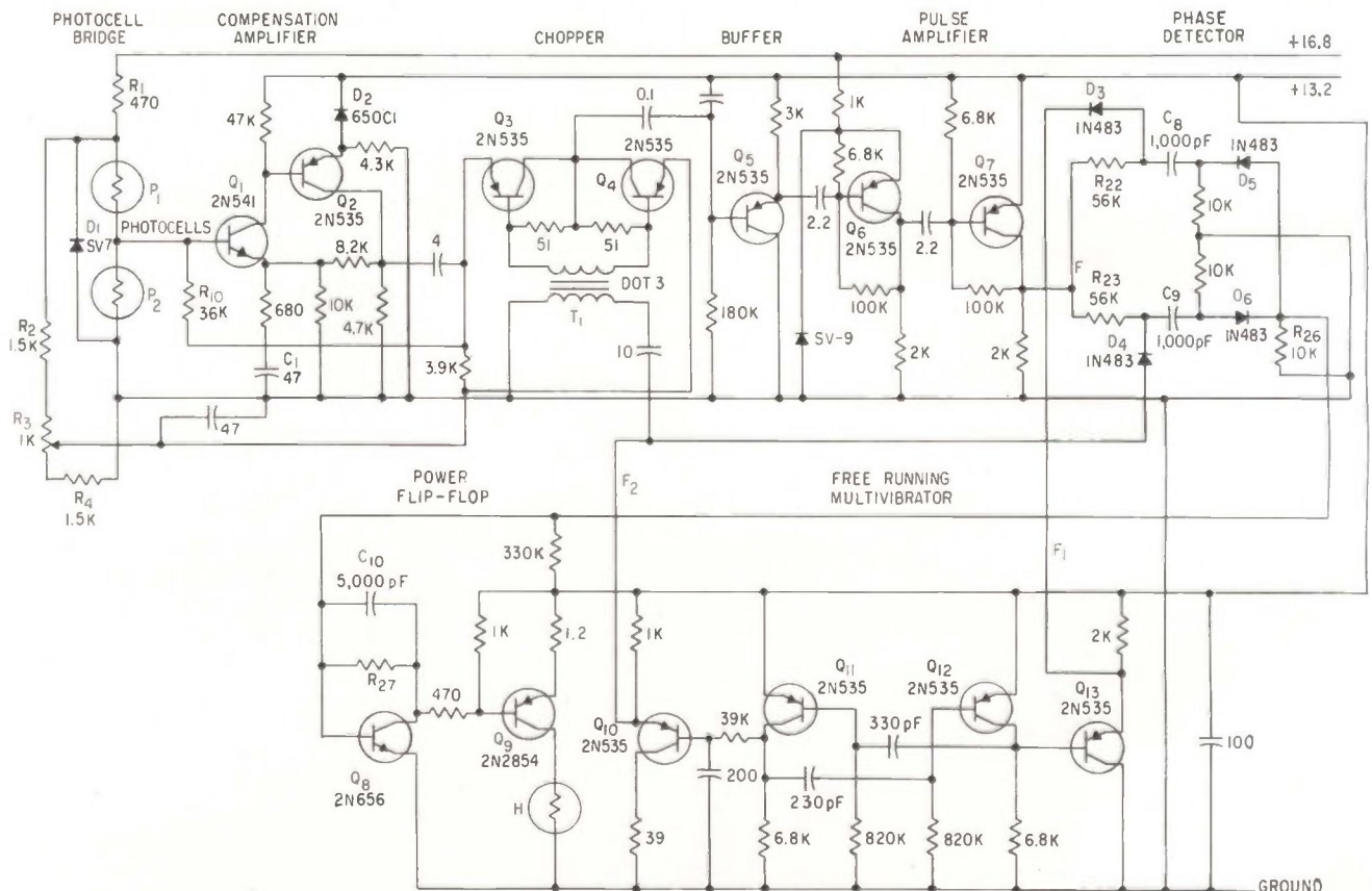
PHOTOCELL bridge circuit develops error signal for the dew point servo system. The heating coil is in the collector circuit of Q_9 —Fig. 3
