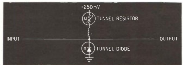
MONOSTABLE STAGE using tunnel resistor—Fig. 3
