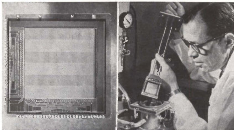
SUPERCONDUCTIVE, THIN FILM memory, shown recently by RCA's Sarnoff Research Center, stores 16,384 bits in 2 \times 2 -inch plate ( ELECTRONICS , June 28, p. 8). Experimental unit, only 120 millionths of an inch thick (left), accepts all connections on the plate itself—with 32 connections from the first plate and two for each additional. L. L. Burns of RCA Laboratories (right) lowers the memory into 3.6-degree K liquid helium.
