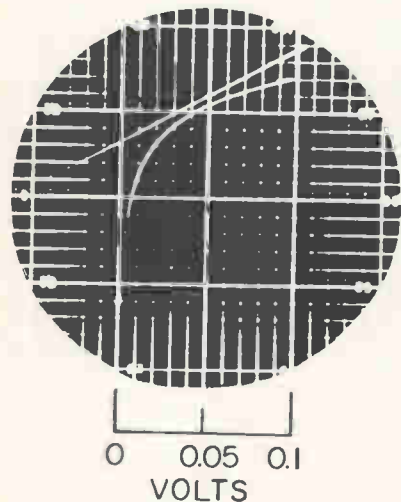
LOG I AGAINST V characteristics are viewed using this simple arrangement—Fig. 1
