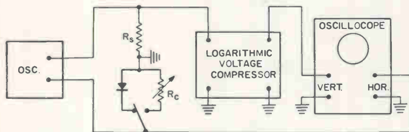
LOG I AGAINST V characteristics are viewed using this simple arrangement—Fig. 1
