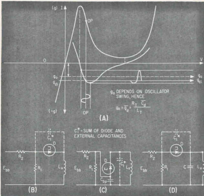
GRAPHICAL determination of time-average conductance g_o(t) and of its average value |g_d| (A). Lumped-constant circuits: series configuration, (B), parallel circuit (C), series-parallel version (D)—Fig. 2
