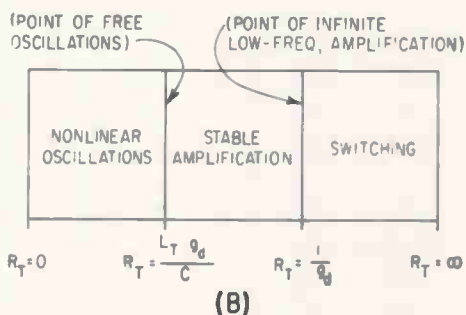
EQUIVALENT circuit of tunnel diode and its external circuit (A), graphical conditions for operating-stability (B), istics (C), evolution of tunnel diode package for minimum self-inductance, (photo, right)—Fig. 1
