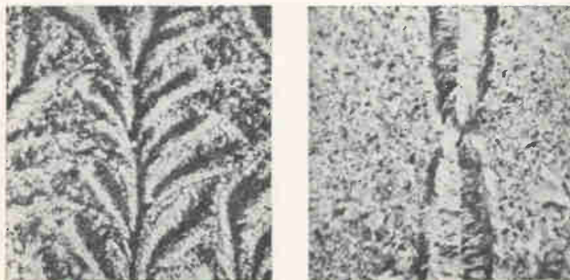
APPLIED ELECTRIC d-c field causes dendritic growth in silver telluride thin film. Recrystallization process is illustrated at left. Effect of a-c field on silver telluride growth is shown at right. From paper presented by C. Paparoditis of C.N.R.S. Laboratories, Bellevue, France, at single-crystal thin-film conference at Philco Research Center, Blue Bell, Pa.
