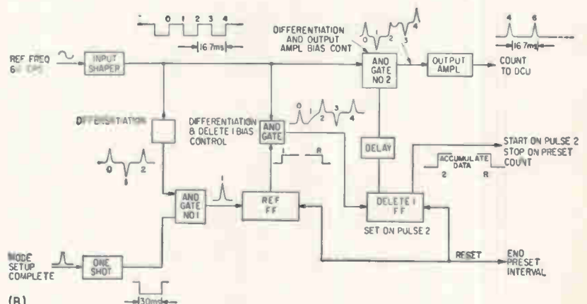
SIGNAL FLOW and switch-setup for a single preset time (A) synchronizing circuit shows how array of mode switches selects a preset time interval (B)—Fig. 4
