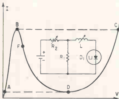
EQUIVALENT and practical circuits of multi-diode oscillator (A) with test results; crystal oscillator for 40 Mc (B), alternative oscillator locks onto 5th overtone of crystal at 160 Mc (C), characteristic curve traces operation of tunnel diode as it executes cycle of operation (D)—Fig. 4
