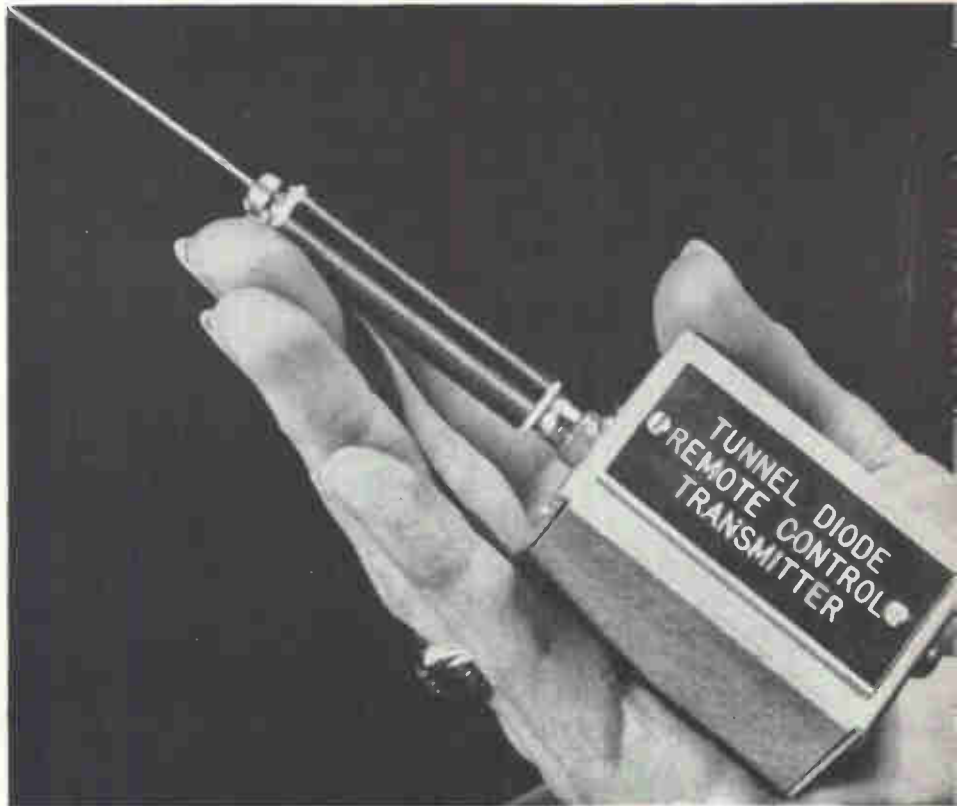
REMOTE-control transmitter features circuit simplicity, component economy, and long life from low-voltage batteries
