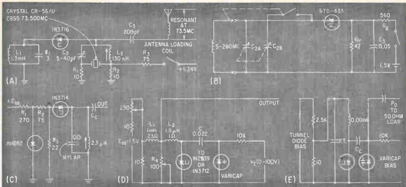
SELF-MODULATED low power transmitter (A) operates at 73.5 Mc; wide range oscillator (B) covers range 3 to 260 Mc using different plug-in tuning coils. Temperature-sensing oscillator changes frequency with changing temperature (C), voltage-variable capacitor enables oscillator to be tuned electrically over the 12-22 Mc range (D); high-frequency electrically tuned oscillator operates in the 200 to 400-Mc range (E)—Fig. 5
