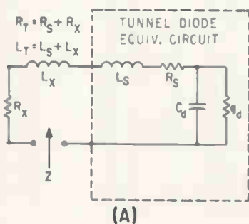
EQUIVALENT circuit of tunnel diode and its external circuit (A), graphical conditions for operating-stability (B), istics (C), evolution of tunnel diode package for minimum self-inductance, (photo, right)—Fig. 1
