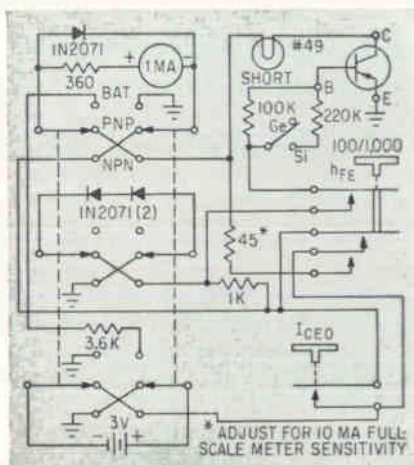
THE h_{FE} push switch has two depth positions. First multiplies meter value by 100. Fully-depressed position multiplies value by 1,000
