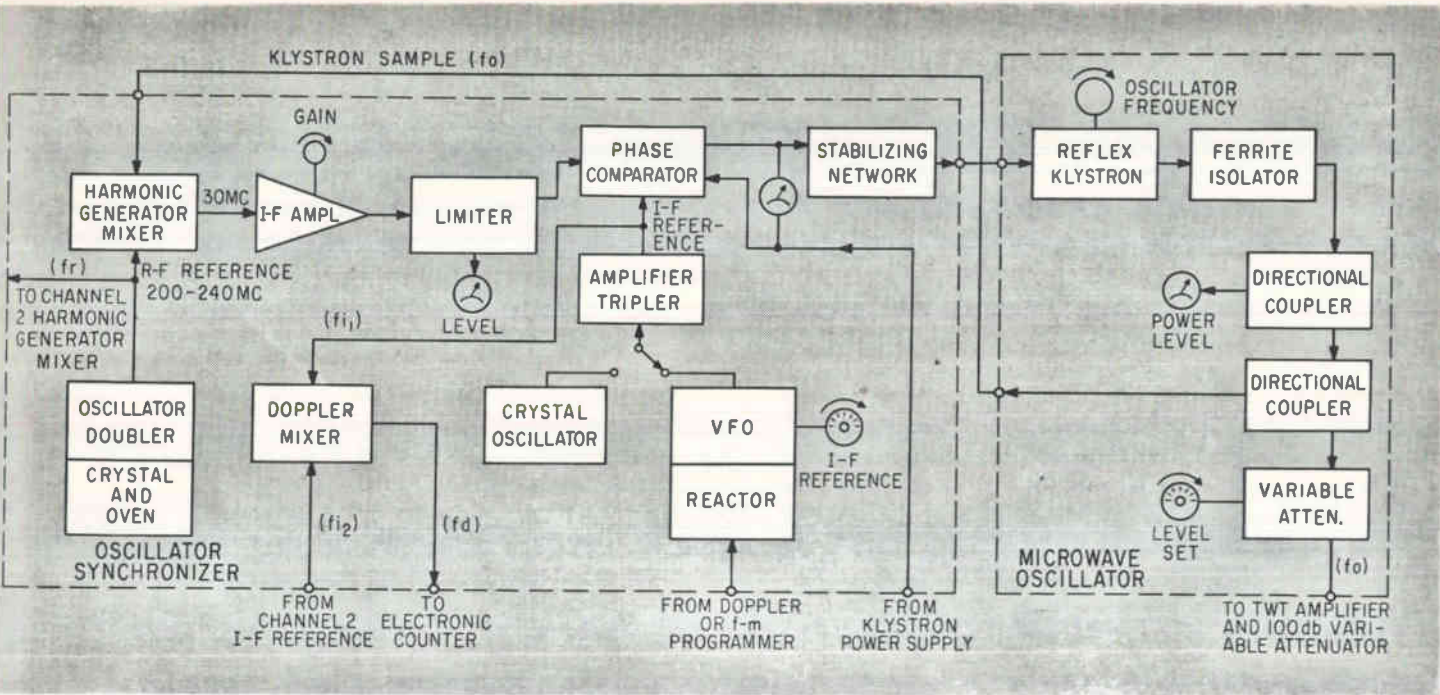
CHANNEL 1 of the doppler-simulator. Channel 2 is identical, except as noted—Fig. 1
