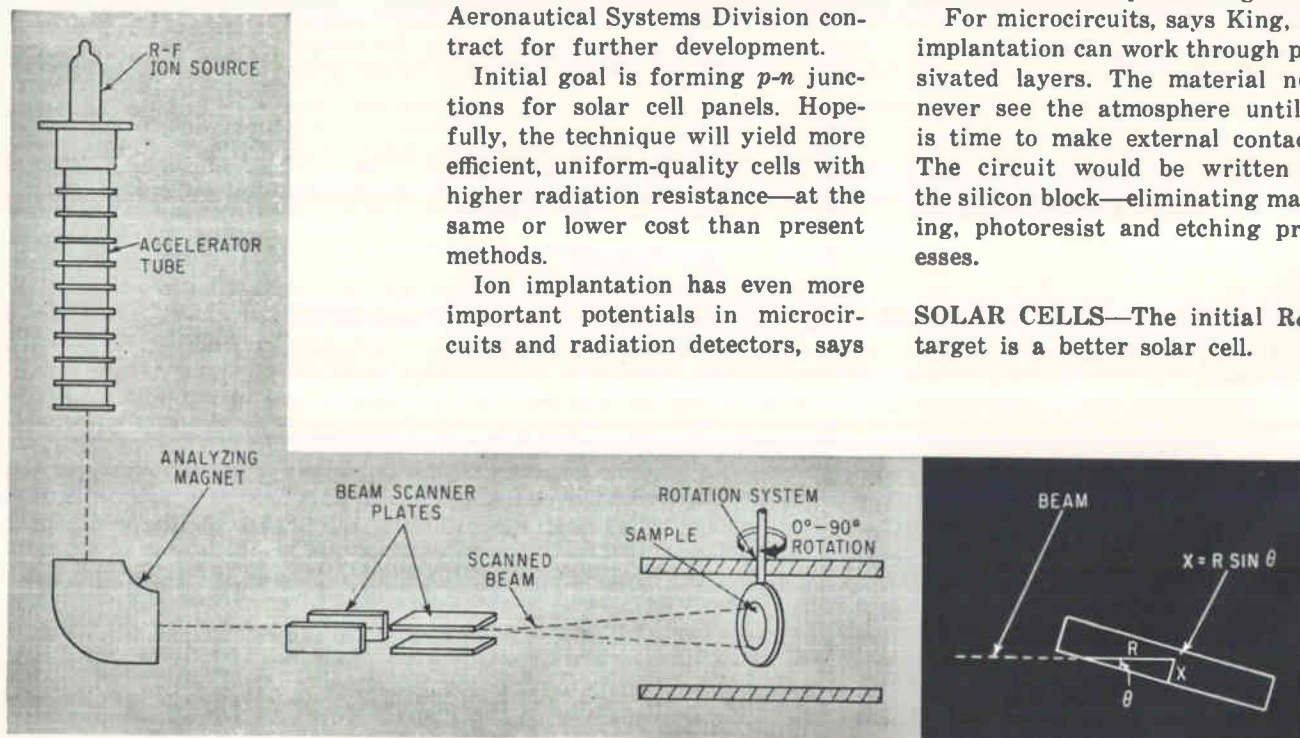
ROTATION SPEED of sample controls integrated flux at predetermined depth below surface
