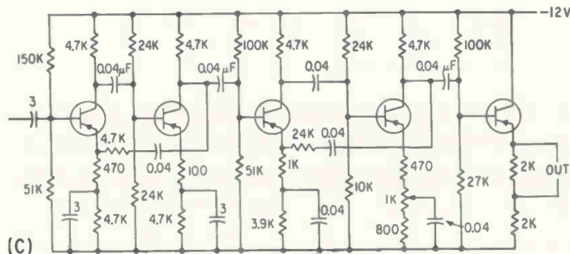
MULTIPLIER phototube output of system (A) is fed to impedance transforming circuit (B) and to amplifier (C) in two channels—Fig. 1
