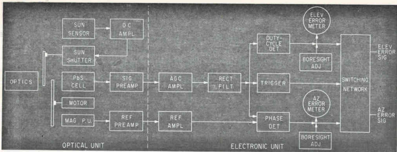
OPTICS package includes clock generator that provides reference signal for elevation and azimuth information. Electronic unit uses agc that accommodates variations in target intensity over 10,000:1 range—Fig. 3
