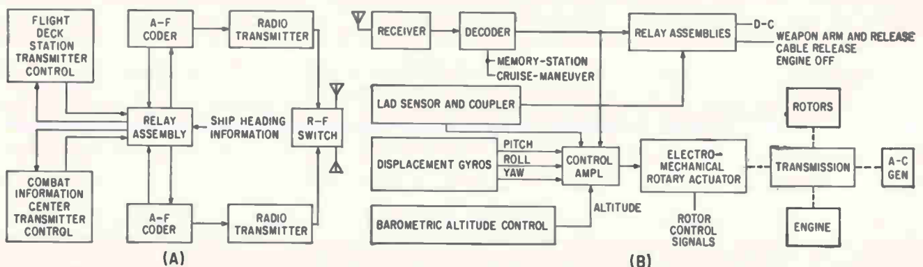
SHIPBOARD CONTROL system (A) guides the drones. Redundancy in coders and uhf transmitters provides reliability. Airborne electronics system (B) converts digital signals to analog for drone control. Amplifier controls attitude and altitude servo clutches of electromechanical actuator in response to commands from decoder and attitude sensors
