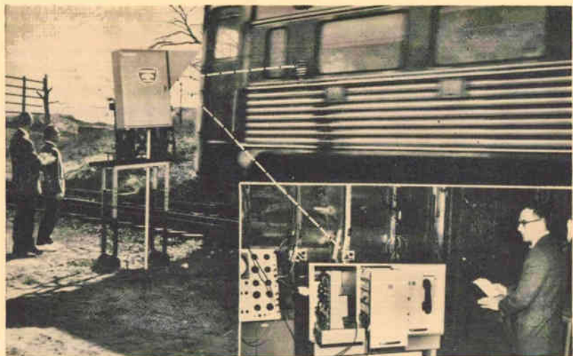
SCANNER developed by Sylvania identifies and records number of moving railroad car. Number is coded on colored, reflective strips on the side of the car. The scanner sends out white light and gets back colored light, which is then converted into electronic impulses. The decoding and printing units are shown in the inset.
