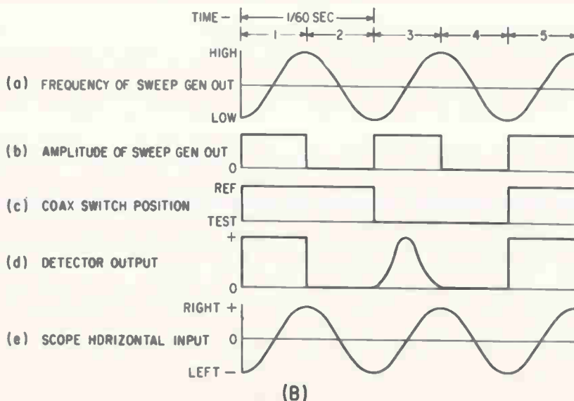
COAXIAL comparison circuit measures high-frequency loss with sweep-frequency display (A); waveforms show how display is generated (B)—Fig. 1
