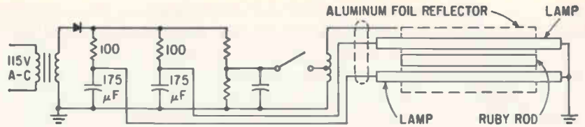
SAFETY FEATURE in the laser system is isolation of the capacitors by resistors so they cannot accidentally discharge together at full power
