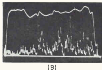
RETURN LOSS of the triple-tuned bandpass filter with 130-Mc center marker and side markers at \pm 3.5 -Mc (A) and return loss at one end of a 1,000 ft length of good coax cable between 4 and 100-Mc (B)—Fig. 6
