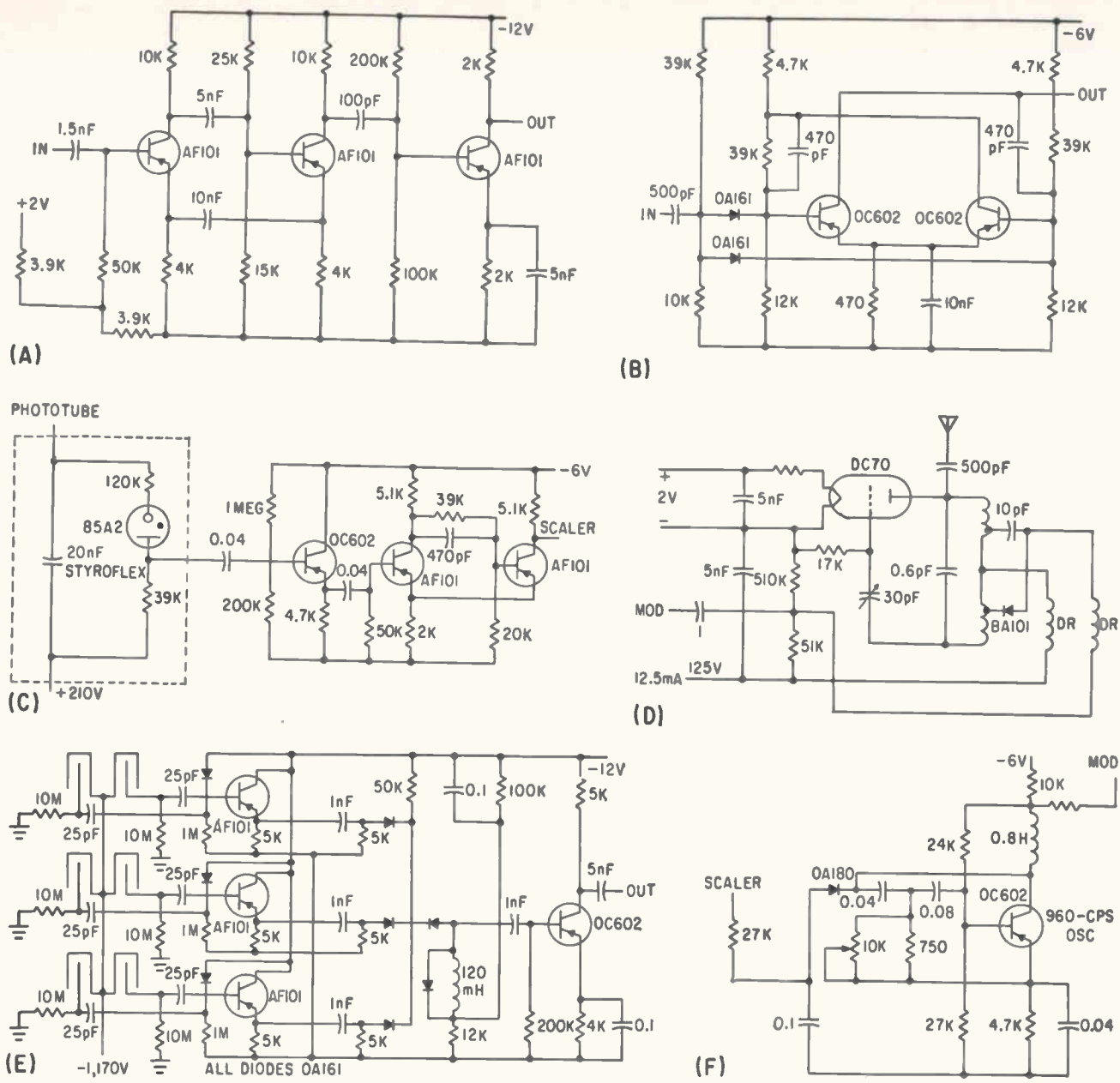
CIRCUITS are shown of discriminator (A) binary scaler stage (B), ionization channel input circuit (C), vhf transmitter (D), counter telescope (E) and subcarrier oscillator (F)—Fig. 2
