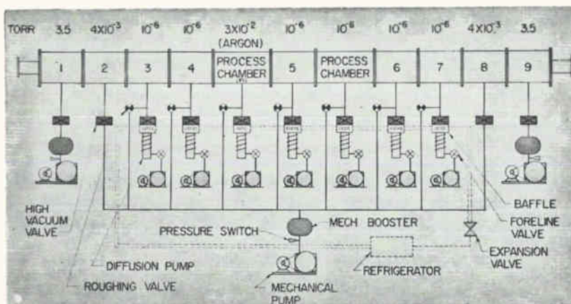
TANTALUM resistors are now being deposited in first process (deposition) chambers. Second process chamber will be used to deposit gold conductors. When in use, pressures in process chambers are higher than in adjoining
