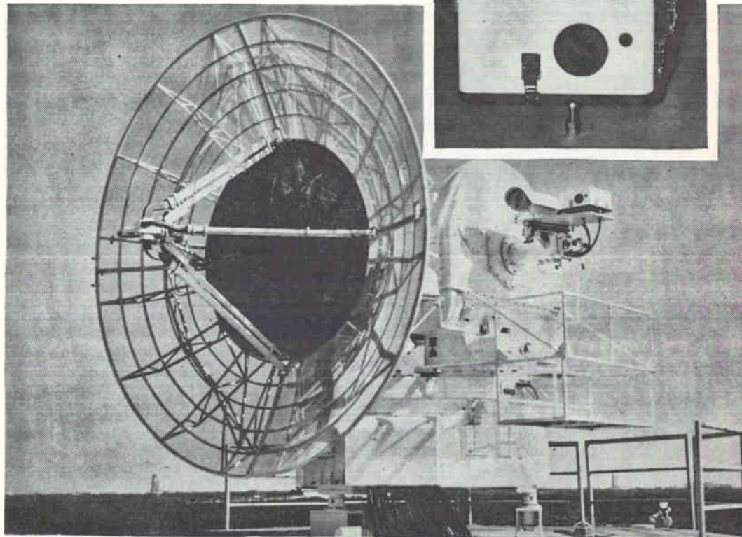
INFRARED OPTICS package mounted on radar bowl's elevation trunnion to the right of bowl's rim and expanded view of optics package
