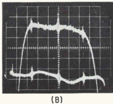
CHANNEL 13 tv amplifier with reference trace at a gain level of 57 db (A) and the identical response with vertical gain expanded 5 times (B)—Fig. 5
