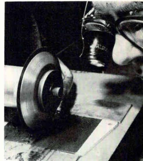
Each plate is spirally cut with a 0.006-in. diamond saw
