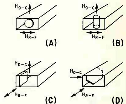
FIG. 3—Microwave circuit was for different type samples
