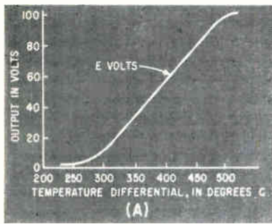
FIG. 3—Output voltage versus temperature differential (A), terminal voltage versus load impedance (B) and output current versus load impedance (C)
