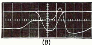
FIG. 4—Number of bits that can share sense-digit circuits is shown at (A) for various cycle rates. Word access time for 5-Mc memory is shown at (B) with sense amplifier output on upper trace and word line voltage on lower trace. Large horizontal divisions are 0.02 usec and large vertical divisions are 2 volts
