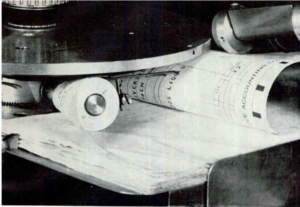
Cycloid paper pickup developed by Rabinow handles flimsy papers
