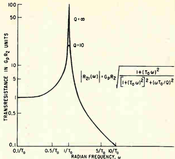
FIG. 3—Effect of Q on transresistance
