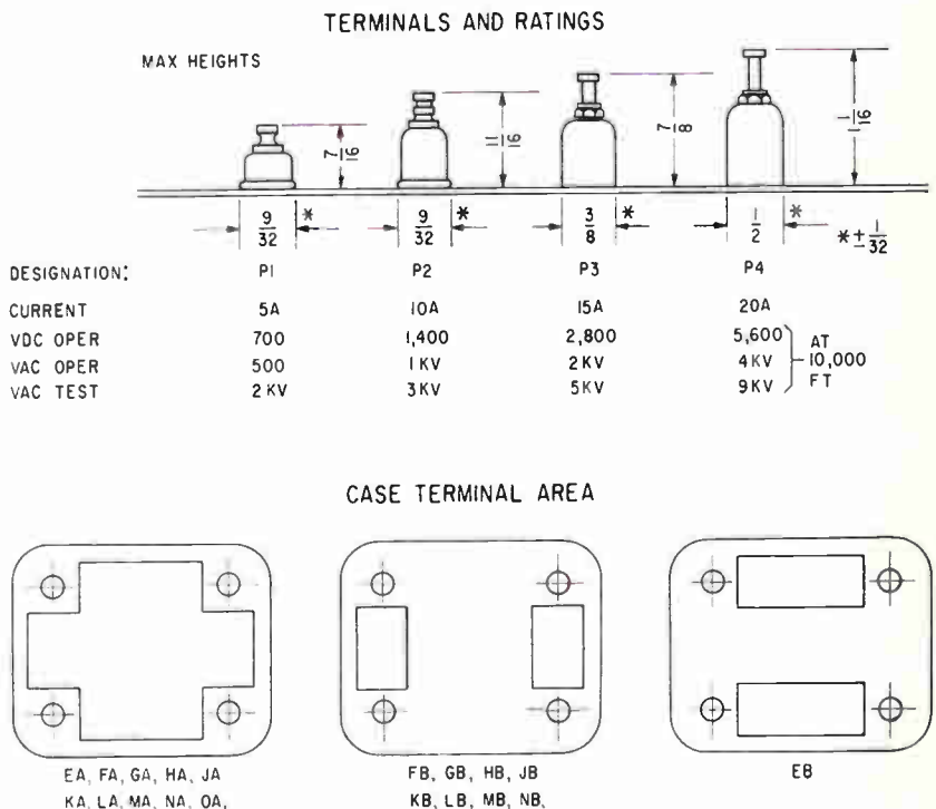
FIG. 3—Terminals and terminal layout guide
