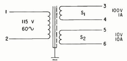
FIG. 1—Electrical requirements of transformer in example
