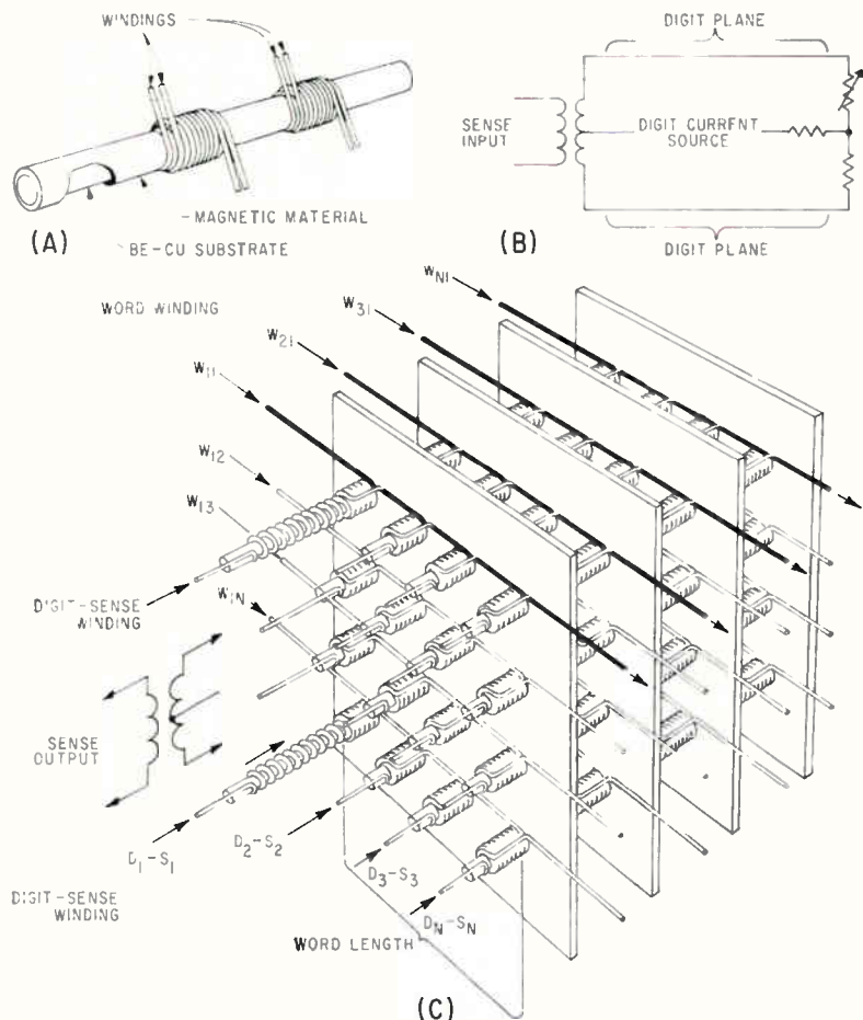
FIG. 1—Rod structure with solenoid windings is shown at (A), shared sense-digit winding bridge at (B) and memory organization at (C)
