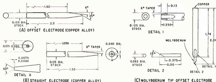
The right electrode for each weld depends on such factors as the diameter of the wire being welded, accessibility of the weld area, flexibility of component leads, and pressure-energy requirements of the weld schedule
