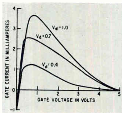
FIG. 2—Current-voltage characteristic of the gate circuit for various values of drain voltage
