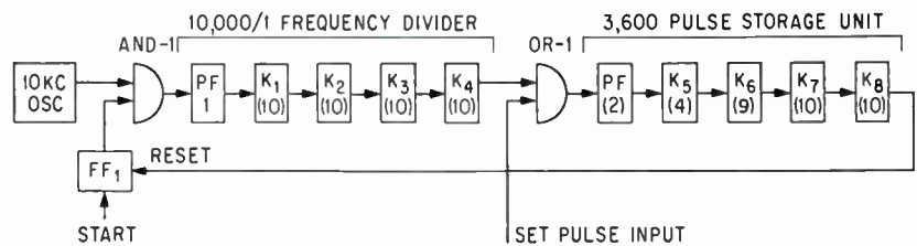
FIG. 3—Divider chain delivers output pulse after preset number of seconds when driven by 10 Kc oscillator. Storage unit is partly filled (saturated) before counting; delivers output when last stage reaches saturation. Information may be stored for days without deterioration
