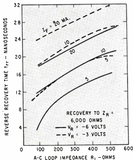
FIG. 4—Reverse recovery characteristics for 3DG001 and 2DG001 diodes, with different circuit parameters
