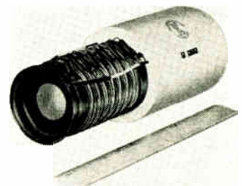
Magnetically focused image intensifier with encapsulation partially sectioned
