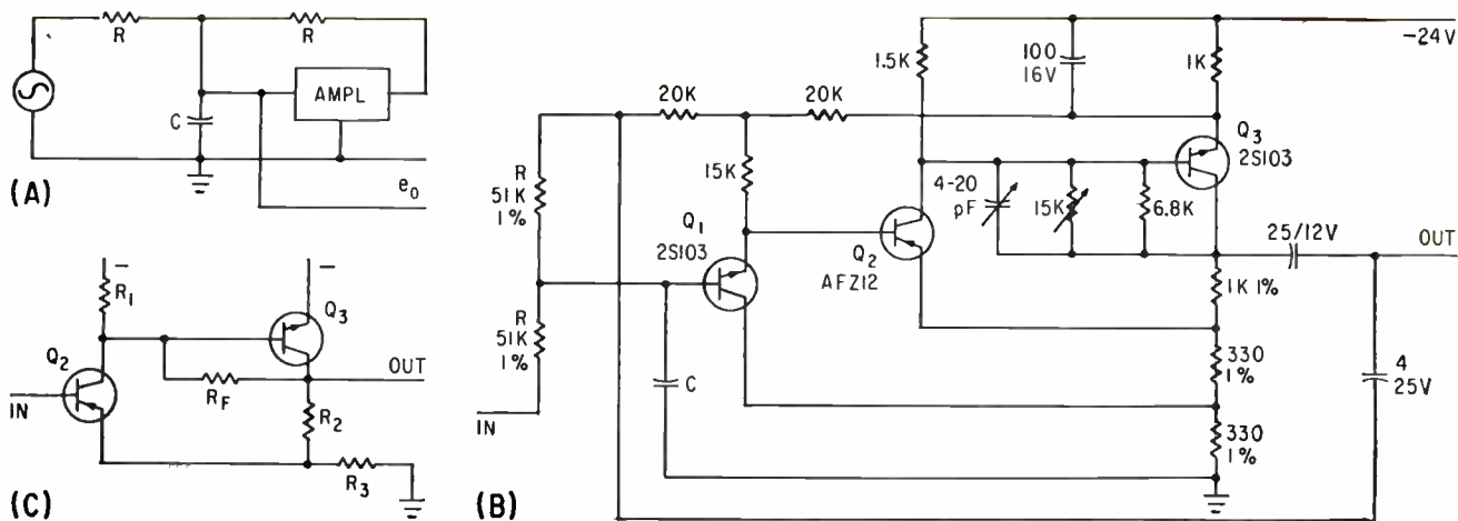
FIG. 1—Basic integrator (A); complete integrator circuit (B); simplified circuit of feedback pair (C)
