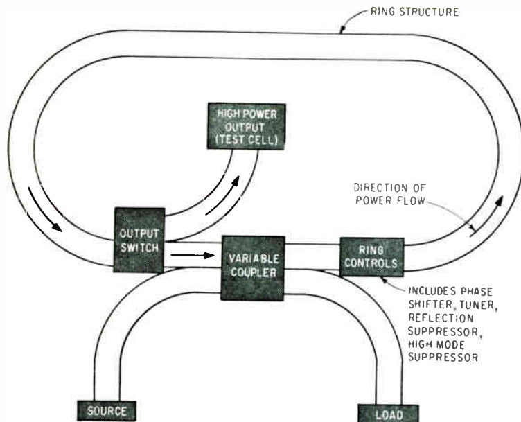
FIG. 3—Pulses are fed into the microwave flywheel (A) from the source in phase with the energy in the ring. Proposed low pressure arc-discharge gaseous-shutter output switch (B) is made as part of a waveguide section
