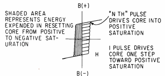
INCREMENTAL MAGNETIZATION OF COUNTER'S CORE
