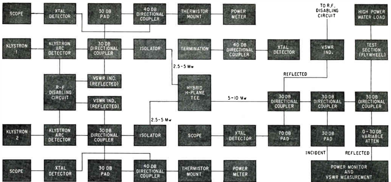
FIG. 2—R-F output circuit combines output of each klystron in a high power hybrid. Monitoring and protective circuits are shown
