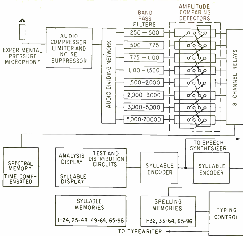
Speech input to microphone is analysed and converted into syllable code for operation of coded typer. RCA system types out words in real time
