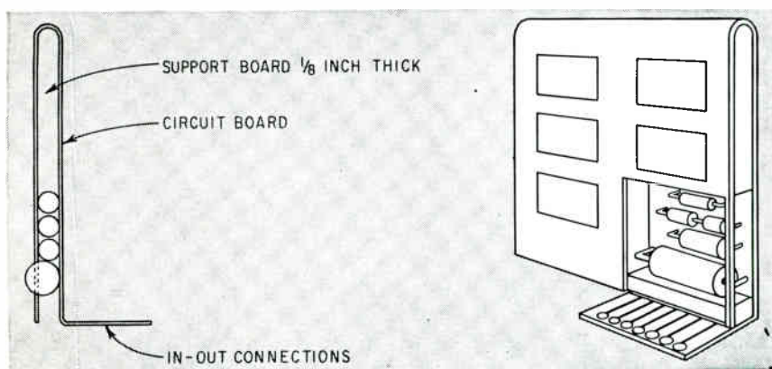
FIG. 3—Method of folding flexible board over the Silastic core
