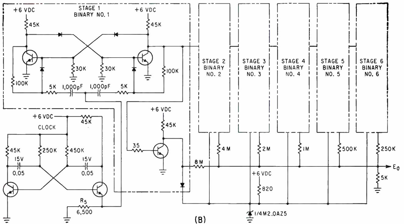
version of the generator circuit (B). Power-supply voltage has been lowered to 6 volts to reduce component sizes
