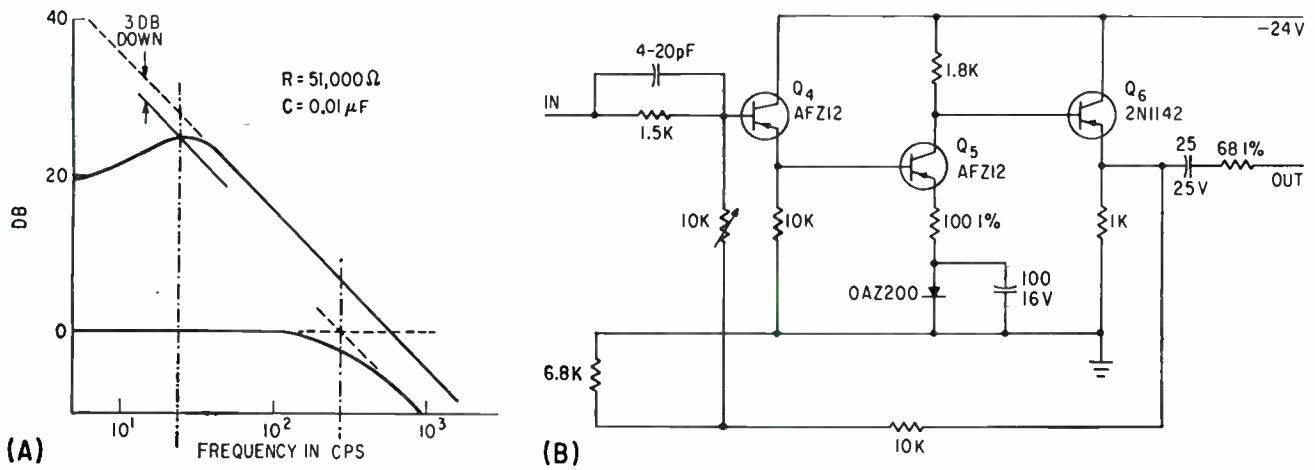
FIG. 2—Measured low-frequency response of integrator (A); line-driving amplifier (B)
