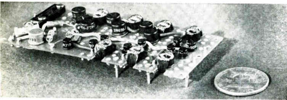
Timer-programmer designed for satellite application uses incrementally magnetized cores. Reliability is excellent
