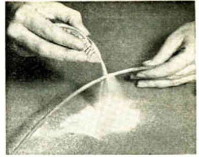
Conductive powder can be applied by pouring, dusting, spraying
