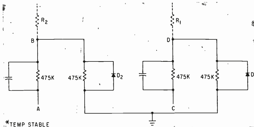
FIG. 2—Temperature compensation for the timing capacitors is obtained by inserting this circuit between AB and CD of Fig. 1
