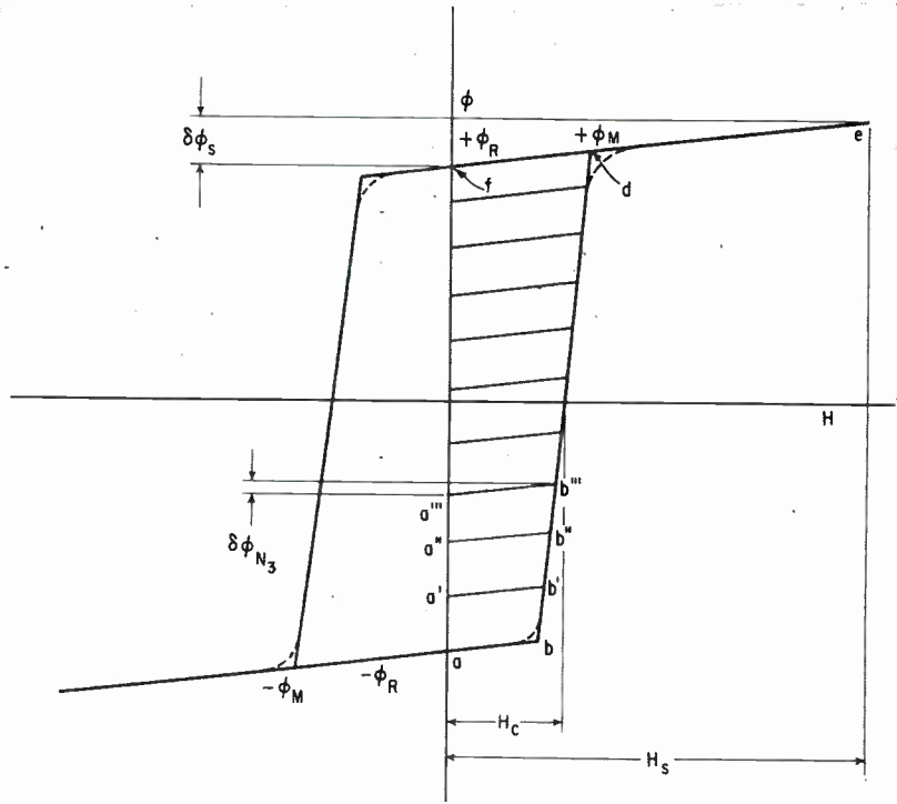
FIG. 2—Hysteresis loop shows this core is saturated by tenth input pulse. For given core, external circuit resistance and other parameters are adjusted to insure correct count. Adjustable counting is available with some cores; maximum count is 16
