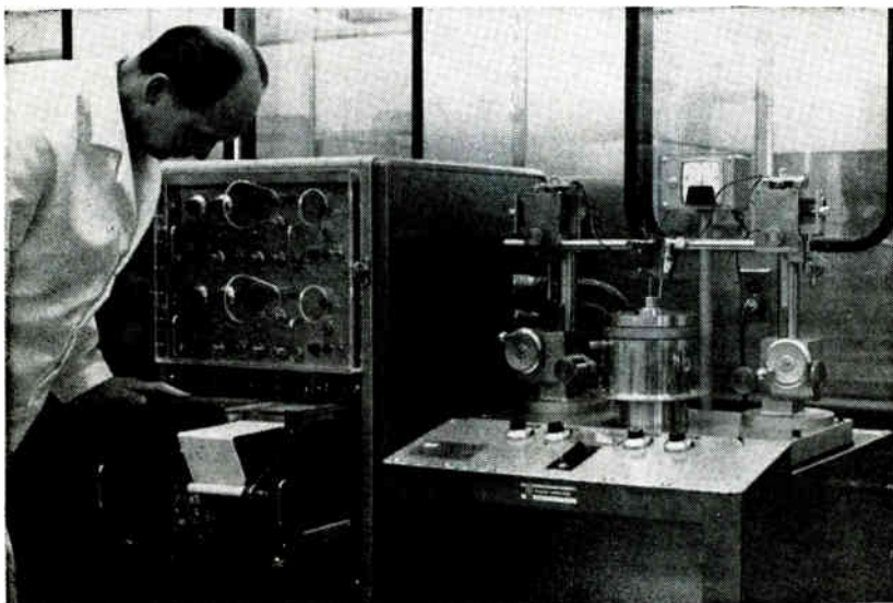
Movement of feeler arm is detected electrically as part is rotated to measure roundness within two-millionths inch using General Motors Roundrecorder at AC Spark Plug Division standards laboratory
