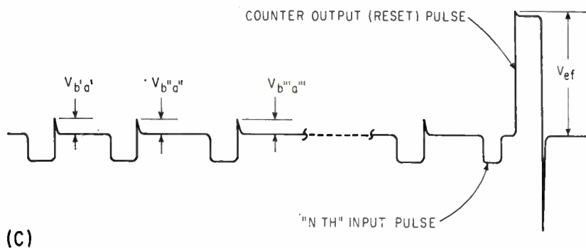
FIG. 1—Schematic circuit shows pulse shaper and first stage of a counting chain (A); redrawn circuit shows arrangement of blocking oscillator used to reset core (B); final saturating input pulse triggers blocking oscillator and produces output waveform (C)
