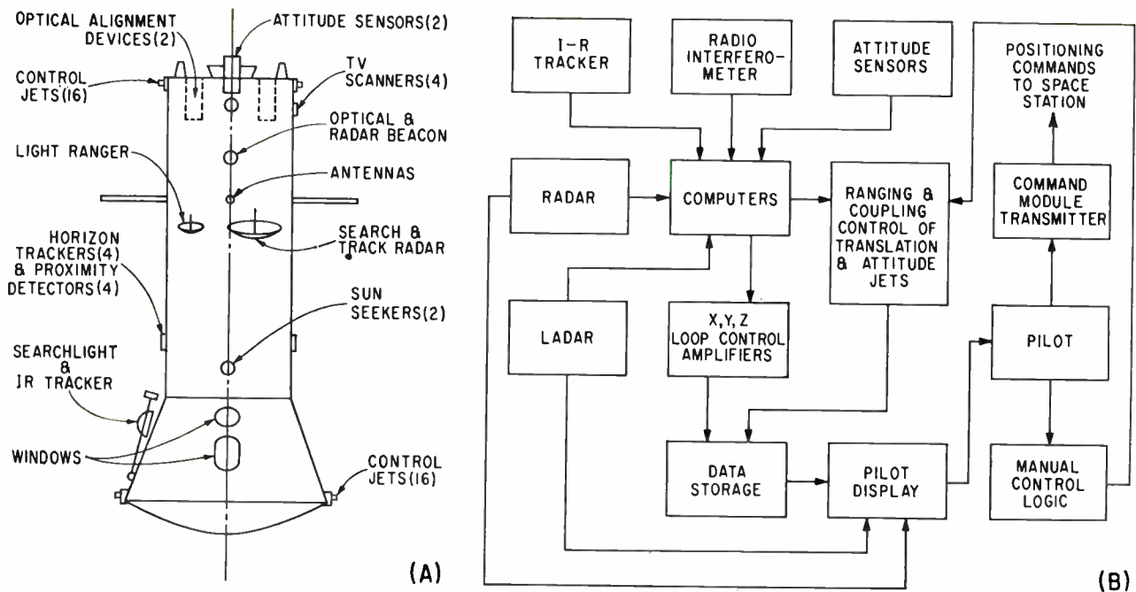
Space rendezvous homing and docking system proposed by Northrop. Sensors on manned capsule (A) would provide data for automatic and pilot control systems (B)
