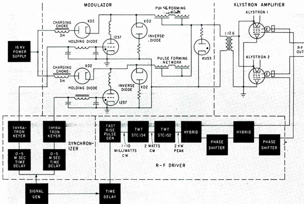
FIG. 1—Time delays in the modulator circuit and phase shifters in the r-f circuit synchronize beam and r-f pulses to permit parallel operation of the klystrons
