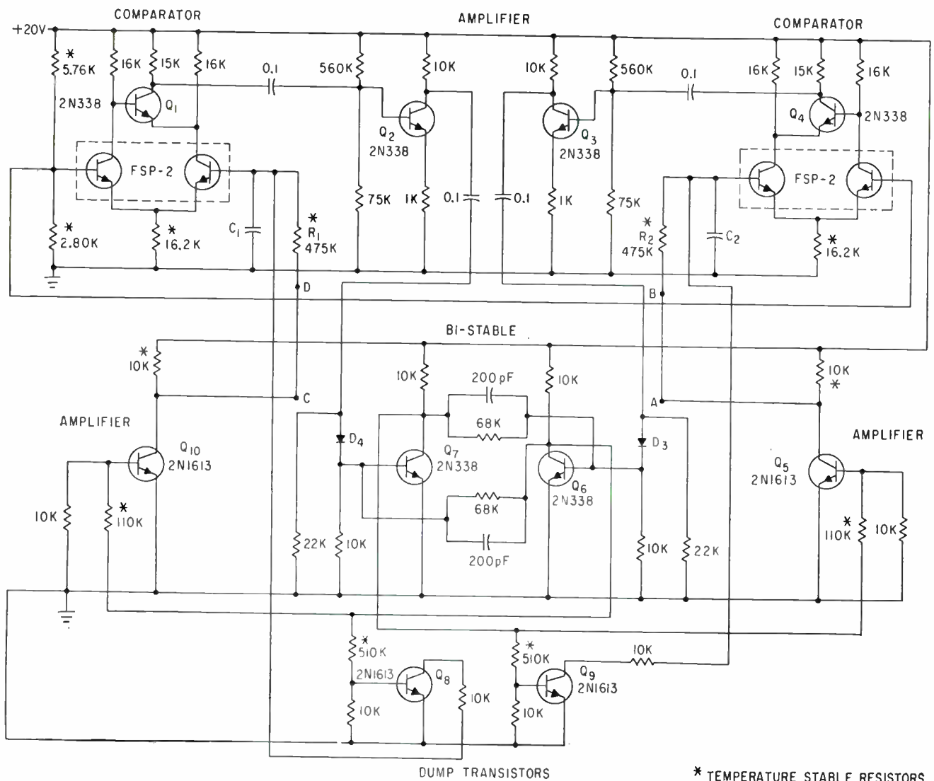
FIG. 1—Temperature stable resistors aid in reducing temperature coefficient
