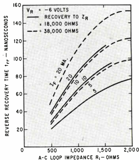
FIG. 4—Reverse recovery characteristics for 3DG001 and 2DG001 diodes, with different circuit parameters
