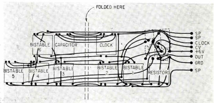
FIG. 2—Layout of the flexible printed board
