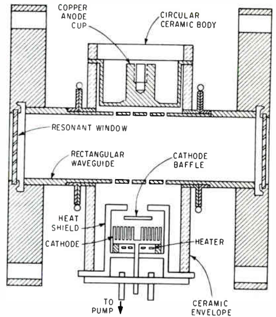
FIG. 3—Pulses are fed into the microwave flywheel (A) from the source in phase with the energy in the ring. Proposed low pressure arc-discharge gaseous-shutter output switch (B) is made as part of a waveguide section
