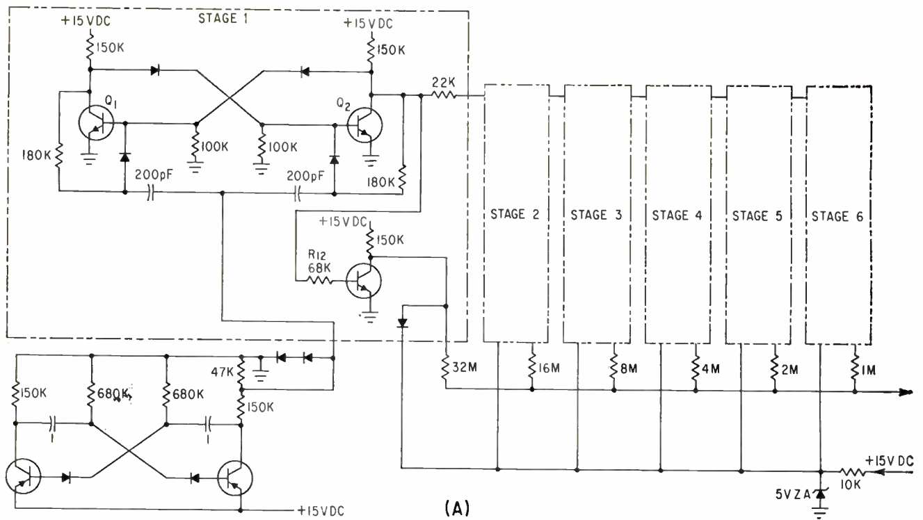
FIG. 1—Original circuit of the staircase generator before modification for thin-film construction (A), and modified
