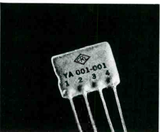
10 Couplate consists of plate and grid resistors, plate by-pass and coupling capacitors. Minimum soldered connections speed production.
