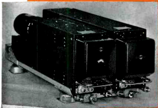
Collins 17L-2 vhf transmitter and 51R-2 vhf navigation-communication receiver in dual shock-mount.
