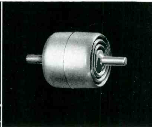
5 Hi-Vo-Kaps are filter and by-pass capacitors combining high voltage, small size and variety of terminal connections to fit most TV needs.
