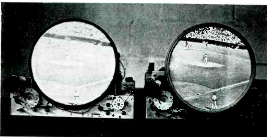
Picture tube at left has clear glass face that, although it transmits 90 percent of light from phosphor, has low contrast ratio because of room lighting and reflection of light from phosphor from front surface into dark areas. Tube at right has Teleglas face that transmits about 65 percent of light but shows contrast ratio of 35 to 1
