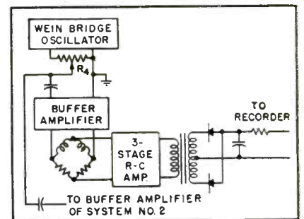
FIG. 2—Block diagram of complete carrier-type d-c amplifier system
