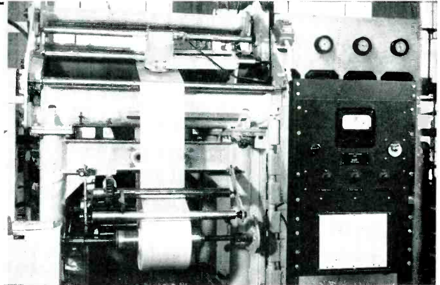
Installation of indicating radioactive thickness gage on machine producing thin plastic sheets at Dewey-Almy Chemical Co. plant in Lockport, New York. Ionization chamber is over plastic sheet at top of machine and radioisotope housing is directly under it beneath moving sheet material. Calibration chart is on rack at right, below indicating meter
