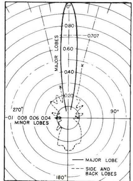
FIG. 1—E-Plane field pattern using dipole and disc reflector in a scale model parallel-wire paraboloid at a frequency of 1.325 mc. The H-plane pattern is similar except for slightly larger minor lobes
