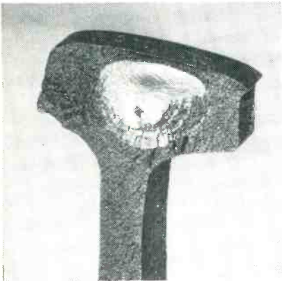
Transverse rail fracture of the type which is now prevented by early detection
