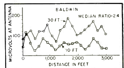
FIG. 5—At Baldwin, on the Jamaica radial, the median signal ratio was 2.4 (see position on profile in Fig. 3B)
