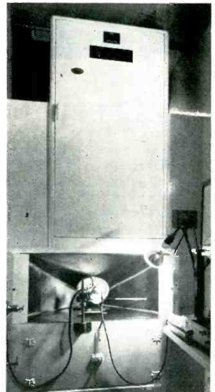
Constant speed rotating work table insures uniform deposits, and Raytheon electrostatic precipitator above table removes air-borne particles
