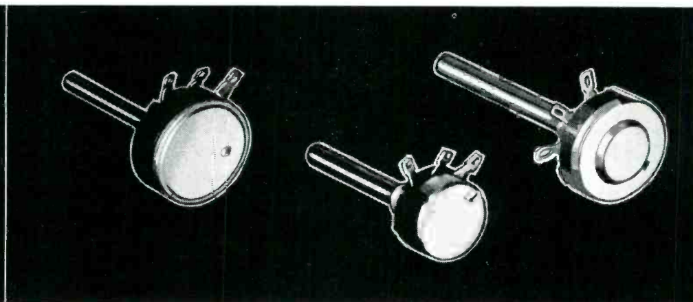
8 Let Centralab's complete Radiobm line take care of your special needs. Wide range of variations: Model "R" — wire wound, 3 watts; or composition type, 1 watt. Model "E" — composition type, 1/4 watt. Direct contact, 6 resistance tapers. Model "M" — composition type, 1/2 watt.
