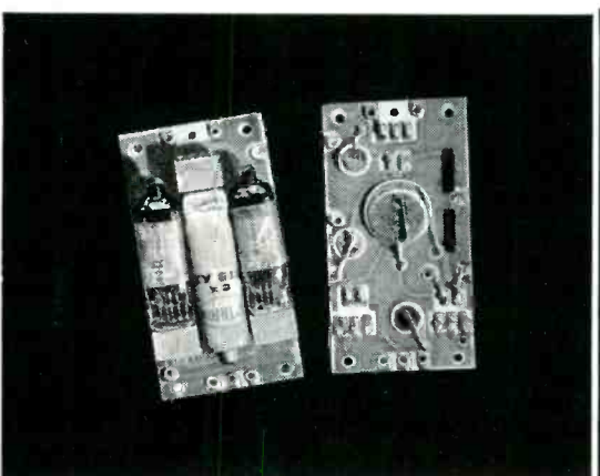
9 Centralab's Ampec , above, is an integral assembly of tube sockets, capacitors, resistors and wiring combined into one miniature amplifier unit.
