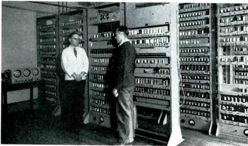
Convenience in replacing tubes is provided in the Edsac by its designers M. V. Wilkes and W. Renwick
