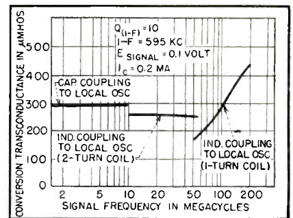
FIG. 6—Crystal-tetrode frequency characteristic for several coupling methods
