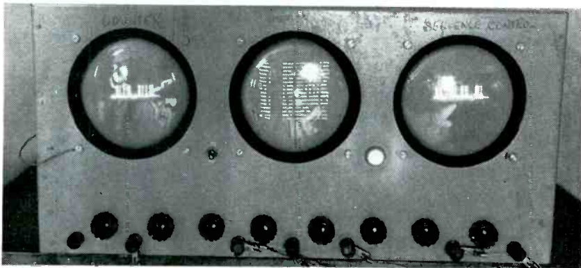
Timing monitor or counter tube, memory tube and sequence control tube are cathode-ray tubes in the Edsac
