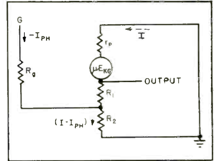
FIG. 3—Equivalent circuit of Fig. 2 for voltage analysis
