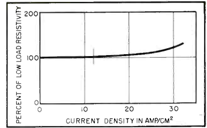
FIG. 4—Effect of current density on resistivity of MS-501 conductive plastic
