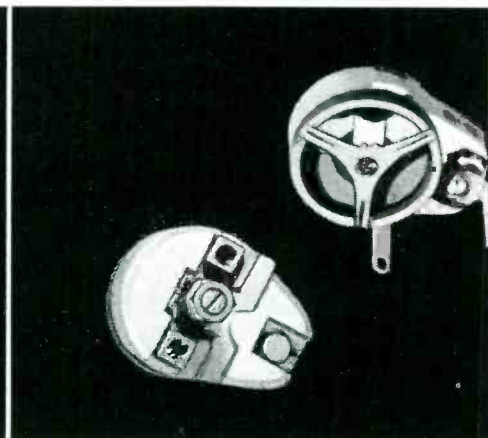
6 Ceramic Trimmers are made in five basic types. Full capacity change within 180° rotation. Spring pressure maintains constant rotor balance.
