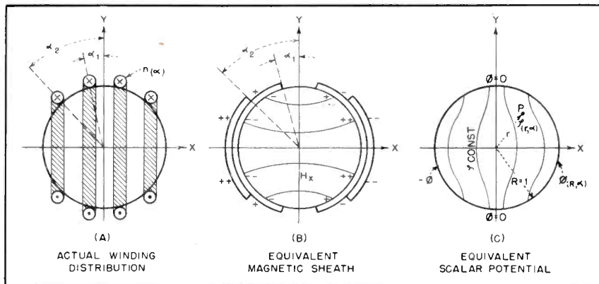
FIG. 3—Two-dimensional theory of deflection coils
