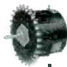
MULTITAPPED MODEL B HELIPOT AND 4-GANGED TAPPED MODEL F This Model B HELIPOT contains 28 taps, placed as required at specified points on coil. The Four-Gang Model F Potentiometer contains 12 taps on each section. Such taps permit use of padding resistors to create desired non-linear potentiometer functions, with advantage of flexibility, in that curves can be altered as required.
