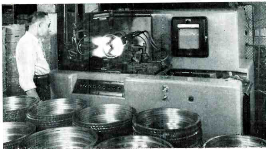
METALS INDUSTRY Newest application of electronic control in this major market for instrumentation maintains surface temperature of gears accurately to within 5 degrees F of required red-heat temperature, for selective surface hardening in Cincinnati Flamatic hardening machine. Sensitive radiation thermopile in overhead housing is focused onto work
