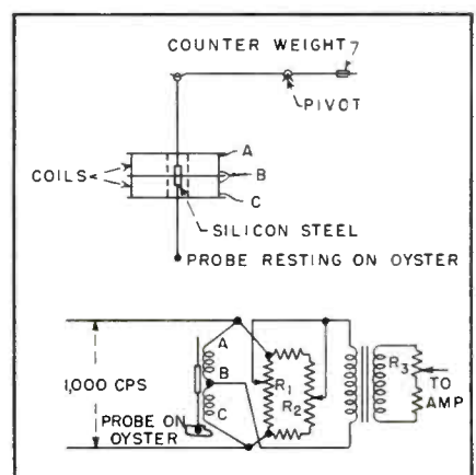
FIG. 1—Details of probe coils and detecting bridge
