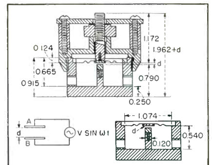
FIG. 1—Cross-sections of cavity and basic representation of secondary-emission switch
