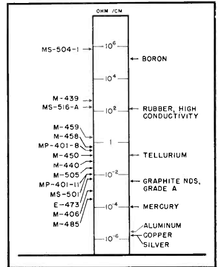
FIG. 5—Representative resistivity values of various Markite conductive plastics, compared with familiar conductors
