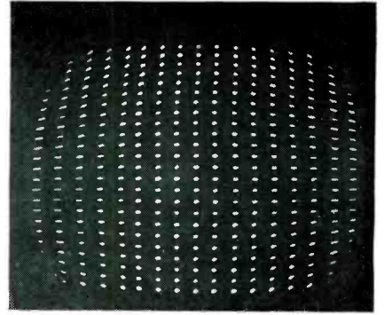
FIG. 12—Slotted-yoke pattern with vertical deflection corrected and horizontal deflection uncorrected
