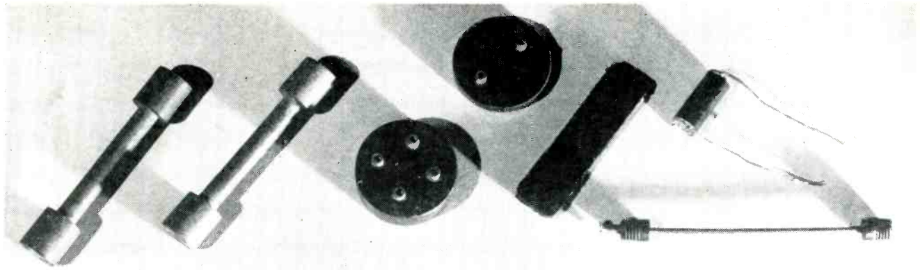
Samples of typical thermosetting, thermoplastic and elastomeric conductive plastics. Rods at left have less than 1 ohm resistance between ends. Leads are soldered directly to ends of
