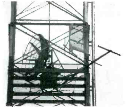
An eight-foot parabola was mounted on a platform of the WMAL-TV tower in Washington
