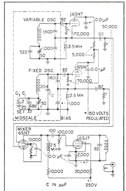
Schematic diagram of highly stable twin oscillator with output from 1.75 to 2 mc
