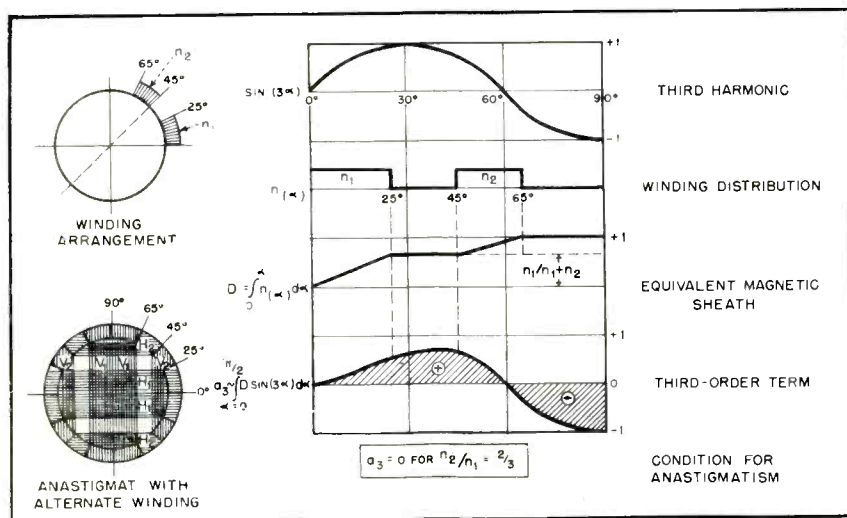
FIG. 5—Anastigmatic deflection yoke with alternate winding
