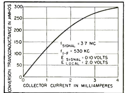
FIG. 3—Curve of conversion transconductance with respect to collector current
