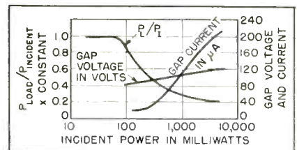
FIG. 2—Operating characteristics of cavity, showing the electron current in the gap, the gap voltage and the ratio of power transmitted to the load as functions of the incident power upon the cavity as functions of the incident power
