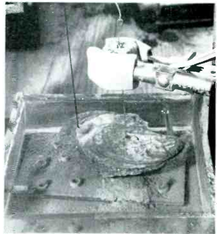
Pickup mechanism of instrument as positioned for observing the heart beat of an oyster that is slowly dying in a salt-water environment simulating that produced by industrial pollution. Coils are held by clamp. For this usage, the instrument has been named an astredynamometer
