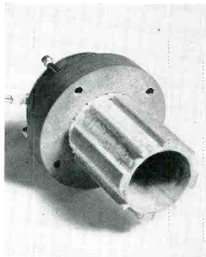
FIG. 11—Winding form for a slotted yoke
