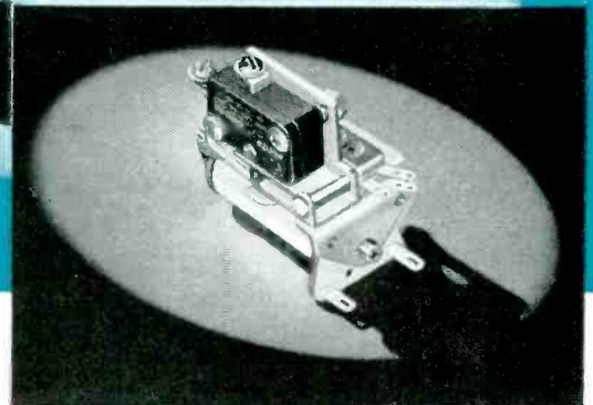
Showing mounting of snap-action switch on CLARE Type "JMS" Relay with single armature.
