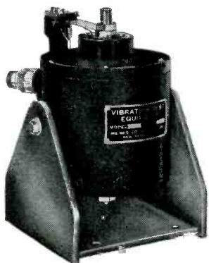
MODEL SA VIBRATION EXCITER Delivers 3 pounds force from 20 to 1,000 c.p.s., usable to 20,000 c.p.s.
