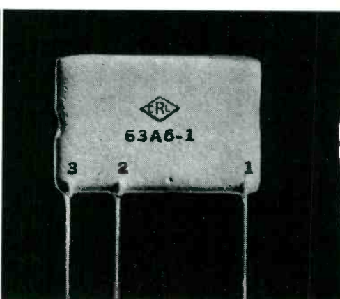
11 This is the new CRL Vertical Integrator Network used in TV sets. Variations of this Centralab Network are available on special order.
