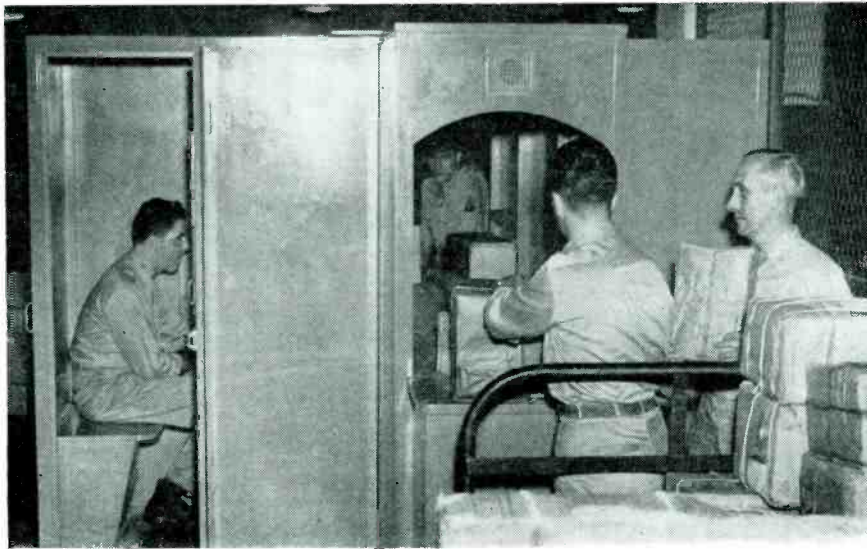
Fig. 1—Military mail clerks at the right are placing packages from soldiers abroad into the examining bay of the Inspectoscope which x-rays them for illegal objects
