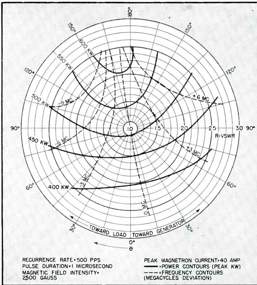
FIG. 3—Rieke diagram of the 4139 megawatt tube, a contour diagram showing the output frequency and power level as functions of the standing wave ratio and position of the voltage minimum along the attached transmission line or waveguide
