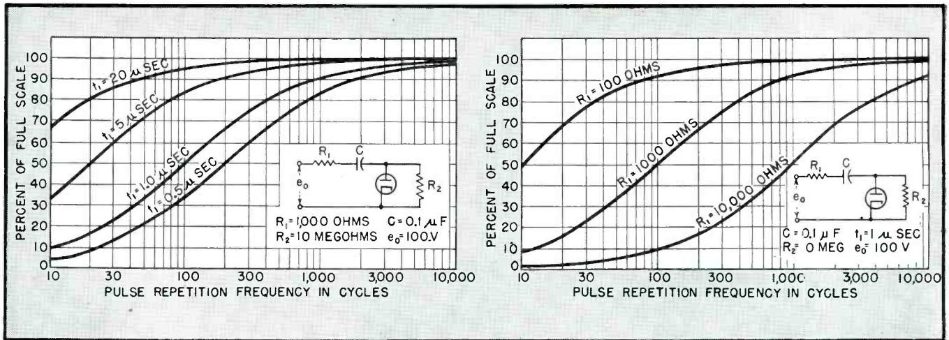
FIG. 3—Effect of pulse width on meter indication
