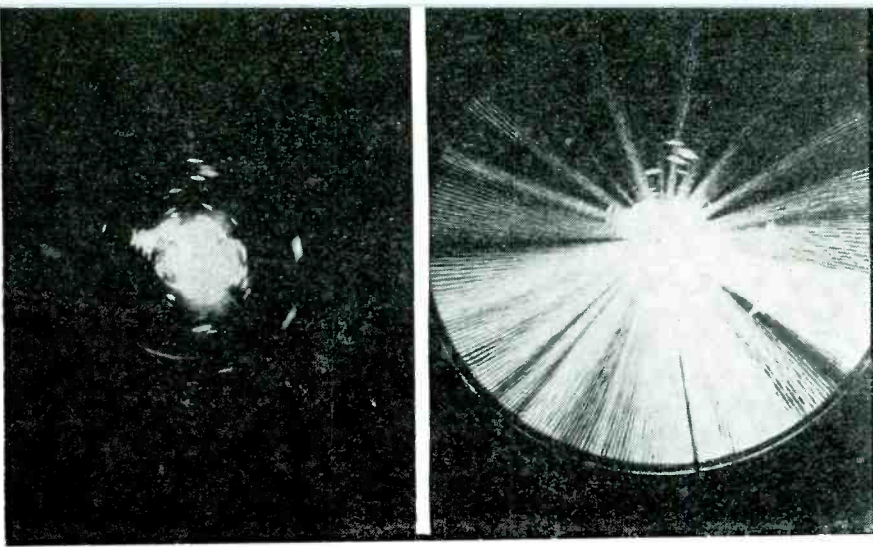
Effect of electronic jamming on plan position indicator (ppi). Left, normal indication. Right, radial traces, brightened by jamming signal, obscure echo signals
