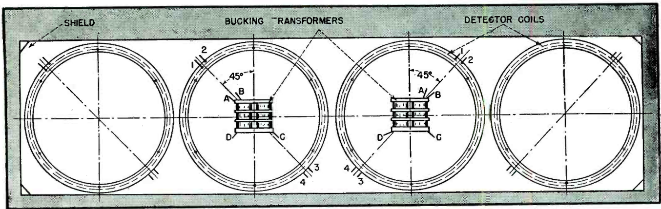
FIG. 3—The arrangement inside the coil box
