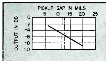
FIG. 11— Decibel output from the pickup is nearly a linear function of gap width
