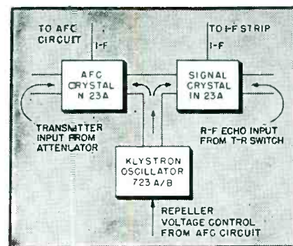
FIG. 8—The afc crystal employs a minute portion of the transmitter signal to operate the frequency control. A separate crystal develops the echo signal intermediate frequency
