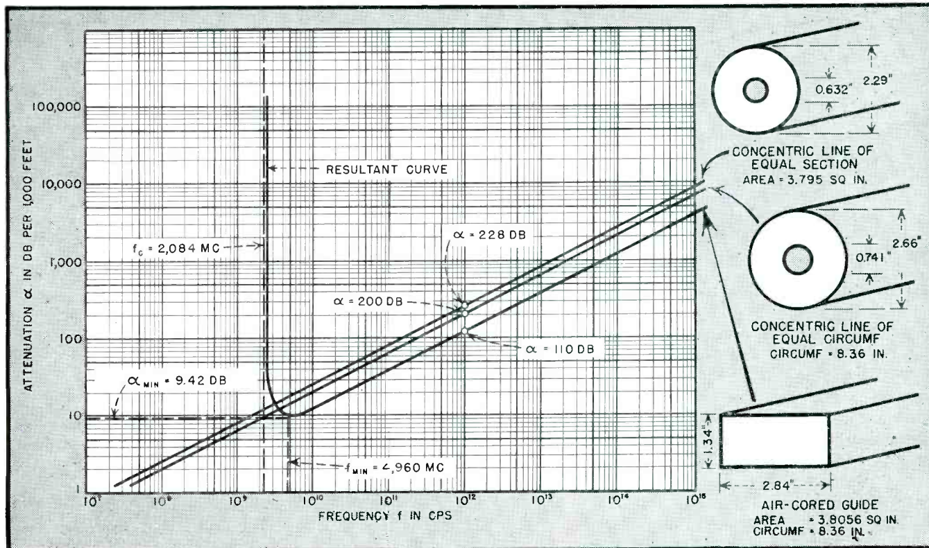
FIG. 2—Graphical construction of attenuation curve for 1.34 by 2.84-inch rectangular waveguide, and corresponding curves for two types of concentric lines
