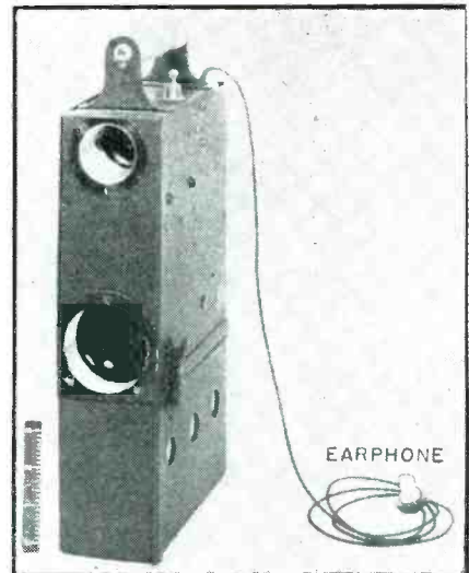
Experimental model of the sensory aid for the blind developed at the Signal Corps Engineering Laboratories
