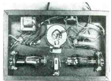
Fig. 6—Mechanical arrangement of tube and components in the balanced bridge circuit. The a-c blocking potential is applied to the slotted plate mounted on a standoff insulator
