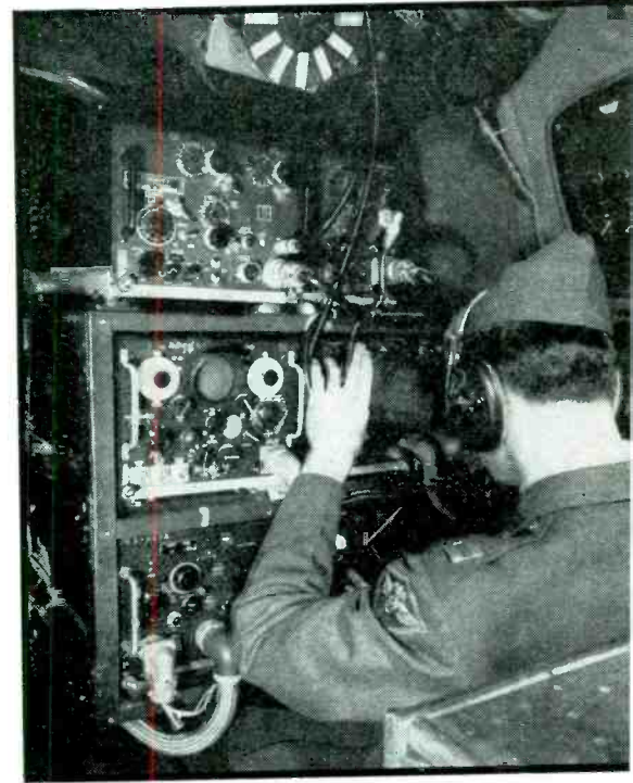
Search and jamming equipment on a Navy rcm plane: from top to bottom: antenna selector switch, APT-1 electronic jammer, panoramic adapter (to sweep receiver frequency) pulse analyzer, cathode-ray d-f indicator (in use by operator), second jamming transmitter, and search receiver (hidden by operator)
