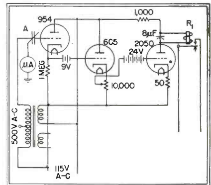
Fig. 3—Improved stability resulted when the three-plate capacitor shown at A was used in this control circuit
