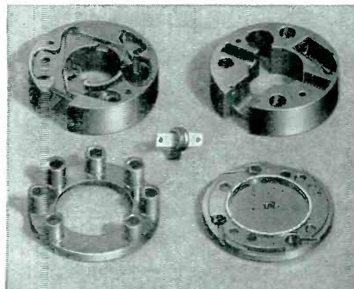
These small but highly intricate plastic pieces are vital parts of the new famous VT fuse.
