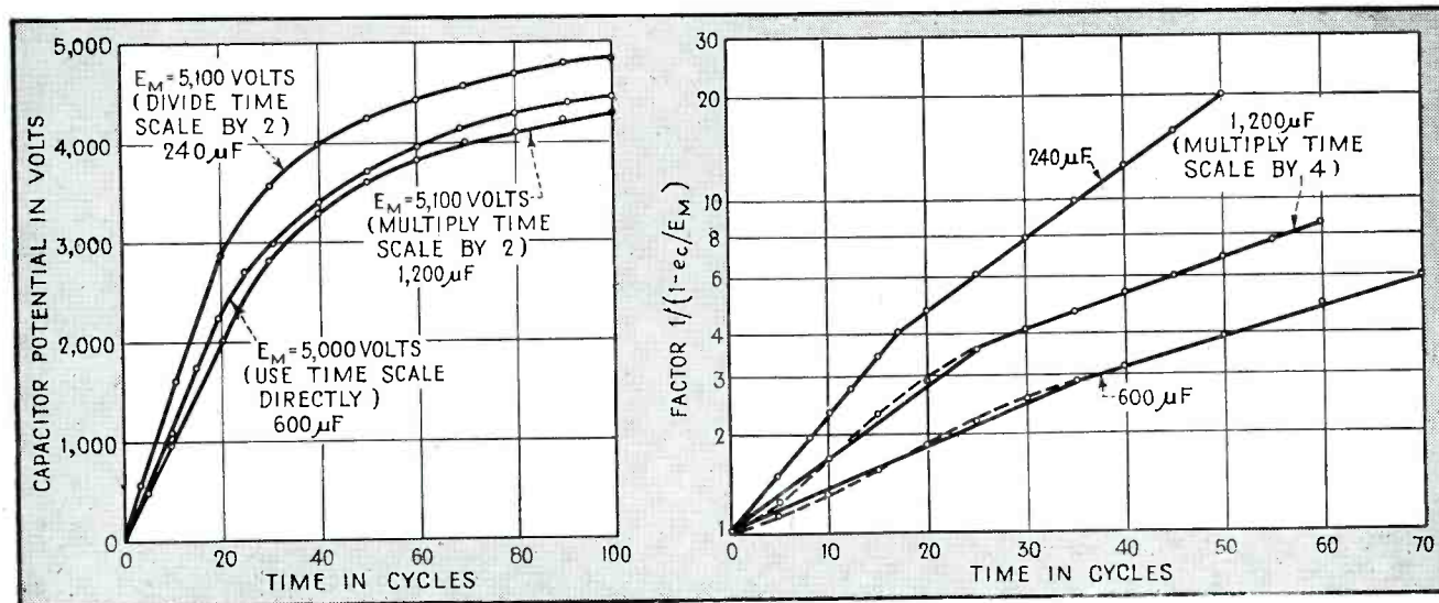
FIG. 4—Logarithmic plot shows that capacitors charge first at a fast rate, then change abruptly to a slow rate
