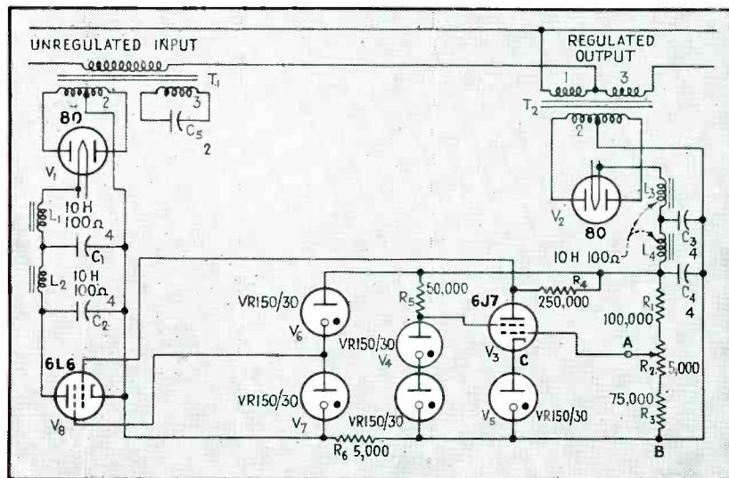
FIG. 2—Circuit diagram, with values of components. Transformers T_1 and T_2 are ordinary radio receiver power types. With the regulator, voltage changes at the output are only 6 percent of line voltage changes at the input
