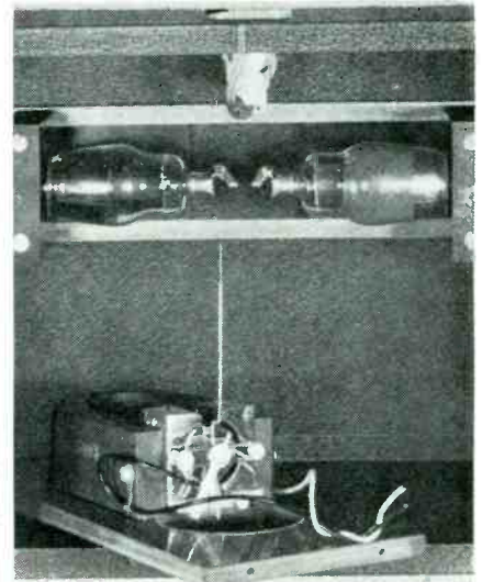
Fig. 7—In the final version, the tubes were mounted on a track and the meter movement made rotatable so that stray capacitance effects could be compensated
