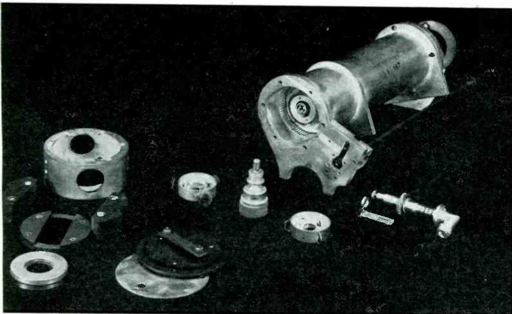
Oscillator of APT-9 jamming transmitter, using disk-seal tube. This oscillator covers the enormous range of 300 to 2500 mc with a power output of 10 to 25 watts, continuous wave
