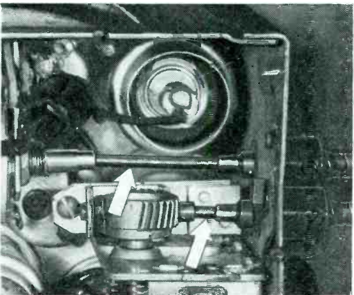
Coupling external control shafts to tuning elements—as in this radio receiver—damps noise-causing vibration, eliminates need for precise mounting and alignment of tuning elements—also gives complete freedom in their location.
