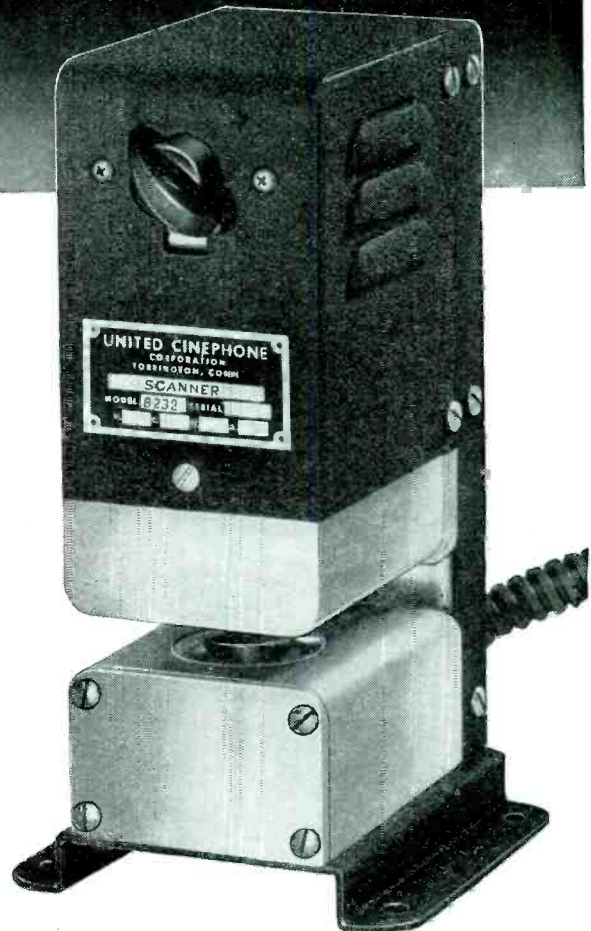
SCANNER MODEL No. 8232 Approximate size: 7½" x 4" x 3¾"
