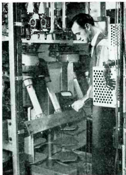
Power tubes and tuning capacitor of the 125,000-watt electronic vulcanization unit installed at the Firestone plant in Fall River, Mass.
