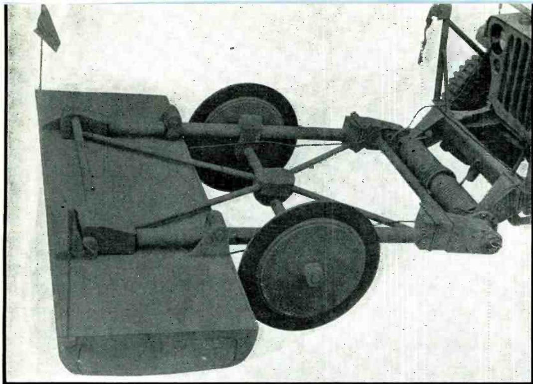
FIG. 1—The vehicular-mounted mine detector with boom lowered
