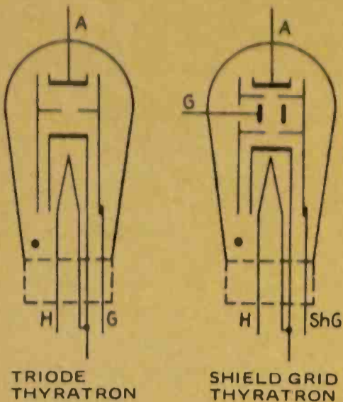
Fig. 12 Internal construction of triode and tetrode thyratrons.
