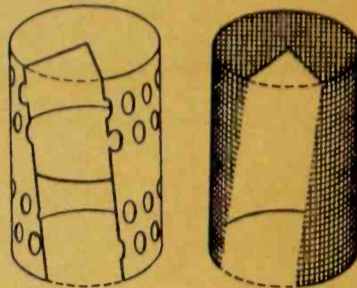
Fig. 12 Internal construction of triode and tetrode thyratrons.
