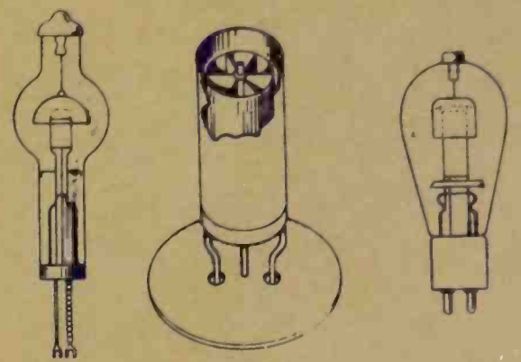
MERCURY-VAPOR TUBES WITH HEATER DETAILS
