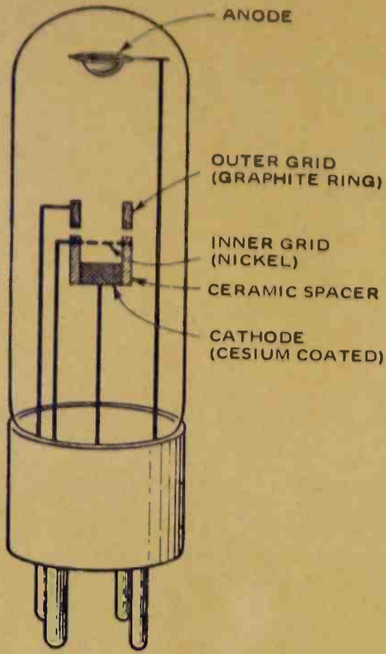
Fig. 23 Structure of the strobotron tube.
