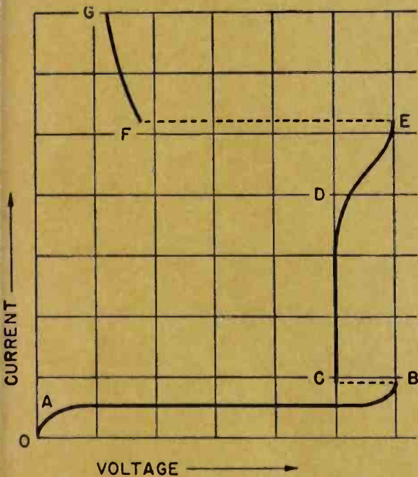
Fig. 19 Voltage-current characteristic of a neon tube.
