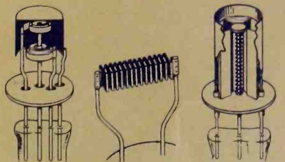
HOT-CATHODE EMITTING STRUCTURES
