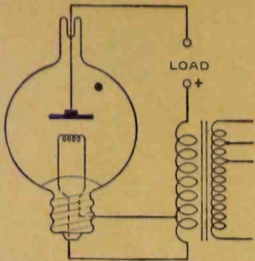
Fig. 10 Plan of a Tungar rectifier bulb.
