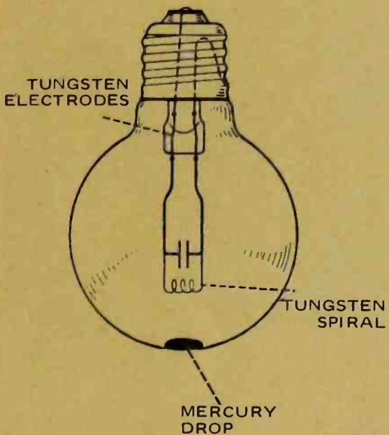
Fig. 6 Plan of a filamentary mercury-vapor lamp.
