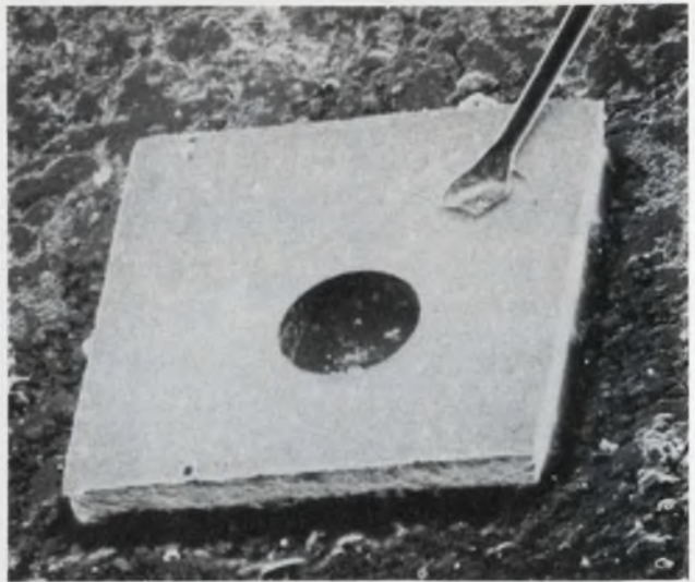
The best emitters for optical communication systems up to 50-Mbits/s are Burrus-type diodes, like this General Telephone and Electronics diode chip.
