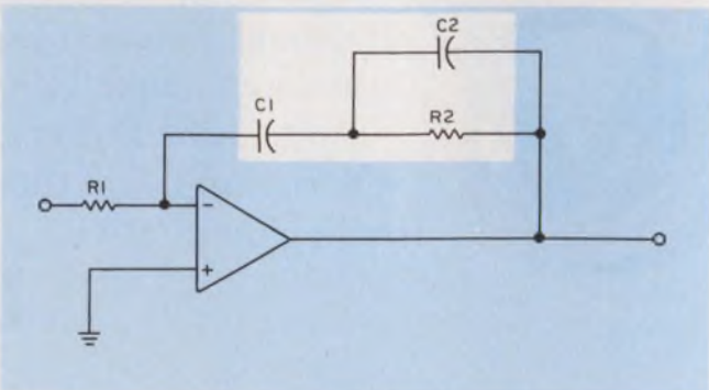
3. An integrator/filter circuit can be built with a wideband op amp and RC feedback network.
