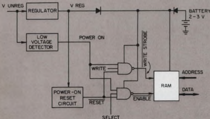
1. A battery-backup RAM circuit has gates that are powered by the battery when +V REG is off. Typical power-on reset circuits generate premature outputs,
