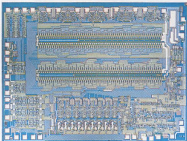
The first single-chip monolithic data-acquisition system, the ADC0816 by National Semiconductor, has an 8-bit a/d, a 16-channel multiplexer and microprocessor-interface logic. It performs a conversion in 50 \mu s.
