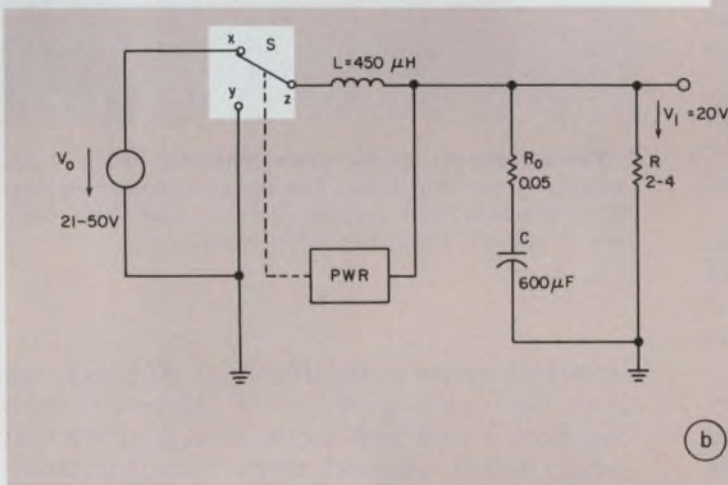
6. Ripple reduction in a down-converter (a) is most effective with the nonlinear sawtooth (1), less so with the linear sawtooth adjusted for best compensation (2), and
