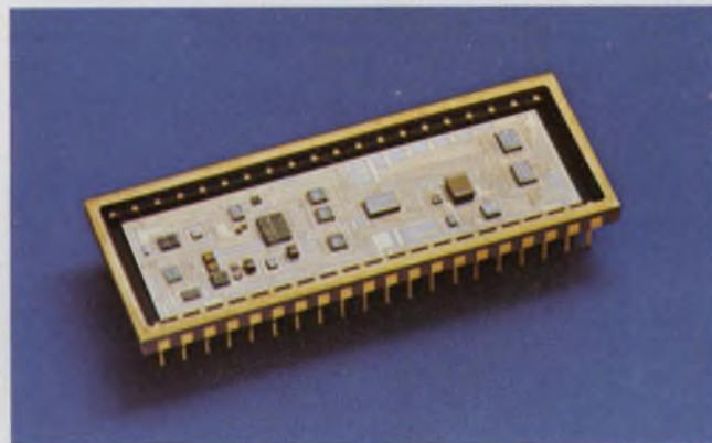
Local control of data acquisition at the sensors is provided by new hybrid components like this d/a microperipheral interface package, the MN5500 by Micro Networks.
