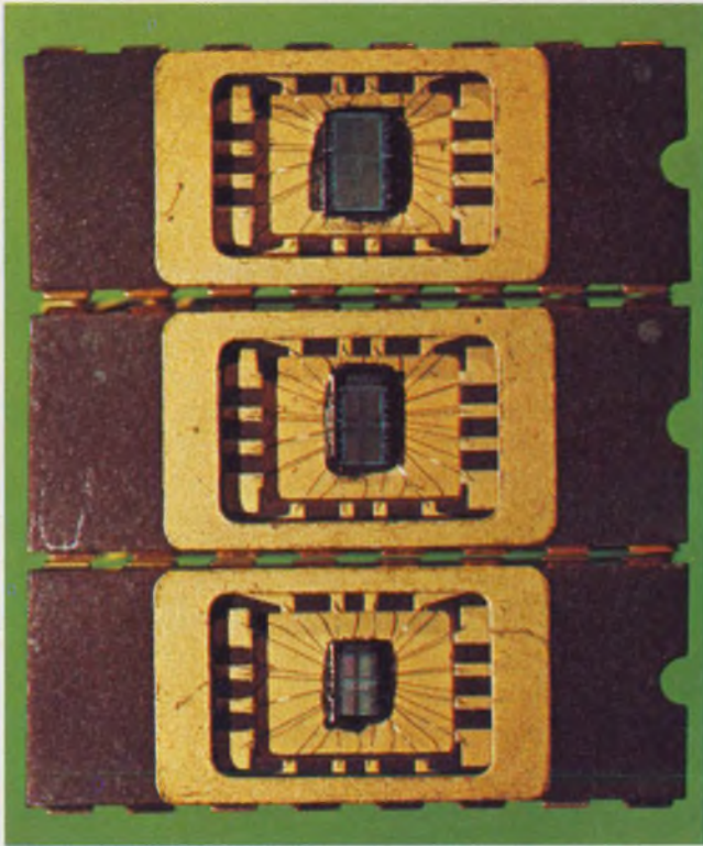
VMOS shrinks static RAMs. These three AMI 1-k static devices went from 100 to 83 to 66 mils on a side, while access times dropped from 45 ns to 35 to 25.
