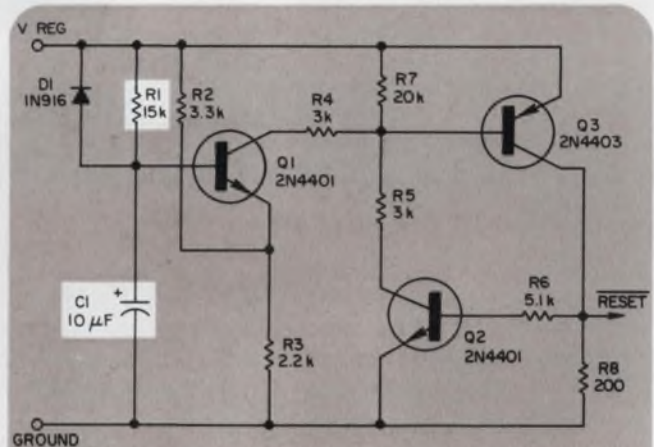
2. This power-on reset circuit has no premature output signal, and its output has a low impedance to ground when no power is applied.
