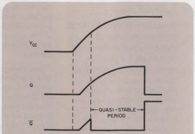
2. A single pulse from the multi's Q output rises with the applied supply voltage. The \bar{Q} output also begins to rise, but reaches only 2.3 V before going low.
