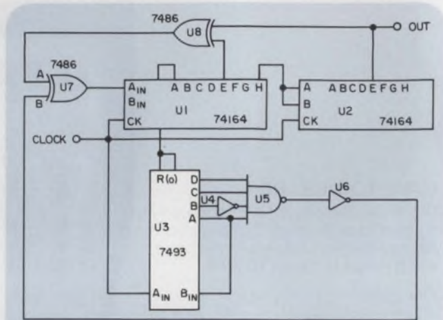
Stop pseudorandom generator interruptions with a binary counter that feeds a logic ONE into the shift register when too many zeros occur.
