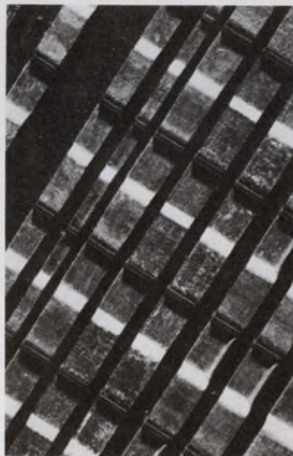
Formed strips of aluminum-magnesium foil, bonded to the platelets and activated after assembly by oxidation, form a layer of magnesium oxide, which is a good secondary emitter.
