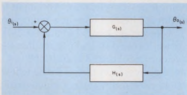
2. The phase-lock loop's generalized open-loop transfer function, G(s)H(s) , has a third-order denominator—from which the circuit's name is derived.
