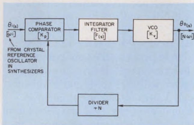
1. A type-2 phase-lock loop has two true integrators—the integrator/filter ( F_s ) and the VCO ( K_v ). Replacing the integrator/filter with a passive-RC network converts the circuit to a type-1 system.
