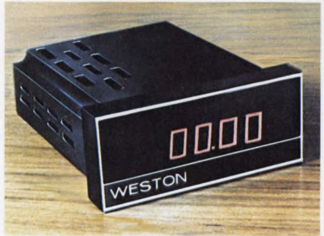
Zero means zero on Weston's 4 1/2-digit Model 2470. The unit has \pm 1 -count stability at zero over a 0 to 50 C operating range, and no dead band at zero.
