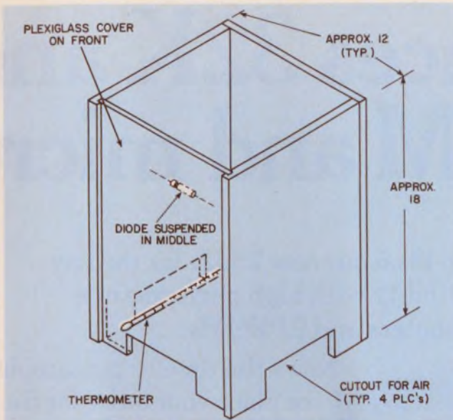
1. A rectifier test chamber for making thermal-impedance measurements in still air suspends the diode in the center and the thermometer beneath.
