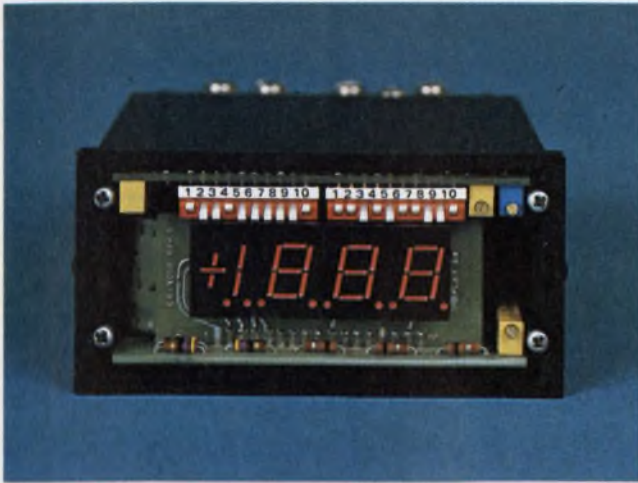
Programming controls, accessible through the front panel, tailor the Analogic AN2573 digital rate indicator. Switches select data averaging and other functions.
