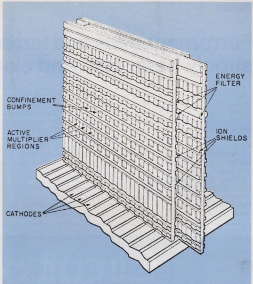
These platelets, or vanes, have confinement bumps to isolate separate picture lines. All electrodes in a column are bused together.
