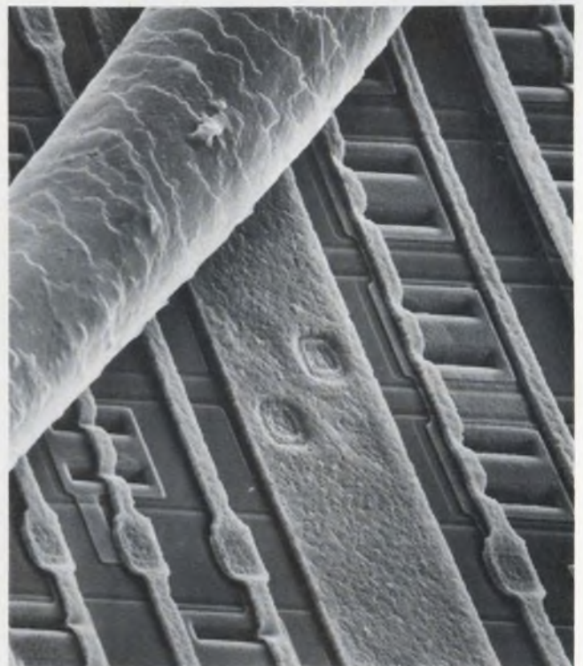
Using three dimensions, VMOS shrinks memory cells until eight fit in the cross-section of a human hair. This photo is a 10,000-time enlargement from AMI.
