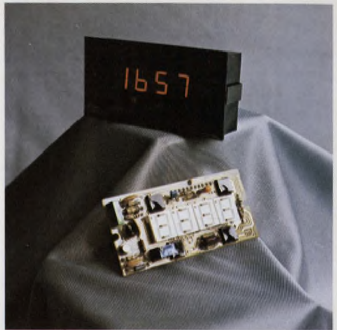
One board holds all in Fairchild's low-cost DPM. Integrated circuits are bonded directly to the board, which also holds discretes and displays. Behind-panel depth is only 3/4 in.
