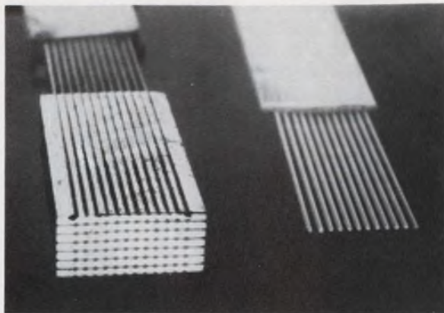
Single and multiple optical fibers can be spliced several ways. Multiple fibers in Bell Telephone ribbon cable are spliced with the fixture shown here.
