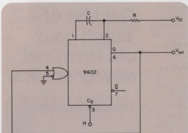
1. This retriggerable multivibrator generates a single pulse whenever V_{cc} comes on. The pulse can be made long enough to reset storage elements in digital circuits.
