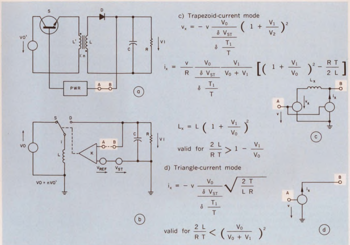
2. An up-converter switching supply (a) relies on the same combination of voltages (b), at K, as the down-converter.
