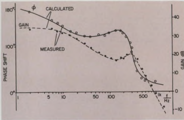
5. Calculated and measured gain and phase-shift values for the down-converter PWR of Fig. 4 correspond closely. The closeness shows that the equivalent circuit indeed represents the actual circuit.
