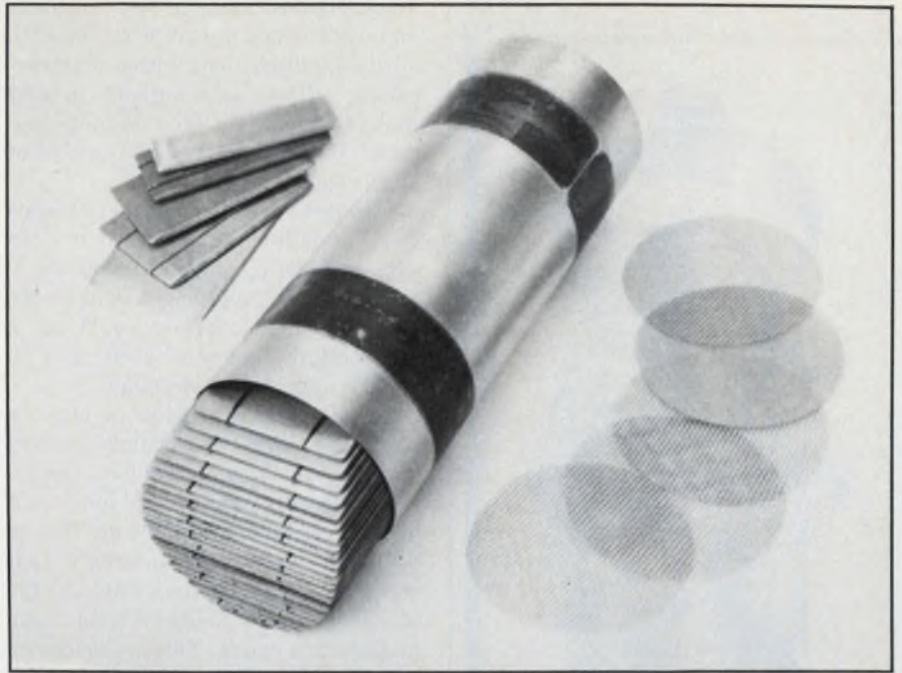
This working element of the magnetic cooling system is a 2-in. stainless-steel cannister containing stacks of 40-mil gadolinium plates. The plates have spaces between them for fluid flow. The wire screens smooth out the flow pattern.
