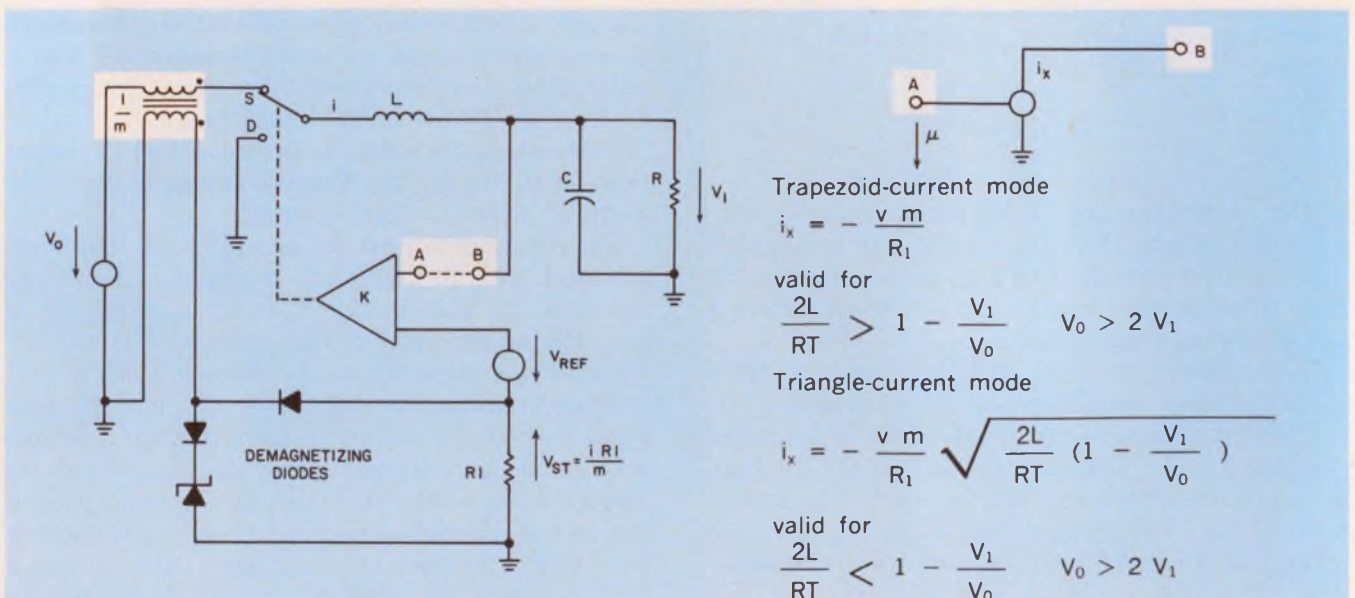
7. This down-converter combines the best features: It operates in the trapezoidal-current mode and acts as a
