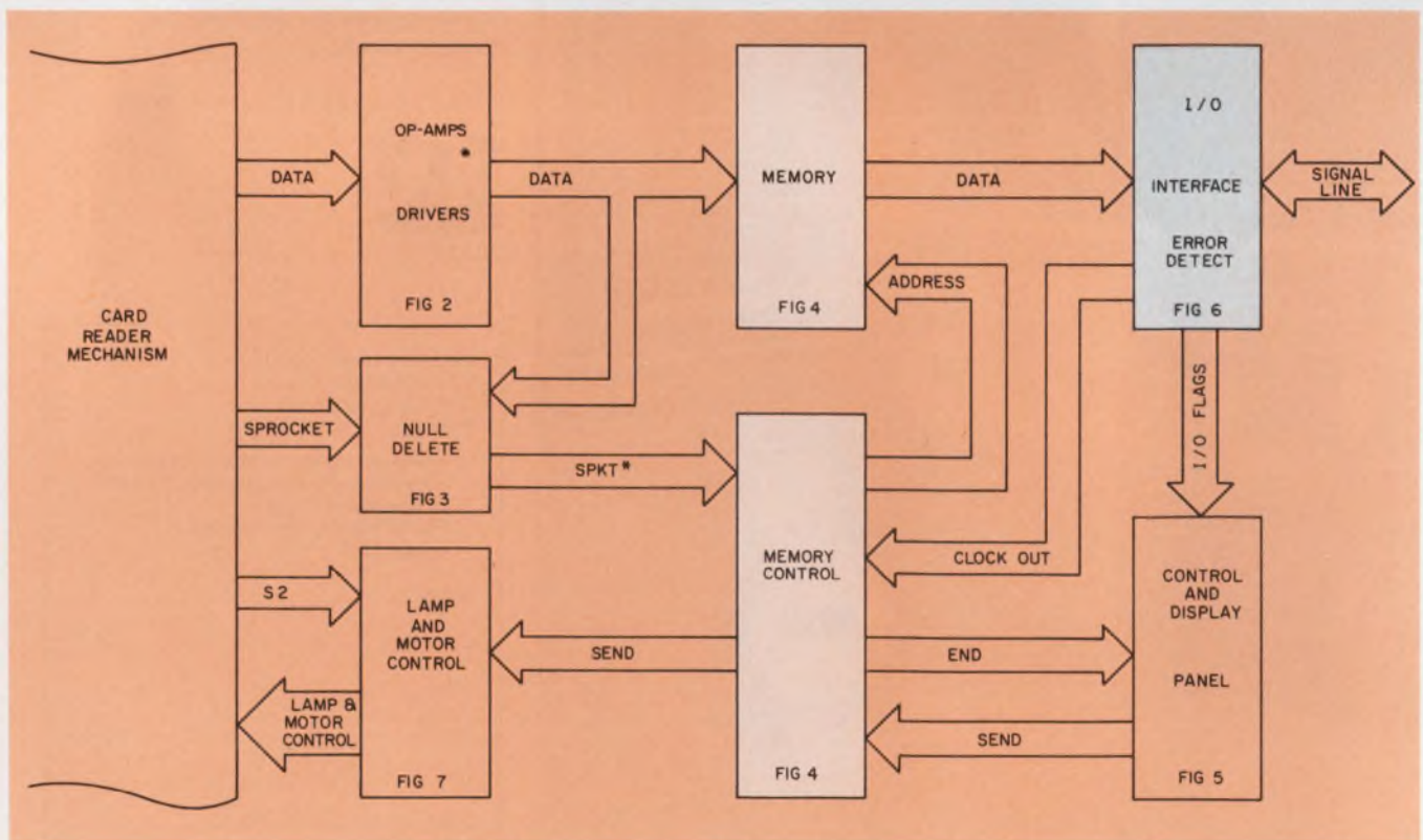
1. Internal memory in a card reader accepts parallel input data, delivers serial data, and simplifies the I/O design.
