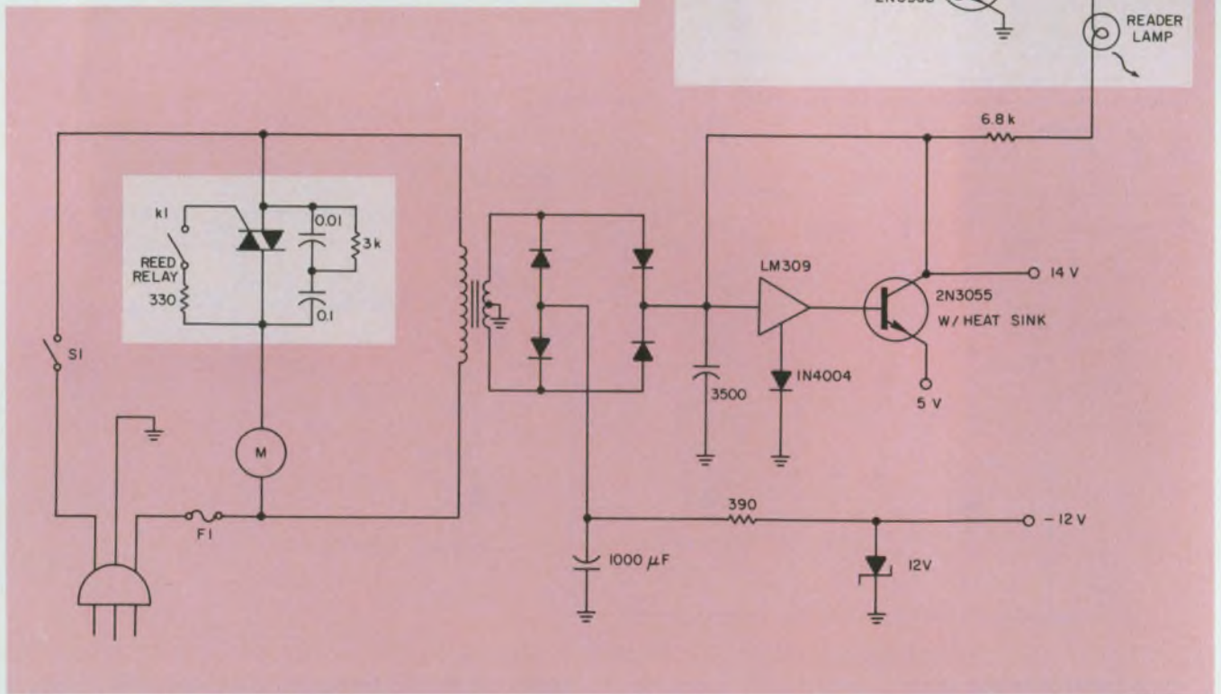
7. Power-supply and motor-control circuits are straightforward. The R-C across the triac suppresses noise.
