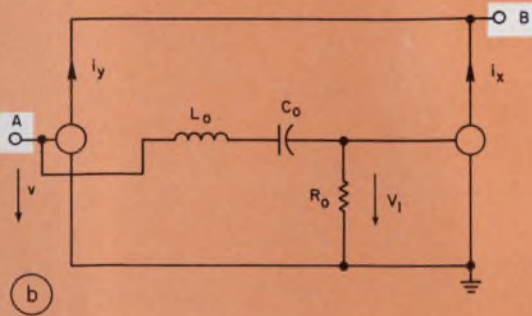
b) Trapezoid-current mode
