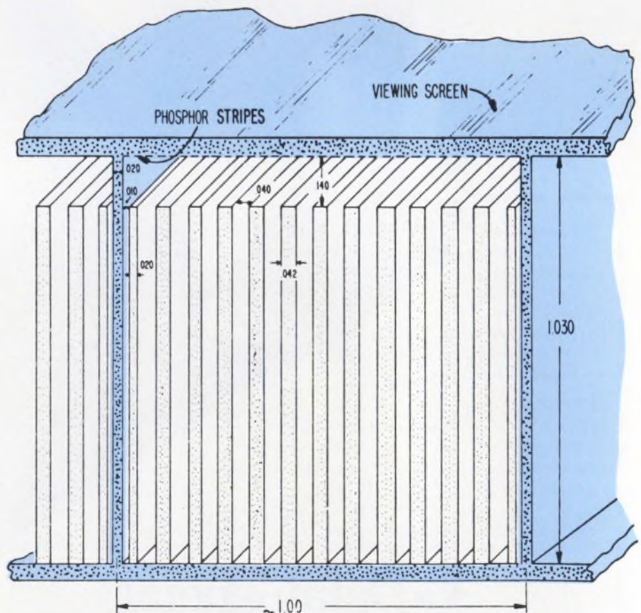
One of 40 display modules is shown in this top view of a display cross-section. Each module consists of 13 platelets, between which 12 columns of feedback-multiplier cells are formed.
