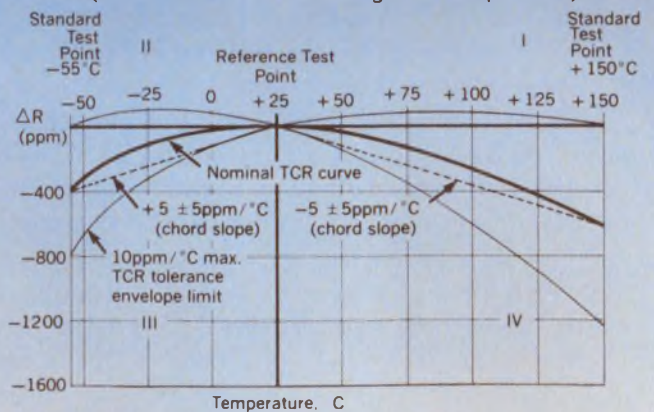
TCR characteristics of Vishay trimmers (End-to-end resistance change with temperature)
