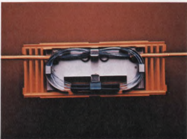
Optical cables are spliced in this field-junction box, by Siecor. The fibers are centered in V-shaped grooves for precise alignment, and bonded together by a quick-set adhesive. A plastic sleeve protects the joint.
