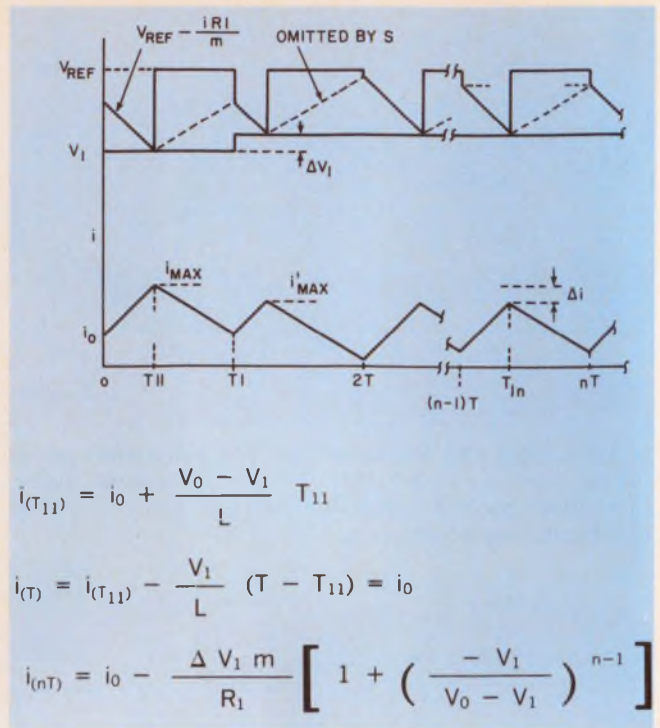
8. Two waveforms for the down-converter of Fig. 7 are plotted on one time scale. The upper trace shows how the comparator-input voltage varies in time. The lower trace shows the inductor-current waveform.
