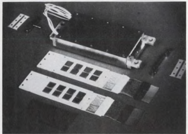
Four PPS-8 \mu Ps control four independent bubble-memory channels in this NASA 102.4-Mbit solid-state recorder, which replaces tape machines. One of the channels is shown here. Total rate for all channels is 2.4 MHz.
