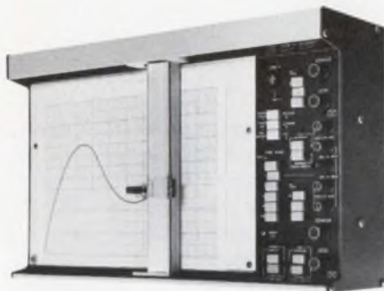
The 7015B lab X-Y recorder is a low cost, open instrument that features maximum electrical and mechanical flexibility to fit many and varied applications.
