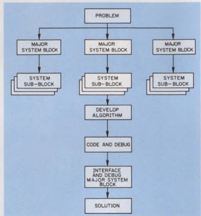
1. In top-down design the complete program is broken down into blocks and sub-blocks that can be coded and tested easily.
