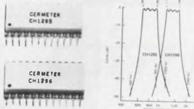
CH1295-1296 Front Frequency Response
