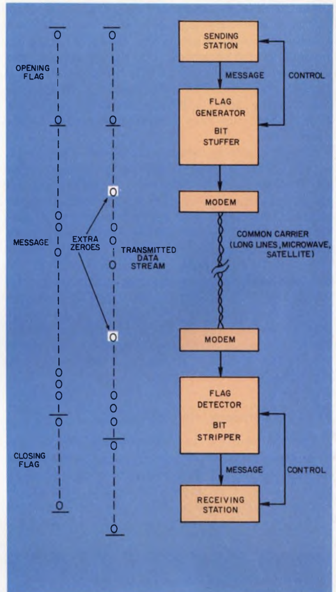
Bit stuffing (and bit stripping) is the key to bit-oriented protocols. A flag generator/bit stuffer is normally part of the computer’s software system, but new protocol chips will make this overhead invisible to processors at both ends of the data-communication link.
