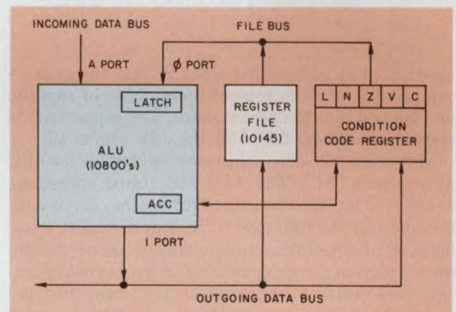
7. The data-processing section of the MOD boards consists of an 8-bit ALU, a 16 x 8 register file and a condition-code register.
