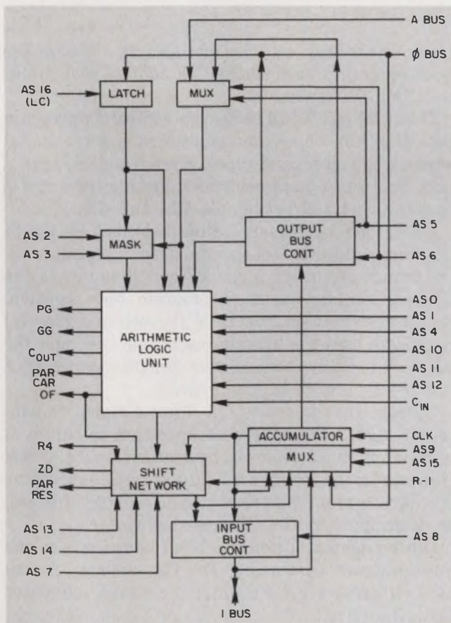
2. Capable of 28 logic and 23 arithmetic operations as well as 16-data-routing options, the M10800 4-bit ALU slice can form the heart of a flexible computer system.
