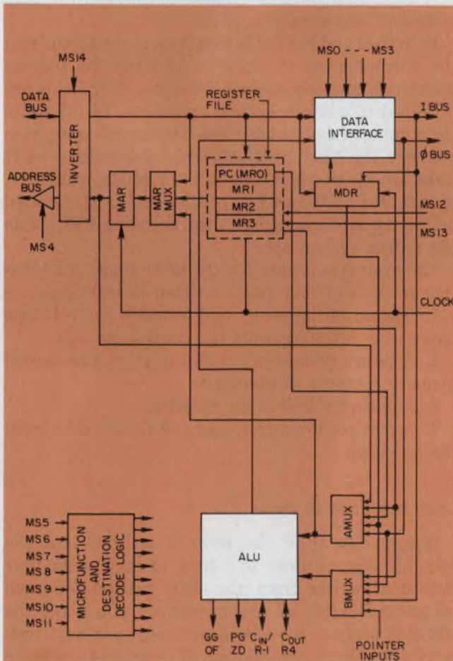
4. Built with five I/O ports, the M10803 memory interface circuit offers very flexible operation along with 17 different data-routing instructions.
