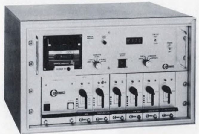
Scan, record and time 16 channels for 240 days with a cassette data-acquisition system from Climatronics.
