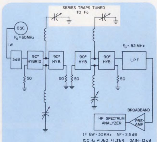
2. A noise measurement setup with carrier-suppression circuits was used to establish that the oscillator noise output is 145 dB below the carrier.
