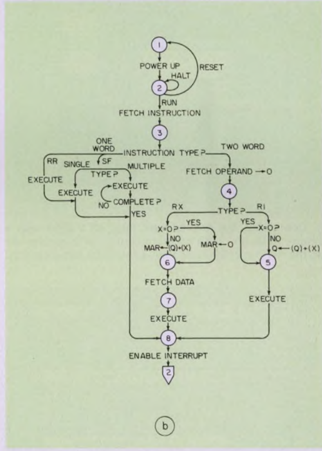
7. Breaking a 16-bit minicomputer into its various function blocks permits you to take advantage of the diverse circuits in the 2900 series (a). Computer operation can be shown very simply if a state-transition diagram is used to map the flow of an instruction.
