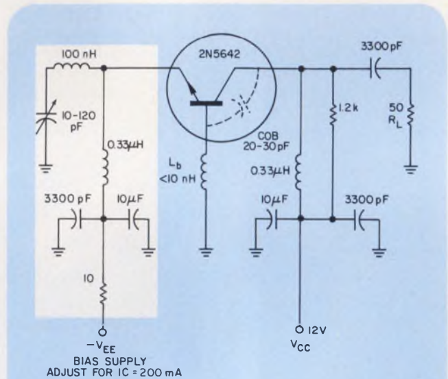
1. High negative feedback in the emitter circuit reduces the noise output of this 1-W power oscillator to very low levels.
