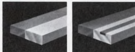
1. Thrulay welded base metals. 2. Thrulay with inlay.
