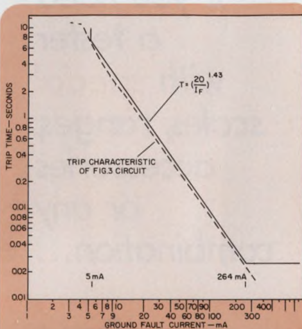
1. UL specs for GFCI systems allow slow response to small currents, but demand very rapid response when the current is substantial.
