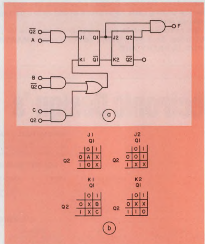
2. The equivalent circuit of the four-state machine (a), as diagrammed in Fig. 1, can be derived by use of Karnaugh maps and J-K flip-flops (b).
