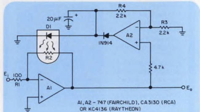
1. The output of the compression amplifier can be set from about 0.2 to 3 V by changing R 3 from 100 Ω to an open circuit.
