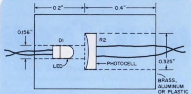
2. A housing for the LED/photocell assembly can be made from almost any material, but it must be light tight.
