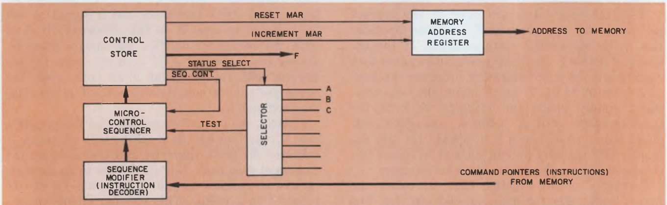
5. Accessing commands stored in a large memory becomes simple when the memory-address register is
