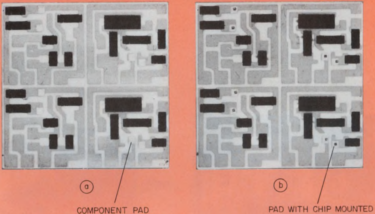
4. Printed epoxy pads (a) must be large enough to allow room for component positioning tolerances (b).
