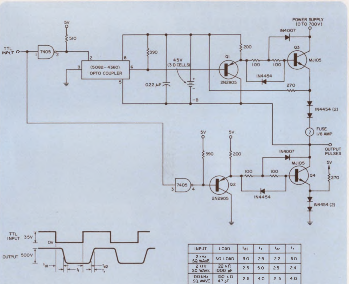
High-voltage pulse amplifier uses an optocoupler to enable TTL levels to control greater than 500 V
