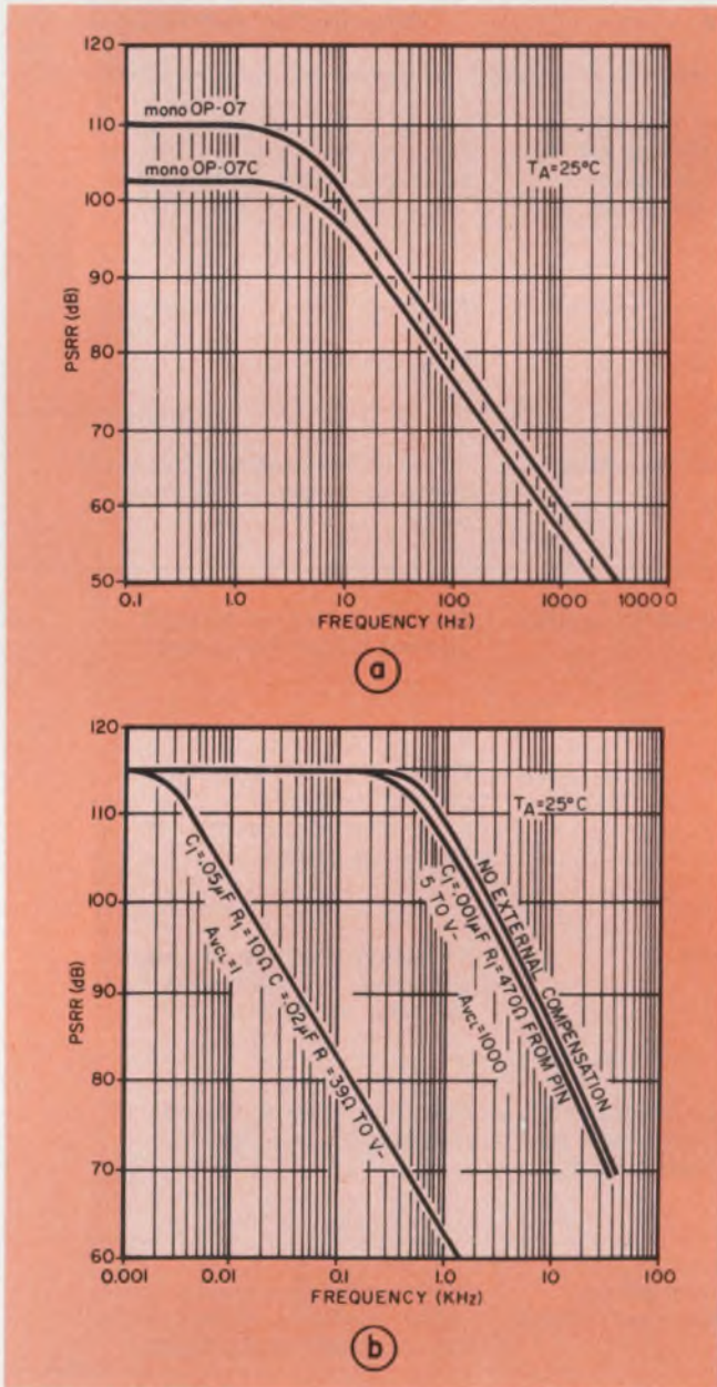
3. Power-supply noise rejection decreases as ripple frequency increases for all op amps. Internally compensated op amps have low PSRRs (a) compared with externally compensated op amps (b) when the externally compensated units are connected for high closed-loop gain applications.
