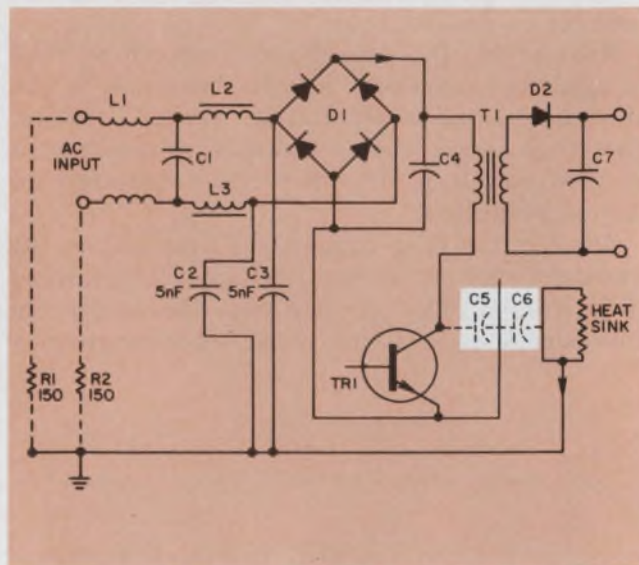
4. Collector-to-heat-sink capacitance is a source of interference currents. One way to minimize the problem is to place a screen between the sink and transistor.
