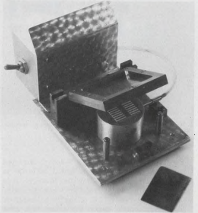
3. Epoxy mounting pads can be applied by printing. This hand printer uses an etched-foil screen, but automated printers and wire-mesh screens can be used.
