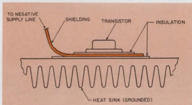
5. Shielding construction needed to reduce an output transistor's capacitance to ground. Each supply has its own optimum arrangement.
