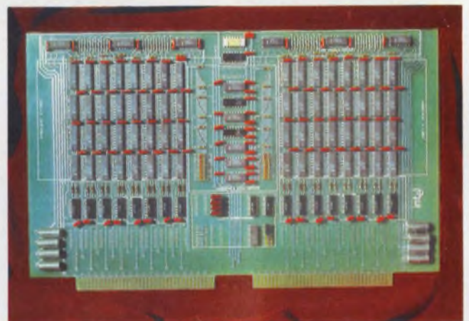
16-k bit CCD memory chips—Intel's 2416—are the main element of a 1-Mbit prototype board. Of all the packages, 30% provide support circuits.
