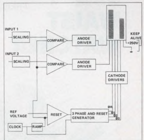
This block diagram for a dual linear bar graph shows you how simple the operation really is.
