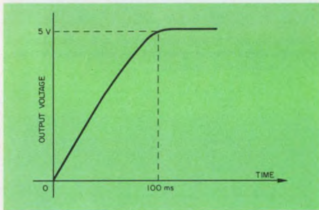
6. Output voltage is "delayed" by limiting of the thermistors until all bias and drive signals are established. Normal operation then begins.
