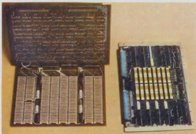
Memory boards employ 512-bit CMOS static RAMs —American Microsystems' S2222. The boards are used in Rolm's Rugged Nova system.
