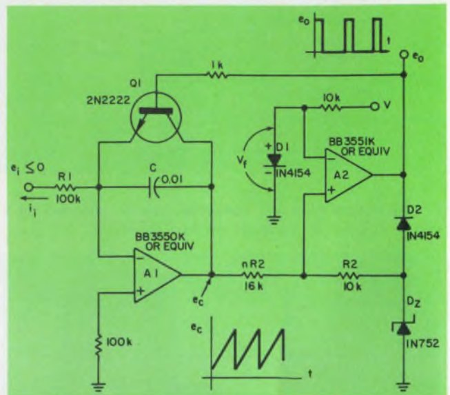
3. Higher precision ( 0.1\% ) v/f converters use a comparator-controlled reset circuit.
