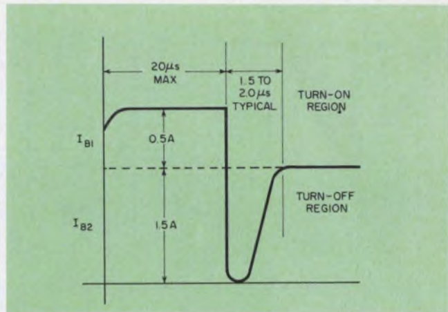
8. Critical to proper operation is the Darlington base-drive current, which must have fast transitions.
