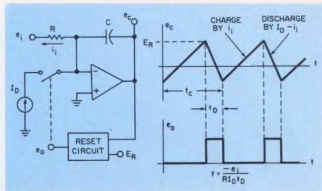
4. Controlled-charge reset circuits eliminate the linearity error caused by a separate reset interval.
