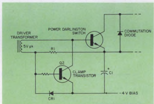
9. Turn-off current, I_{B2} , is provided by a transistor clamp arrangement at the base of the Darlington.
