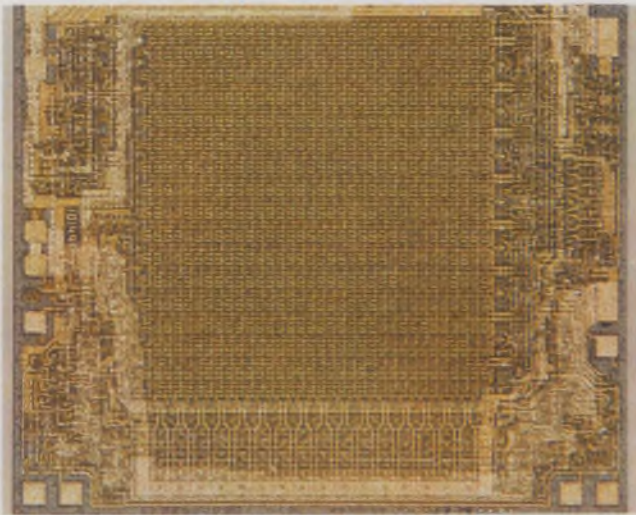
The largest ECL-10,000 PROM —Motorola's MCM 10149—has 256 \times 4 -bit organization and maximum access of 25 ns. The bipolar PROM employs fusible links.
