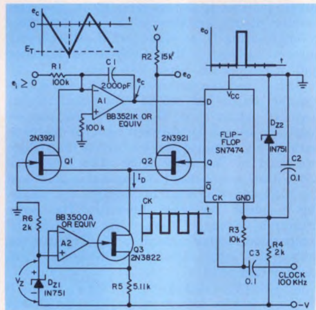
6. If clocked control of the discharge time is used, accuracies to within 0.01% are obtainable.
