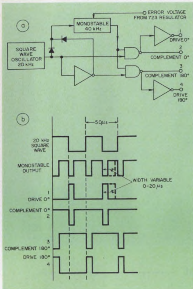
7. To derive the four signals to drive the Darlington bridge, the one-shot output is "mixed" with the 20-kHz clock in two NAND gates (a). The resulting waveforms consist of two out-of-phase signals and their complements (b).
