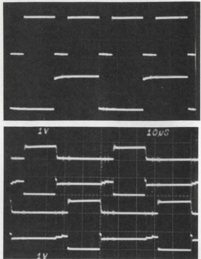
Signal and phase relationships (top to bottom): DM8601, MC4024 and DM 8090 outputs at full load, nominal line.
