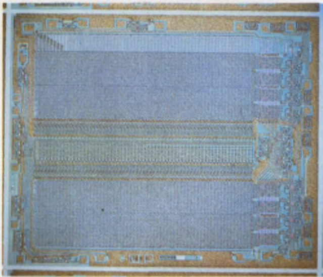
Bipolar PROMs reach 4-k bit densities. Here is Monolithic Memories' 5340, the first 4-k bipolar PROM. The IC has a typical programming time of 5 ms/bit.
