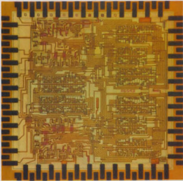
Random logic I 2 L array fabricated by Bell Laboratories has the equivalent of 256 gates on it.
