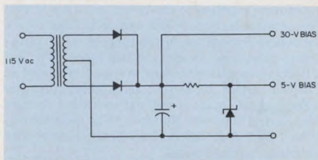
11. Bias power for the TTL and driver circuitry is provided by a simple auxiliary supply.
