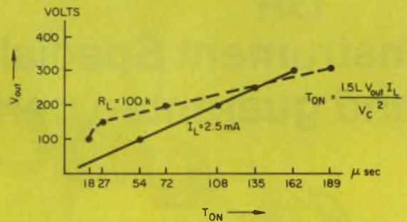
Output voltage of a regulated high-voltage power supply is controlled by variable-resistor R_1 .
