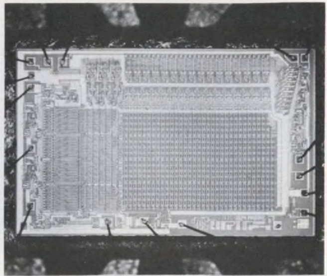
A field-programmable ROM from Harris Semiconductor, the company that introduced PROMs, has a 1024-bit capacity. The PROM features access time of 50 ns.
