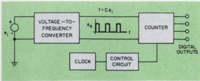
1. The output of a v/f converter can be encoded by a digital counter to simulate an a/d converter.
