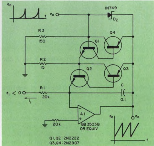
2. A low-precision (0.4%) v/f converter uses an integrator and a voltage-sensing reset switch.
