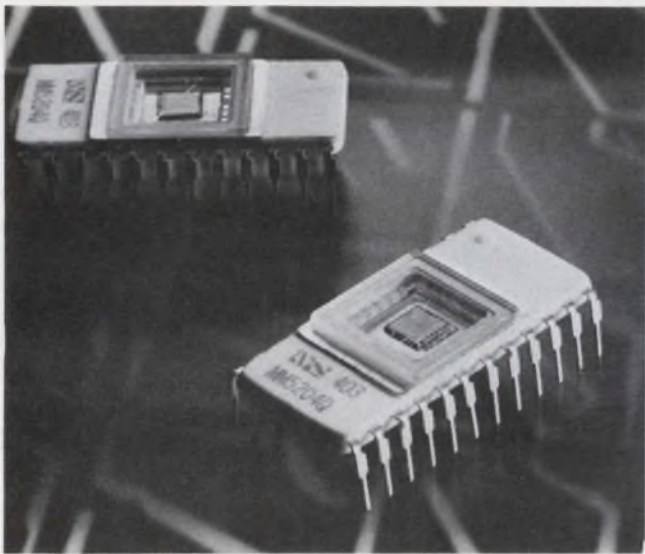
The storage capacity of ultraviolet erasable PROMs reaches 4-k bits with the MM5204 from National Semiconductor. The listed programming time is 30 sec.
