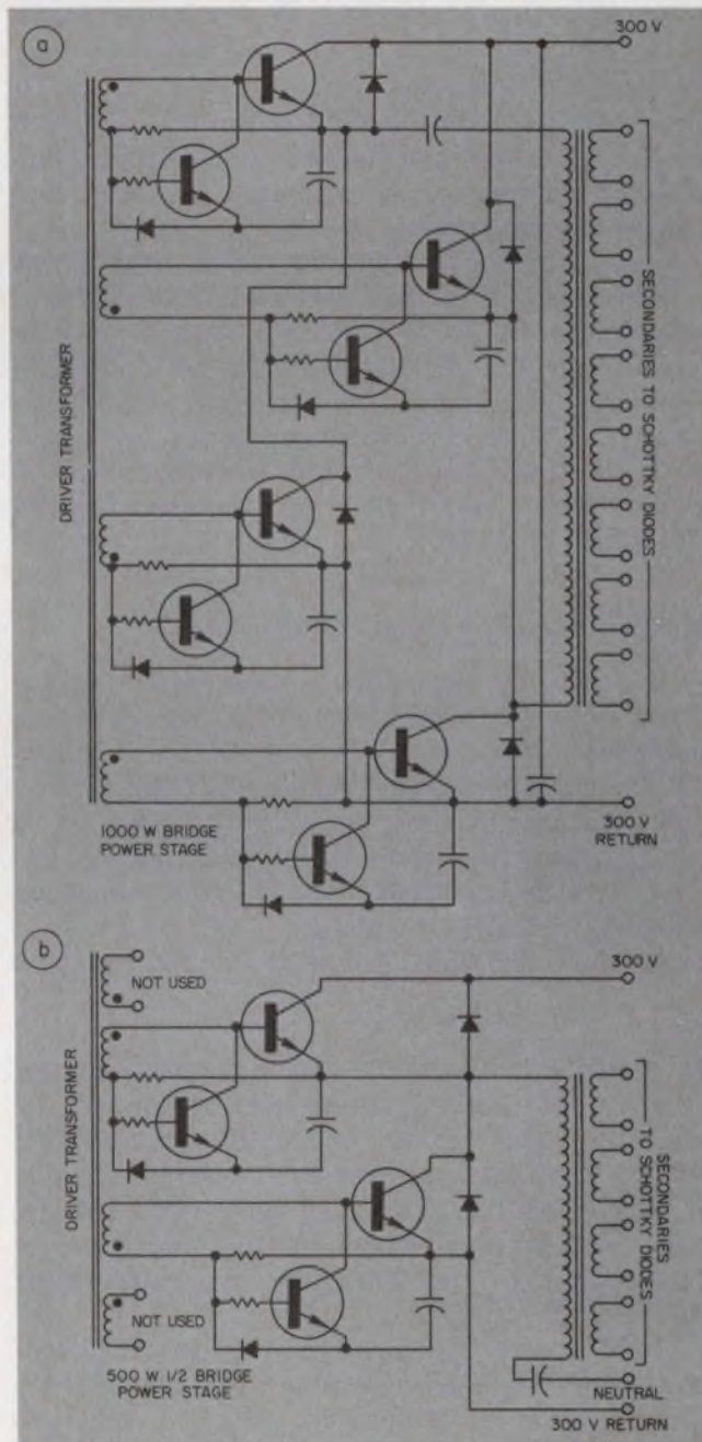
12. Power stage for a 1000-W output (a). Commutating diodes and other circuitry shunt the output-transformer inductive currents to ensure proper turn-off. If only 500 W are needed, a half-bridge connection can be used (b).
