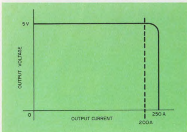
5. Regulation provides a constant-voltage output up to the overload point (250 A) and then goes into a constant-current mode to 0 V.
