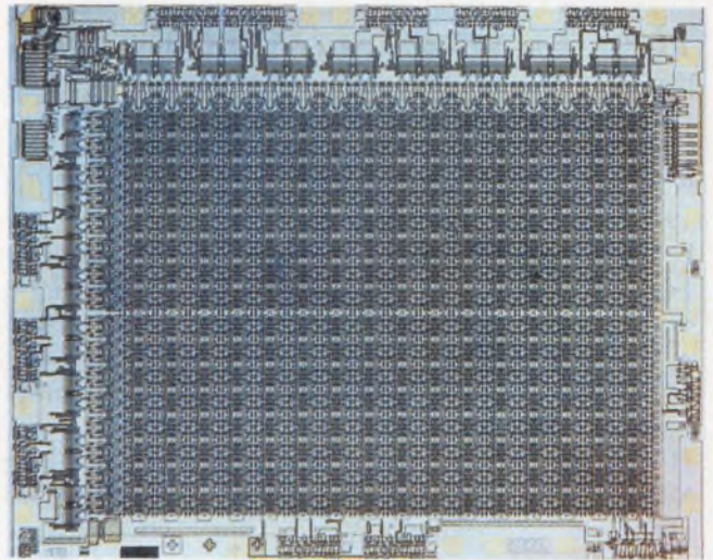
A 1024-bit CMOS static RAM, Intersil's IM6508, offers 250-ns access time over the full temperature range with a 5-V supply. Access drops to 100 ns at 10 V.
