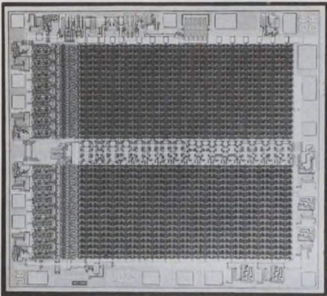
One of the most popular memories is the 2102, introduced by Intel. The 1-k NMOS static RAM can be used as a direct replacement for comparable bipolar ICs.
