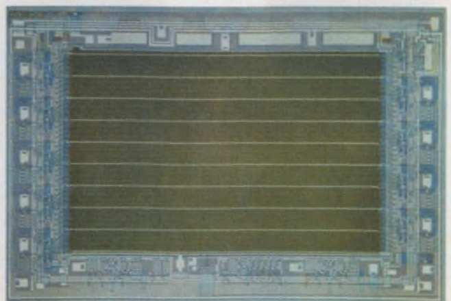
The first CCD memory chip —Fairchild's 9-k-bit circuit—employs nine 1024-bit registers that are shifted in parallel. The operating frequency is specified at 3 MHz.
