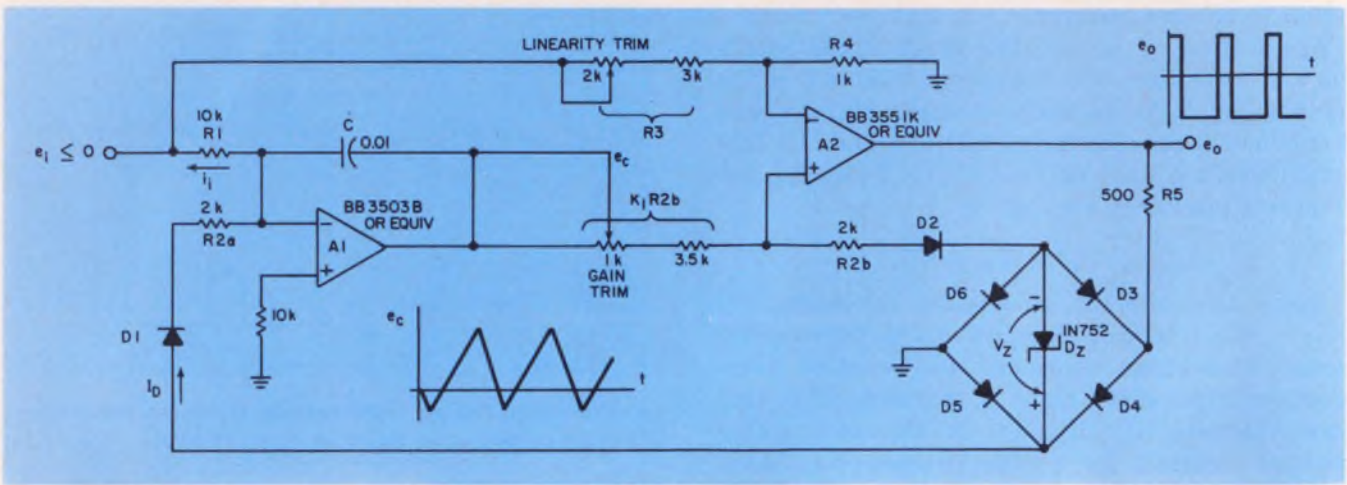
5. A 10,000:1 dynamic range and accuracy of 0.04% are obtained when controlled-charge reset is used.
