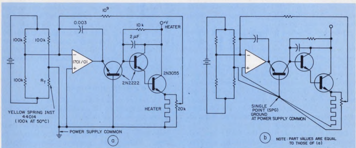
2. A precision temperature-control circuit that has ground problems (a) uses a chopper-stabilized amplifier to provide microdegree accuracy over a predetermined
