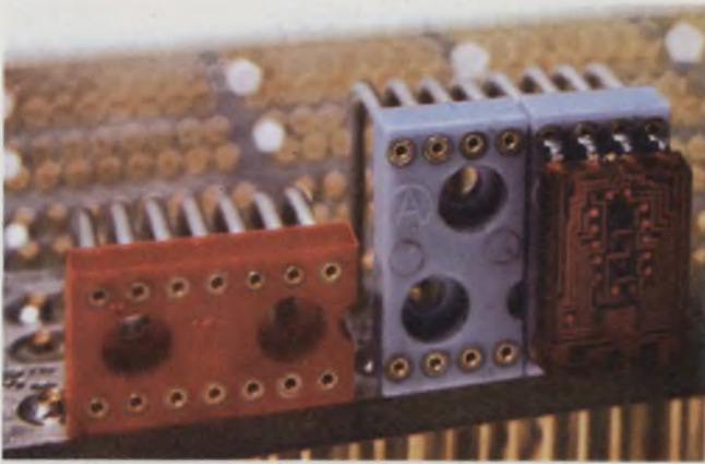
Sockets for LED displays handle practically any pattern, including different row spaces. The Augat units mount at right angles to the PC board.
