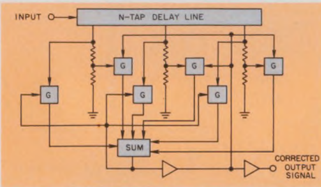
5. An adaptive transversal filter is needed for 4800-bit/s transmission. Additional circuits (not shown) set the tap gains by cross-correlation of the median channel characteristics with symbol error. This algorithm minimizes the combined effects of noise and intersymbol interference of the channel.
