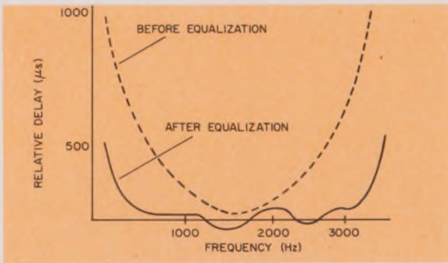
4. Factory-set equalizers cannot compensate for line characteristics over the full frequency range of the modulated signal. Delay ripple remains. Such equalization is useful, however, up to 2400-bit/s.
