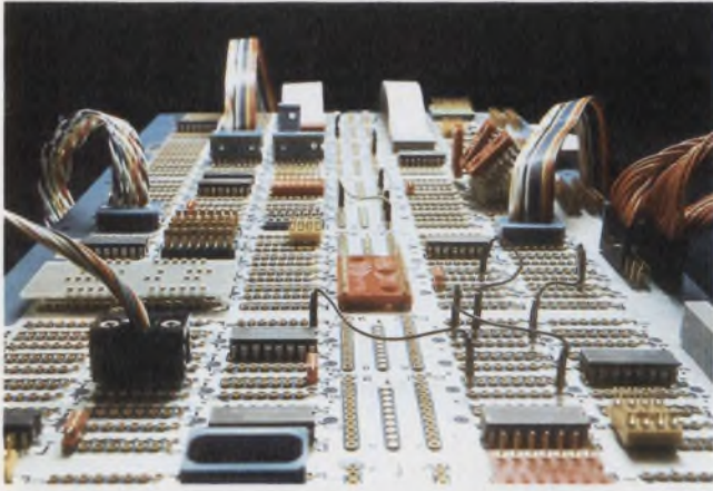
A new ECL packaging board offers pluggable terminating components (left). A single in-line package (SIP) holds the components and is plugged-in between the ICs. Like
