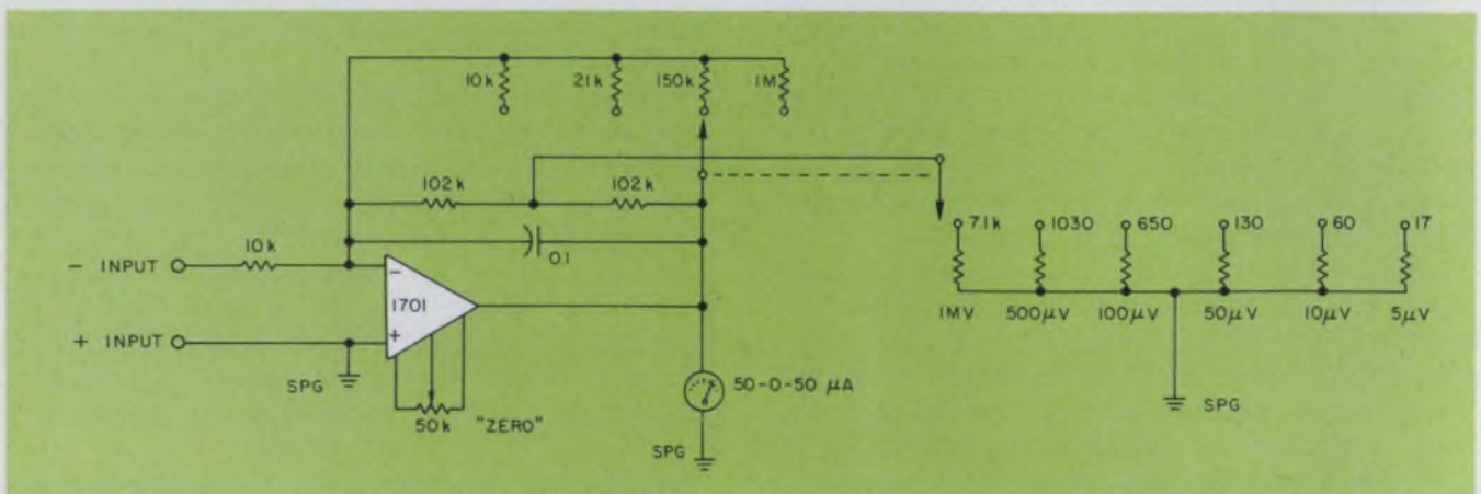
6. Band-limiting of a null voltmeter is easily accomplished if a 0.1- \mu F capacitor is placed across the input and
