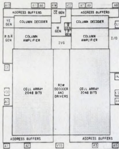
The newest standard in semiconductor memories is the 4-k, n-channel RAM. Intel's 2107 is shown here.
