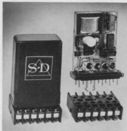
4-pole solid-state relay from Struthers-Dunn uses both photoisolation and transformer isolation.
