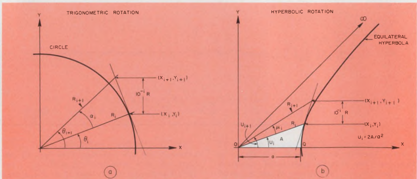
1. Although the geometry of trigonometric functions is based on the characteristics of a circle (a) and hyper-
