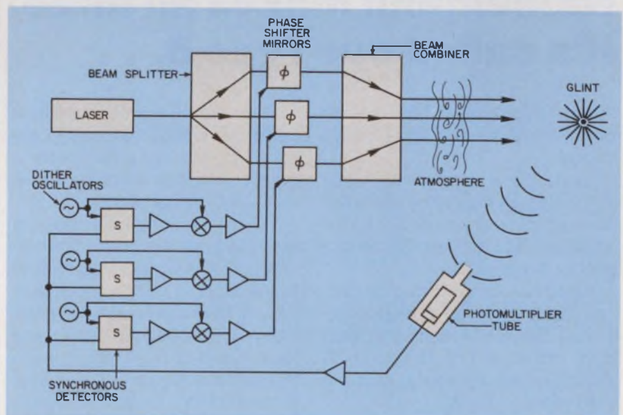
Experimental "ladar" system with a three-element array incorporates the Coherent Optical Adaptive Technique to maintain its effective beamwidth. This system has operated over a 100-meter turbulent airpath.
