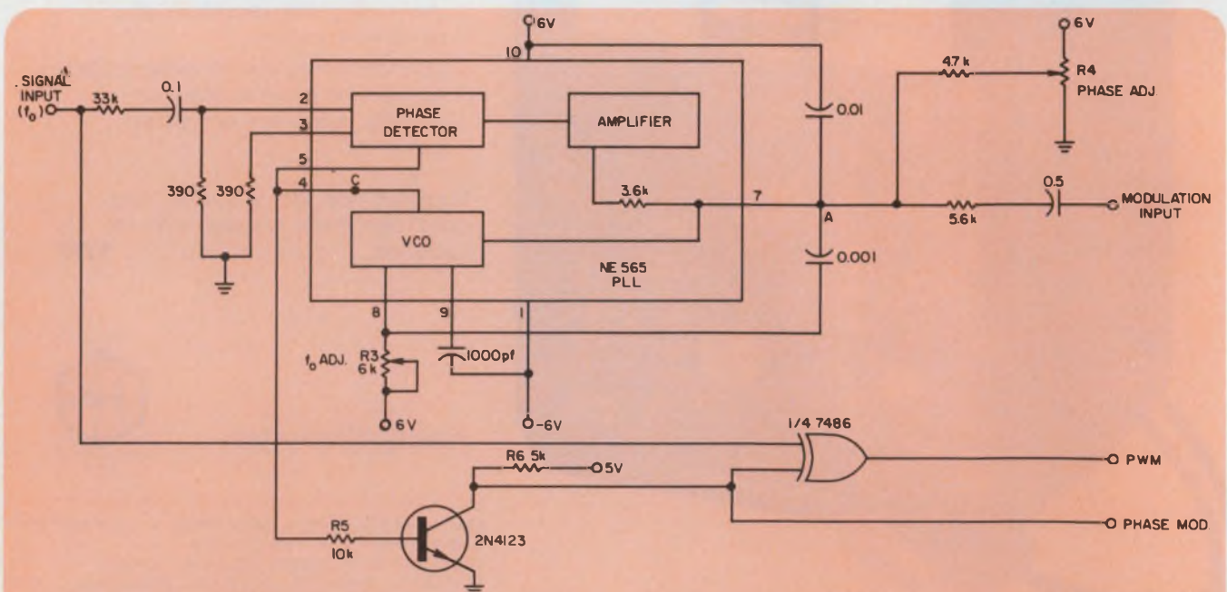
Offsetting the PLL voltage-loop with a modulating signal phase-modulates the VCO output (point C).
