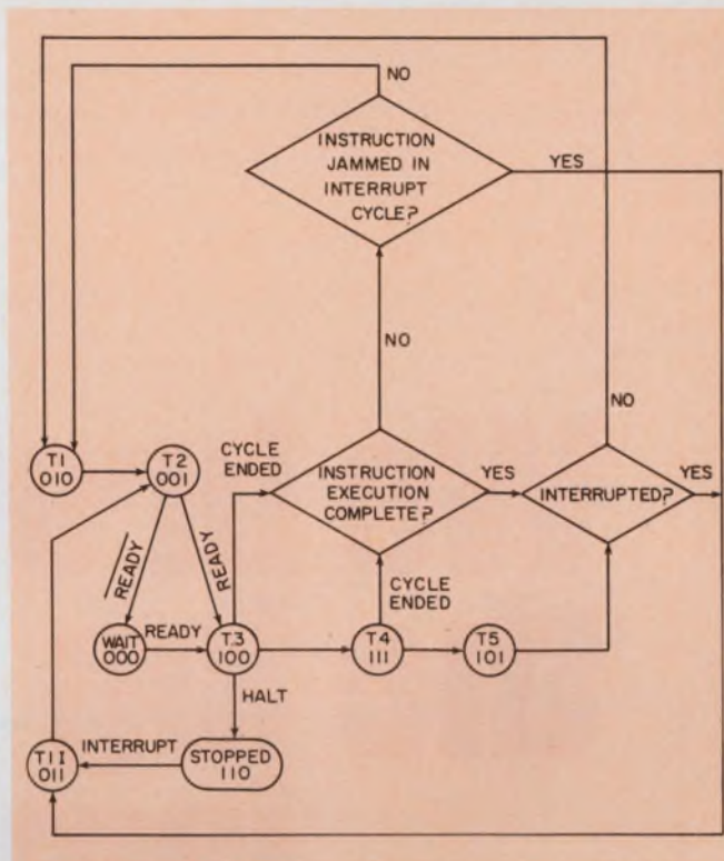
3. Each cycle causes microprocessor state transitions. A cycle begins when status lines indicate state T_1 .
