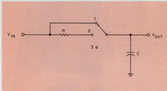
7. An ideal slow opening switch can be modeled by using a simple RC network and a three position switch.
