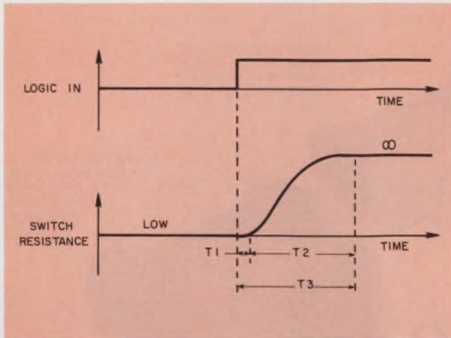
6. A typical analog switch introduces a delay in the sample-to-hold transition.
