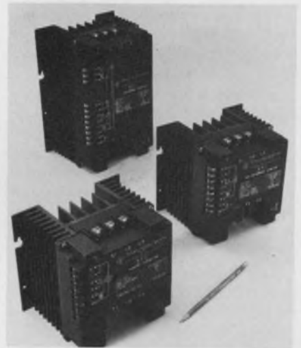
Solid-state motor control relays from Texas Instruments use transformer coupling to provide isolation.
