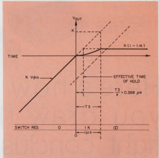
8. The effective time at which hold commences occurs before the switch is fully opened.
