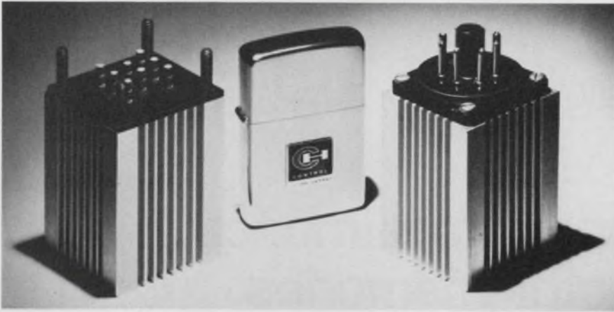
Reed-isolated solid-state relays from Cutler-Hammer can handle up to 8 A. A heat sink type can be used to dissipate internally generated heat.
