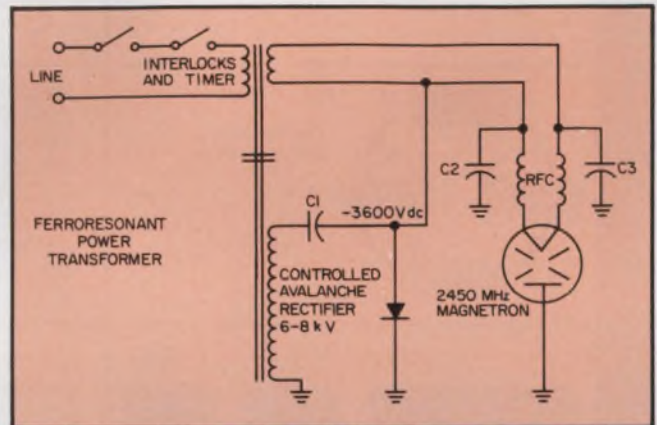
1. A controlled-avalanche rectifier eliminates the need for a separate filament transformer and delay timer in the high-voltage section of a microwave-oven magnetron power supply.
