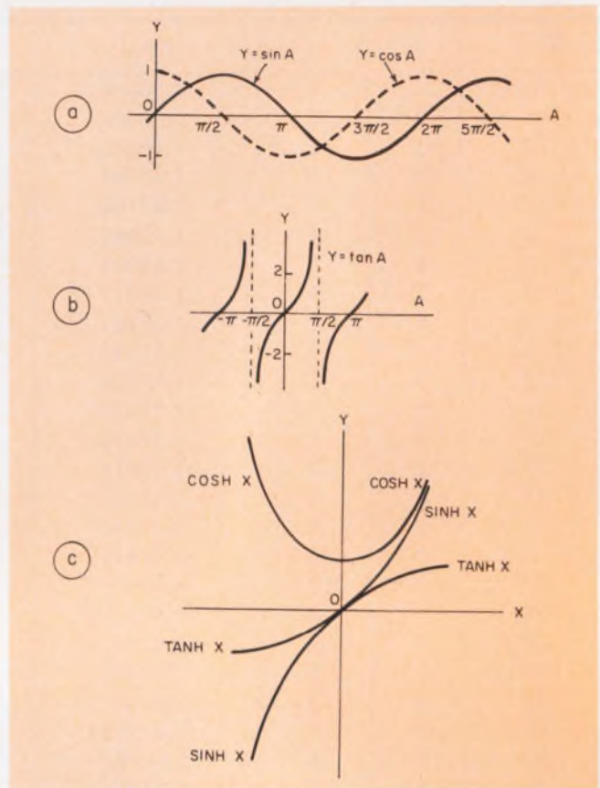
2. Plots of sines and cosines (a), tangents (b) and their hyperbolic counterparts (c), unlike their equations, bear little resemblance to one another.
