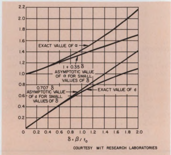
3. Specification of bandwidth divided by center frequency permits graphical determination of dissipation factor ( 1/Q ) and geometrical ratio ( \alpha ) of the two staggered center frequencies, f_0\alpha and f_0/\alpha .
