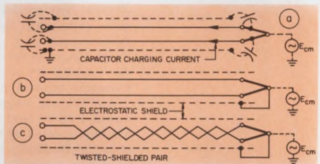
2. Shielding and single-point grounding reduces capacitive pickup. Improper grounding is shown in (a) and (b) is correctly grounded. Twisting the lead pair (c) with the shield reduces inductive pickup in the lead loop.
