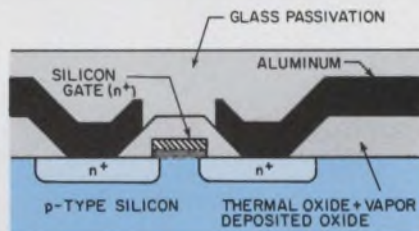
NMOS transistors using silicon-gate technology are being used by most manufacturers of NMOS large-scale integrated circuits.
