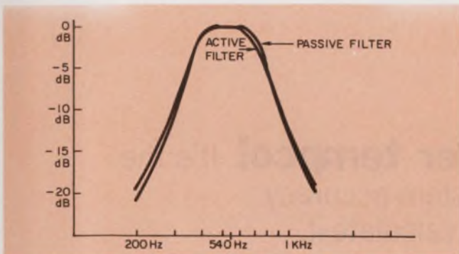
4. Active filter response compared with the original bandpass prototype, \beta = 350 Hz; f_o = 540 Hz, shows a nearly perfect Butterworth response.
