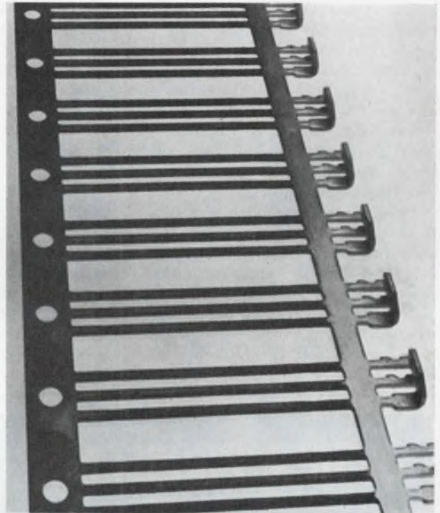
Gold-plated transistor lead frame. (Stamped part)
