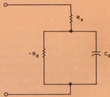
3. The domain capacitance, C_{dl} , of an active gallium arsenide chip is voltage-dependent. In this equivalent circuit model, -R_d is the negative resistance of the diode, and R_s is the ohmic resistance of the material outside of the active area.
