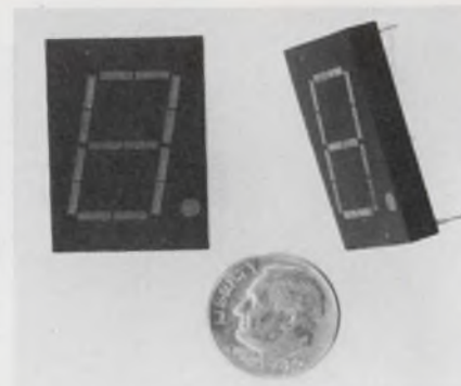
Seven-segment LED display has 0.77-in.-high characters—largest yet.
