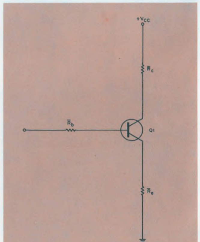
4. The stability of I_{c2} over temperature is indicated quantitatively by Eq. 21. It describes this simplified input stage in which all circuitry is reduced to Thevenin equivalents connected to the input transistor.
