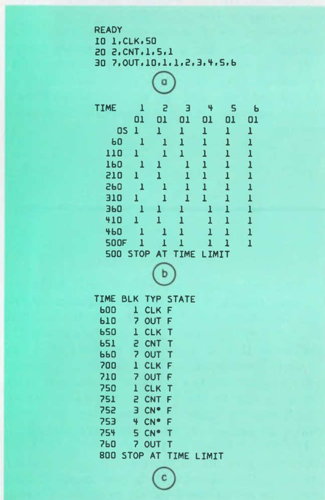
5. This is a LOGIC simulation of a clock (block 1) with a delay of 50 time units, a five stage counter (blocks 2-6) and an output block (7) with a delay of 10 time units. (a) is the data input. (b) is a print-out of the time and the states of blocks 1-6 at each time the output changes starting at 0 time and ending at 500 time units. Any other time period could have been specified. (c) is a printout of the times any changes of state occur starting at time 600 and ending at time 800. In this mode, the time of an event, the number of the block in which it occurs, the type of block involved and the new state of the block are given.
