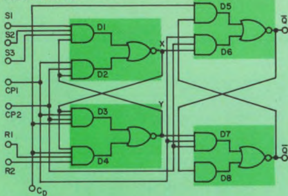
LOGIC DIAGRAM
