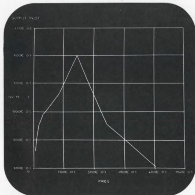
17. Here L=80 \mu\text{H} , and the resonance is more pronounced. Note that, although the frequencies to be plotted are logarithmically related, the frequency scale is linear. ECAP does not plot frequencies on a log scale.
