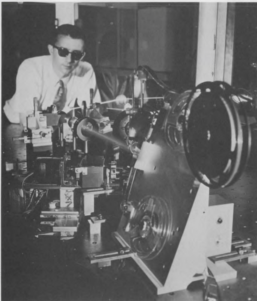
The laboratory setup for making a master holographic tape of a motion picture film for RCA SelectaVision. The movie film coming from the reel at the right is illuminated by a laser beam.
