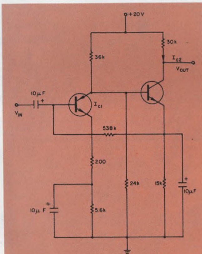
5. A current-feedback pair amplifier using a 2N2060B dual transistor has an I_{c2} drift of about 88 nA/°C, only a 4.5% change from the 250 \mu A collector current from 25°C to 150°C. The kHz voltage gain is 76 dB.
