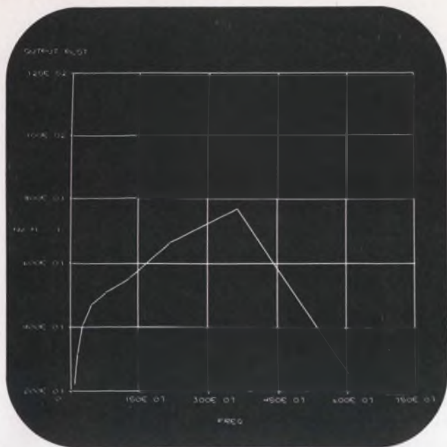
16. The inductance of branch 13 is now increased to 40 \mu\text{H} , giving this response.
