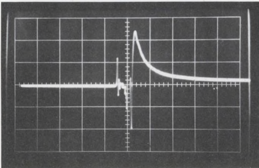
Self-contained $69 10-bit d/a converter displays an output settling time of 750 ns. The spikes shown are produced by command instrumentation.
