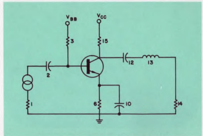
2. A single-stage transistor amplifier is the example selected for a graphic ECAP analysis. The numbers represent the branches of the final ECAP circuit. An R-L-C output network has been chosen to give a dramatic peaked frequency response.
