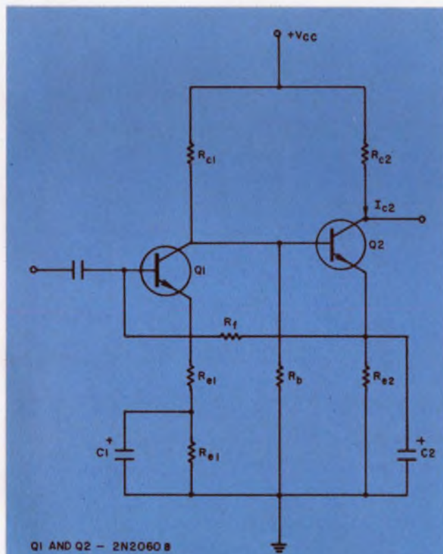
1. Dual npns form a current-feedback pair, in which part of the emitter current of Q2 is fed to Q1 for proper bias. Matched characteristics allow stabilization of the output current up to 150°C.
