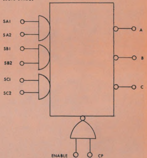
LOGIC SYMBOL
