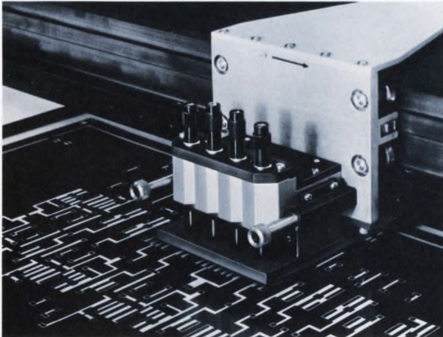
Integrated-circuit mask art work is automatically cut using a computer-driven plotter built by California Computer Products.
