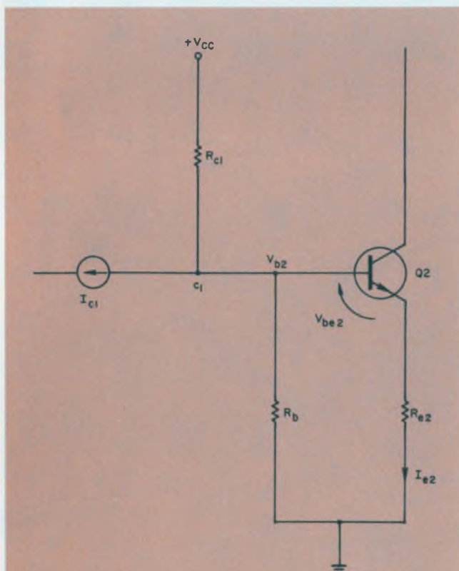
3. The dependence of I_{c1} on I_{c2} is explored by means of this circuit model. The expression for I_{c2} as a function of V_{be1} and V_{be2} is differentiated with respect to V_{be1} and V_{be2} to yield the stability factors \delta_c / \delta_{be1} and \delta_c / \delta_{be2} .
