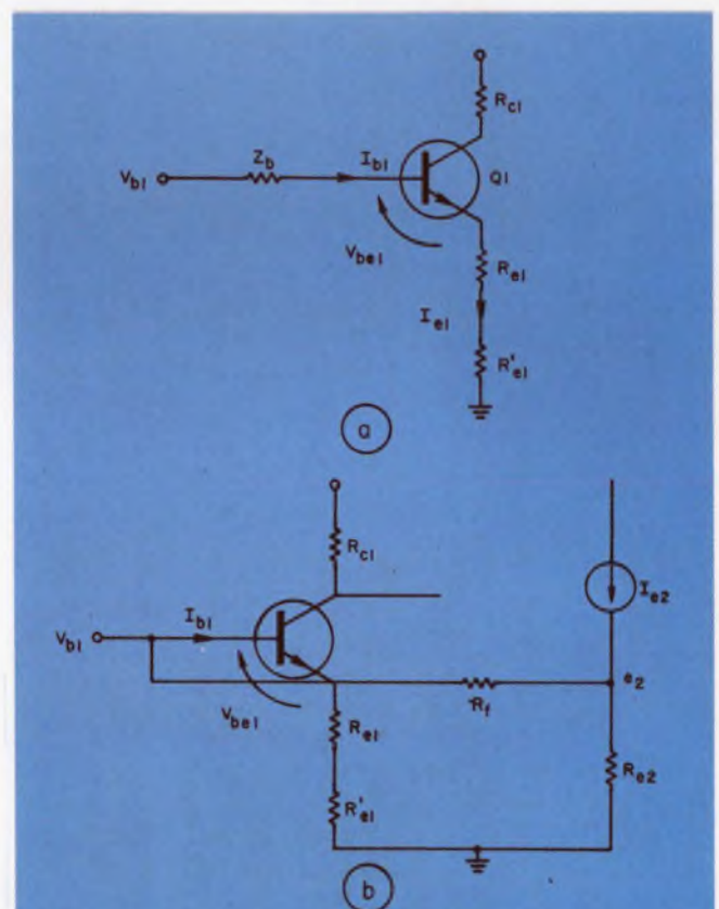
2. Loop equations are derived for the base-emitter circuit (a) and the feedback pair (b) and are solved for I_{c1} and I_{c2} . The stability factor is obtained by differentiation.
