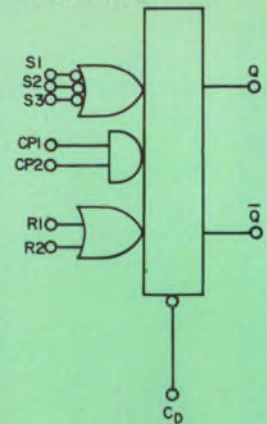
LOGIC SYMBOL
