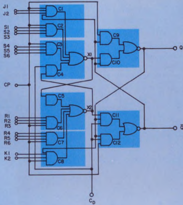
LOGIC DIAGRAM
