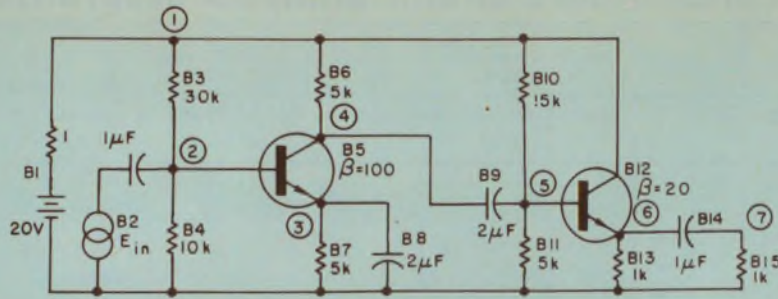
BASE CIRCUIT
