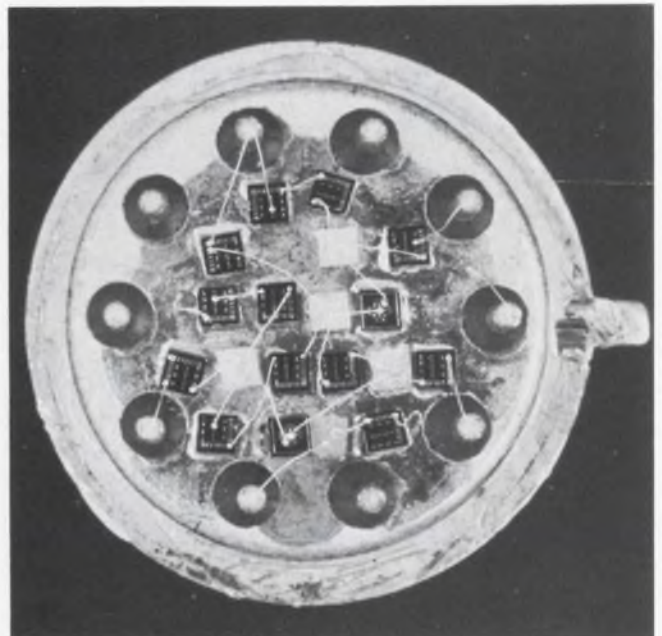
Resistors are diffused into the chips on this multichip header. The resistor chips have many bonding pads, one for each pick-off point. The other two chips are transistors.
