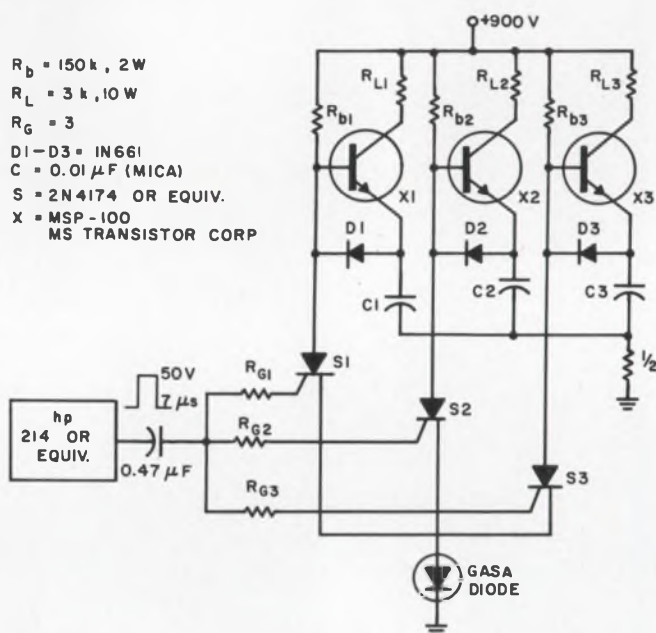
300-A, 80-ns pulses needed to operate a GaAs laser are delivered by this three-parallel-stage circuit at 10 kHz.
