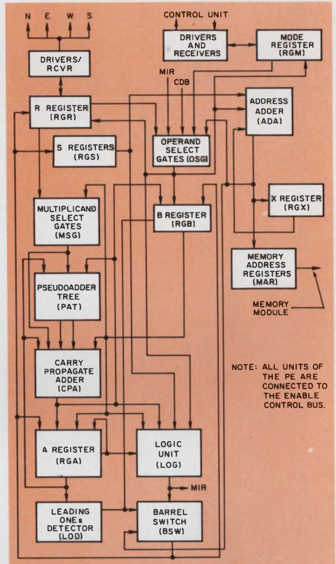
7. The processing element has three principal registers. It will be built from 64-pin ECL logic packages. Instruction execution times are typically 200 ns for floating point add and 400 ns for floating point multiply.
