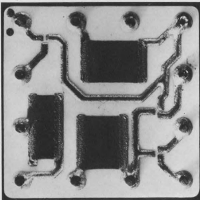
Untrimmed resistors adorn the circuit (left), which is made for an IBM computer. IBM trims down the resistors' values by an automatic sandblast technique (right). This gives the
