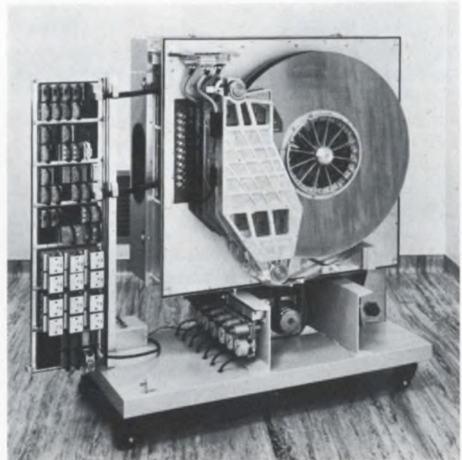
4. The principal secondary storage will be a parallel disk file similar to the current model of Burrough's head-per-track disk file (shown here). Transfer rates will be up to 500 million bits per second.
