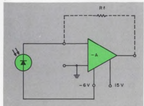
Simplified diagram of the HAD-130 shows the externally mounted feedback resistor.
