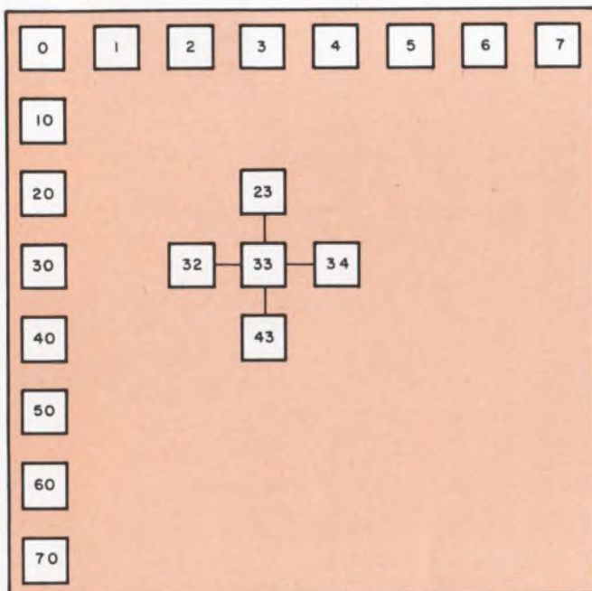
3. Direct parallel word transfers between processing units are only allowed between nearest neighbors. The transfers are maintained for both separate and joined quadrants. Note the octal numbering system.
