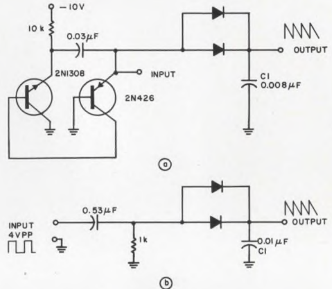
Sawtooth is obtained when a sine, square, or triangular waveform of 4-V pk-pk is applied to the input (a). For square waves the circuit reduces to (b). Two diodes are used to lower output resistance to increase rise time.
