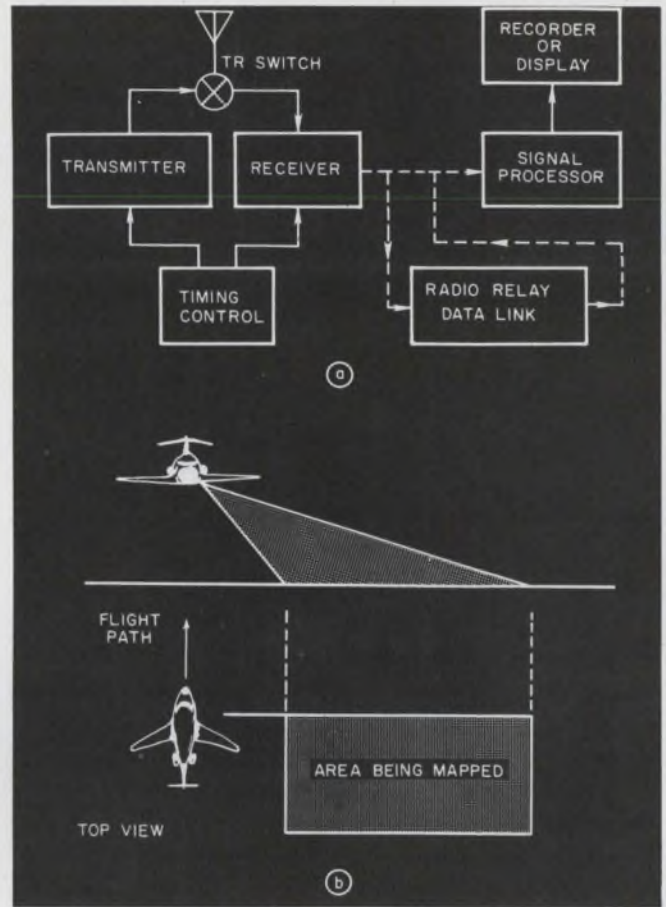
1. Side-looking radar mapping system is based upon a pulsed-Doppler radar, which makes use of a synthetic aperture system and pulse compression and correlation techniques, to achieve a fine mapping resolution (a). The mapping geometry is shown in (b).
