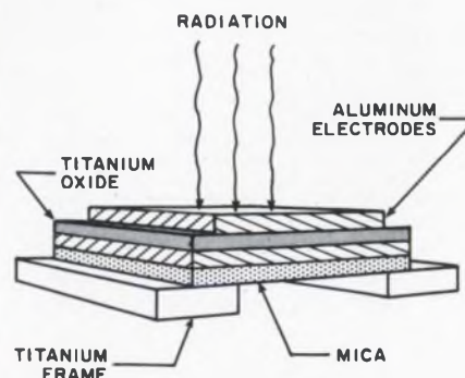
The capacitive bolometer, developed by Jet Propulsion Laboratory, is bonded to a supporting mica film over a hole in a titanium frame.
