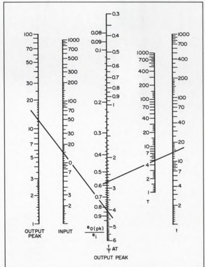
4. Nomogram for finding absolute values.
