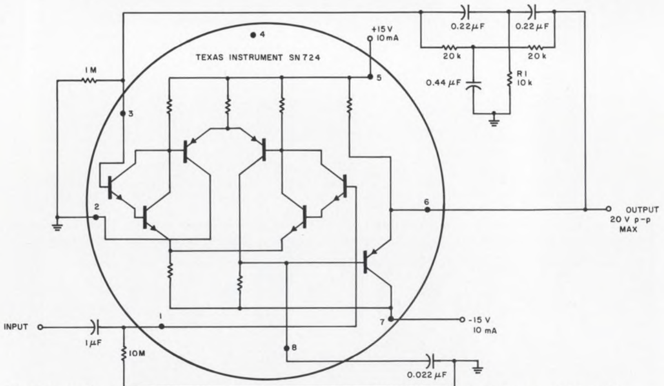
A 3-dB bandwidth of about 0.5 Hz at a center frequency of about 36 Hz is obtained from this simple notch amplifier.
