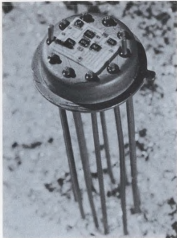
Photodiode op amp for full-spectrum detection in a TO-5 can. Page 114.
