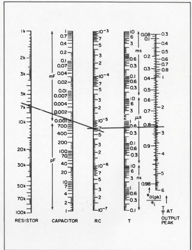
3. Nomogram for finding voltage and time ratios.
