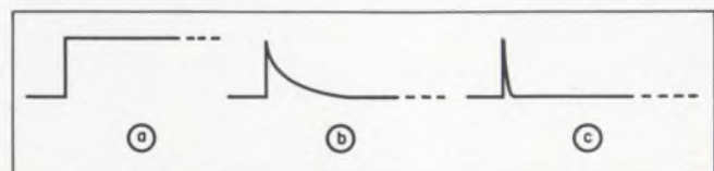
2. The input step (a) is differentiated by the circuit in Fig. 1a. Large RC products yield long trailing edges (b), small RC products have sharp skirts (c).
