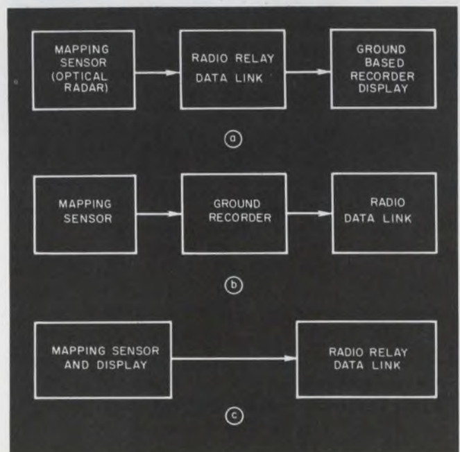
2. The mapping system may be 'boxed' into three stages (a), which can be reduced to a two-stage cascaded-amplifier equivalent (c). This presentation is permitted because the recorder, or display, is really a part of the sensor apparatus (b).
