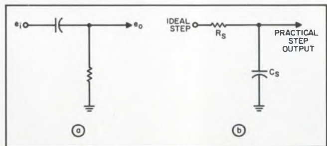
1. Passive RC differentiator (a) passes leading edge of step input but discriminates against a dc level. Equivalent circuit of stray resistance and capacitance (b) is really a lag network. The time constant is difficult to measure — it is easier to think of it as the time it takes the practical step function to reach 63.2% of its maximum value.
