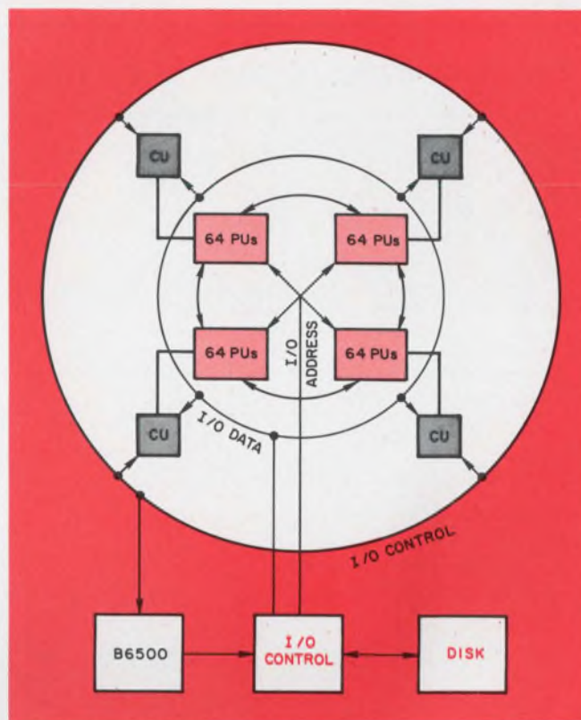
2. The basis of ILLIAC IV is four quadrants of 64 processing units under the command of four control units. Each PU is a computer with an individual thin-film memory of 2048 sixty-four-bit words.
