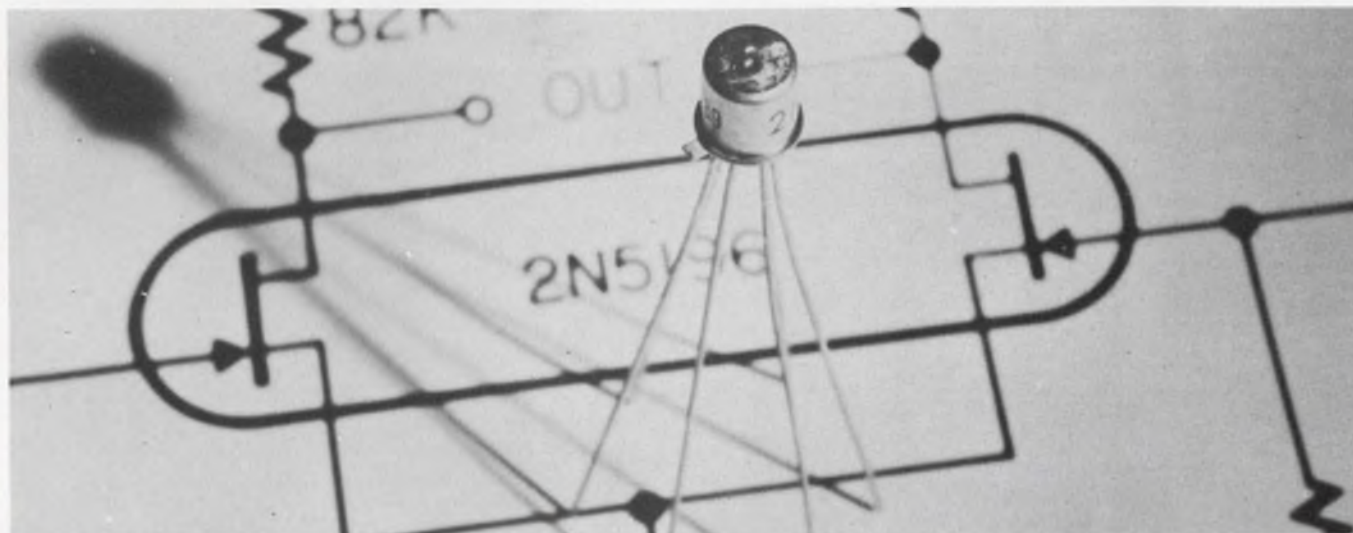
Matched FET-pairs track from 5\mu\text{V}/^\circ\text{C} with an input (gate) current of 15 pA. Page 116
