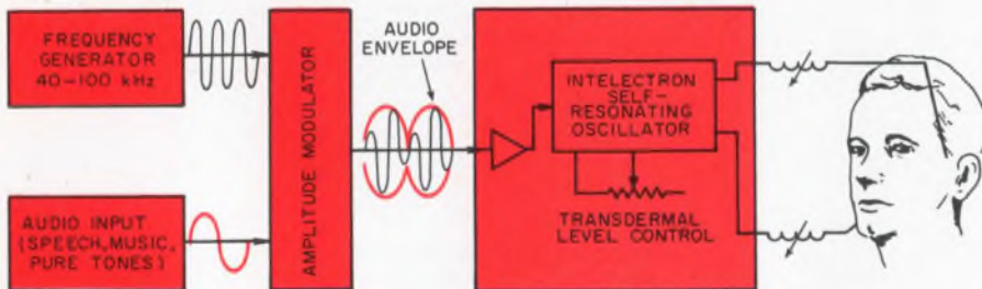
2. Device pumps rf signal into head and nerves demodulate the audio. Insulated electrodes act as plates of a capacitor, and tissues as the dielectric, in a series-resonant LC circuit. Unit handles speech as well as pure tones. Self-resonating oscillator adjusts to shifts in electrode placement.
