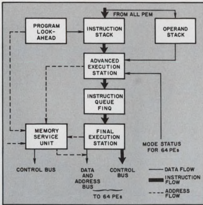
6. Generation of initial instructions and microsequences for each quadrant will be handled by a control unit. It will provide a queue of up to 128 instructions in a content addressable memory.
