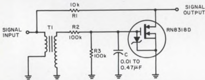
No power supply is needed for this simple volume compressor circuit.
