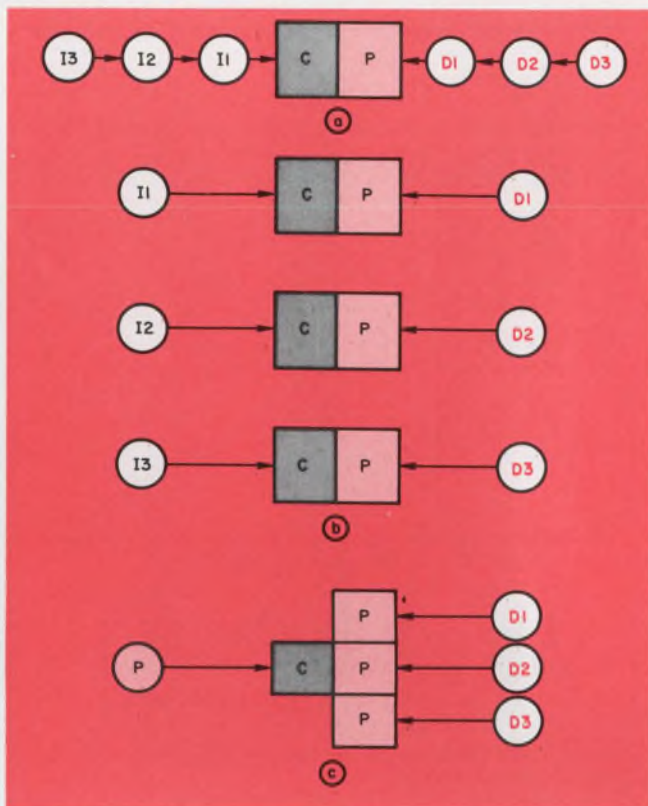
1. Development of parallelism began with the aim of improving the throughput of the pipeline computer (a). Simply paralalled identical processors (b) executing the same program could have common control logic (c).
