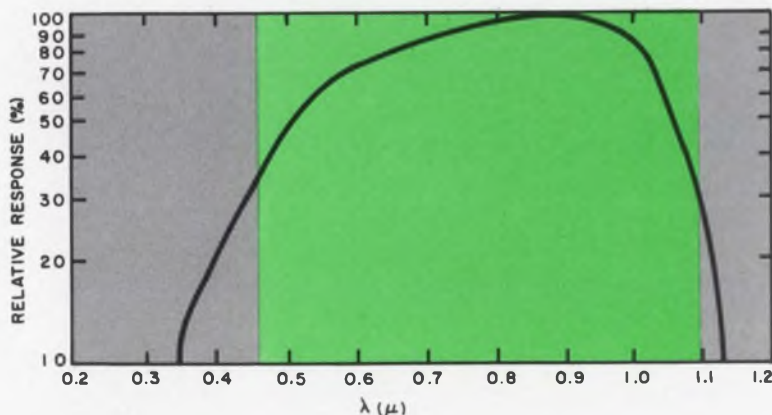
The response of the photodiode is 5 ns from 0.45 to 1.1 microns, or from the near ultraviolet to the near infrared.
