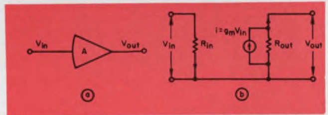
1. Three parameters. g_m , R_{in} and R_{out} , define the simplest building block (b). This simple amplifier may be regarded as a basic computing amplifier without summing and feedback impedances. (a).
