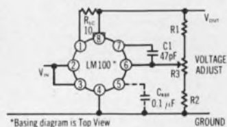
200mA Regulator
