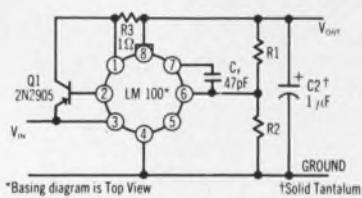
200mA Regulator
