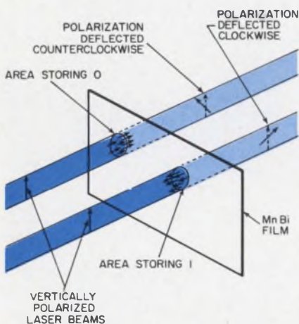
1. Faraday effect in a manganese bismuth film causes opposite rotations of a vertically polarized laser beam for stored ones and zeros.
