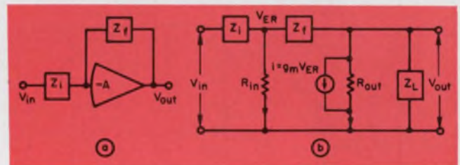
2. Independence of gain and output impedance are characteristic of an analog operational amplifier (a) when used with a computing network. The impedances of the network Z_i and Z_f complete the equivalent circuit of the operational amplifier (b).
