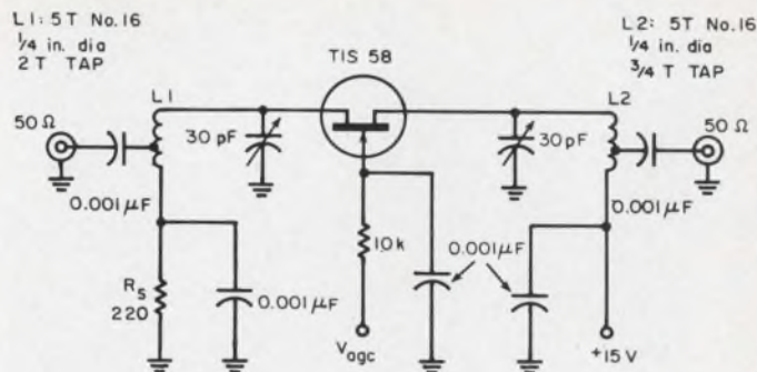
8. Common-gate configuration results in better agc characteristics but the initial gain is lower.
