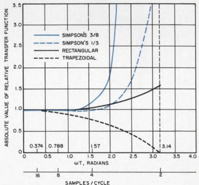
4. Relative transfer functions of various numerical integration methods are plotted against frequency and samples per cycle. These pinpoint the poles of the transfer functions—the gain shoots up to infinity. For example, Simpson's rule of 3/8 blows up at about 3 samples per second, or at 2.2 \omega T radians.
