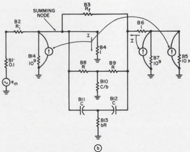
1. Twin-T active-filter (a) performance analysis by a computer reveals that both the bandpass frequency and filter gain deviate from the commonly used expressions. The ECAP computer model of the active filter is shown in (b).
