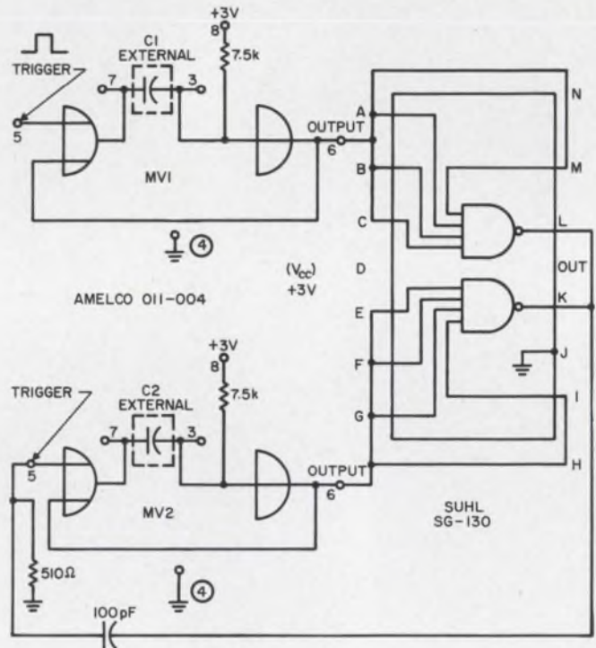
Adjustable pulse width generator uses three ICs and several discrete components.
