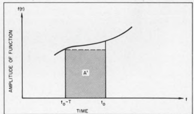
3. Integration with the rectangular rule involves approximation of the area under the curve by the shaded rectangle. This is the simplest numerical integration method.
