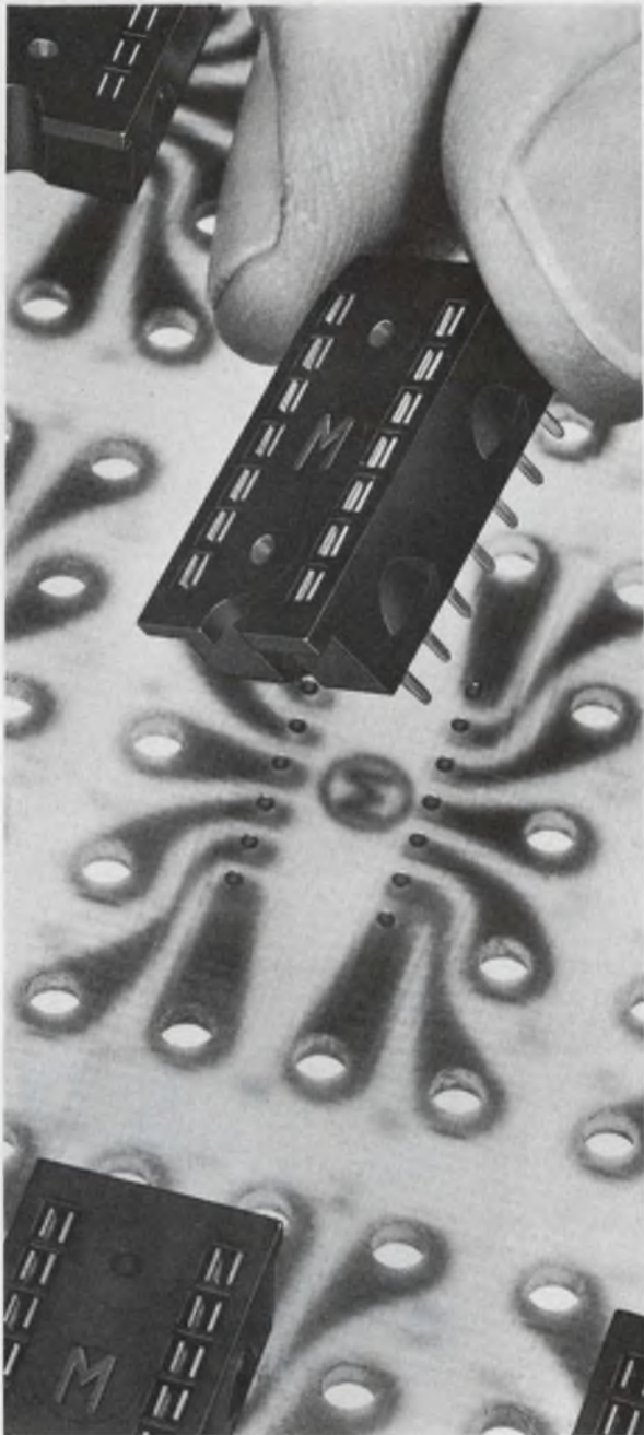
Dual-in-line IC sockets snap in PC boards of aluminum or epoxy glass. Page 92
