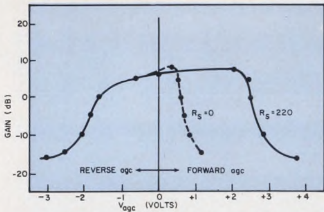
9. Agc characteristic for common-gate circuit of Fig. 8 indicates its superiority over those obtained in the common-source configuration of Fig. 3. Note the effect of the source resistor, R_S , on the forward agc curve.
