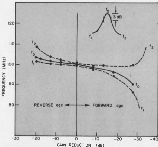
5. Increase in bandwidth occurs for both types of agc because drain-to-gate capacitance, C_{dg} , is a function of gain.
