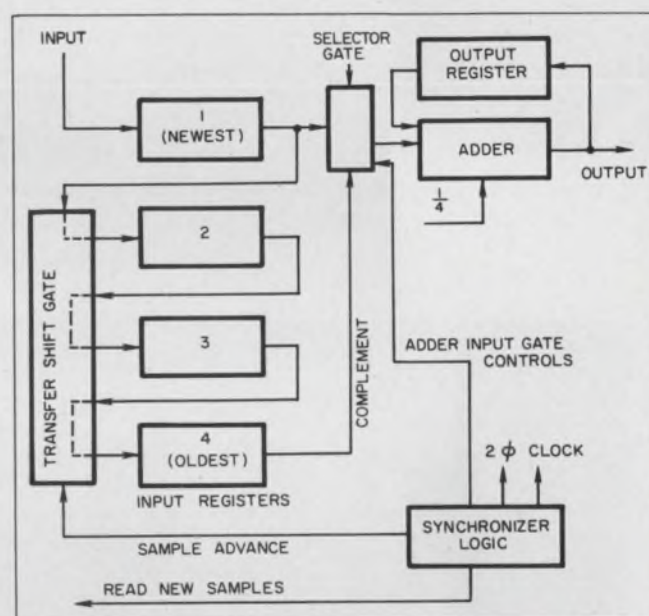
7. Logic diagram of an arithmetic averager uses four samples, updates the average and reads out the result in four steps.
