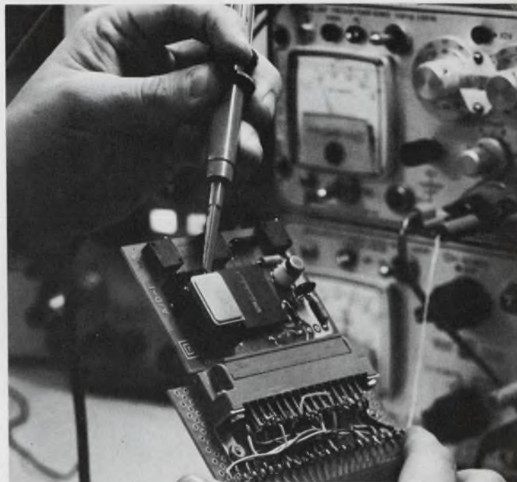
1. At the tip of the probe is the monolithic chip of General Instrument Corp., built into a 10-bit analog-to-digital converter.
