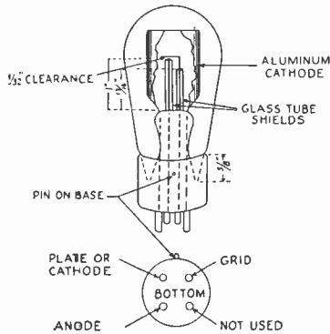
A sectional view of the new relay tube, showing the placement of the elements. Note the small clearance between the grid and the anode.
