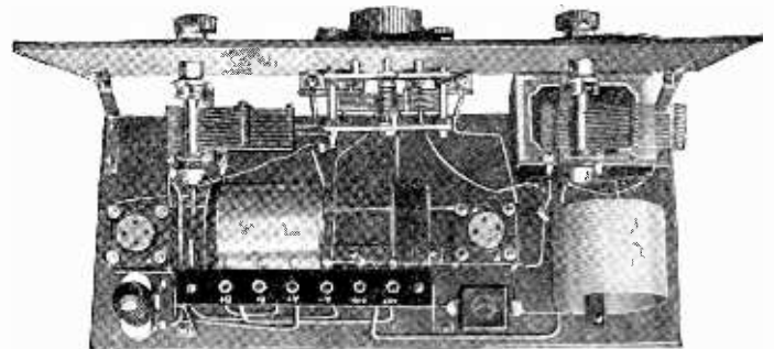
Fig. 2. Here is shown the set with the cabinet removed. The various parts are clearly seen. The variable grid leak is mounted on the base board because frequent adjustment is not necessary. Note that the C battery is incorporated in the cabinet. This is done to keep the leads short and because it is not necessary to replace it very often.
