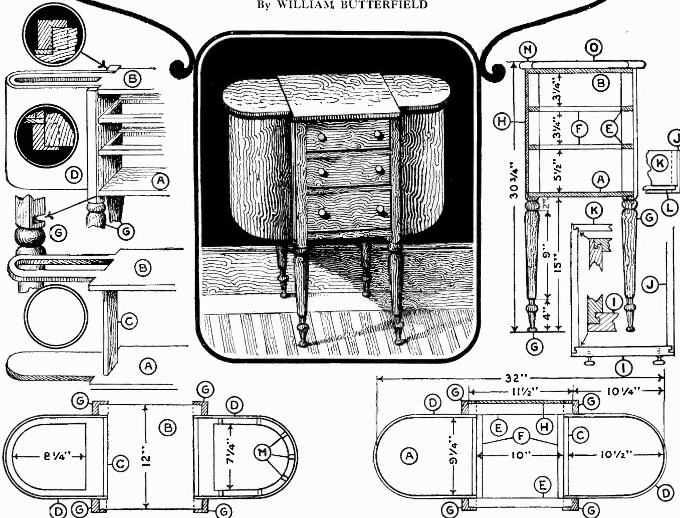
The constructional plan of the body of the sewing cabinet is shown above together with an end view.
