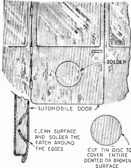
The above illustration shows clearly the method pursued in repairing a closed car body with an exterior patch.
