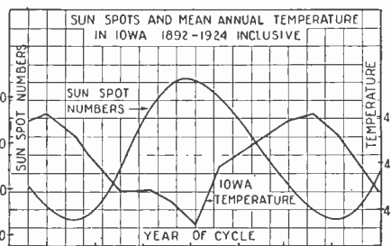
The curves above showing the variation of the Iowa temperature is from means of the Weather Bureau figures for the mean annual temperature of Iowa for the 33 years, 1892 to 1924, inclusive. The 33 years, 3 sun spot cycles, were averaged on one cycle of 11 years.
