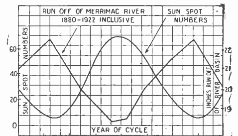
Curves above show run-off of Merrimac River from measurements taken at Lawrence, Mass., over a period of 43 years, averaged on one cycle of 11 years.
