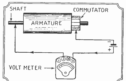
2183. For testing an armature for grounds the connections shown above should be followed. All ground connections should be removed beforehand.
