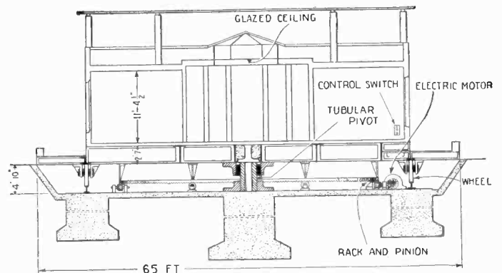
The living room of this strange house is shown above. In the center of the house there is a central court which admits the light through the rear windows of the rooms. Below is a side plan of the revolving house showing the position of the control switch and electric motor. The house turns upon a tubular pivot placed in the center.
