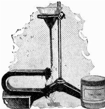
Iron filings mixed with sand or other foreign material are caused to drop past the poles of a magnet. This attracts the iron filings, effecting their separation from non-magnetic material.
