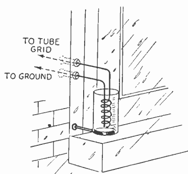
A drop of rain falling between the two wires offers a high resistance path for the grid charge to leak off to the ground.
