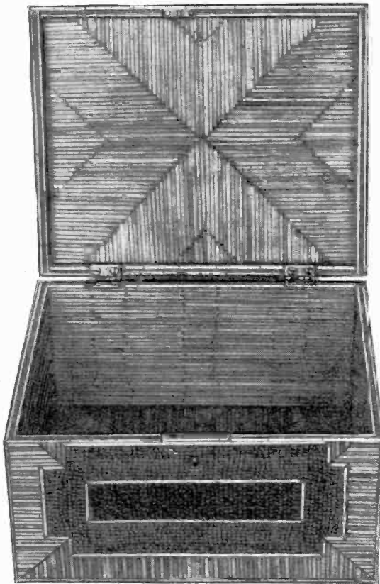
First Prize—$50.00 was won by C. Horte of Altamont, N. Y. The two views here show the construction of this humidor which was polished to a glass-like finish.
