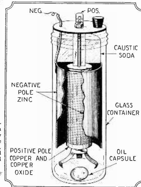
A view of the cell completely assembled is shown above. Note placement of caustic soda.
