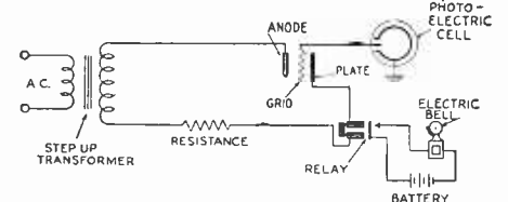
An ordinary photo-electric cell connected between the grid and the ground if exposed to light, will cause the tube to operate.
