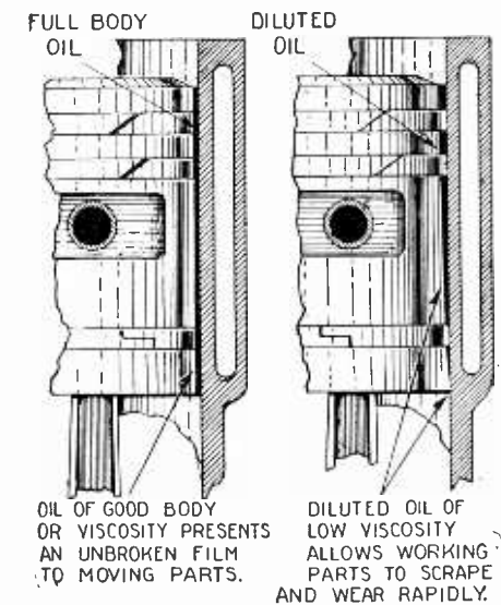
Excessive crankcase dilution causes the parts to wear rapidly.
