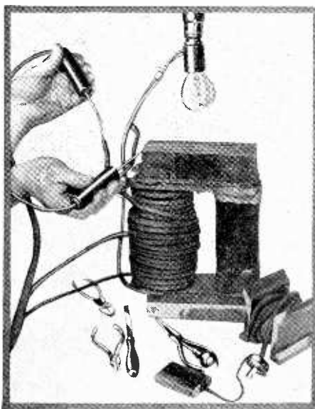
Testing the windings of a high voltage transformer for short, open and ground with the universal trouble shooter, is shown above.
