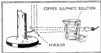
When using a microscope at night, a light comparable with the north light may be obtained with the arrangement shown above.
