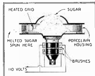
A diagrammatical view of the machine showing the sugar container and wiring to the 110-volt circuit.
