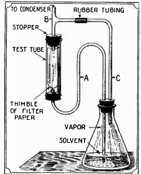
In this apparatus the solvent is evaporated, condenses and falls upon the substance contained in the cut-off test tube. When it fills it to the top the tube A is filled to its upper bend and acts like a siphon and draws all the solution back into the flask when the solvent is evaporated again.
