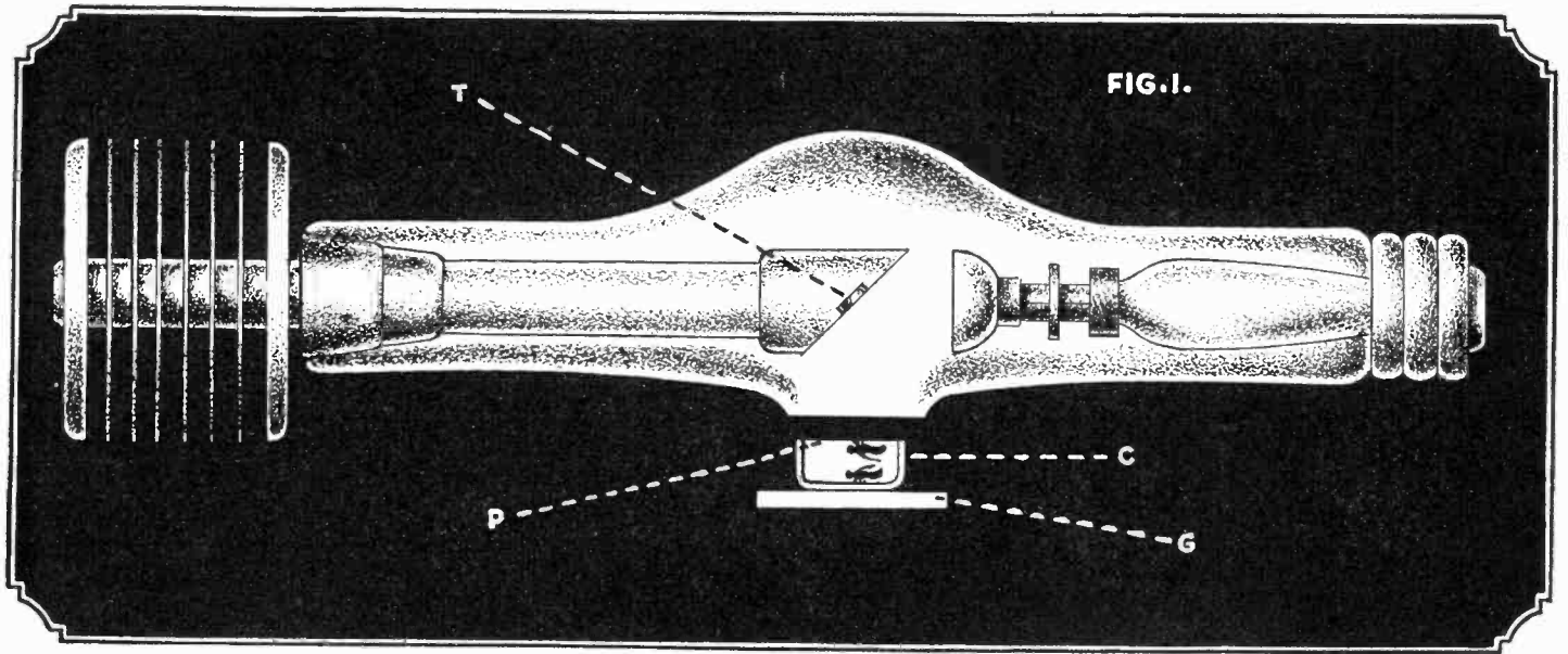
The method of exposing the flies to the X-rays is shown above. T is the target, C small glass cup, P paper cup and G a glass plate.
