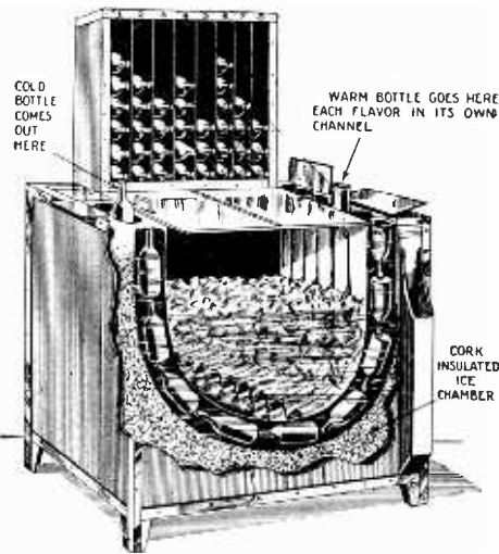
Above is a sectional view of the bottle cooler. Each flavor has its own channel which will accommodate a number of bottles at a time. The ice is placed in the center of the cabinet. The ice chamber itself is insulated with cork. At the back of the cabinet is a space which provides for the storage of additional bottles. —Liquid Carbonic Co.
