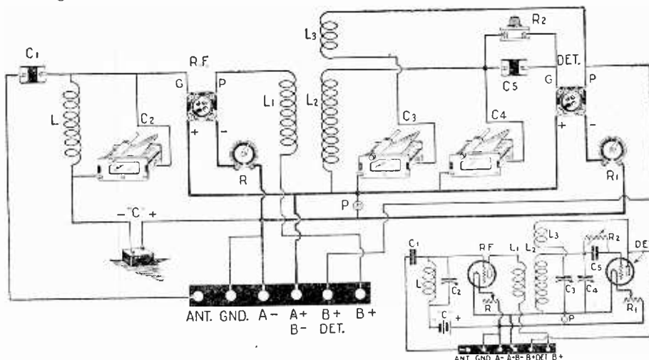
Fig. 5. The circuit diagram of the receiver is illustrated above. The schematic diagram is also shown. The Weagant "X" circuit is used, because of the sharp tuning that it is possible to get with this type of receiver.
