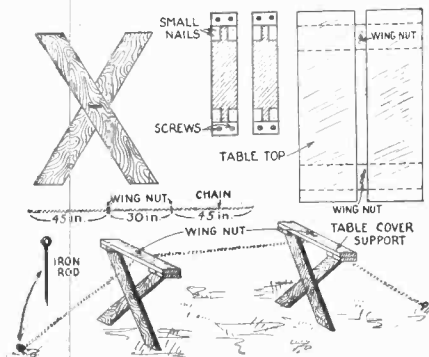
The constructional details of the table and supports are given above. The supporting chain is held secure by two iron rods.
