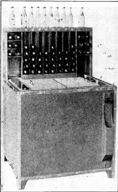
Above we have a view of the bottle servitor or liquid bottle cooler. The cabinet remains entirely closed on the top except for a small opening on either side. The bottles are inserted in the opening at the right and are ejected from the opening at the left.
