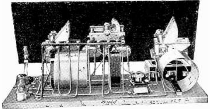
Fig. 3. Celluloid-supported coils and the position of the three variable condensers are clearly shown in this photograph. Note also, the arrangement of the panel to leave room for the variable condensers. The terminal strip is also shown in this photograph.
