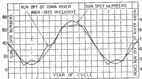
Graph above shows run-off of the Iowa River based on measurements taken at Iowa City, Iowa. The results for 22 years, 2 sun spot cycles, are averaged on one cycle to make this graph.
