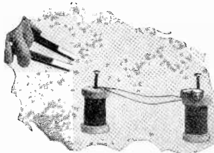
Connecting two coils as shown, an ordinary compass will show the production of a current, when a magnet is brought near a heavy nail which stands in the center of the coil. The action is intensified by the action of a second nail in the other coil.
