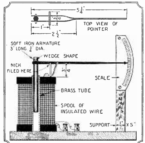
A very sensitive electric meter is shown here, which according to its winding, will act either as a voltmeter or an ammeter. The illustration shows very accurately the different parts and a very sensitive instrument can be constructed on the lines indicated.
