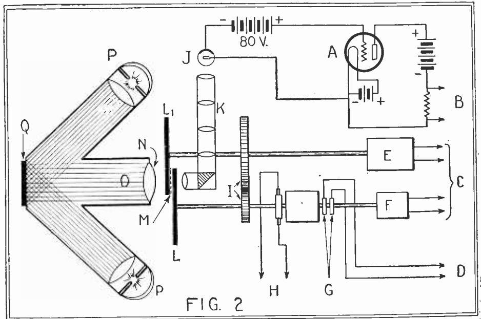
The diagram of the televisor is shown here. The various components of the circuit are as follows: A, amplifying tube; B, circuit to the amplifying battery; C, circuit of the coils of the magnetic reflecting fields; D, lines to the telephone circuit; E, 8-cycle alternator; F, 800-cycle alternator; G, rings connecting to the two points of the motor field coil; H, 110-volt circuit; I, gearing; J, photo-electric tube; collimator; LL1, disks; N, lens; O, beam of parallel light rays; P, arc light; Q, object to be transmitted.
