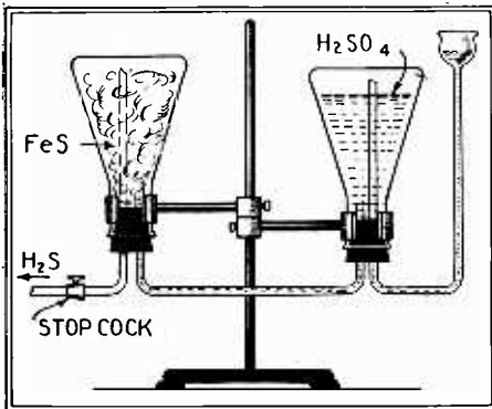
This useful sulphuretted hydrogen apparatus will be found far superior to the ordinary common bottle and funnel tube arrangement, for this is really automatic. Too much acid should not be put in the right-hand bottle.
