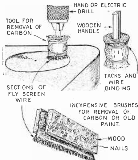
The various forms of brushes used for the removal of carbon and old paint are shown in the above illustration.
