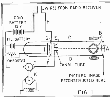
The cathode-ray tube apparatus is shown here. A, cathodic point; B, deflecting magnetic fields; C, path of the gas; D, cathodic emission; E, plate; F, grid; G, filament; J, 800-volt D.C. generator; K, motor.
