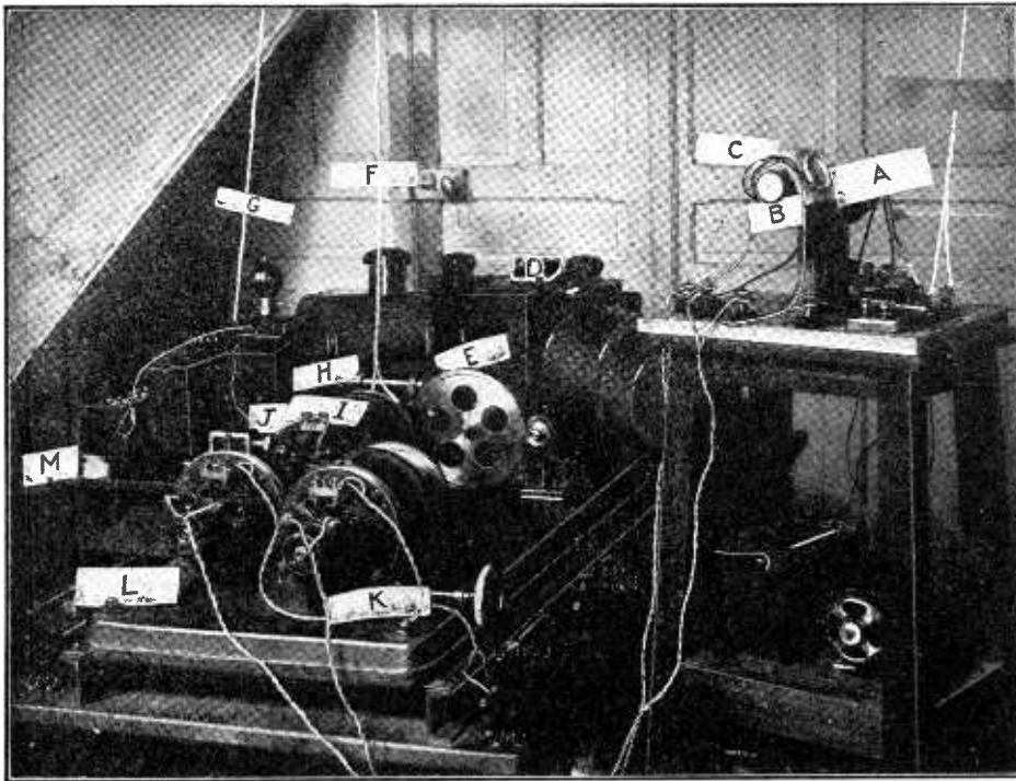
The television apparatus used by Monsieur Valensi, chief engineer of French Post Office, is shown above. The apparatus used is labelled as follows: A, receiving lamp; B, fluorescent screen; C, coils of the magnetic field; D, reflection apparatus; E, explorer disks; F, synchronizing circuit; G, receiving circuit; H, collimator; I, synchronized motor; J, photo-electric cell; K, 8-cycle alternator; L, 800-cycle alternator; M, amplifier. Monsieur Valensi is much more ambitious in his desires and achievements than most of his contemporaries, looking farther into the future.
