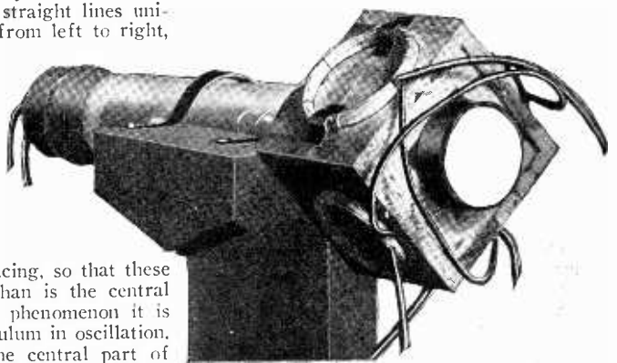
This illustration shows the Cathode-Ray Tube, fluorescent screen, and the four coils which surround the extremity of the tube very near to the fluorescent screen. This unit comprises the apparatus used for projecting the received signal. The currents coming from the radio receiver, act upon the cathode emission of the tube.
